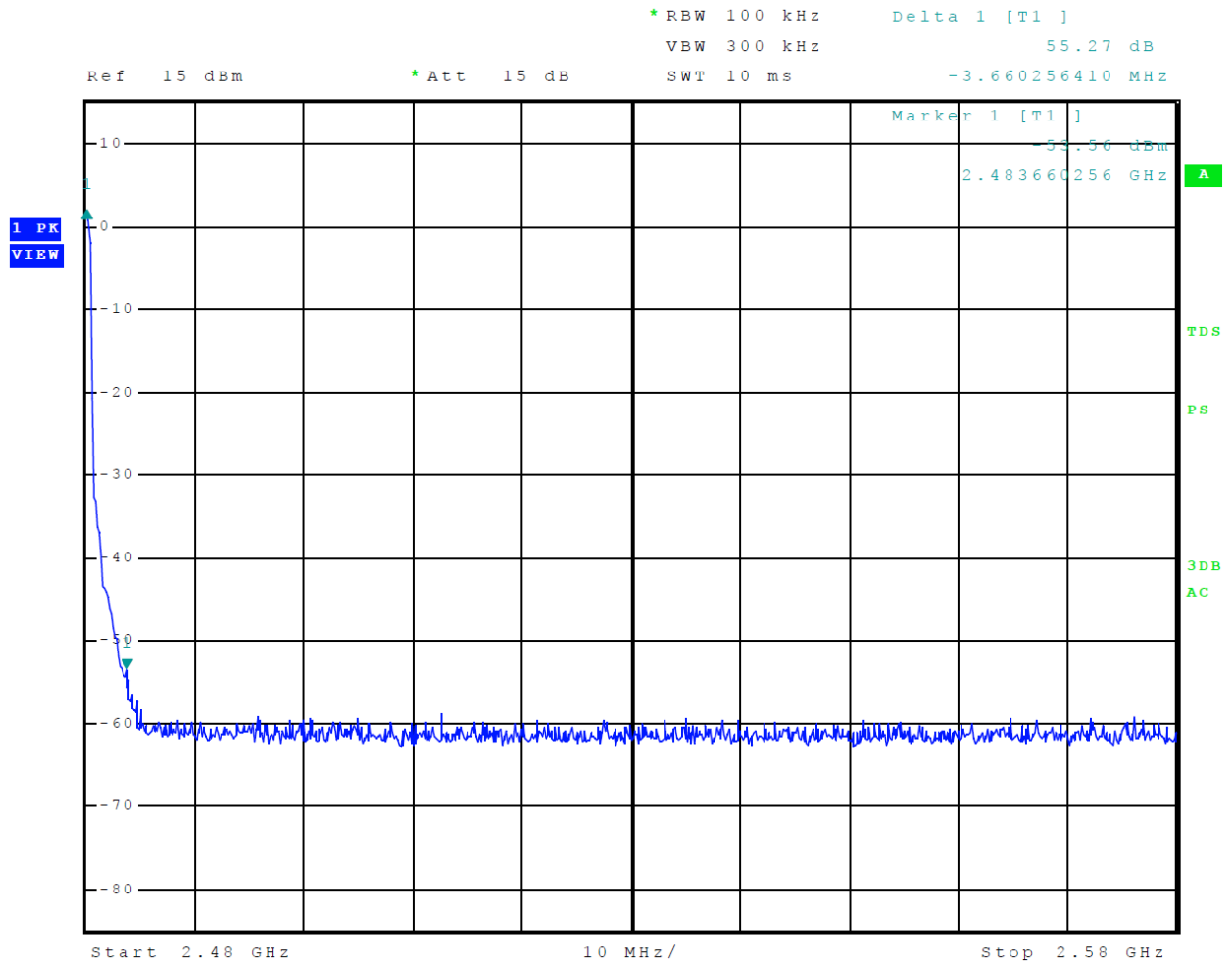
Figure 20 Plot of Transmitter Emissions High Band Edge Mode 4 BR 2EDR
