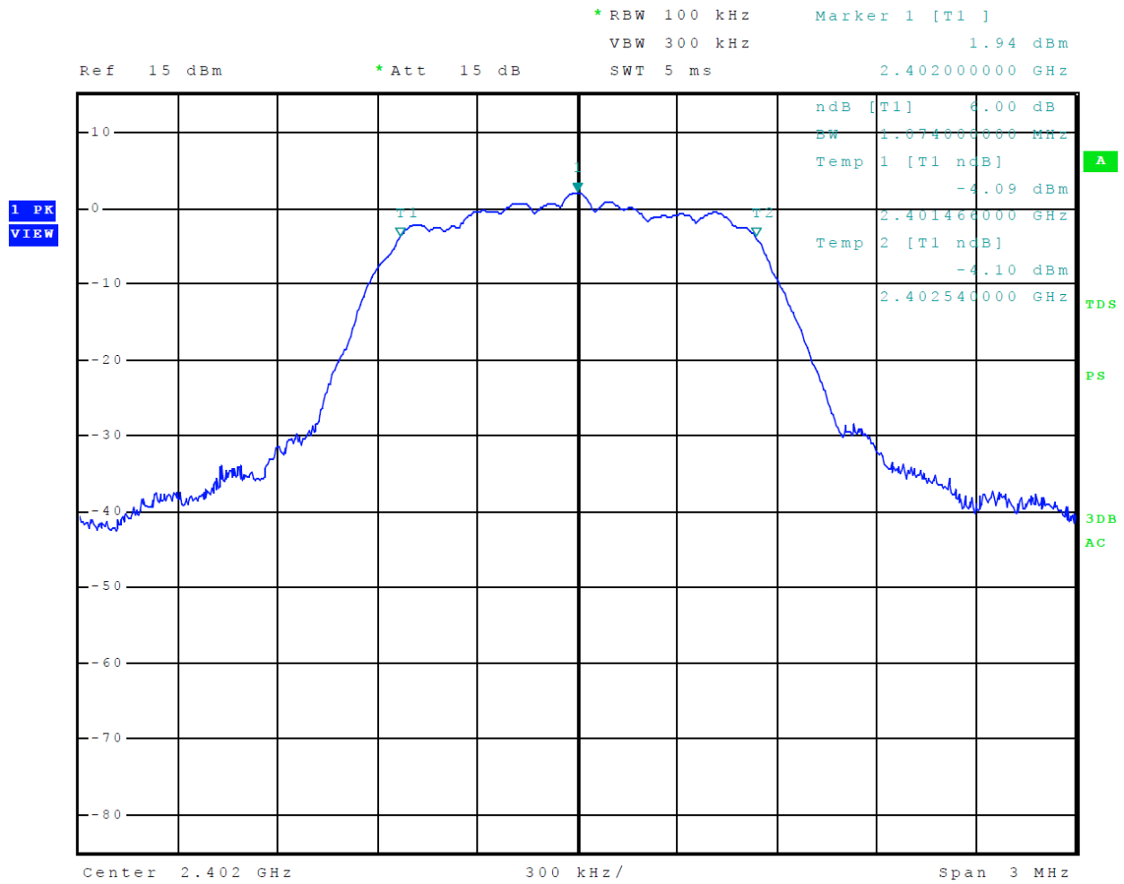
Figure 28 Plot of 6-dB Occupied Bandwidth Mode 4 BT 3EDR
