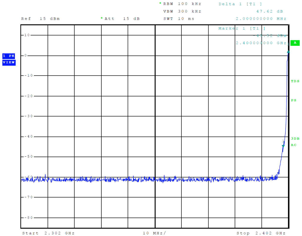
Figure 13 Plot of Transmitter Emissions Low Band Edge Mode 4 BT 3EDR
