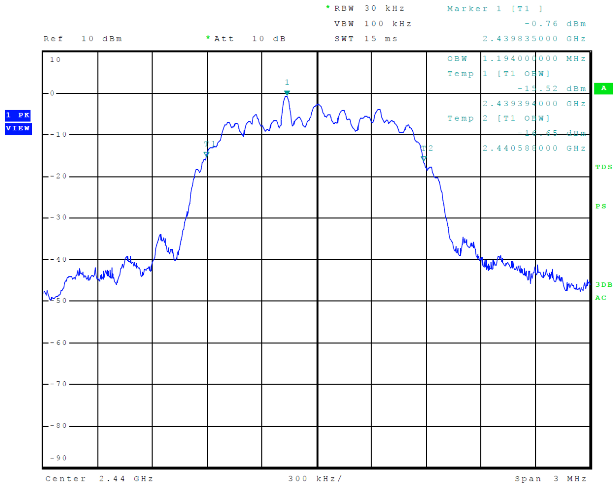
Figure 27 Plot of 99% Occupied Bandwidth Mode 3 BT 2EDR
