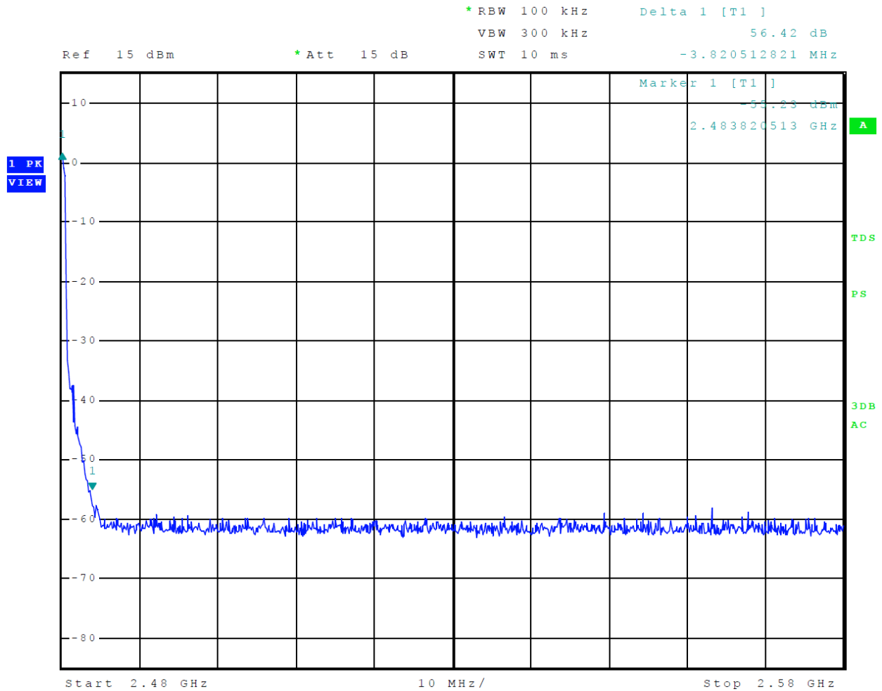
Figure 19 Plot of Transmitter Emissions High Band Edge Mode 3 BT 2EDR
