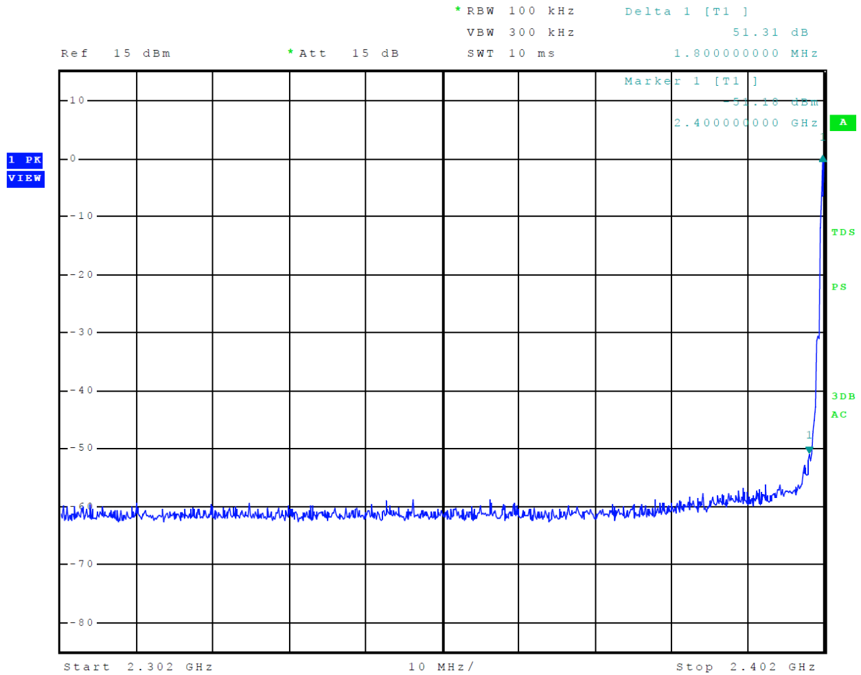
Figure 14 Plot of Transmitter Emissions Low Band Edge Mode 5 BT BLE
