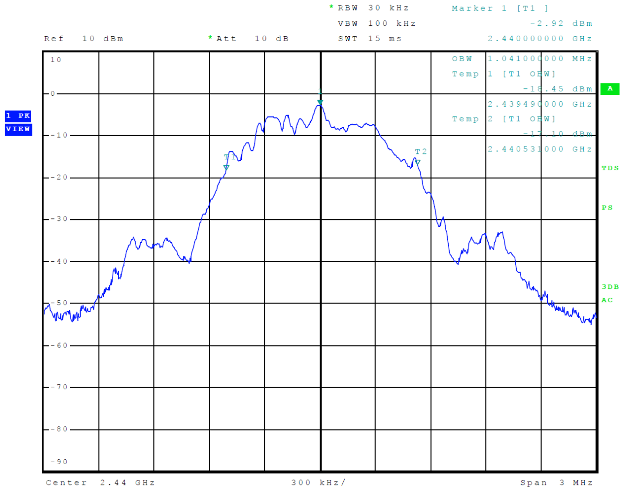
Figure 31 Plot of 99% Occupied Bandwidth Mode 5 BT BLE
