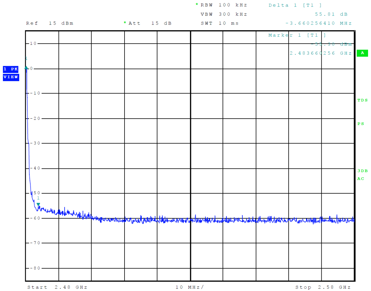
Figure 21 Plot of Transmitter Emissions High Band Edge Mode 5 BT BLE
