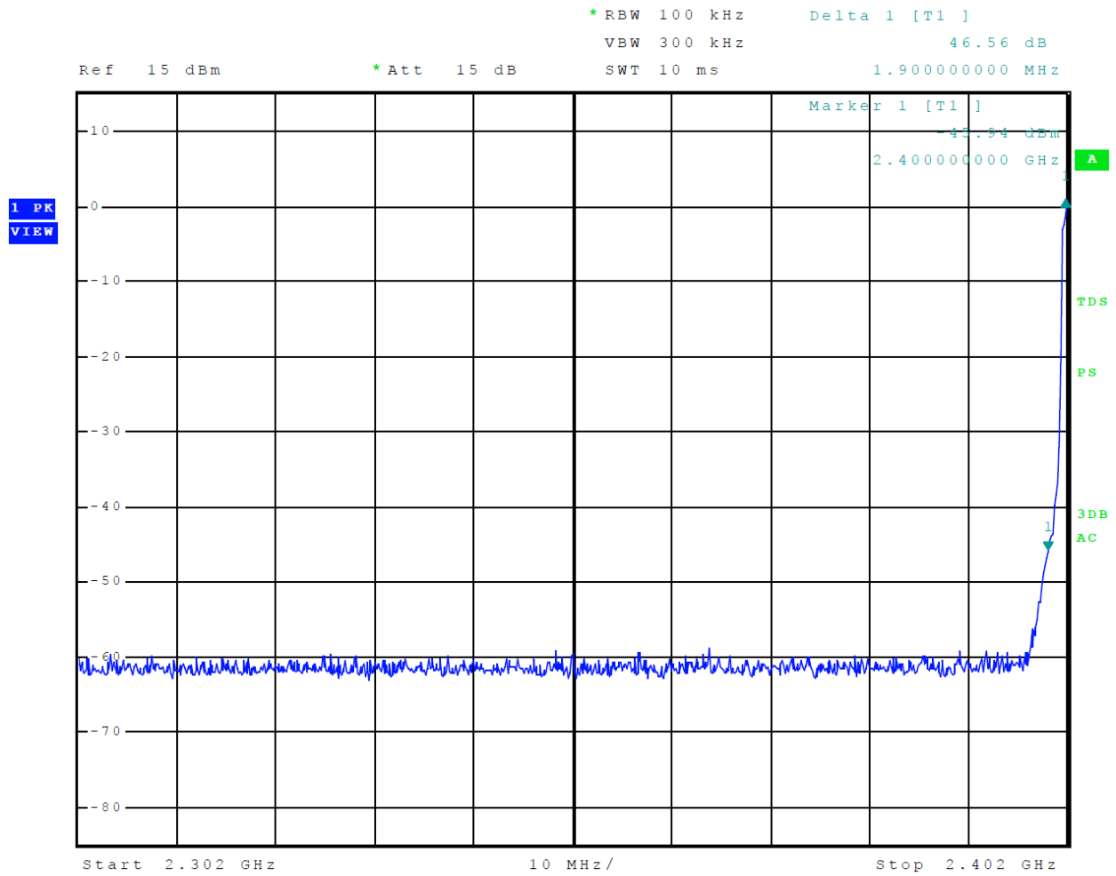
Figure 12 Plot of Transmitter Emissions Low Band Edge Mode 3 BT 2EDR
