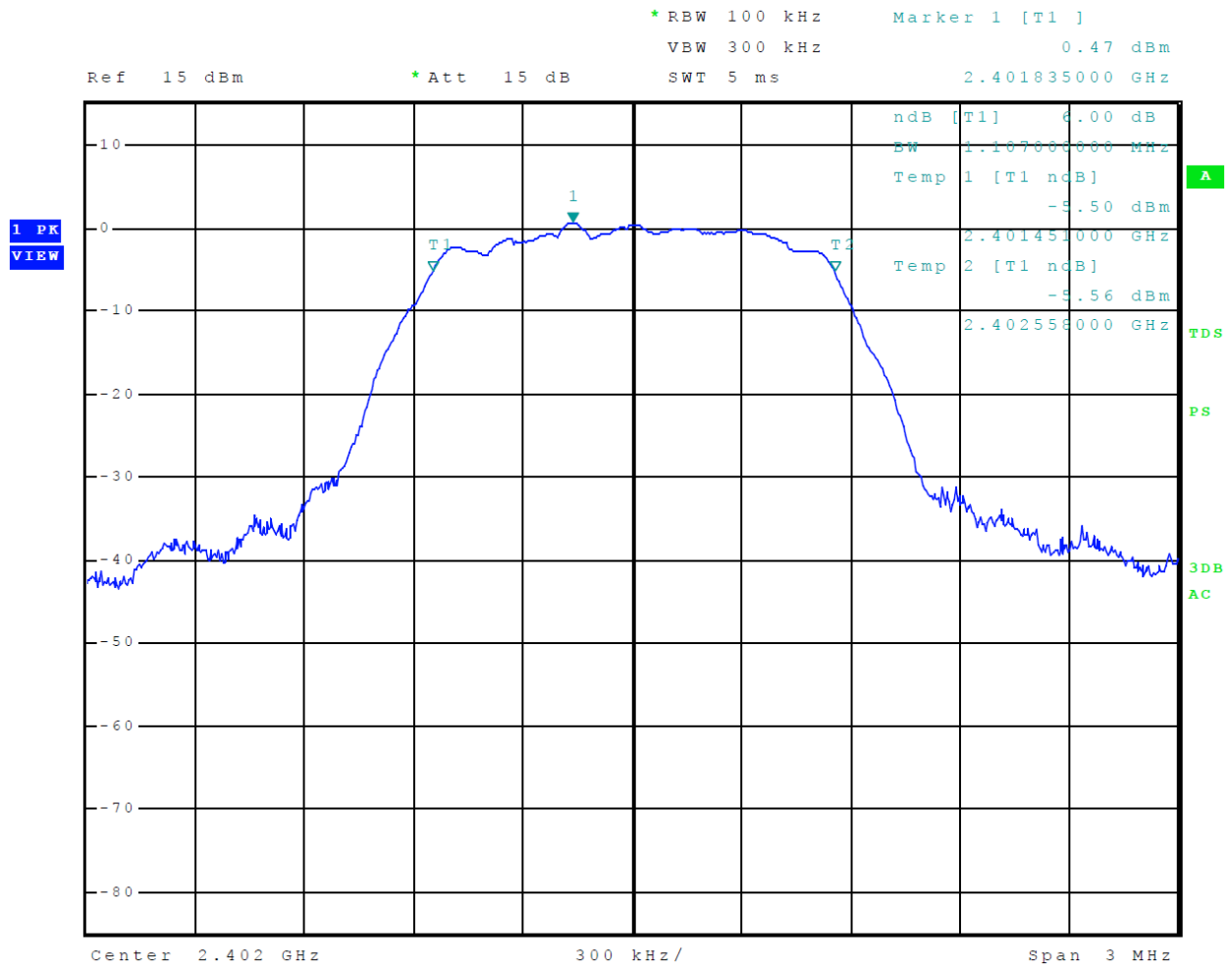
Figure 26 Plot of 6-dB Occupied Bandwidth Mode 3 BT 2EDR
