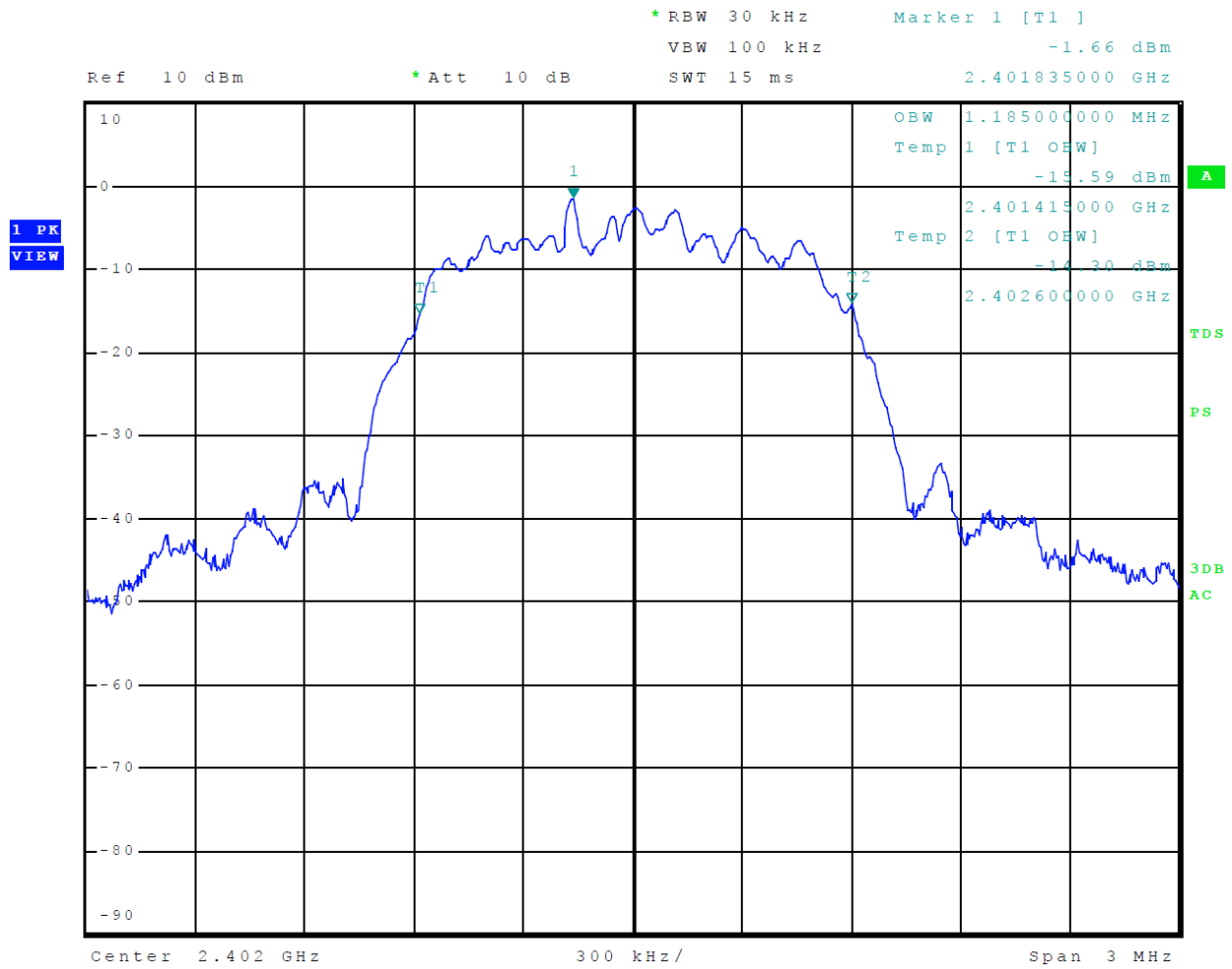
Figure 29 Plot of 99% Occupied Bandwidth Mode 4 BT 3EDR
