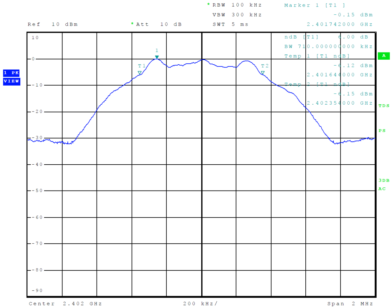
Figure 30 Plot of 6-dB Occupied Bandwidth Mode 5 BT BLE
