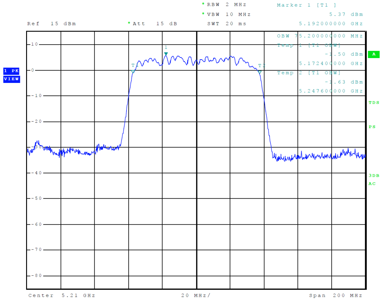
Figure 24 Plot of 99% Occupied Bandwidth 5150-5250 MHz Mode 13 U-NII-1 (802.11ac80)
