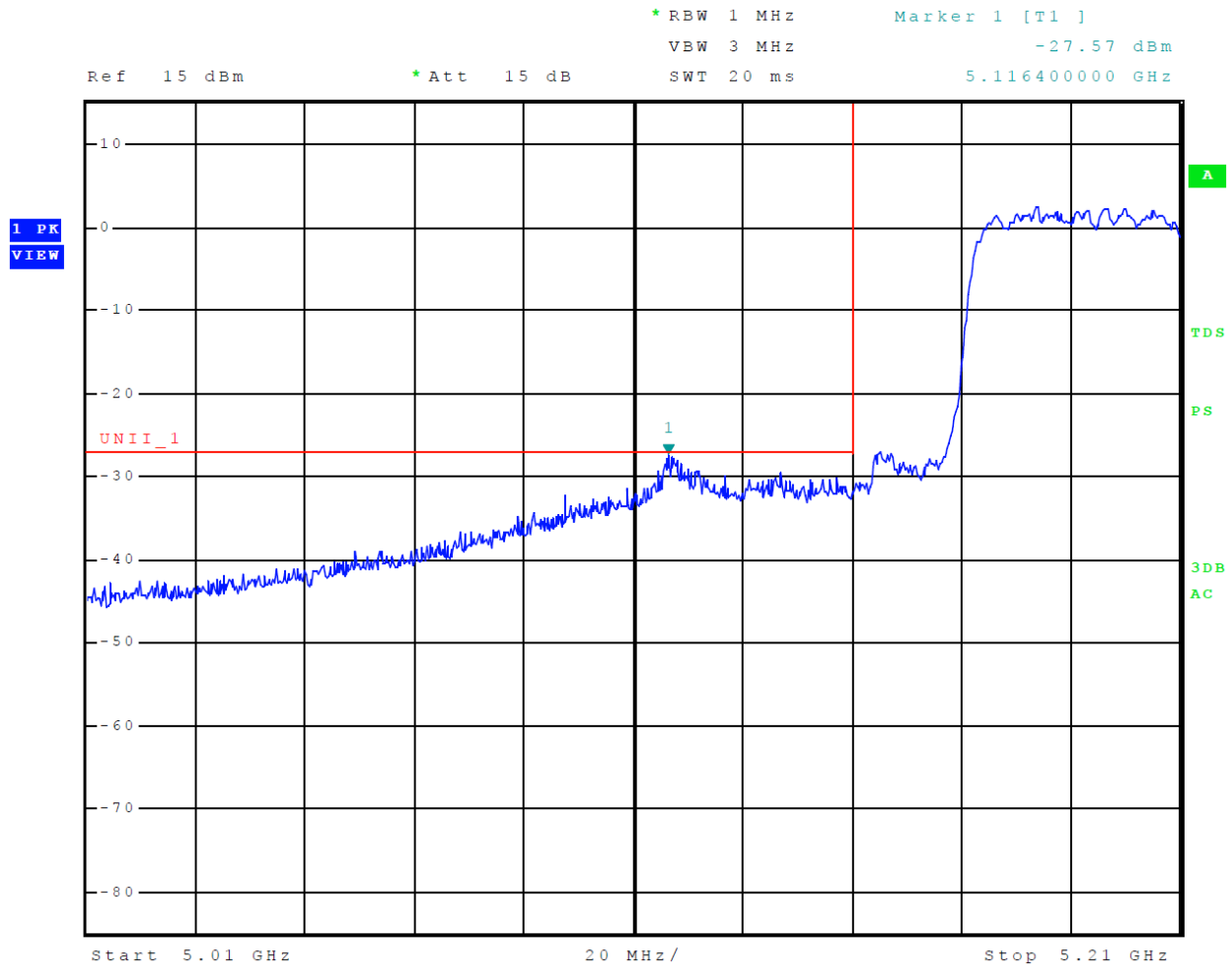
Figure 12 Plot of Lower Band Edge Across 5150-5250 MHz Mode 13 (802.11ac80)
