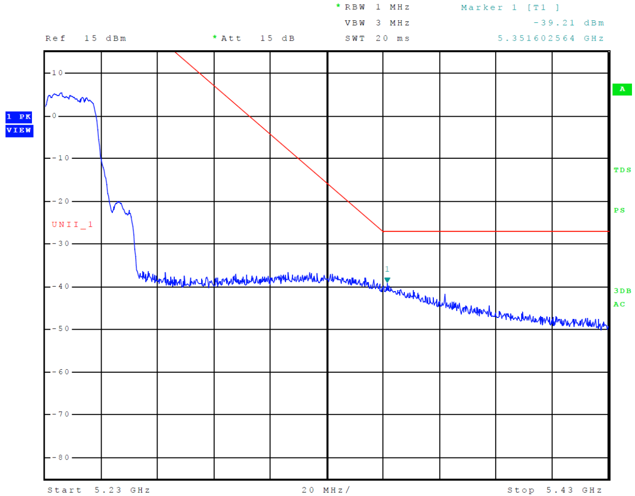
Figure 15 Plot of Upper Band Edge Across 5150-5250 MHz Mode 12 U-NII-1 (802.11n40)
