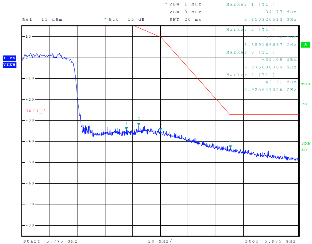
Figure 36 Plot of Upper Band Edge Across 5725-5850 MHz Mode 17 U-NII-3 (802.11ac80)
