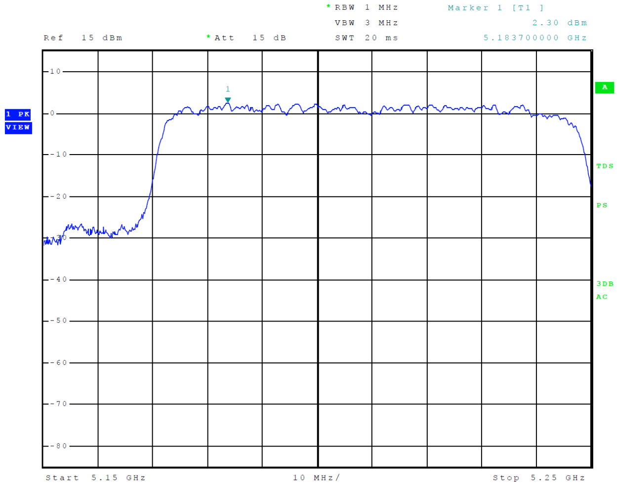
Figure 8 Plot of Transmitter Emissions Across 5150-5250 MHz Mode 13 U-NII-1 (802.11ac80)
