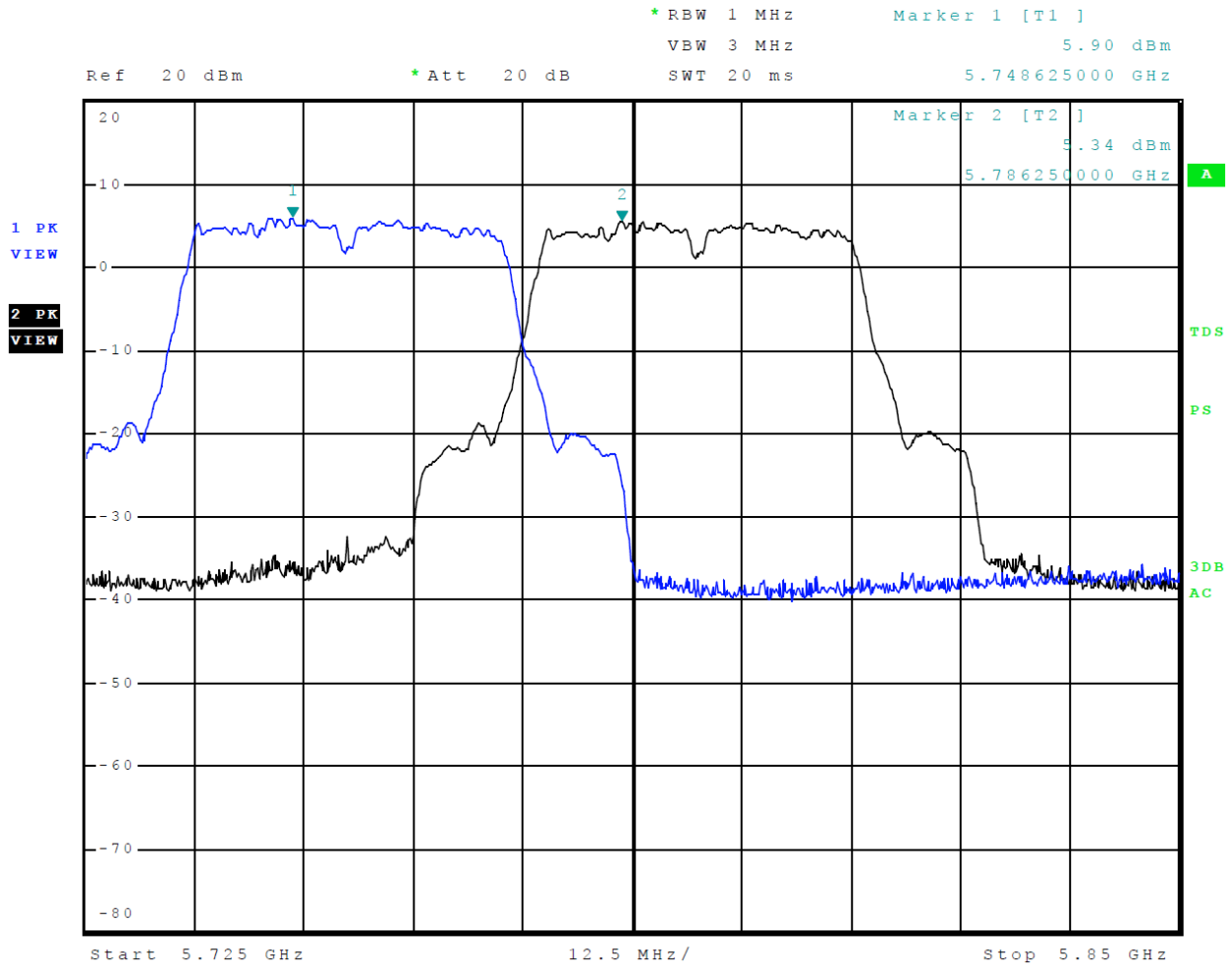
Figure 27 Plot of Transmitter Emissions Across 5725-5850 MHz Mode 16 U-NII-3 (802.11n40)
