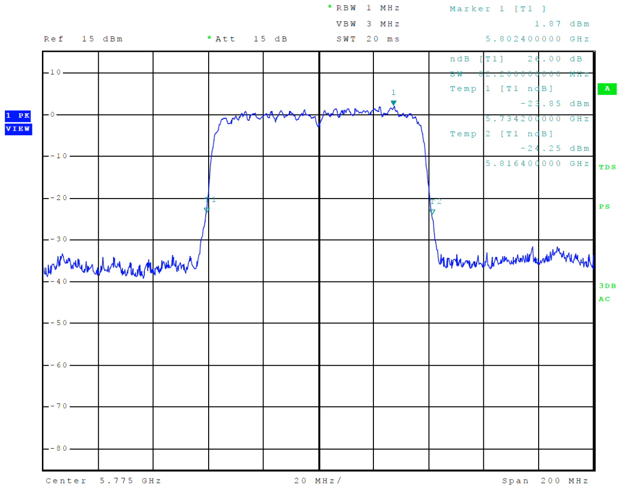
Figure 48 Plot of 26-dB Occupied Bandwidth 5725-5850 MHz Mode 17 U-NII-3 (802.11ac80)
