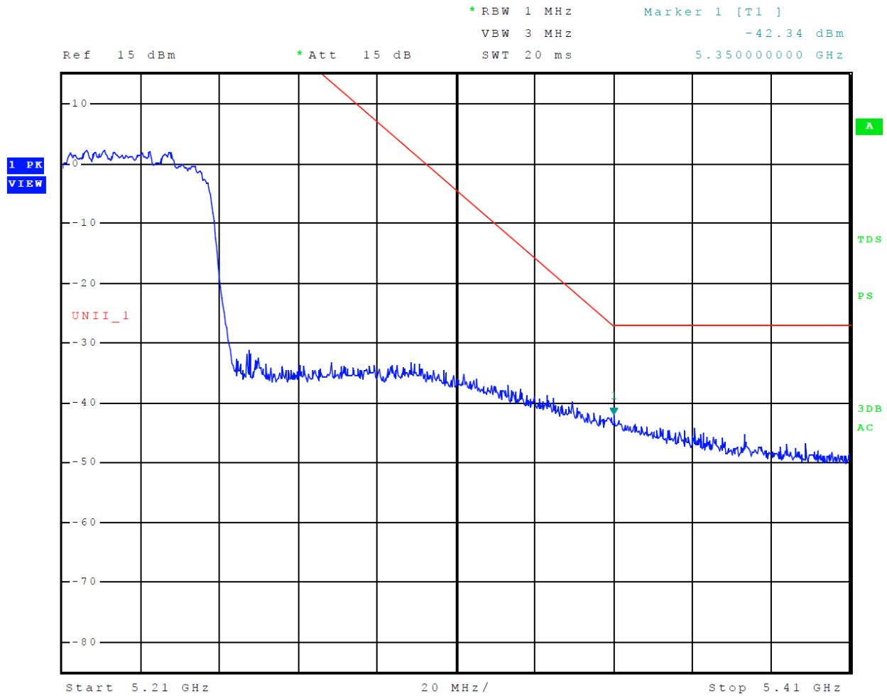
Figure 16 Plot of Upper Band Edge Across 5150-5250 MHz Mode 13 U-NII-1 (802.11ac80)
