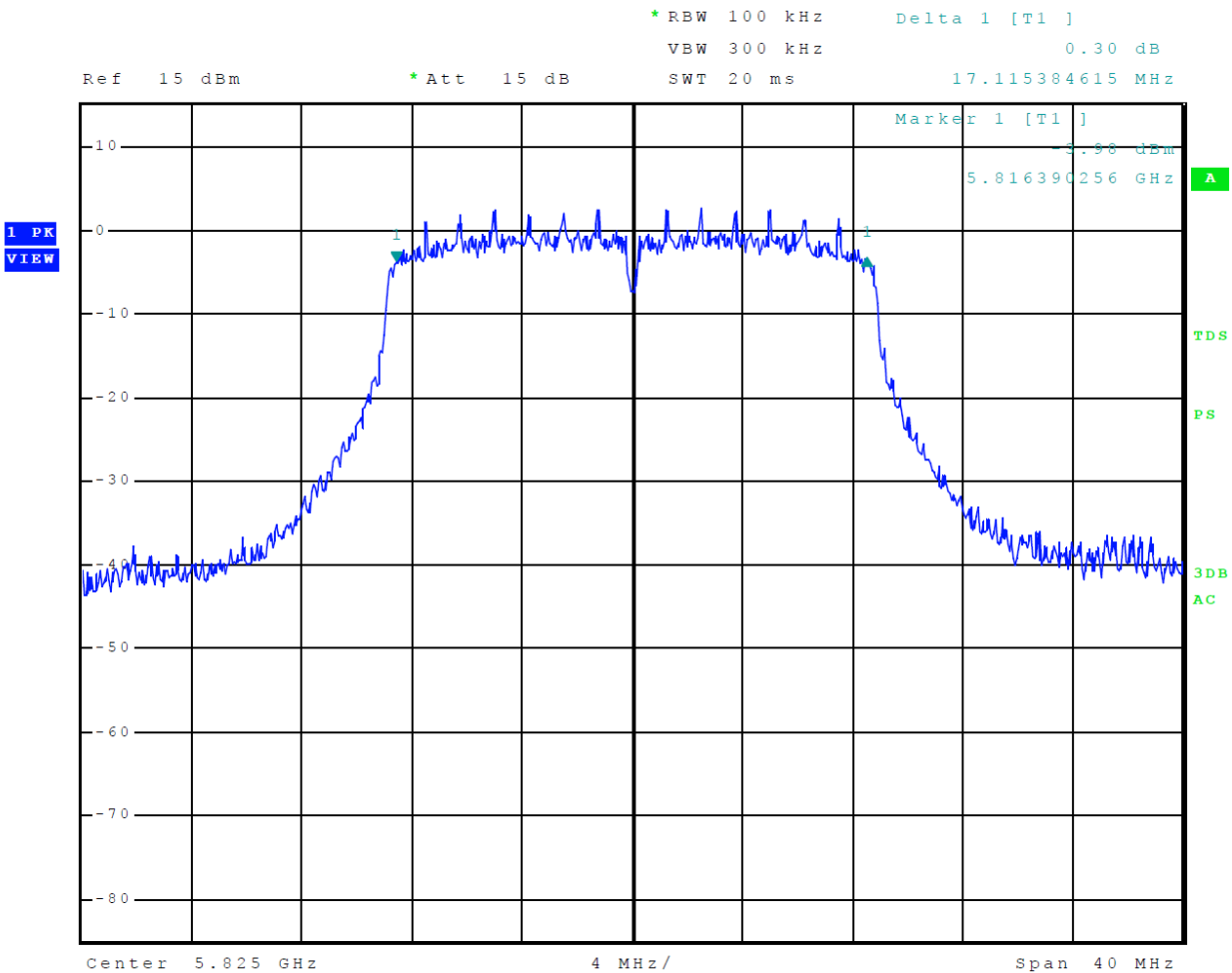
Figure 42 Plot of 6-dB Occupied Bandwidth 5725-5850 MHz Mode 15 U-NII-3 (802.11n)
