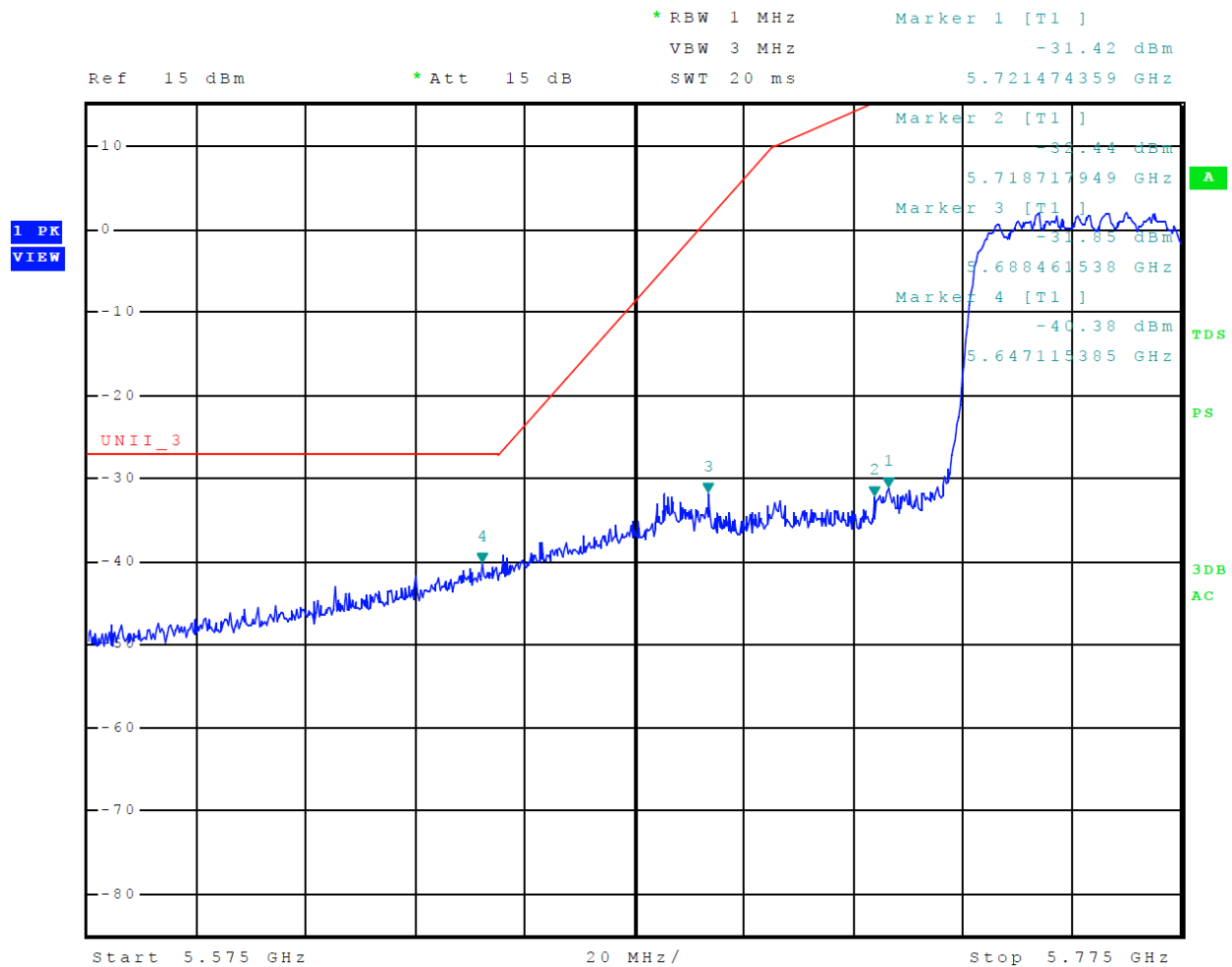
Figure 32 Plot of Lower Band Edge Across 5725-5850 MHz Mode 17 U-NII-3 (802.11ac80)
