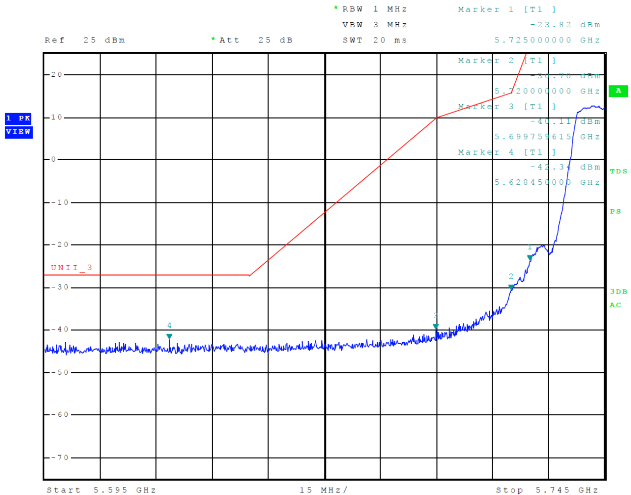
Figure 29 Plot of Lower Band Edge Across 5725-5850 MHz Mode 14 U-NII-3 (802.11a)
