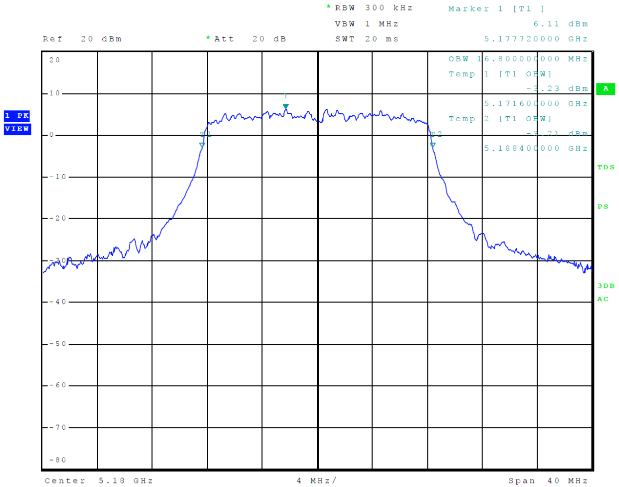
Figure 21 Plot of 99% Occupied Bandwidth 5150-5250 MHz Mode 10 U-NII-1 (802.11a)
