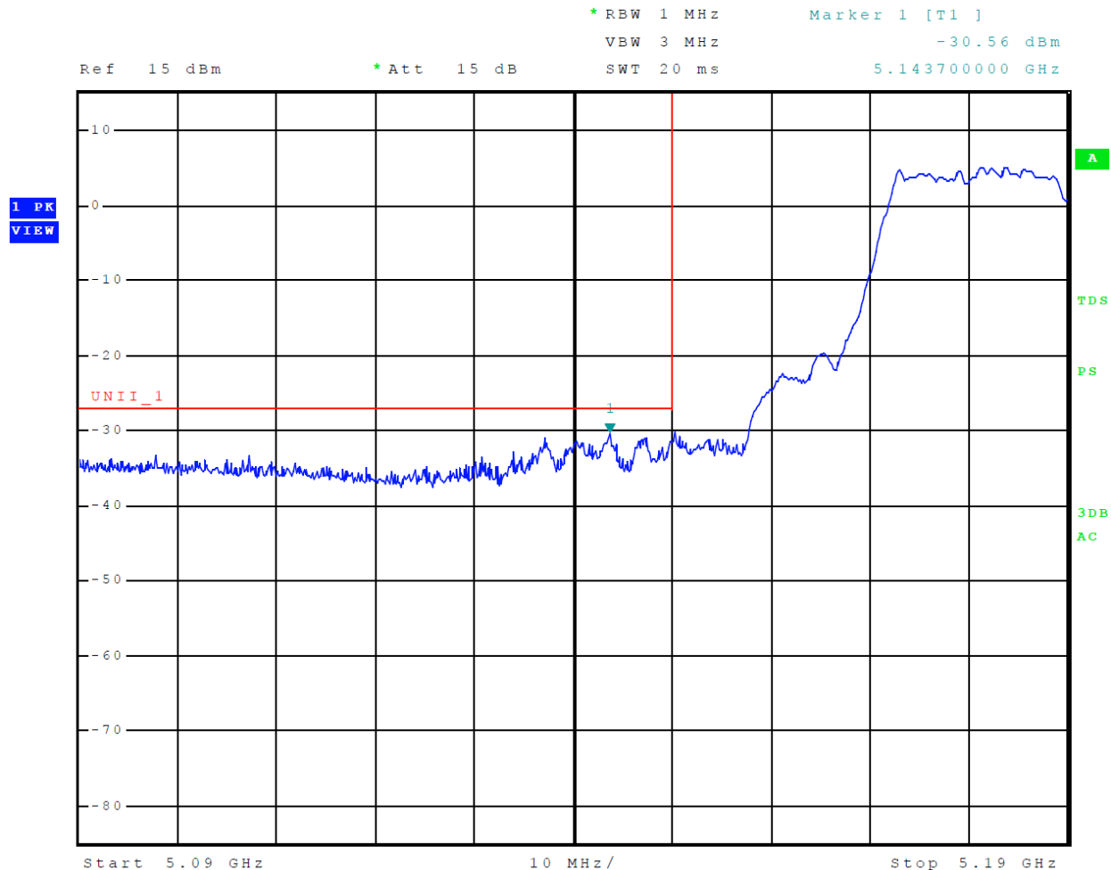
Figure 11 Plot of Lower Band Edge Across 5150-5250 MHz Mode 12 (802.11n40)
