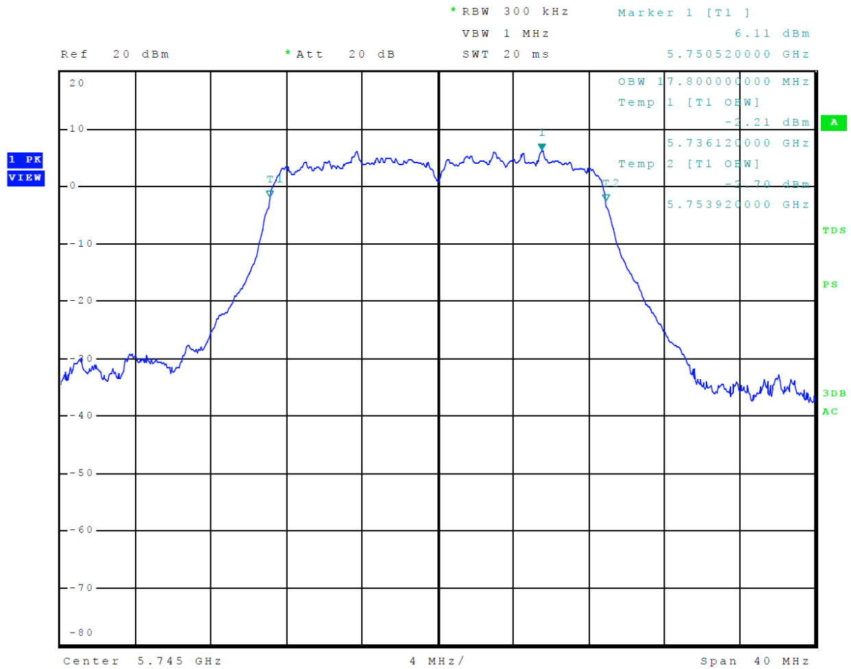
Figure 38 Plot of 99% Occupied Bandwidth 5725-5850 MHz Mode 15 U-NII-3 (802.11n)
