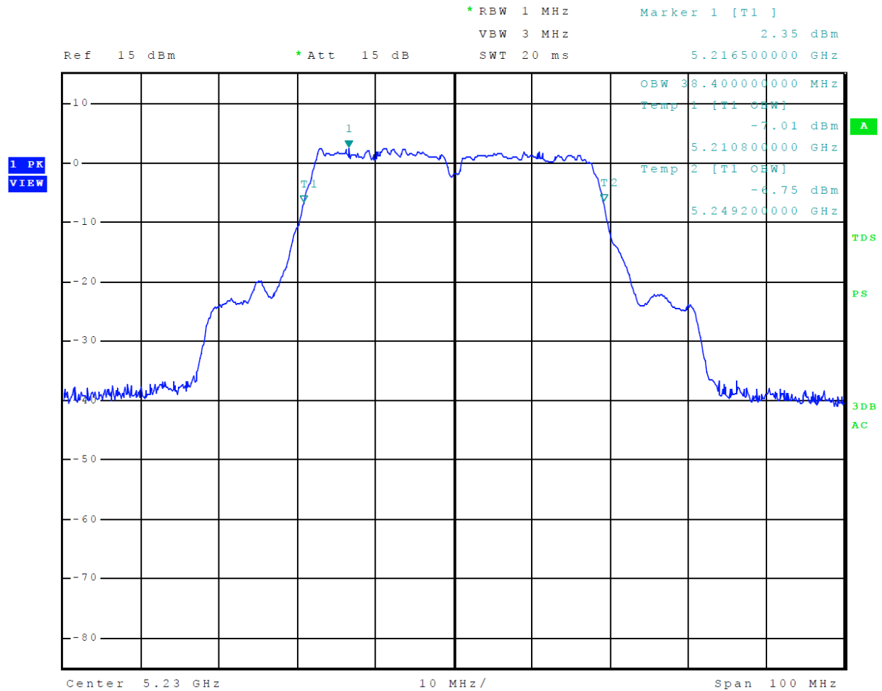
Figure 23 Plot of 99% Occupied Bandwidth 5150-5250 MHz Mode 12 U-NII-1 (802.11n40)
