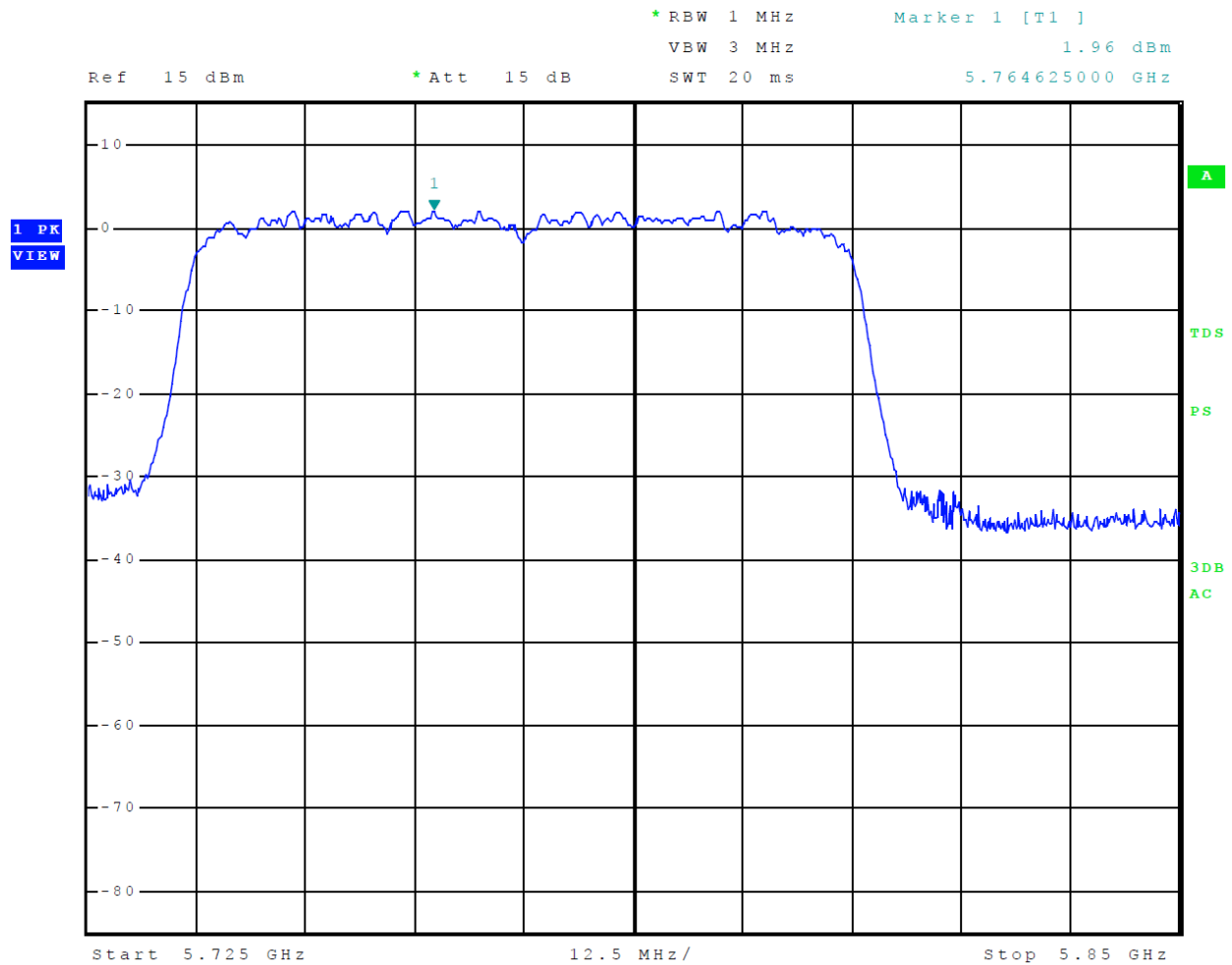
Figure 28 Plot of Transmitter Emissions Across 5725-5850 MHz Mode 17 U-NII-3 (802.11ac80)
