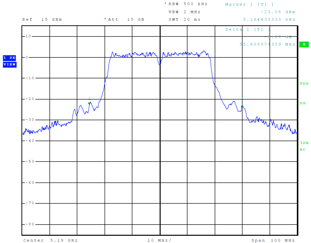
Figure 19 Plot of 26-dB Occupied Bandwidth 5150-5250 MHz Mode 12 U-NII-1 (802.11n40)
