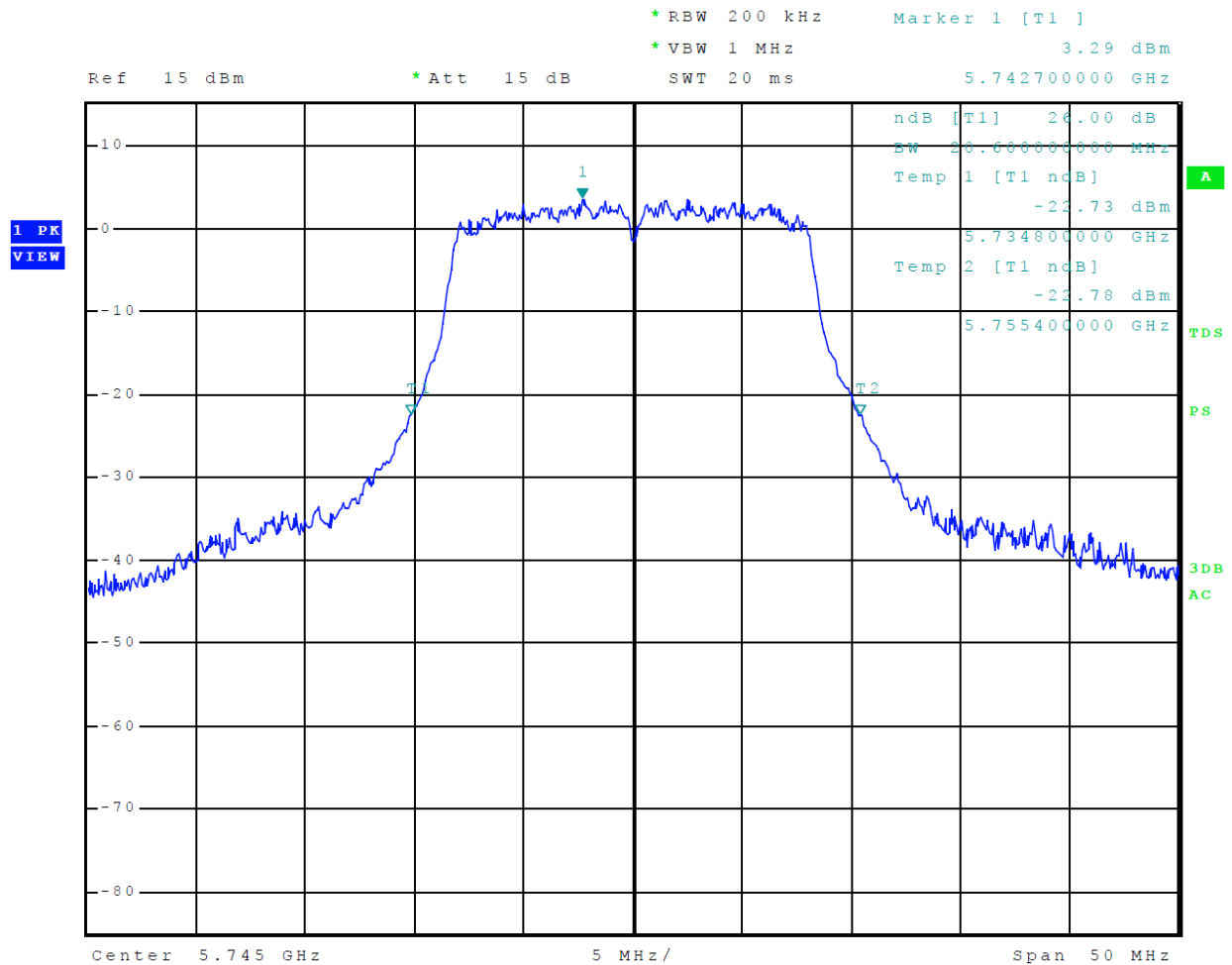
Figure 45 Plot of 26-dB Occupied Bandwidth 5725-5850 MHz Mode 14 U-NII-3 (802.11a)
