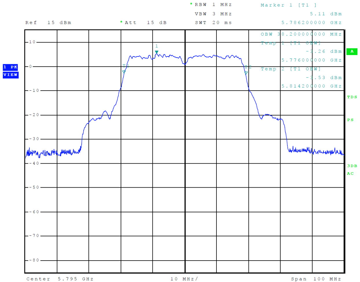
Figure 39 Plot of 99% Occupied Bandwidth 5725-5850 MHz Mode 16 U-NII-3 (802.11n40)
