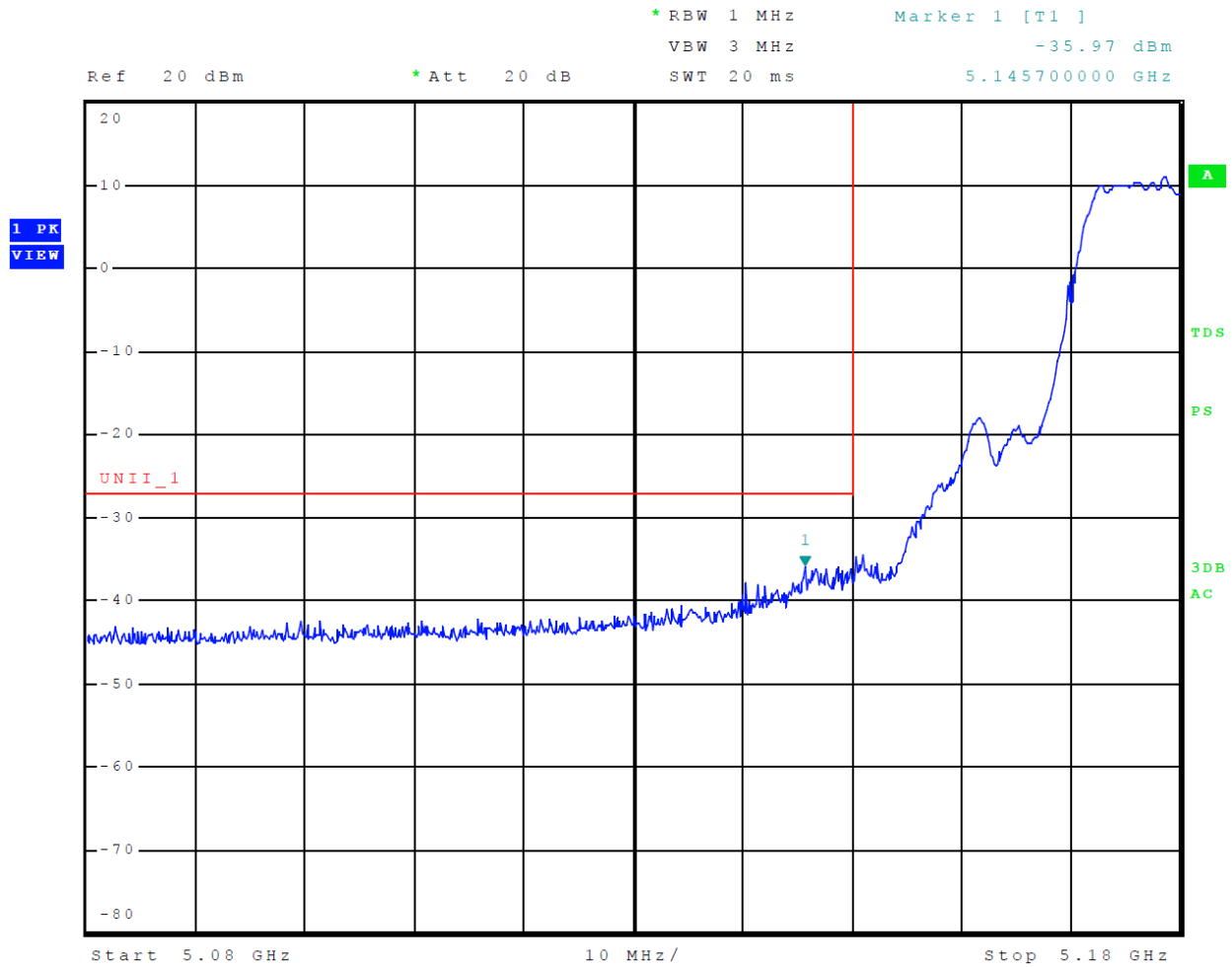
Figure 10 Plot of Lower Band Edge Across 5150-5250 MHz Mode 11 U-NII-1 (802.11n)
