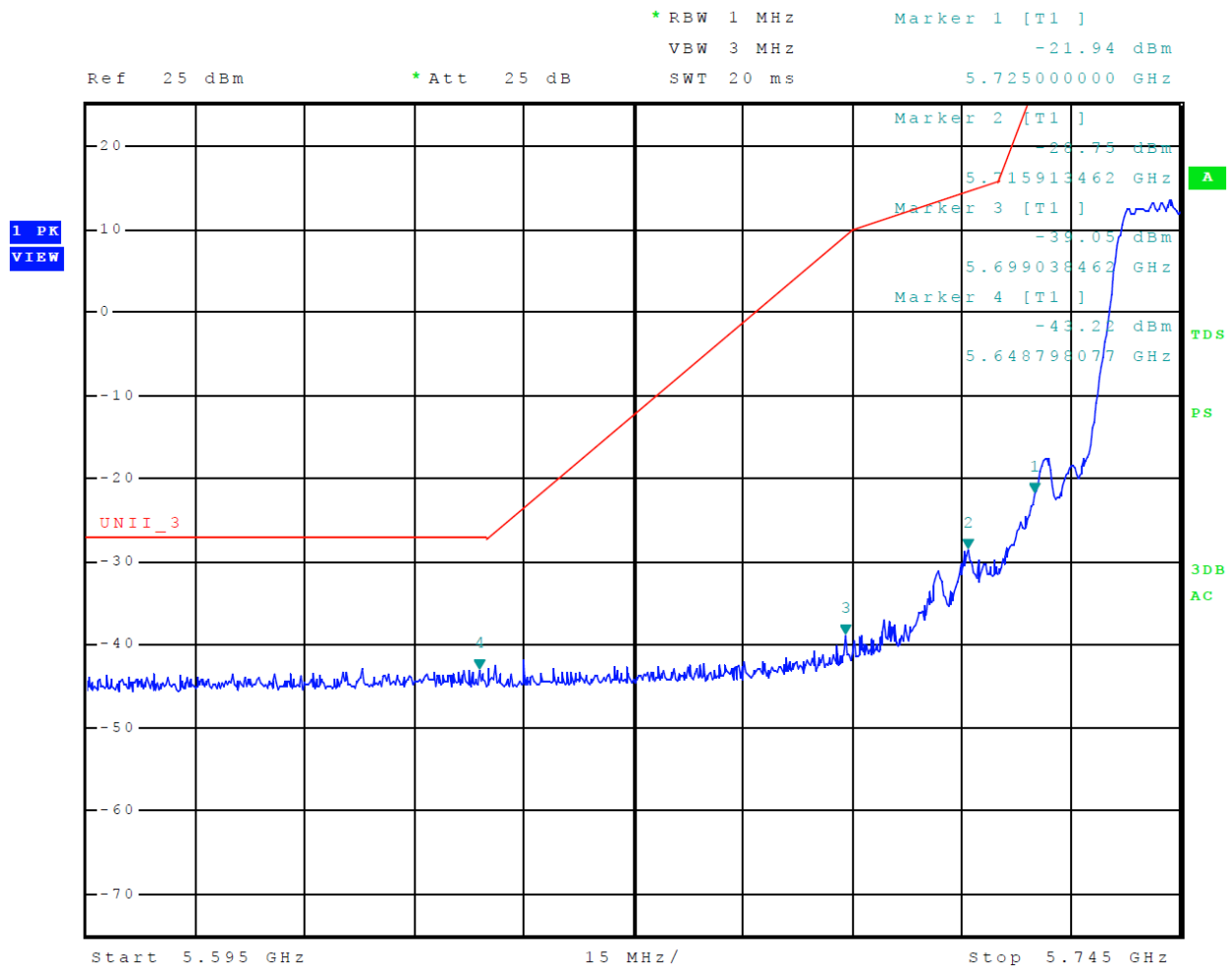
Figure 30 Plot of Lower Band Edge Across 5725-5850 MHz Mode 15 U-NII-3 (802.11n)
