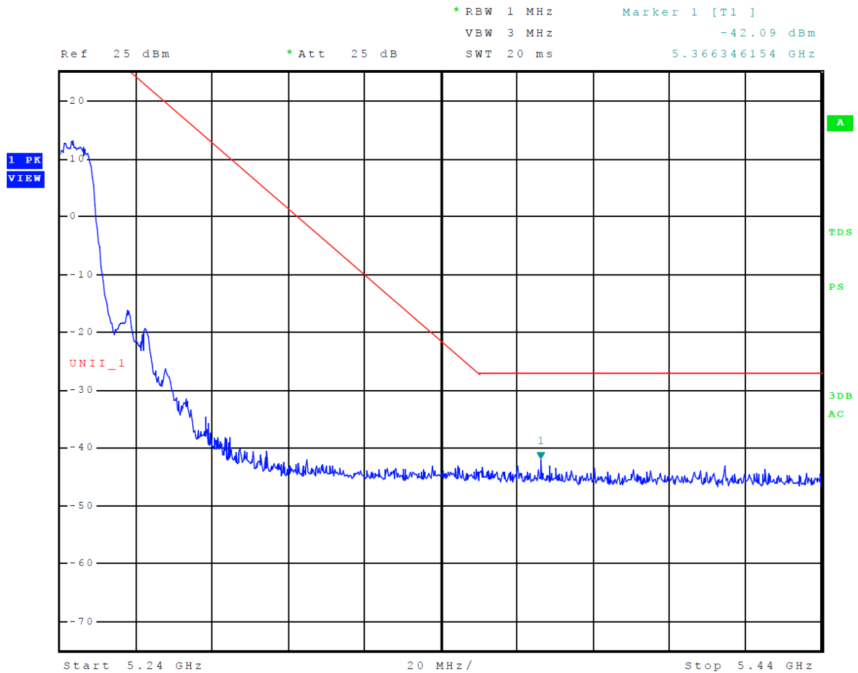
Figure 14 Plot of Upper Band Edge Across 5150-5250 MHz Mode 11 U-NII-1 (802.11n)
