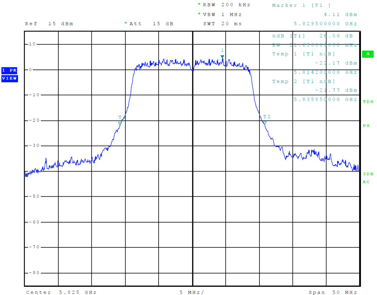
Figure 46 Plot of 26-dB Occupied Bandwidth 5725-5850 MHz Mode 15 U-NII-3 (802.11n)
