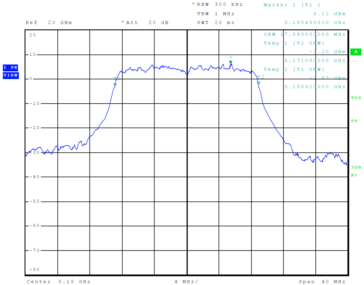
Figure 22 Plot of 99% Occupied Bandwidth 5150-5250 MHz Mode 11 U-NII-1 (802.11n)
