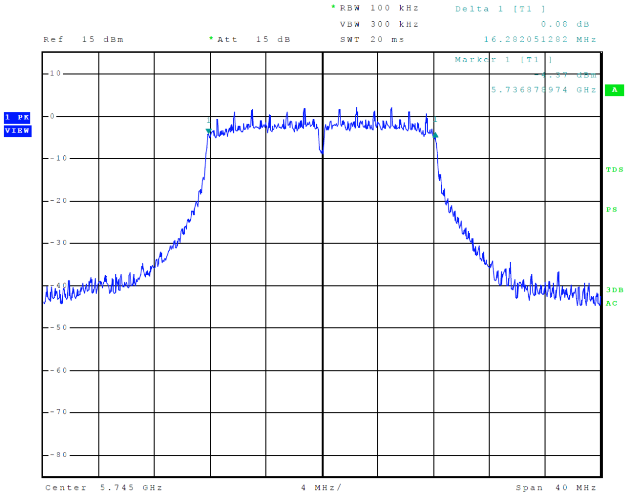
Figure 41 Plot of 6-dB Occupied Bandwidth 5725-5850 MHz Mode 14 U-NII-3 (802.11a)
