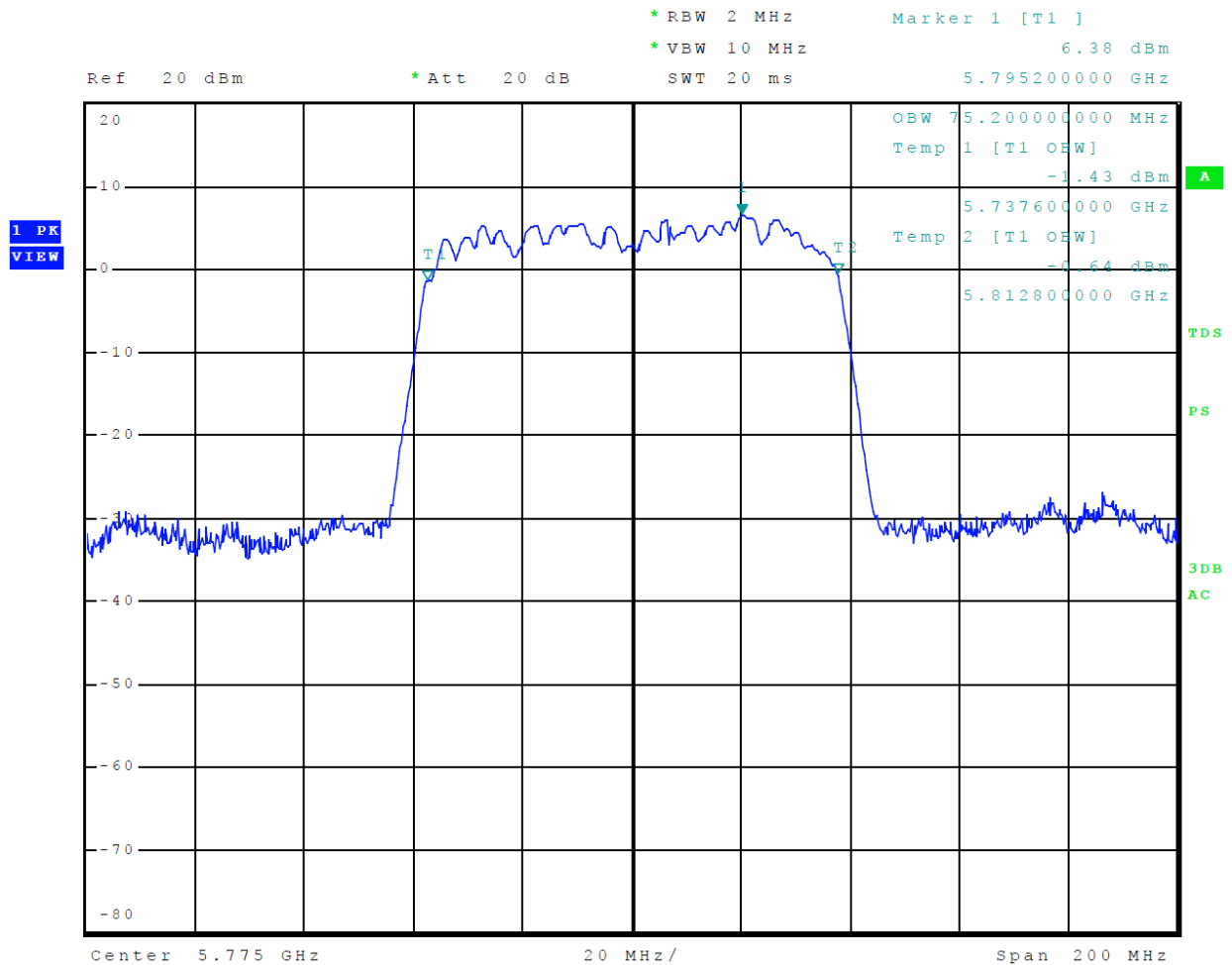
Figure 40 Plot of 99% Occupied Bandwidth 5725-5850 MHz Mode 17 U-NII-3 (802.11ac80)
