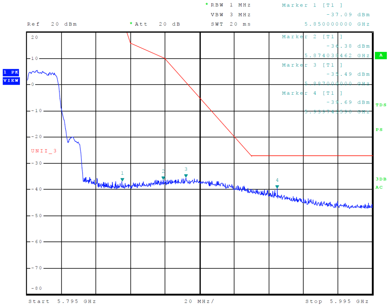
Figure 35 Plot of Upper Band Edge Across 5725-5850 MHz Mode 16 U-NII-3 (802.11n40)
