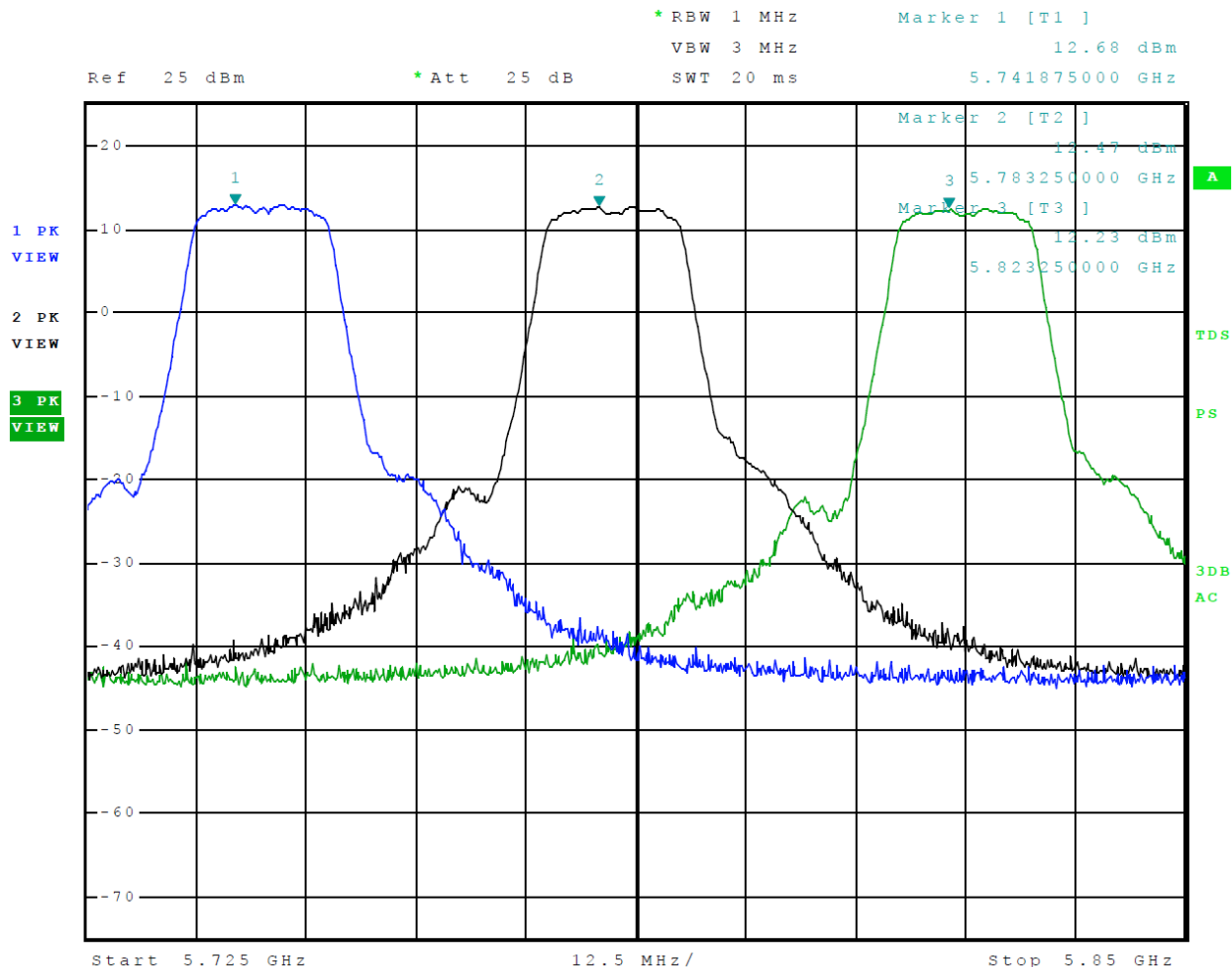
Figure 25 Plot of Transmitter Emissions Across 5725-5850 MHz Mode 14 U-NII-3 (802.11a)
