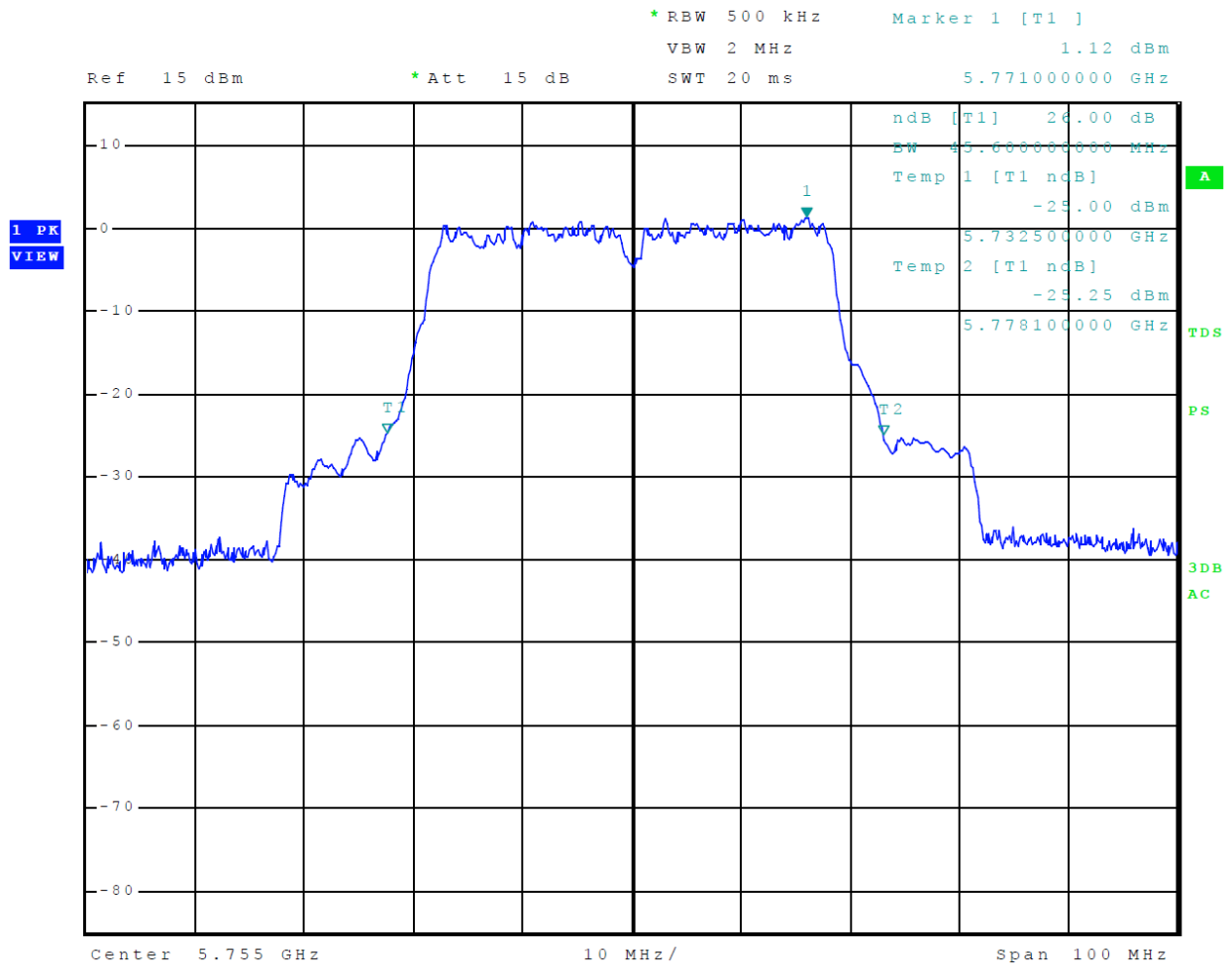
Figure 47 Plot of 26-dB Occupied Bandwidth 5725-5850 MHz Mode 16 U-NII-3 (802.11n40)
