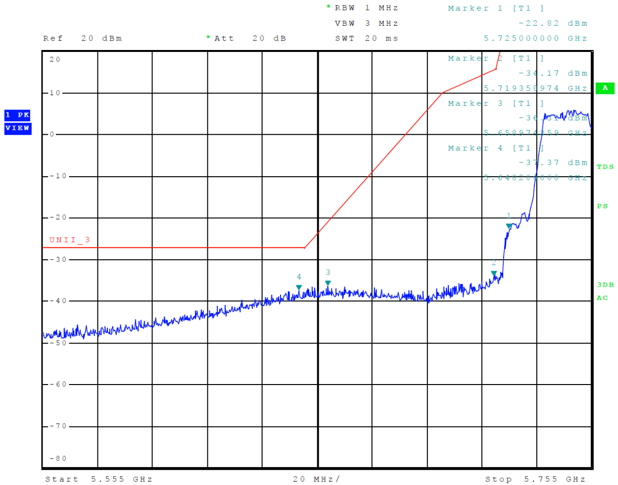
Figure 31 Plot of Lower Band Edge Across 5725-5850 MHz Mode 16 U-NII-3 (802.11n40)
