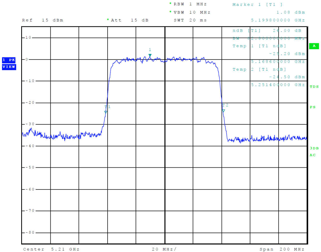
Figure 20 Plot of 26-dB Occupied Bandwidth 5150-5250 MHz Mode 13 U-NII-1 (802.11ac80)
