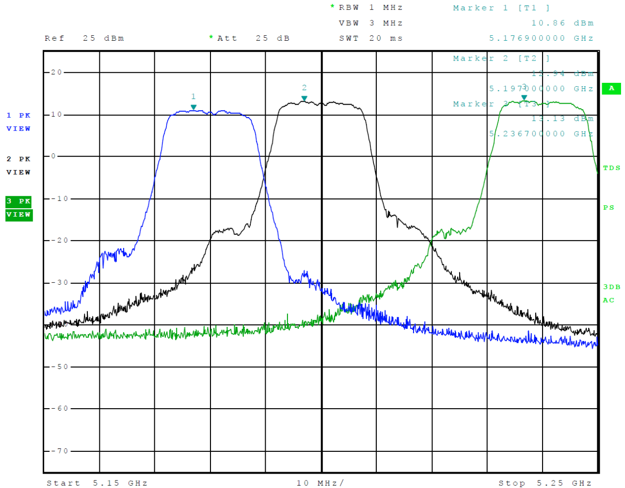
Figure 5 Plot of Transmitter Emissions Across 5150-5250 MHz Mode 10 U-NII-1 (802.11a)
