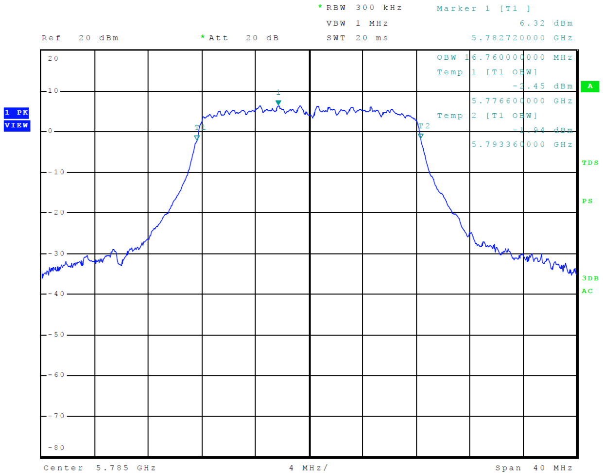
Figure 37 Plot of 99% Occupied Bandwidth 5725-5850 MHz Mode 14 U-NII-3 (802.11a)
