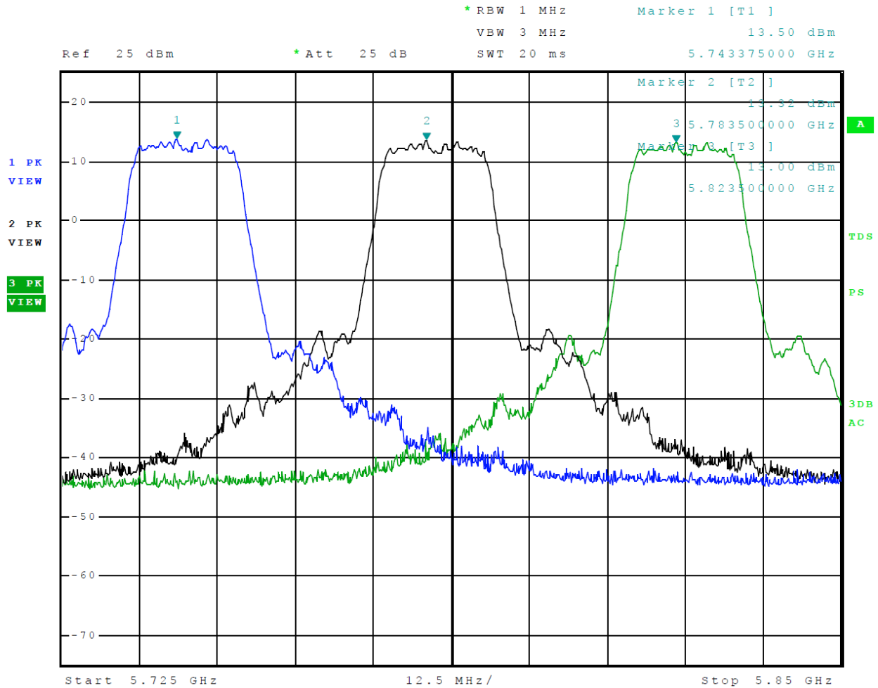
Figure 26 Plot of Transmitter Emissions Across 5725-5850 MHz Mode 15 U-NII-3 (802.11n)
