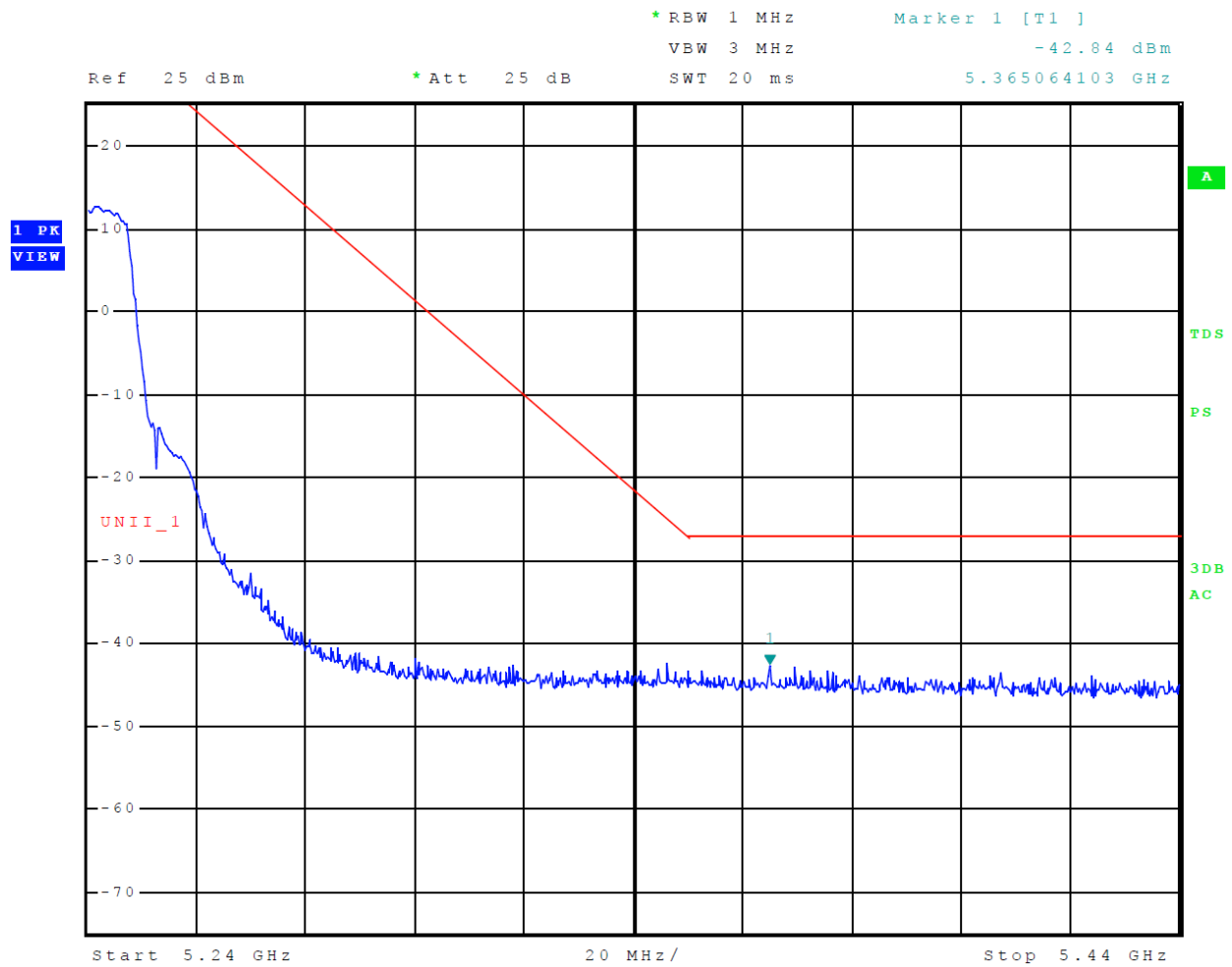
Figure 13 Plot of Upper Band Edge Across 5150-5250 MHz Mode 10 U-NII-1 (802.11a)
