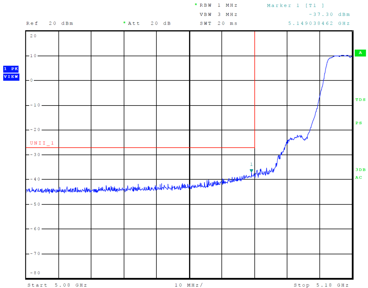
Figure 9 Plot of Lower Band Edge Across 5150-5250 MHz Mode 10 U-NII-1 (802.11a)
