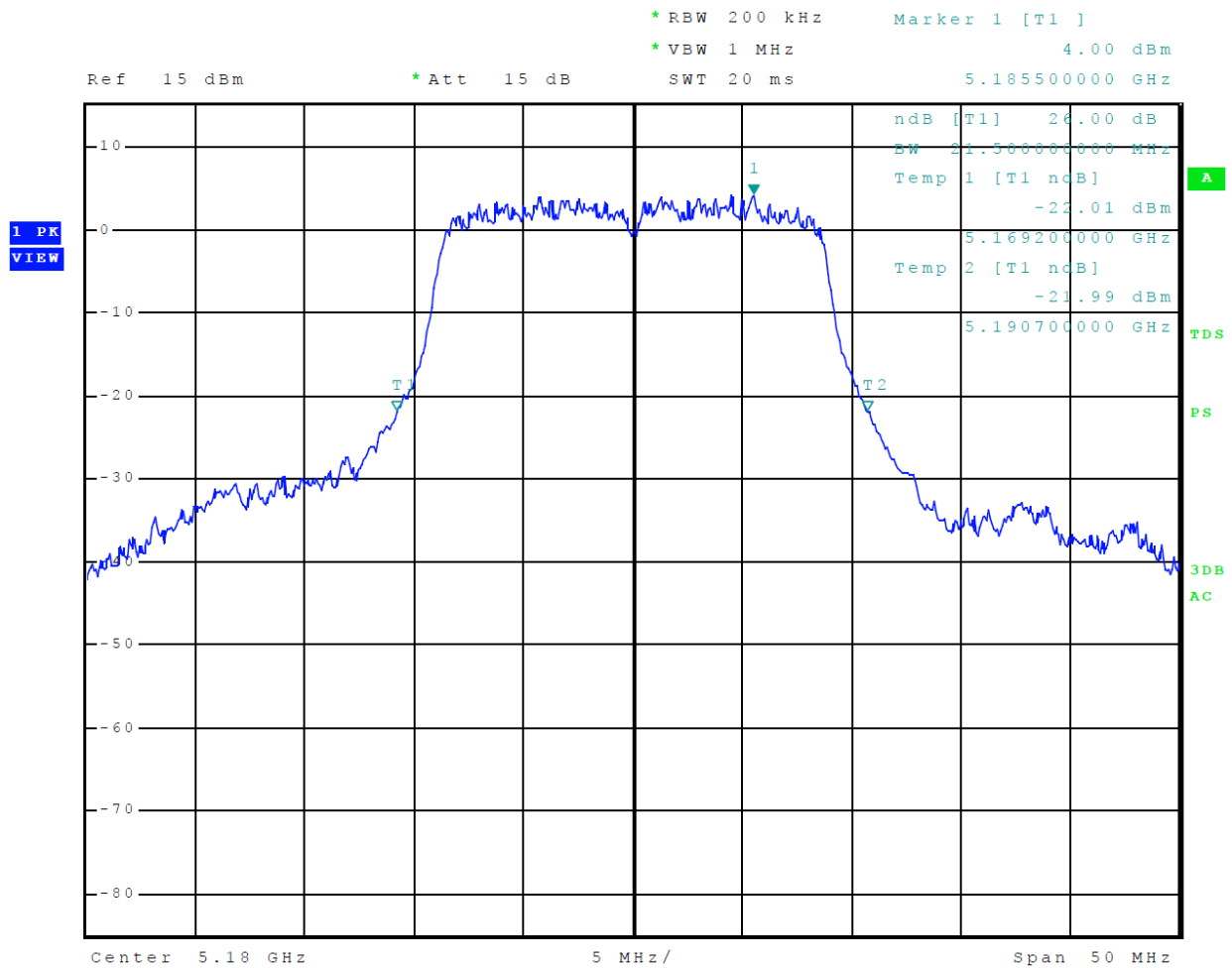
Figure 18 Plot of 26-dB Occupied Bandwidth 5150-5250 MHz Mode 11 U-NII-1 (802.11n)
