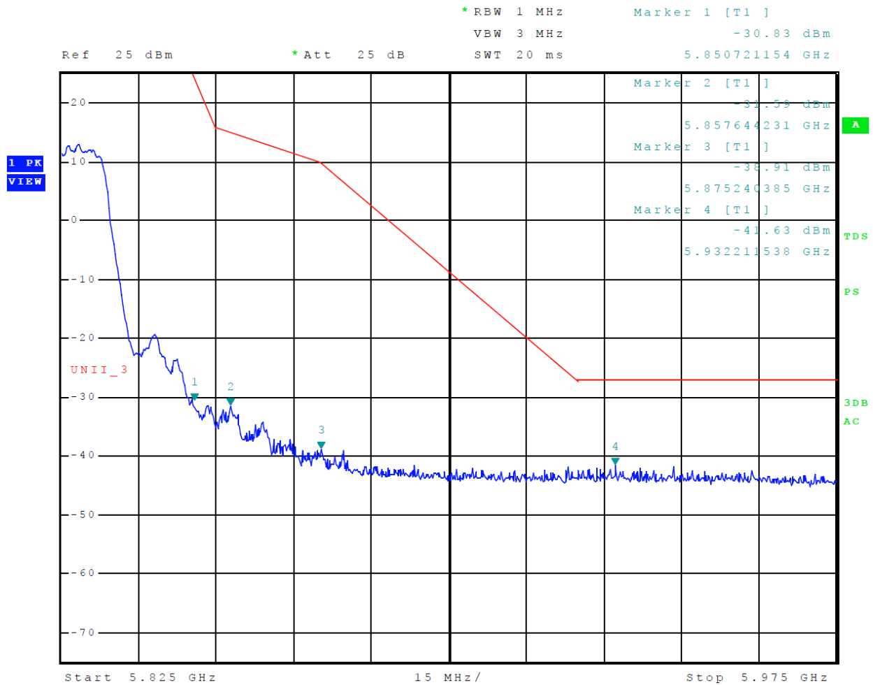
Figure 34 Plot of Upper Band Edge Across 5725-5850 MHz Mode 15 U-NII-3 (802.11n)
