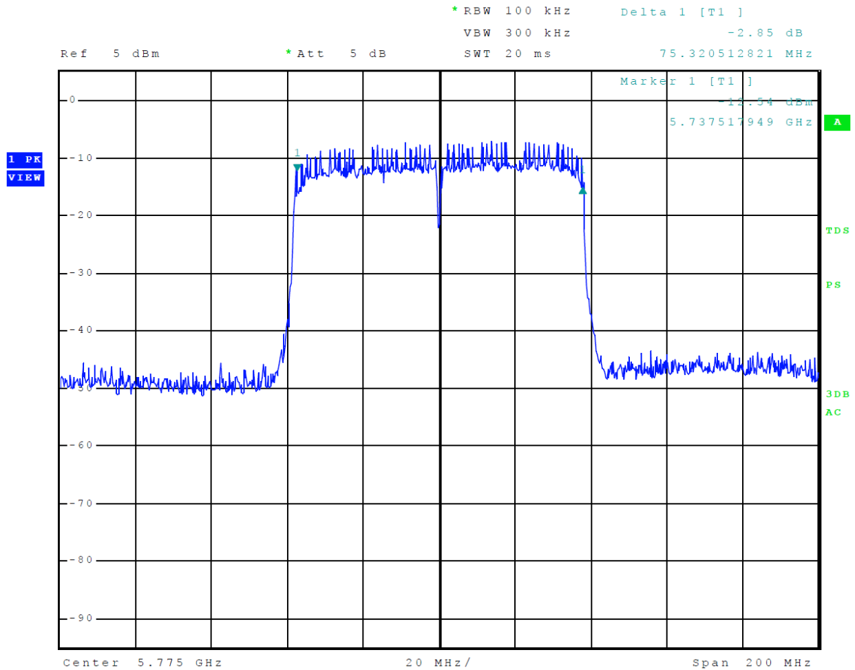
Figure 44 Plot of 6-dB Occupied Bandwidth 5725-5850 MHz Mode 17 U-NII-3 (802.11ac80)
