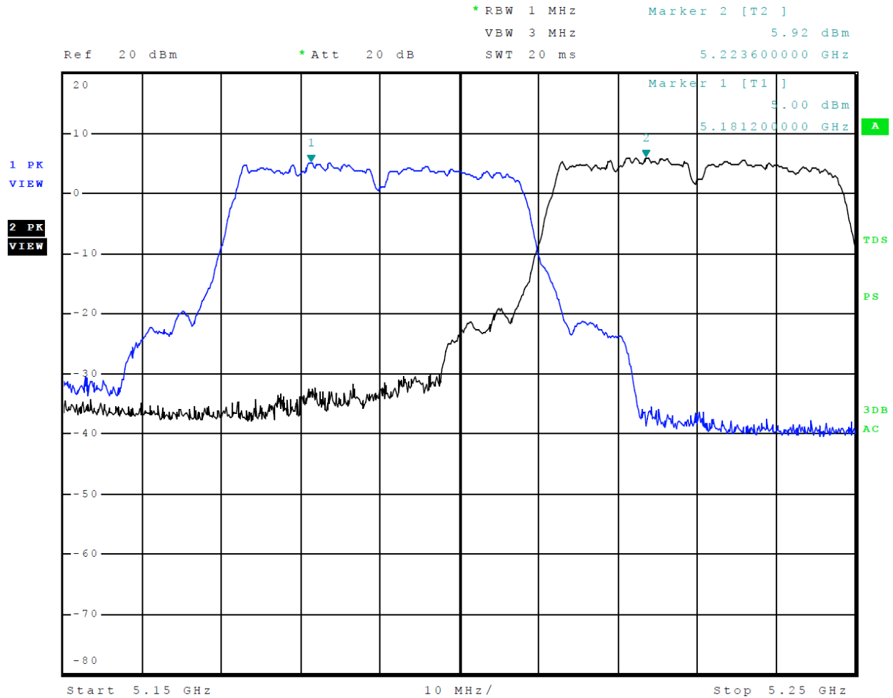
Figure 7 Plot of Transmitter Emissions Across 5150-5250 MHz Mode 12 U-NII-1 (802.11n40)
