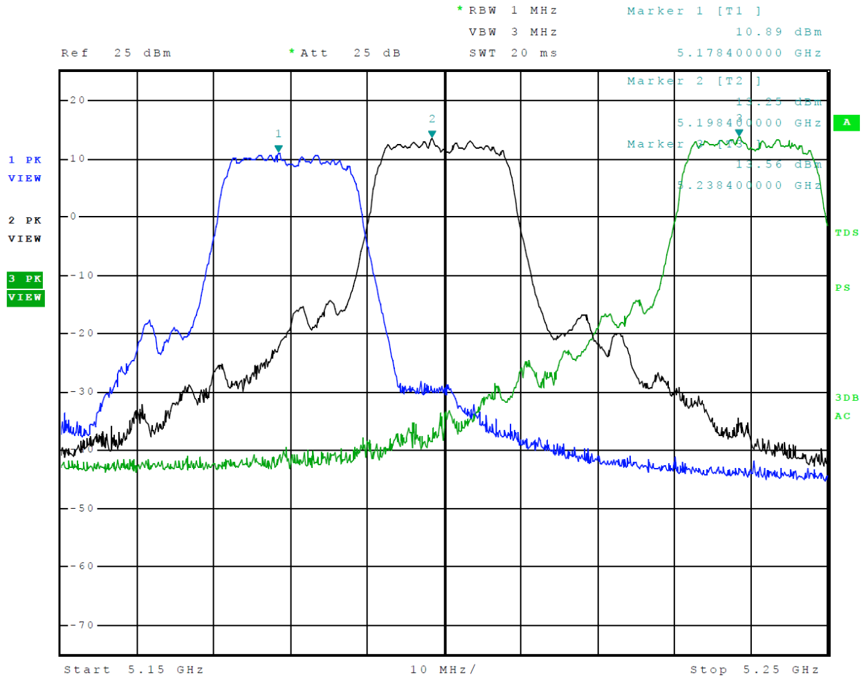
Figure 6 Plot of Transmitter Emissions Across 5150-5250 MHz Mode 11 U-NII-1 (802.11n)
