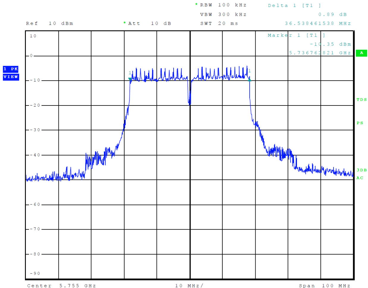
Figure 43 Plot of 6-dB Occupied Bandwidth 5725-5850 MHz Mode 16 U-NII-3 (802.11n40)
