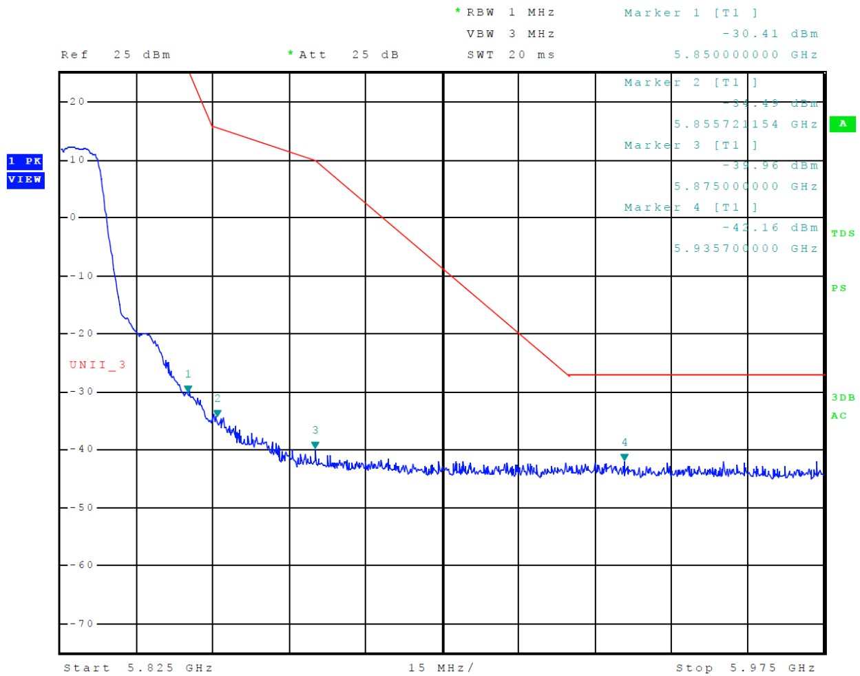
Figure 33 Plot of Upper Band Edge Across 5725-5850 MHz Mode 14 U-NII-3 (802.11a)
