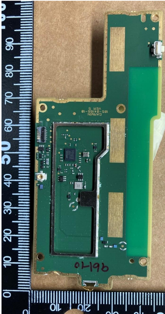
Left PCB Front Side without Shield
