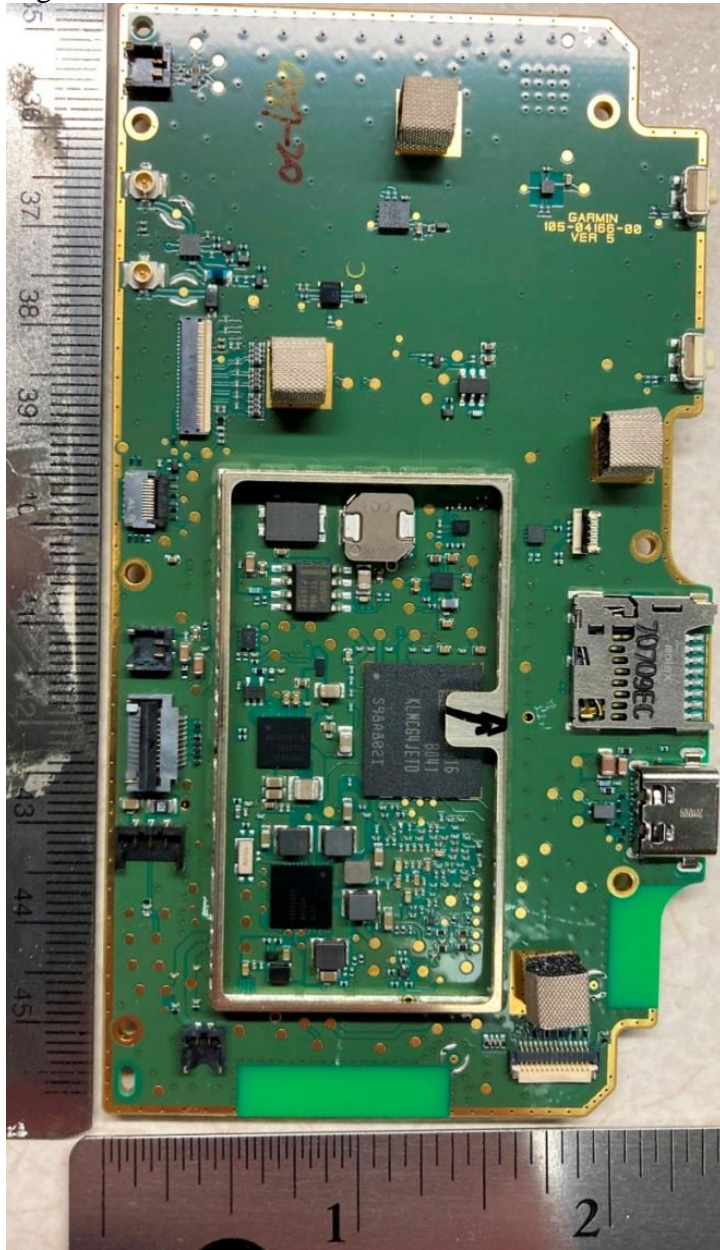
Right PCB Front Side without shield
