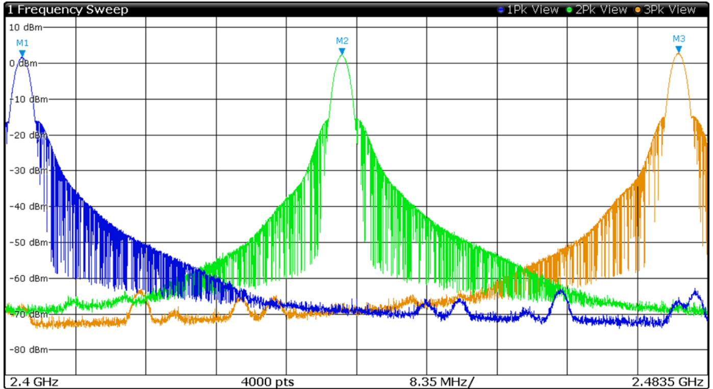
Figure 6 Plot of Transmitter Emissions Operation in 2402-2480 MHz Mode 4 BT 3EDR
