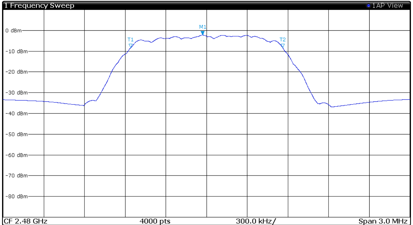
Figure 26 Plot of 6-dB Occupied Bandwidth Mode 3 BT 2EDR
