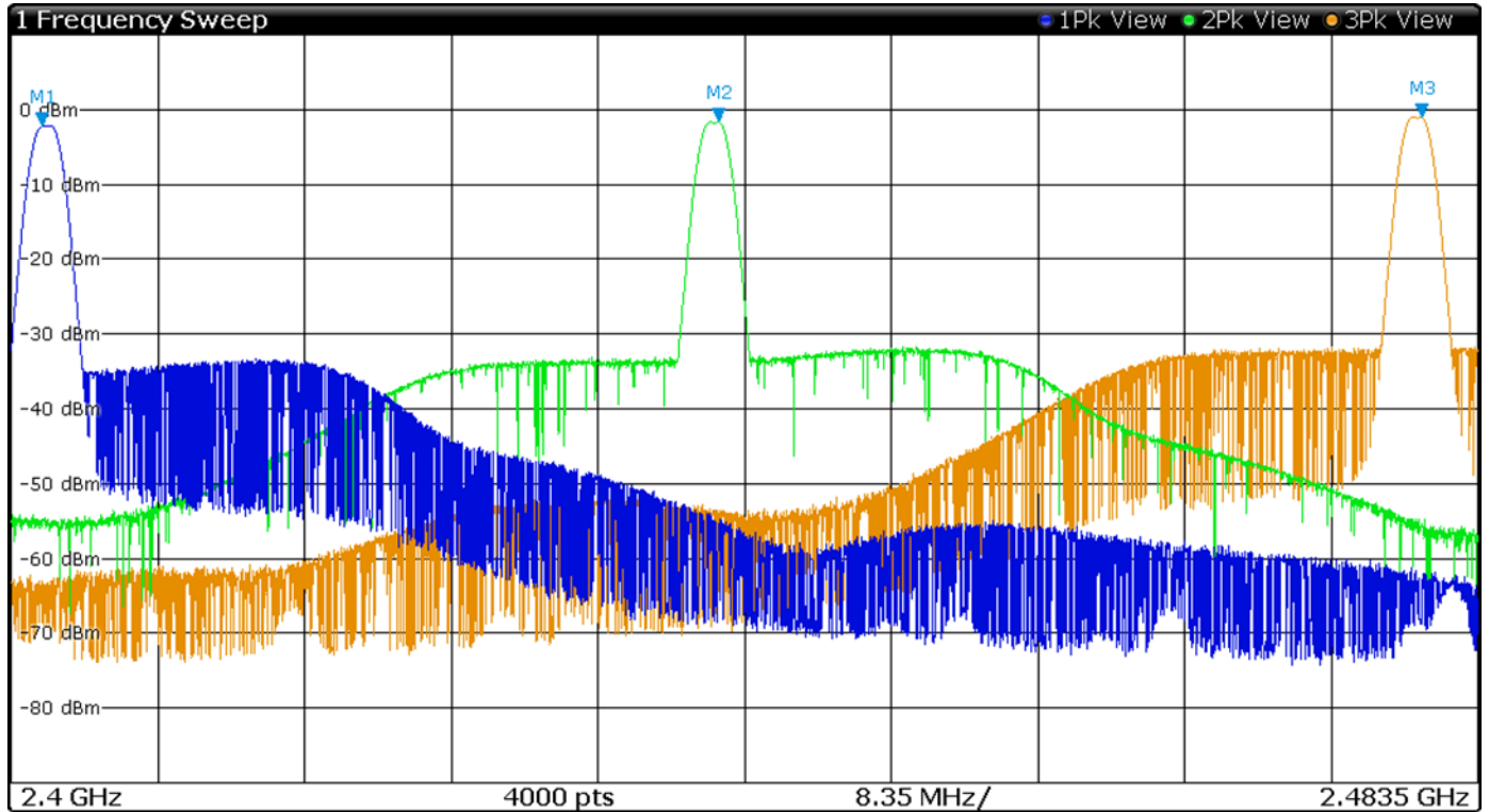
Figure 7 Plot of Transmitter Emissions Operation in 2402-2480 MHz Mode 5 BT BLE
