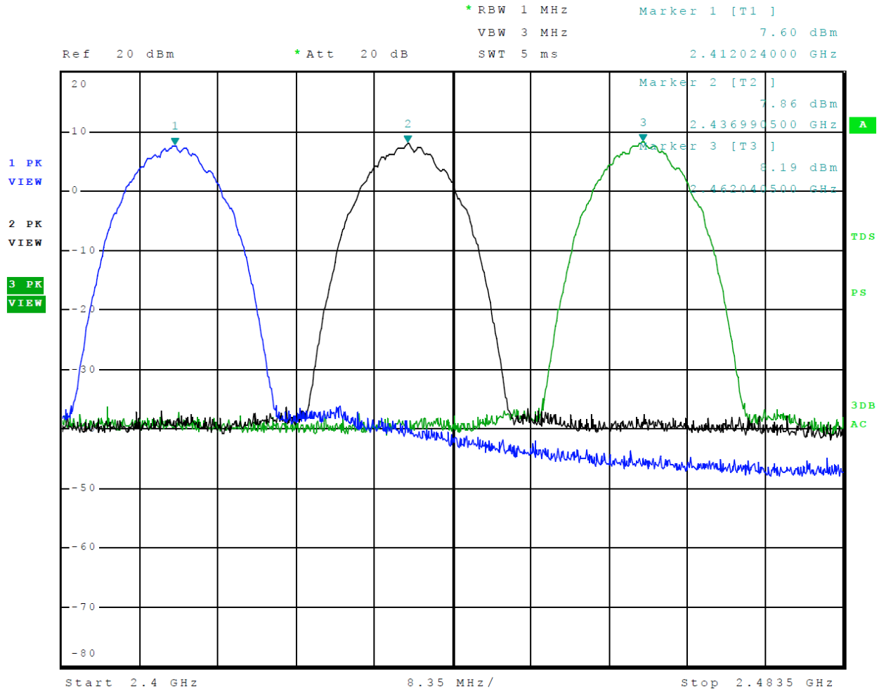
Figure 8 Plot of Transmitter Operation in 2412-2462 MHz Mode 6 802.11b
