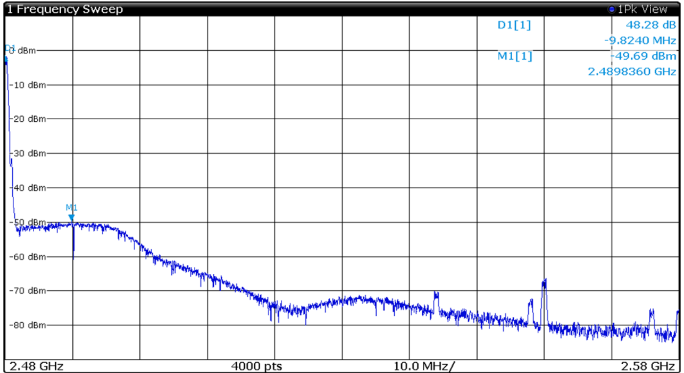
Figure 21 Plot of Transmitter Emissions High Band Edge Mode 5 BT BLE
