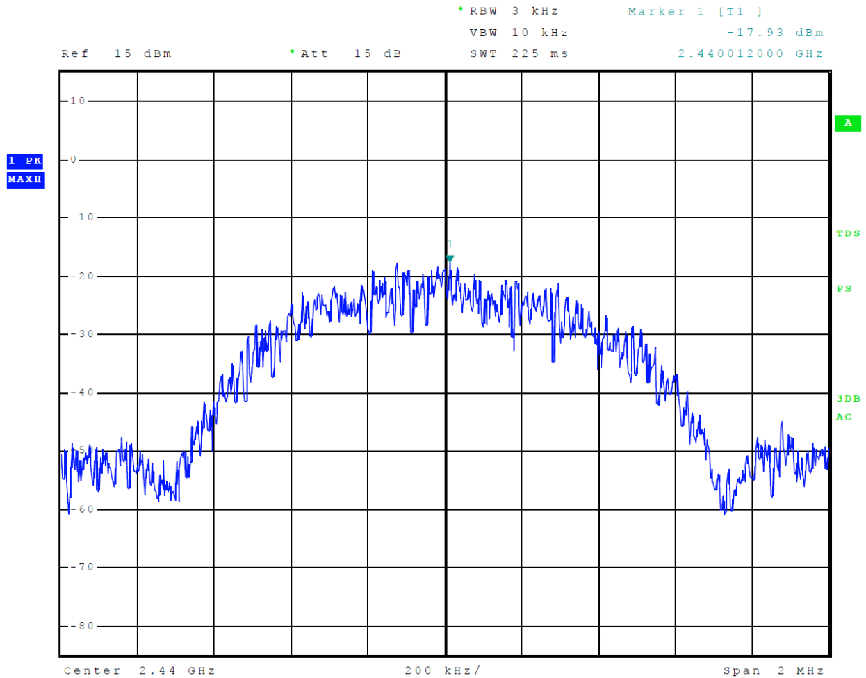
Figure 42 Plot of Transmitter Power Spectral Density Mode 5 BT BLE
