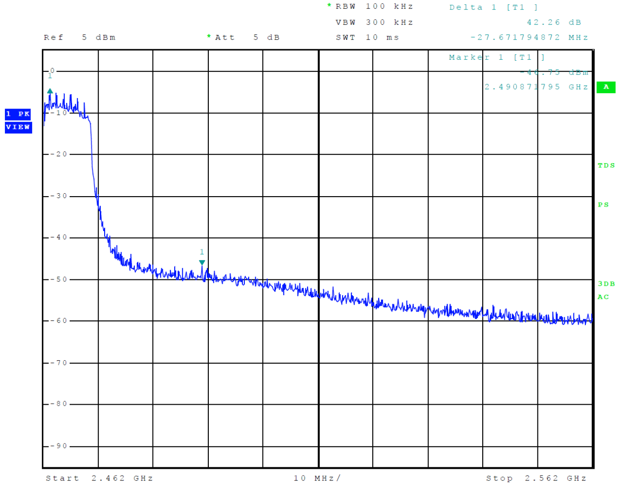
Figure 24 Plot of Transmitter Emissions High Band Edge Mode 8 802.11n
