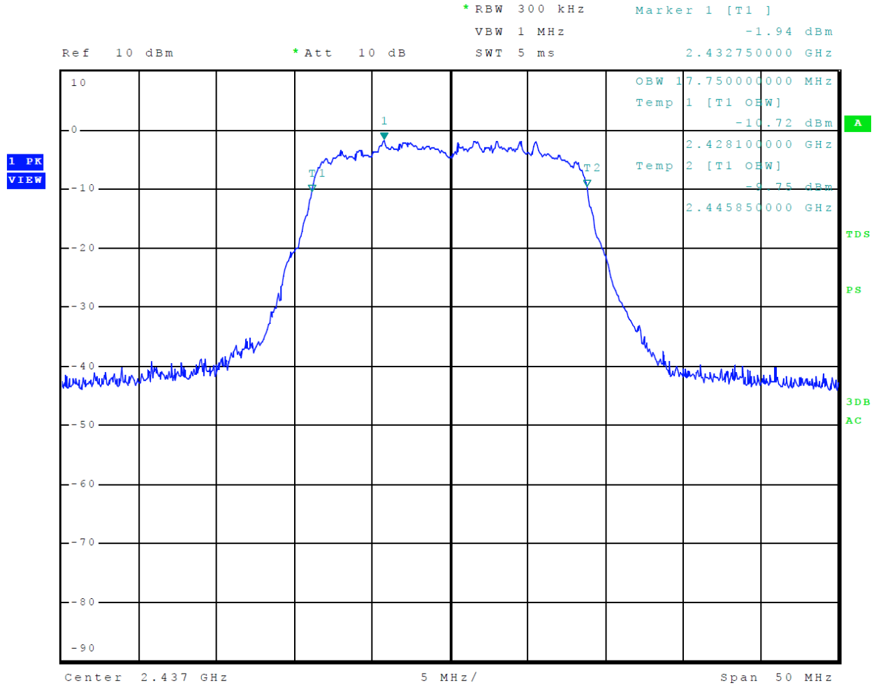
Figure 37 Plot of 99% Occupied Bandwidth Mode 8 802.11n
