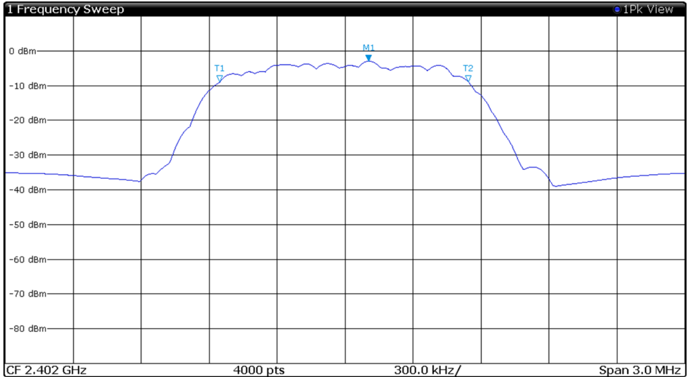
Figure 28 Plot of 6-dB Occupied Bandwidth Mode 4 BT 3EDR
