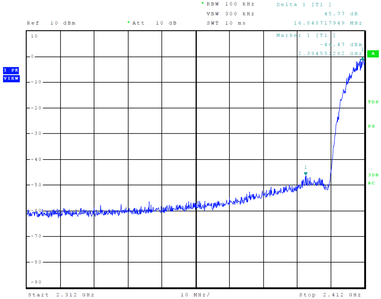
Figure 15 Plot of Transmitter Emissions Low Band Edge Mode 6 802.11b
