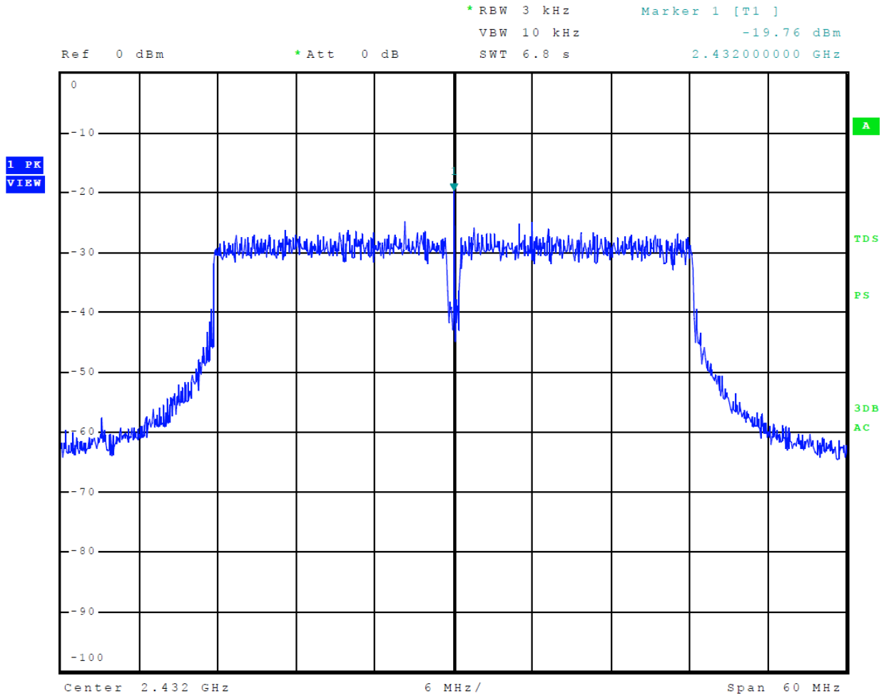
Figure 46 Plot of Transmitter Power Spectral Density Mode 9 802.11n40
