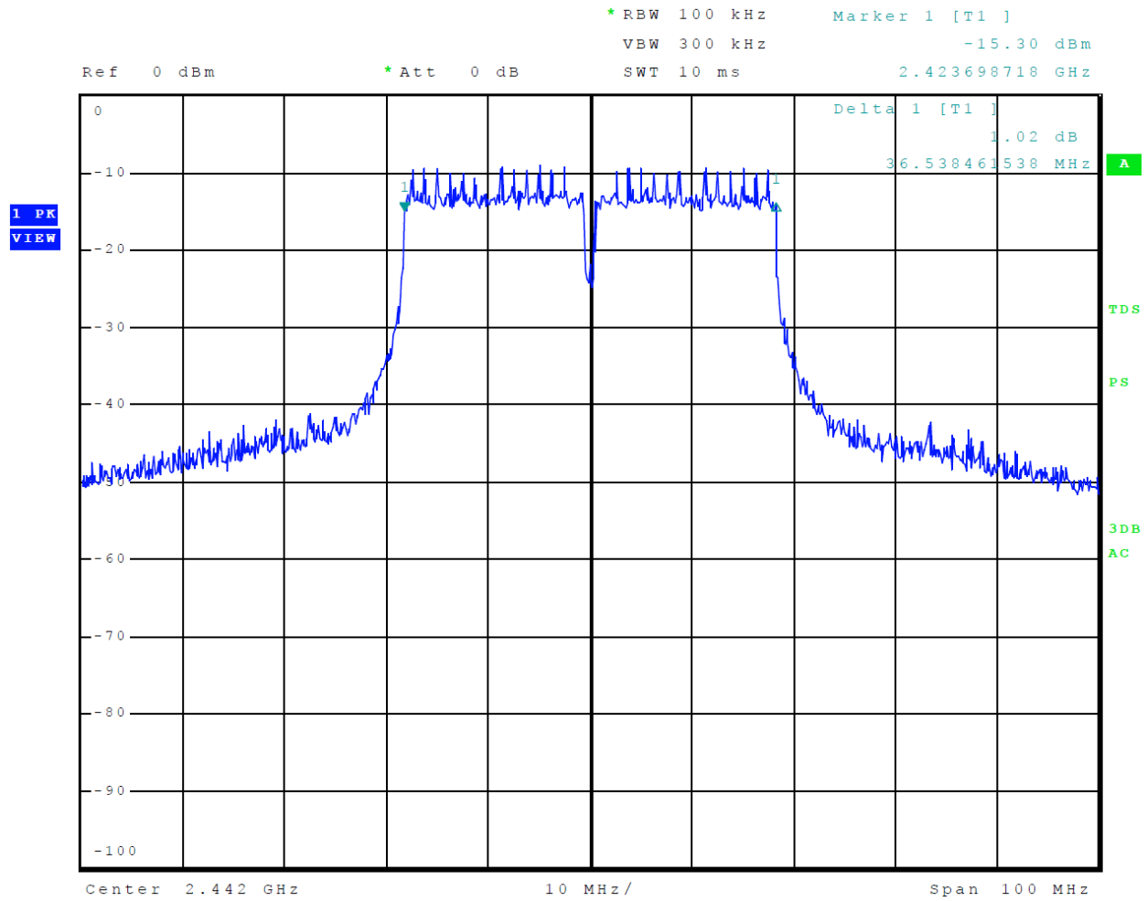
Figure 38 Plot of 6-dB Occupied Bandwidth Mode 9 802.11n40
