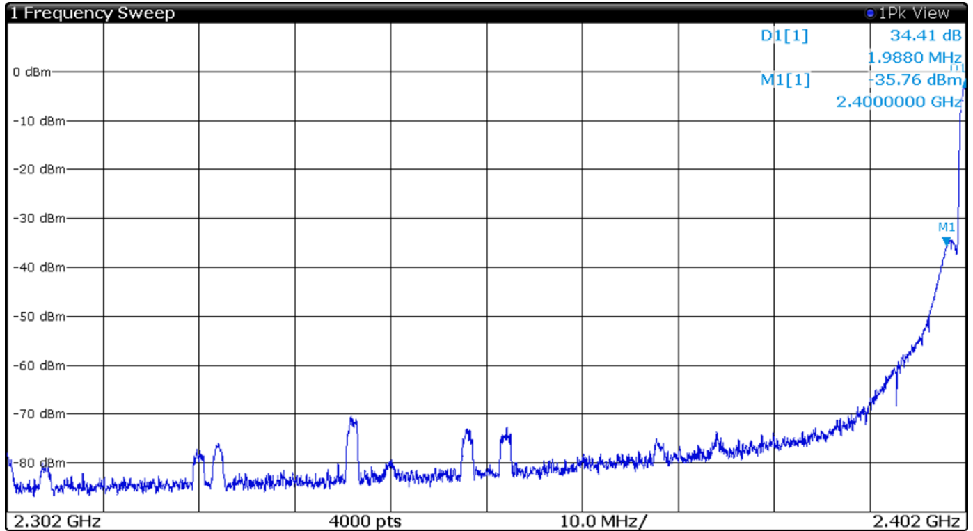
Figure 13 Plot of Transmitter Emissions Low Band Edge Mode 4 BT 3EDR
