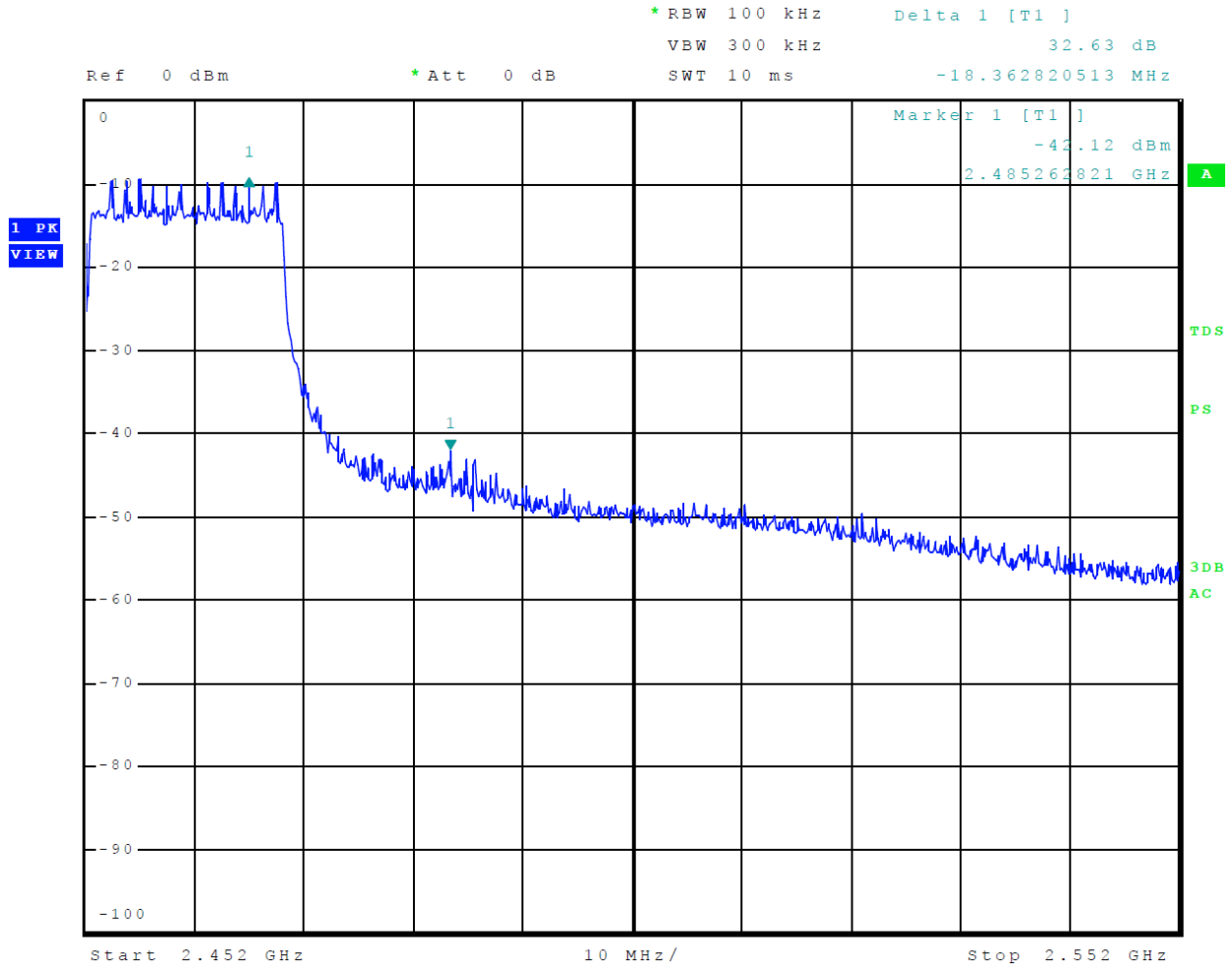
Figure 25 Plot of Transmitter Emissions High Band Edge Mode 9 802.11n40
