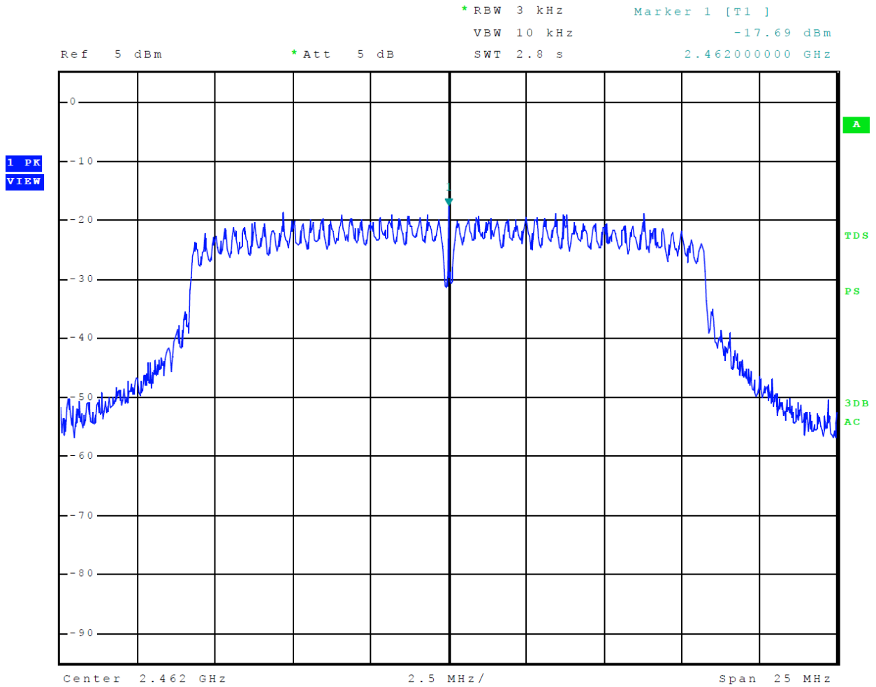
Figure 44 Plot of Transmitter Power Spectral Density Mode 7 802.11g
