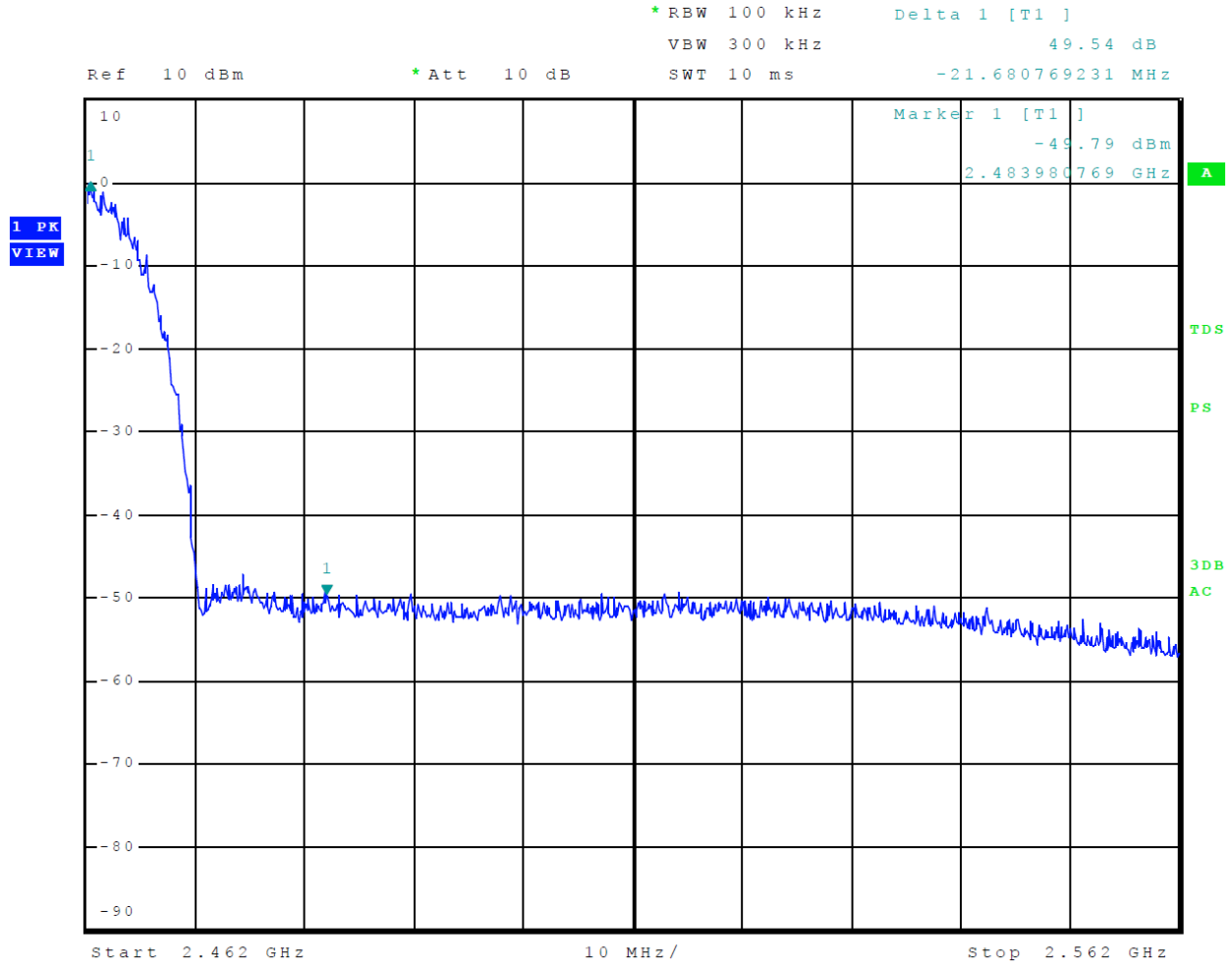
Figure 22 Plot of Transmitter Emissions High Band Edge Mode 6 802.11b
