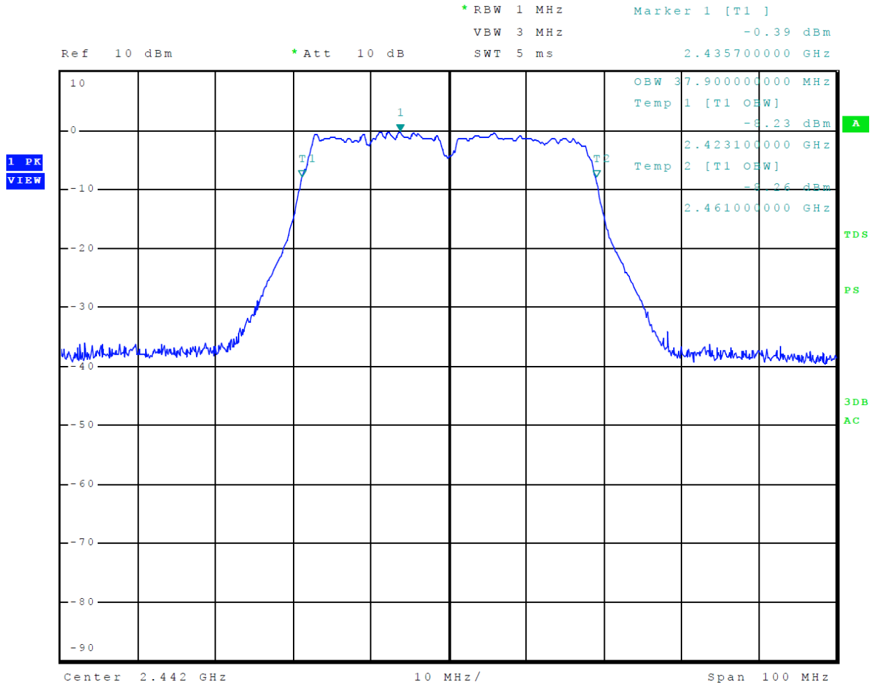
Figure 39 Plot of 99% Occupied Bandwidth Mode 9 802.11n40
