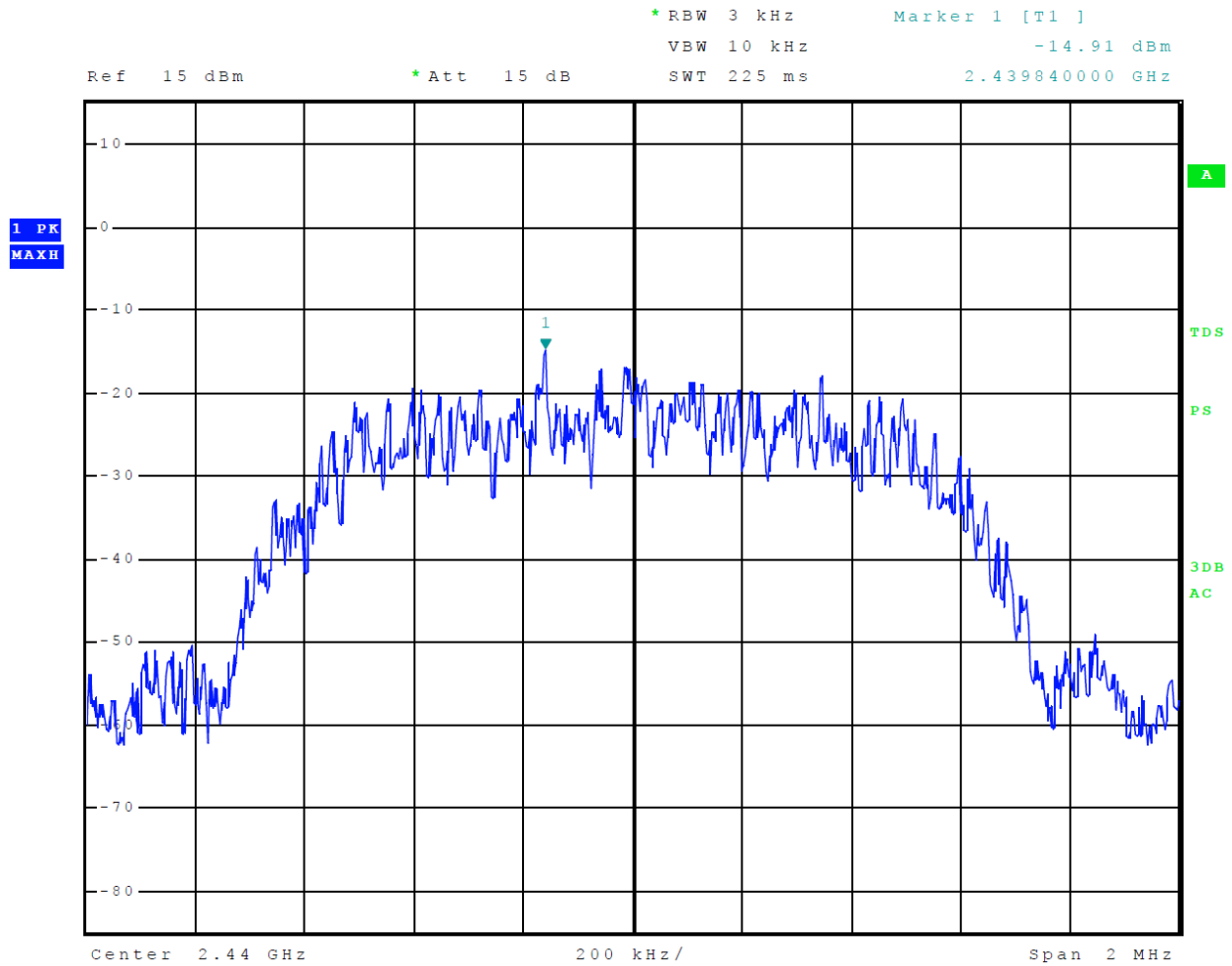
Figure 41 Plot of Transmitter Power Spectral Density Mode 4 BT 3EDR
