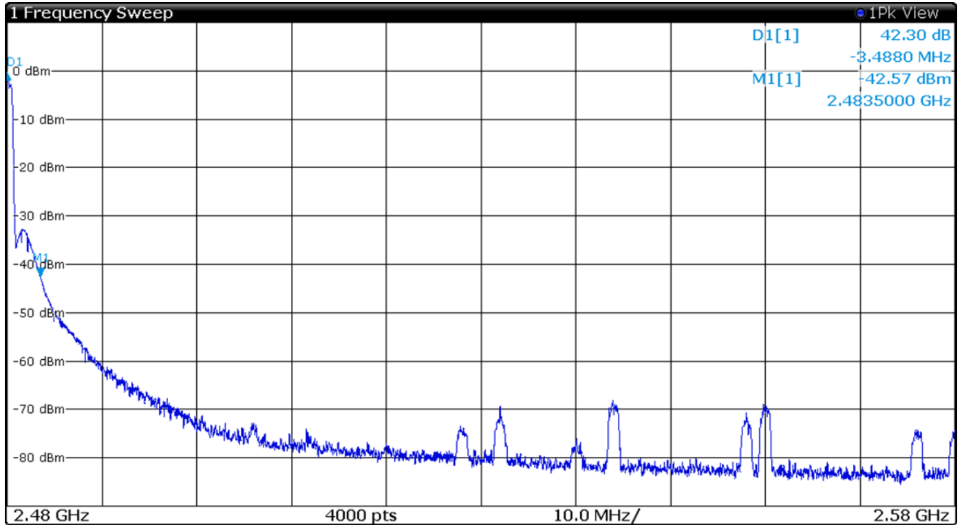
Figure 20 Plot of Transmitter Emissions High Band Edge Mode 4 BR 2EDR
