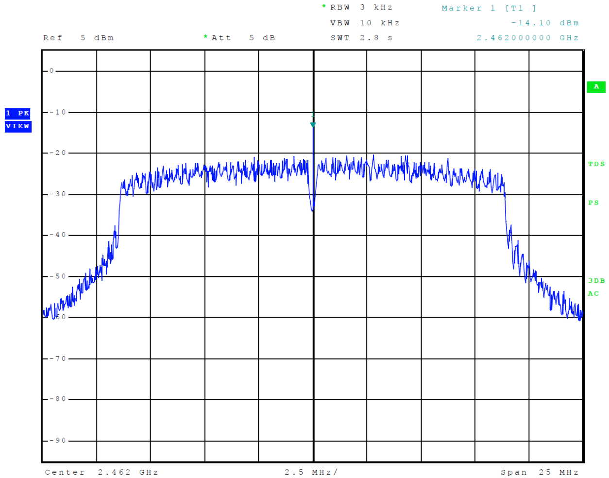
Figure 45 Plot of Transmitter Power Spectral Density Mode 8 802.11n
