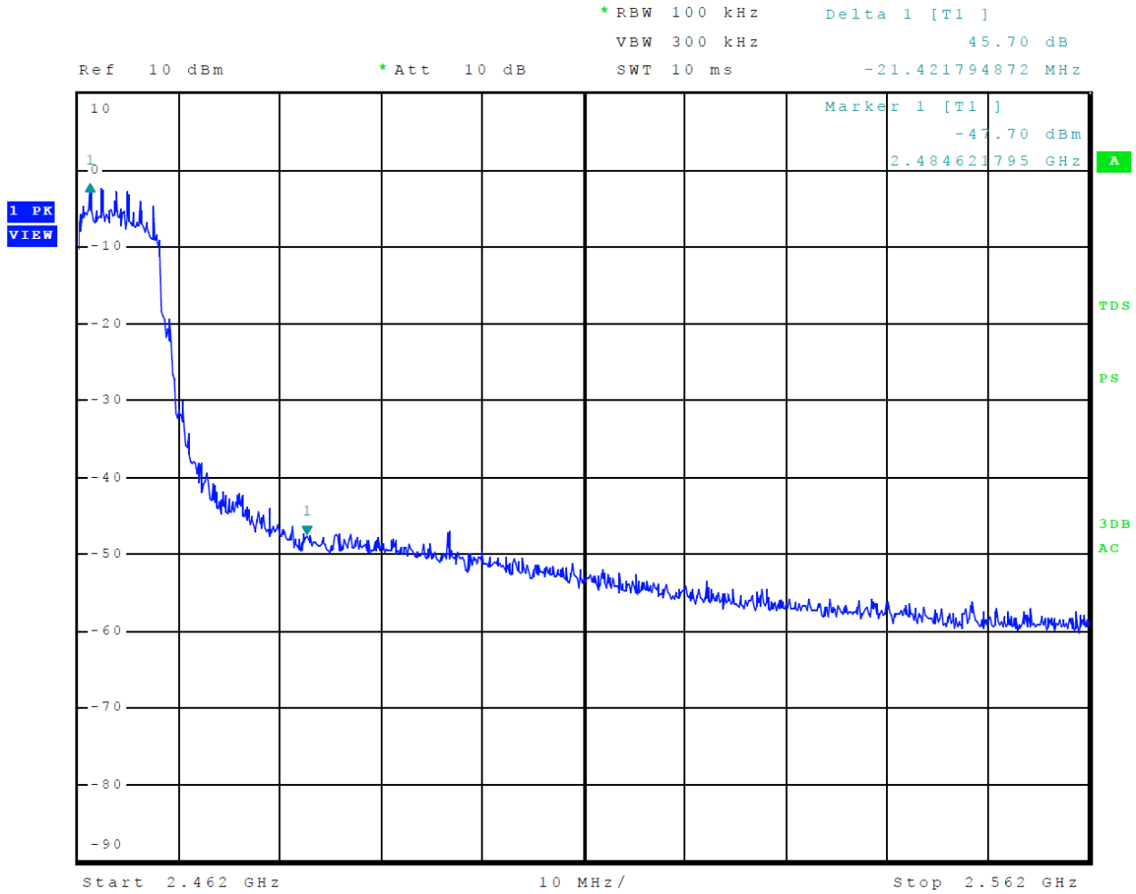
Figure 23 Plot of Transmitter Emissions High Band Edge Mode 7 802.11g
