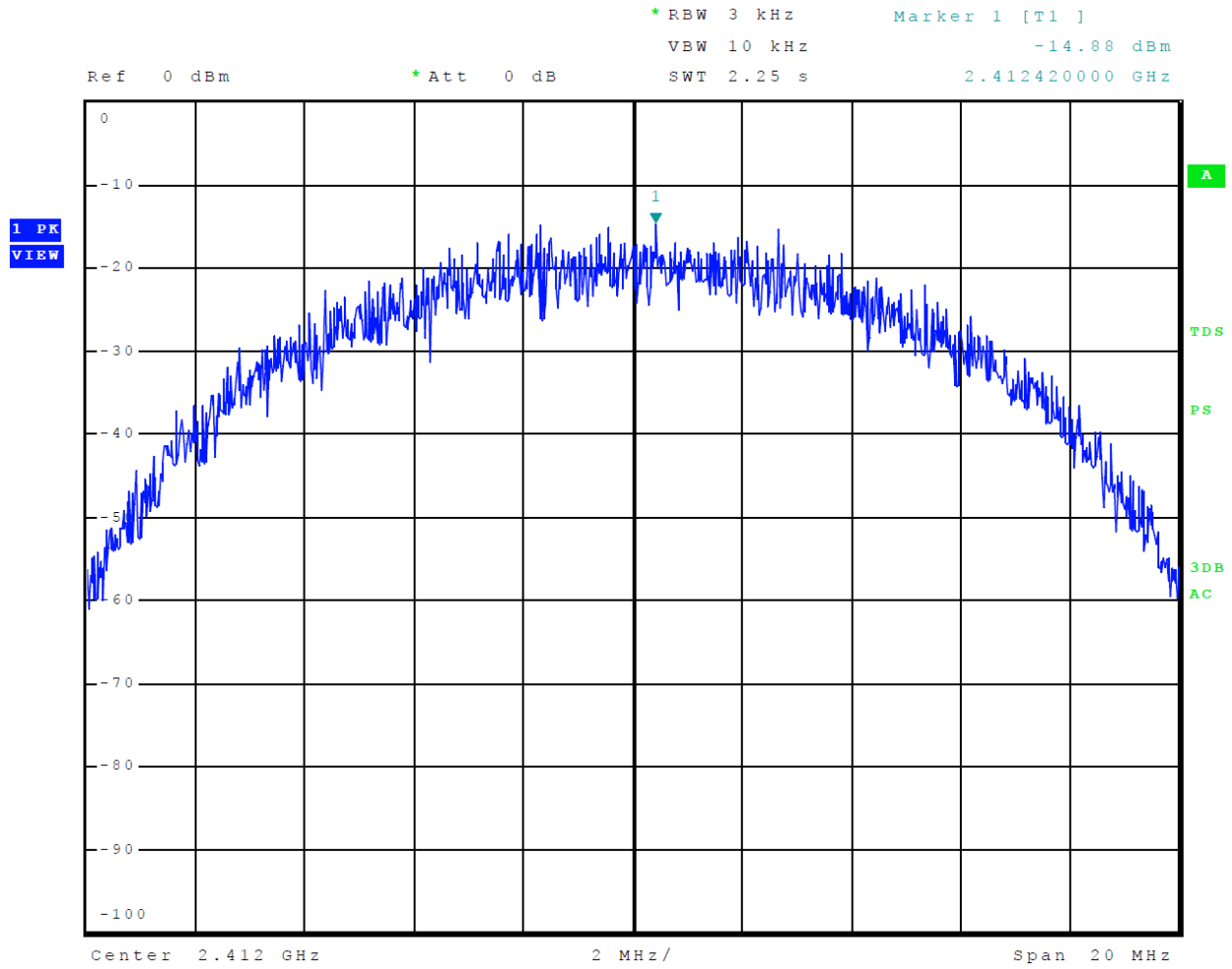
Figure 43 Plot of Transmitter Power Spectral Density Mode 6 802.11b
