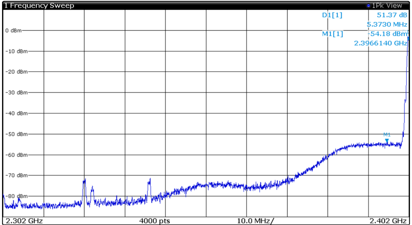
Figure 14 Plot of Transmitter Emissions Low Band Edge Mode 5 BT BLE
