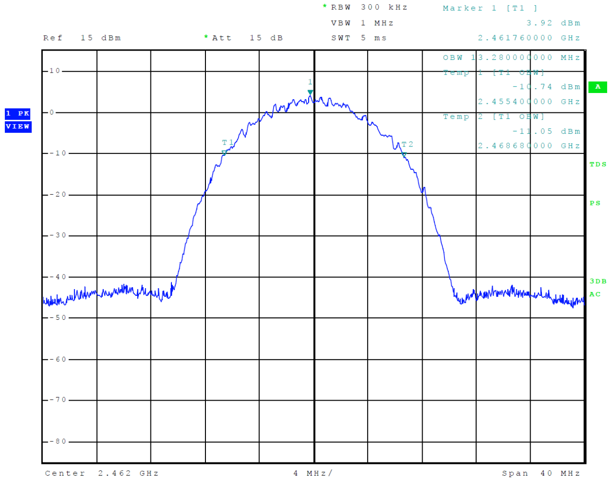
Figure 33 Plot of 99% Occupied Bandwidth Mode 6 802.11b
