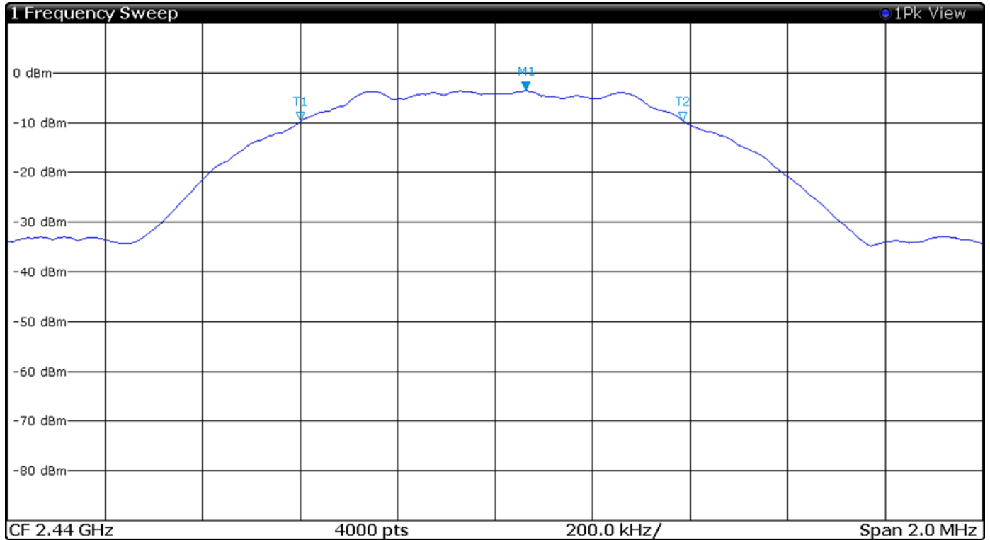
Figure 30 Plot of 6-dB Occupied Bandwidth Mode 5 BT BLE
