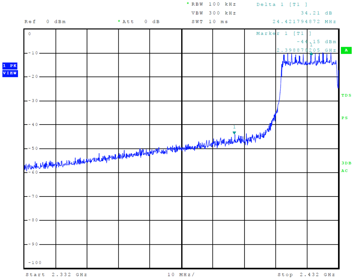
Figure 18 Plot of Transmitter Emissions Low Band Edge Mode 9 802.11n40
