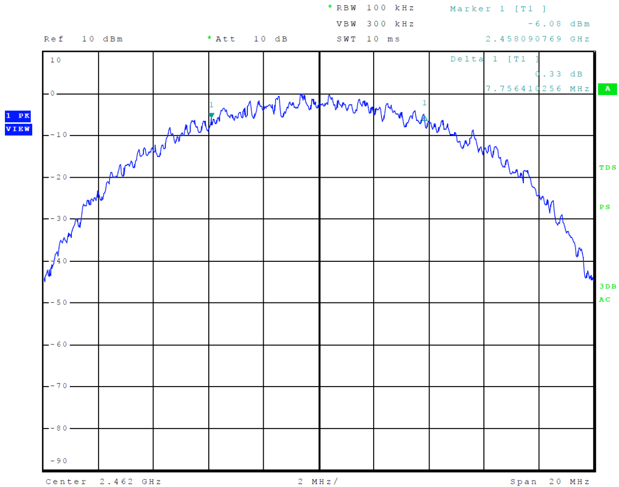
Figure 32 Plot of 6-dB Occupied Bandwidth Mode 6 802.11b
