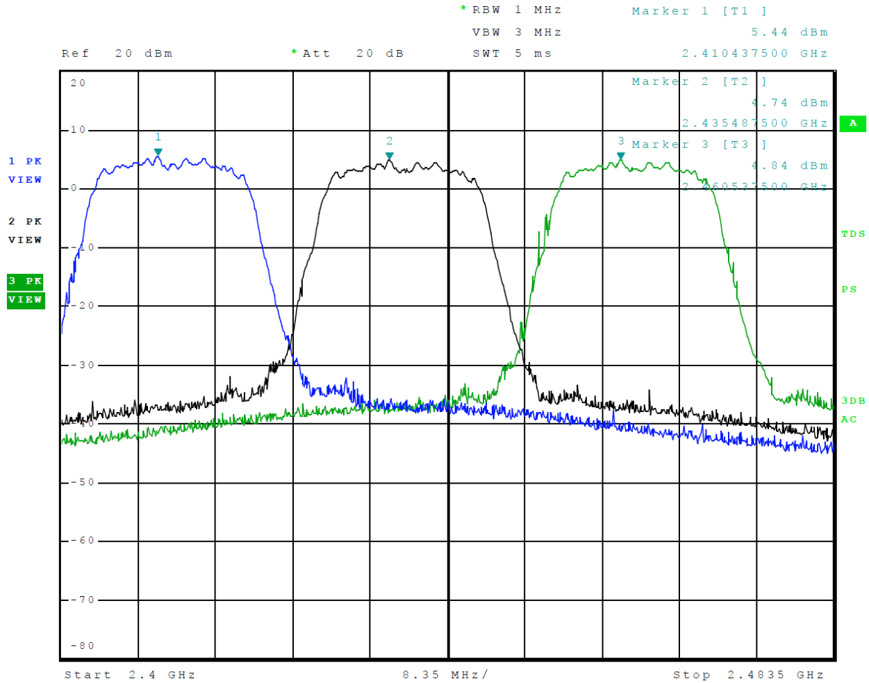
Figure 10 Plot of Transmitter Operation in 2412-2462 MHz Mode 8 802.11n
