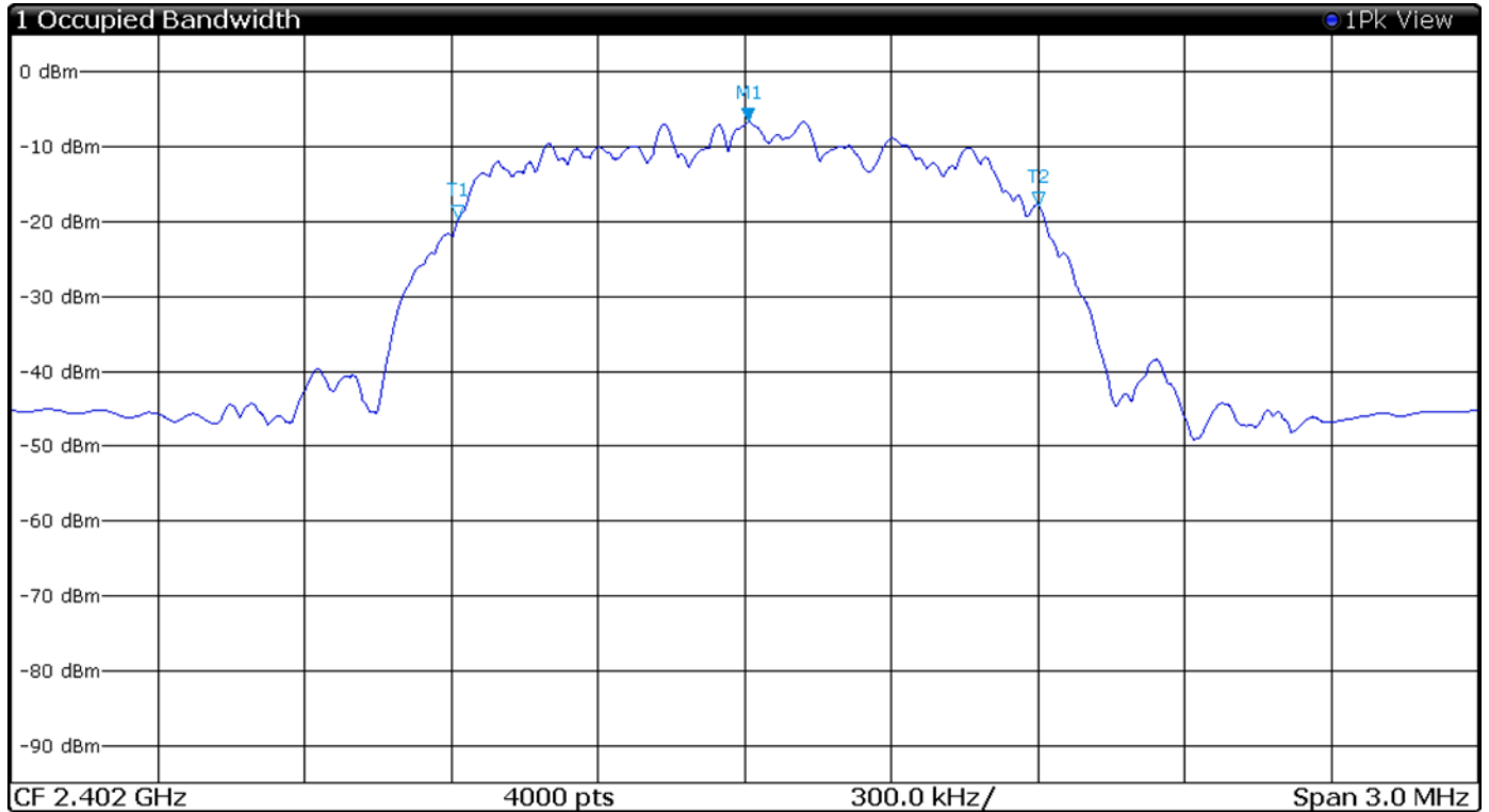
Figure 29 Plot of 99% Occupied Bandwidth Mode 4 BT 3EDR
