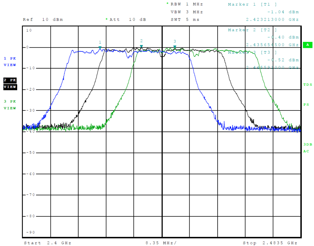
Figure 11 Plot of Transmitter Operation in 2412-2462 MHz Mode 9 802.11n40
