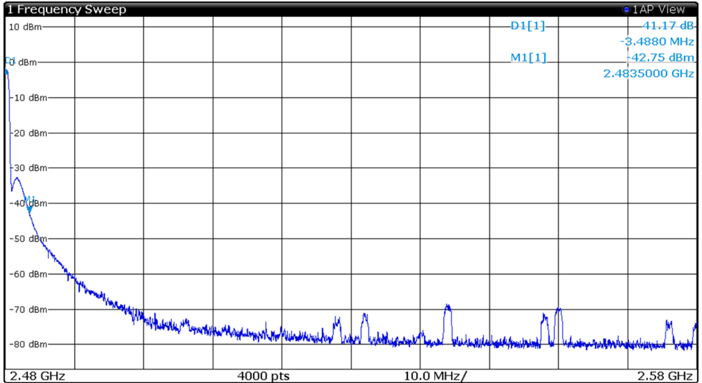
Figure 19 Plot of Transmitter Emissions High Band Edge Mode 3 BT 2EDR
