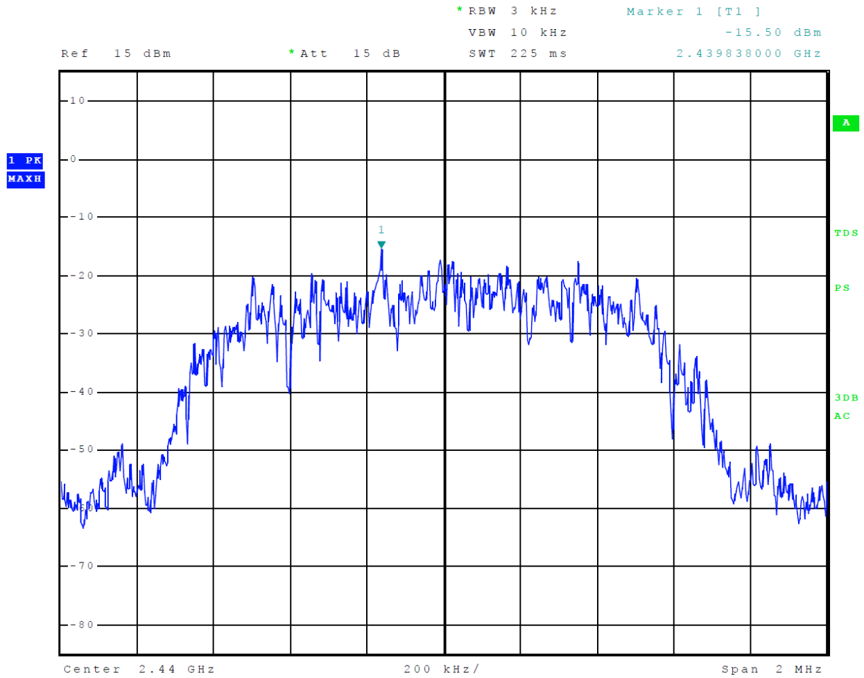
Figure 40 Plot of Transmitter Power Spectral Density Mode 3 BT 2EDR
