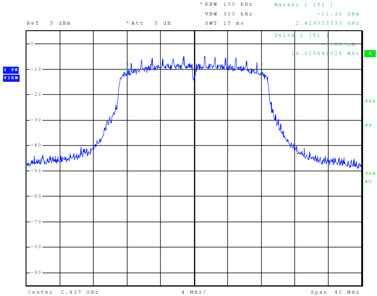
Figure 36 Plot of 6-dB Occupied Bandwidth Mode 8 802.11n
