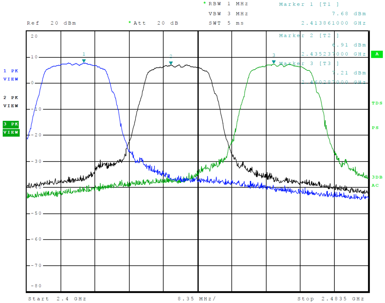
Figure 9 Plot of Transmitter Operation in 2412-2462 MHz Mode 7 802.11g
