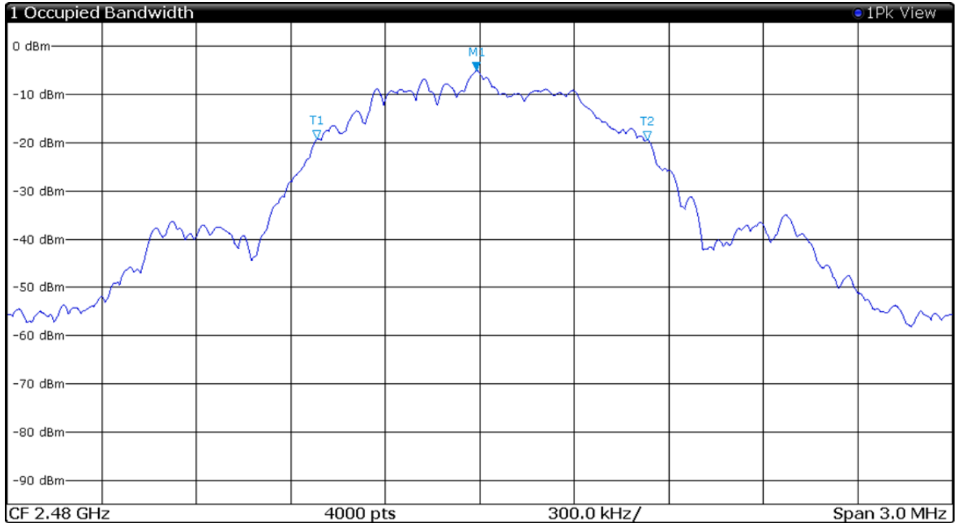
Figure 31 Plot of 99% Occupied Bandwidth Mode 5 BT BLE
