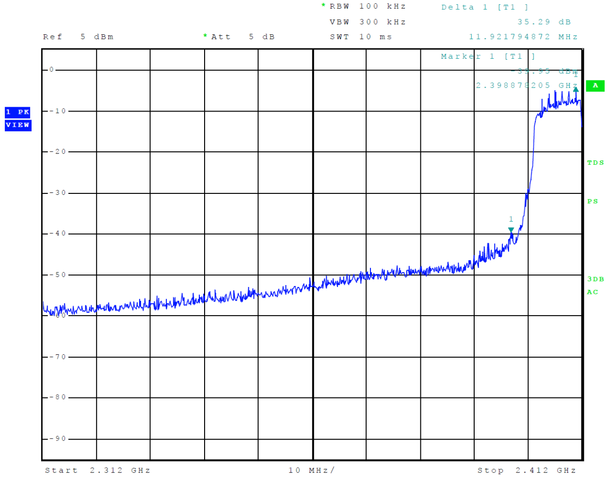
Figure 17 Plot of Transmitter Emissions Low Band Edge Mode 8 802.11n
