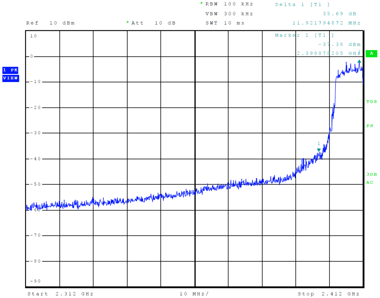
Figure 16 Plot of Transmitter Emissions Low Band Edge Mode 7 802.11g
