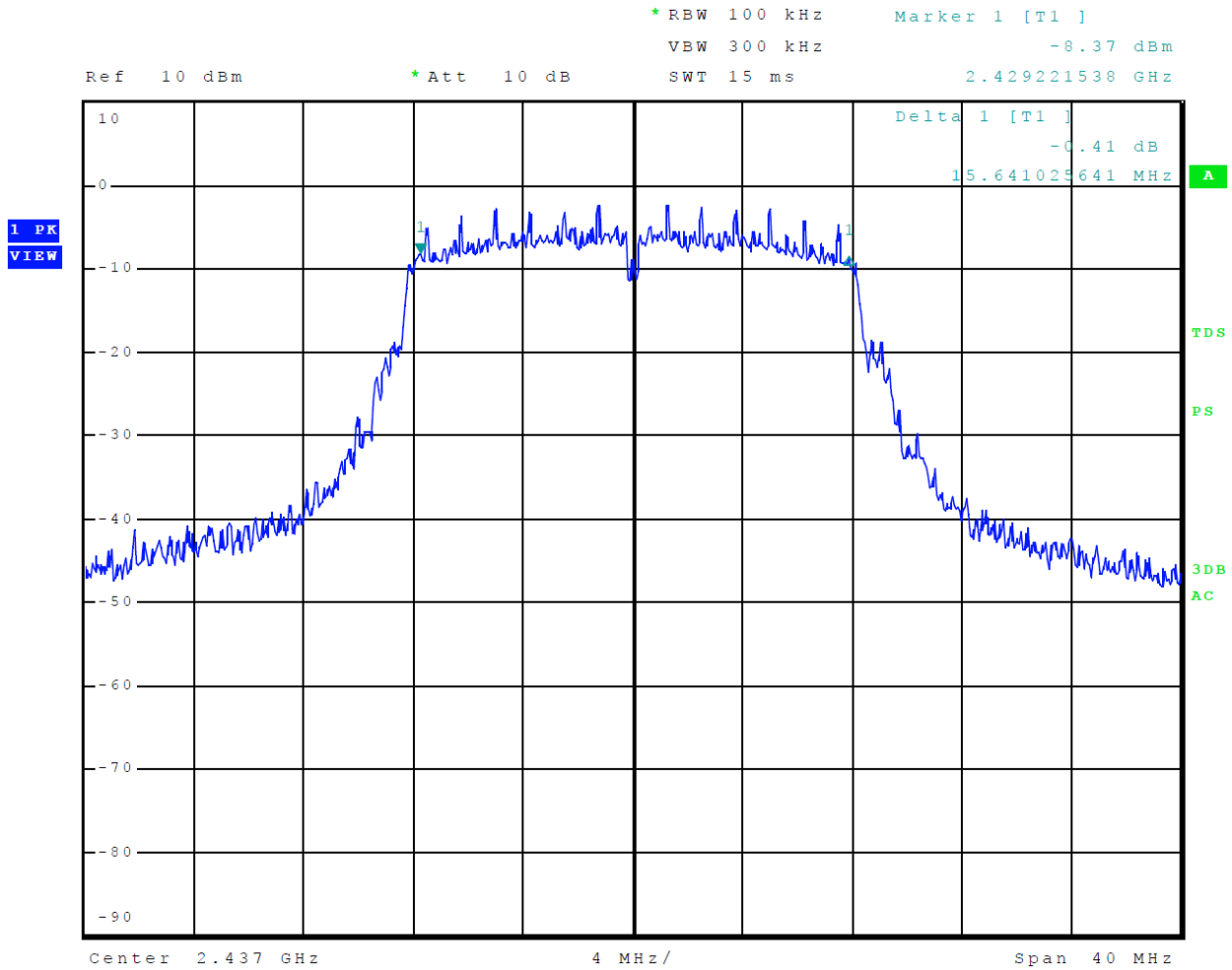
Figure 34 Plot of 6-dB Occupied Bandwidth Mode 7 802.11g
