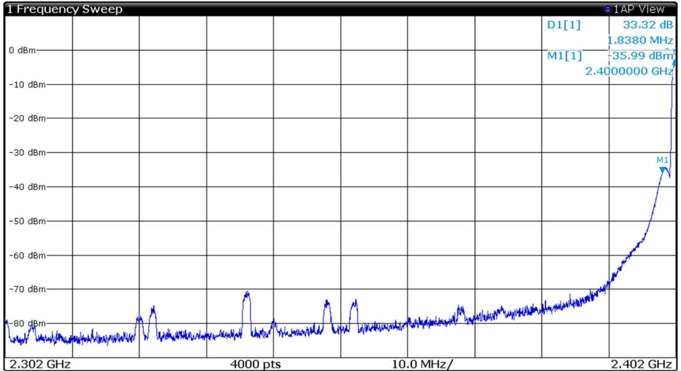
Figure 12 Plot of Transmitter Emissions Low Band Edge Mode 3 BT 2EDR
