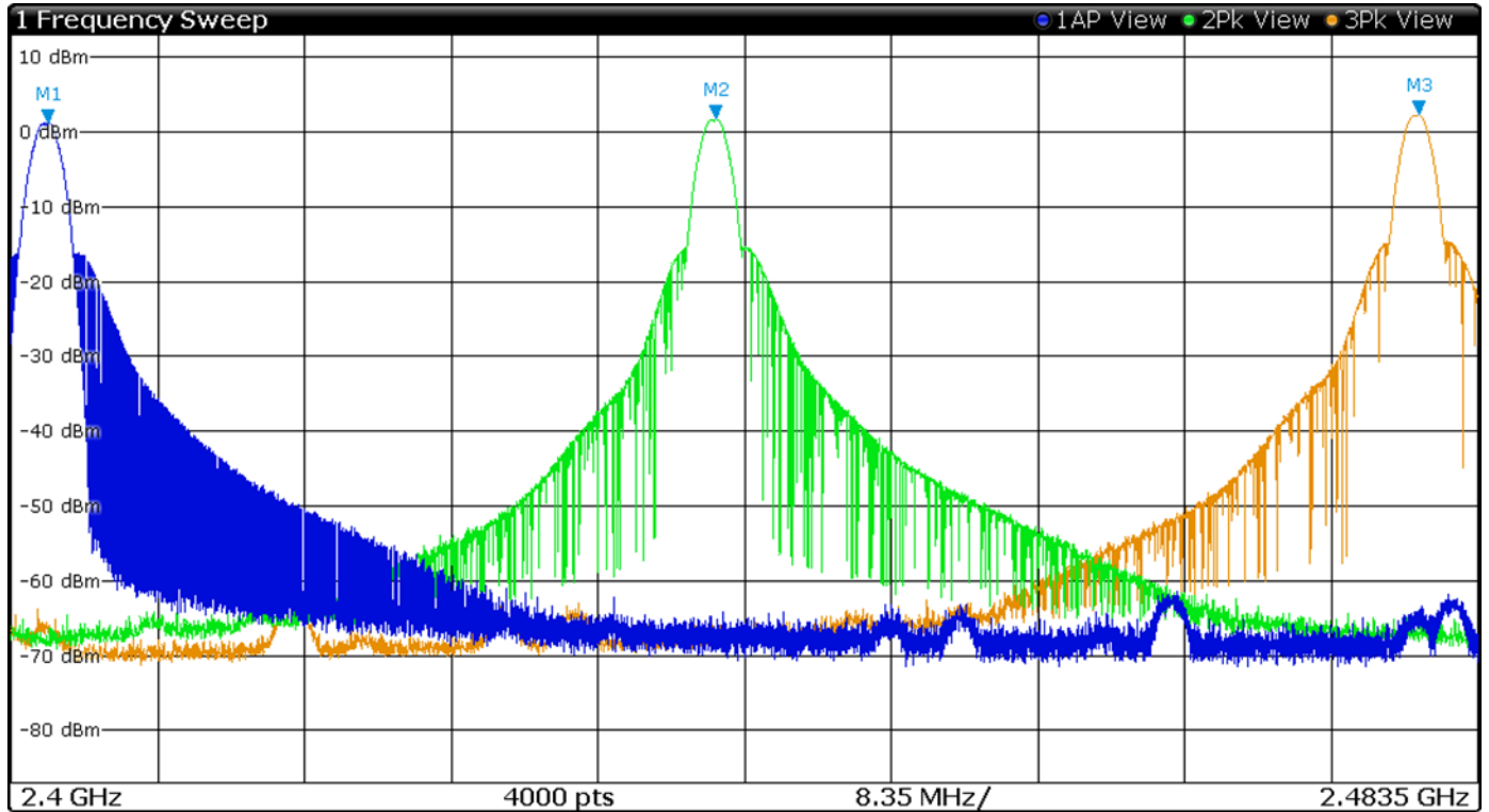
Figure 5 Plot of Transmitter Emissions Operation in 2402-2480 MHz Mode 3 BT 2EDR
