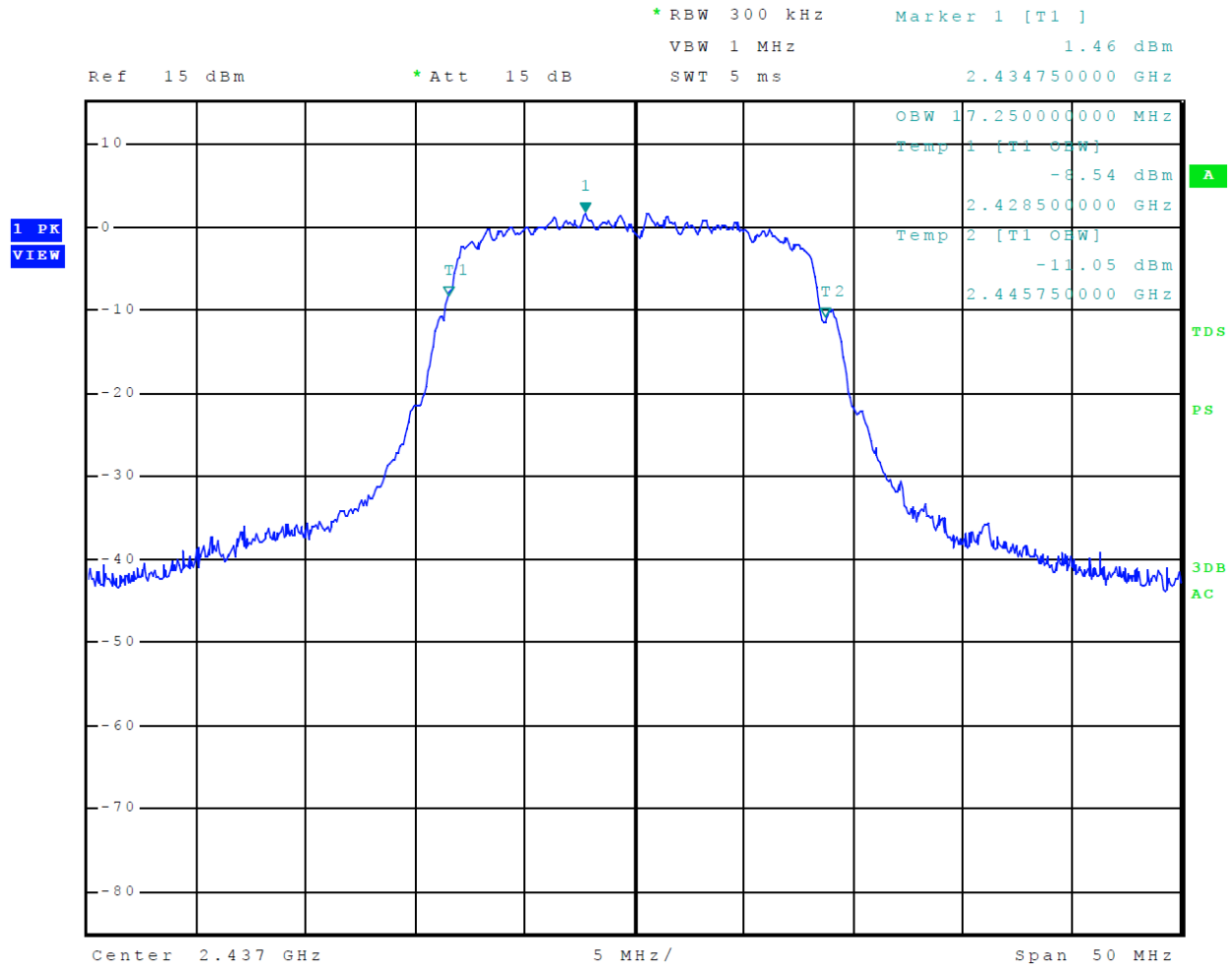
Figure 35 Plot of 99% Occupied Bandwidth Mode 7 802.11g
