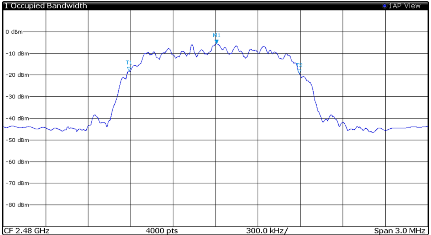
Figure 27 Plot of 99% Occupied Bandwidth Mode 3 BT 2EDR
