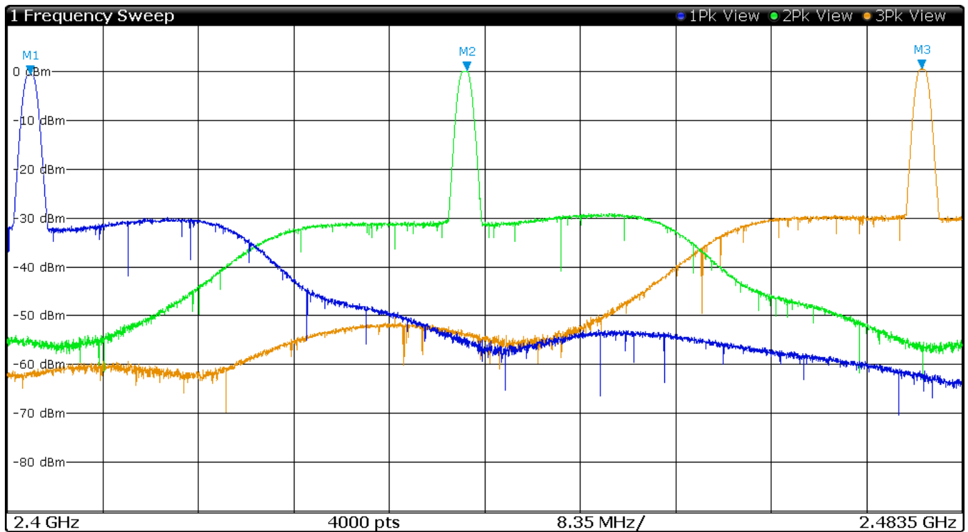
Figure 9 Plot of Transmitter Emissions Operation in 2402-2480 MHz Mode 2 BT BR (GFSK)
