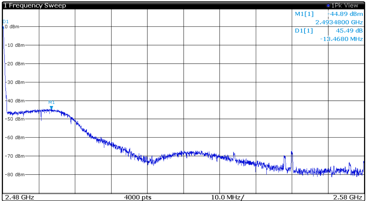
Figure 11 Plot of Transmitter Emissions High Band Edge Mode 2 BT BR (GFSK)
