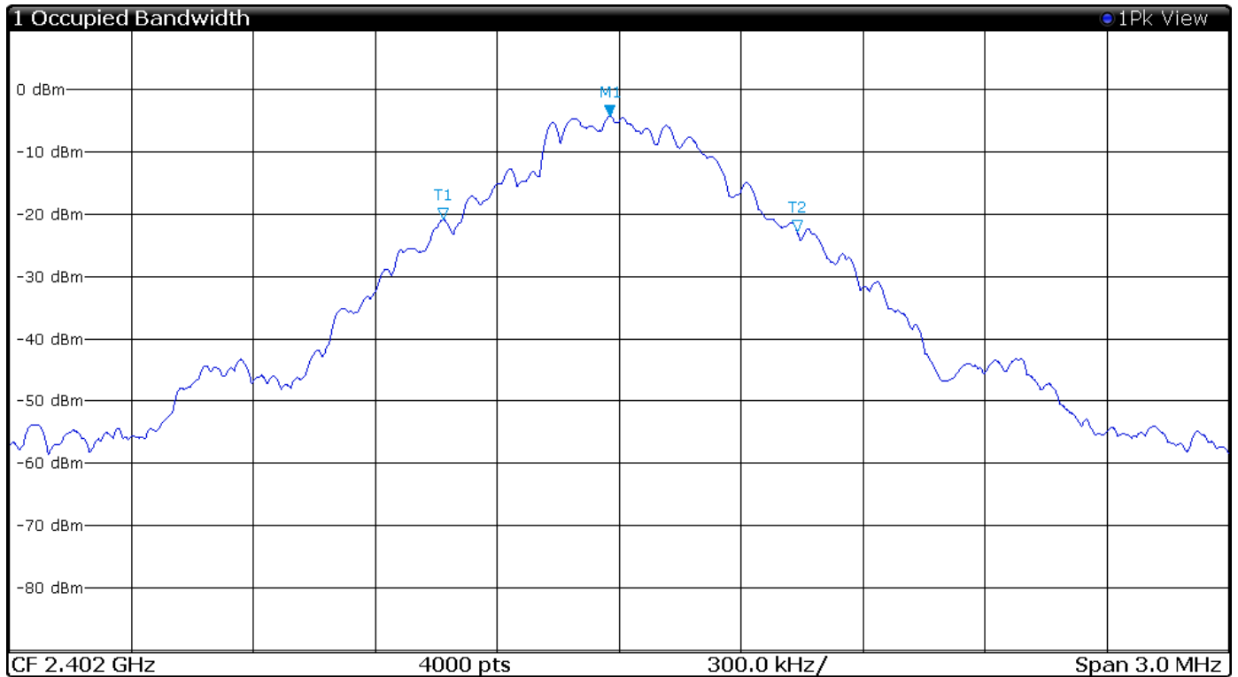
Figure 12 Plot of Transmitter Emissions 99% Occupied Bandwidth Mode 2 BT BR (GFSK)
