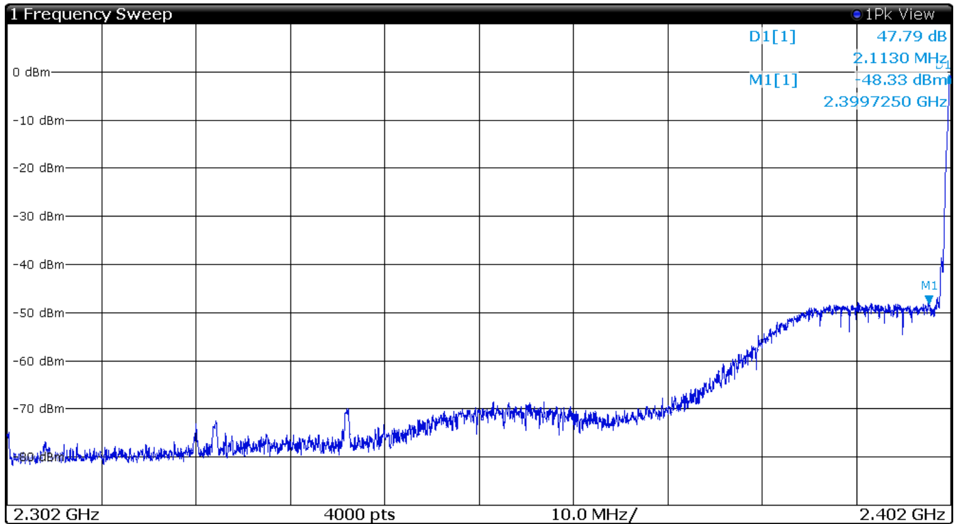
Figure 6 Plot of Transmitter Emissions Low Band Edge Mode 1 ANT (GFSK)
