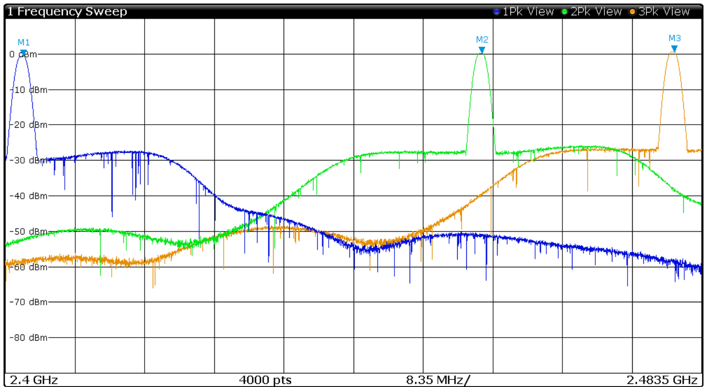
Figure 5 Plot of Transmitter Emissions Operation in 2402-2480 MHz Mode 1 ANT (GFSK)
