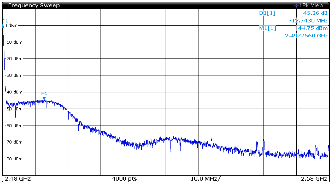
Figure 7 Plot of Transmitter Emissions High Band Edge Mode 1 ANT (GFSK)
