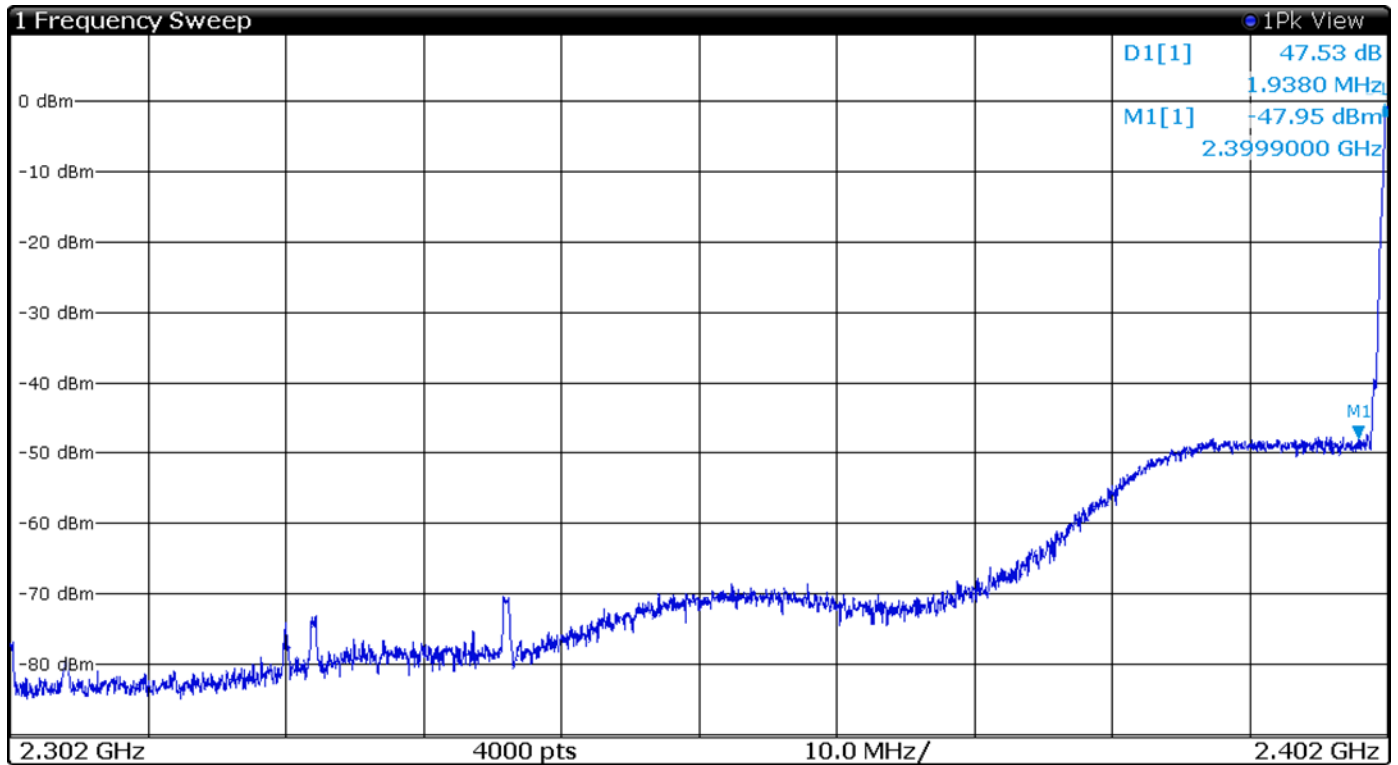
Figure 10 Plot of Transmitter Emissions Low Band Edge Mode 2 BT BR (GFSK)
