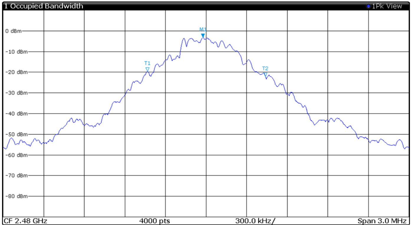
Figure 8 Plot of Transmitter Emissions 99% Occupied Bandwidth Mode 1 ANT (GFSK)
