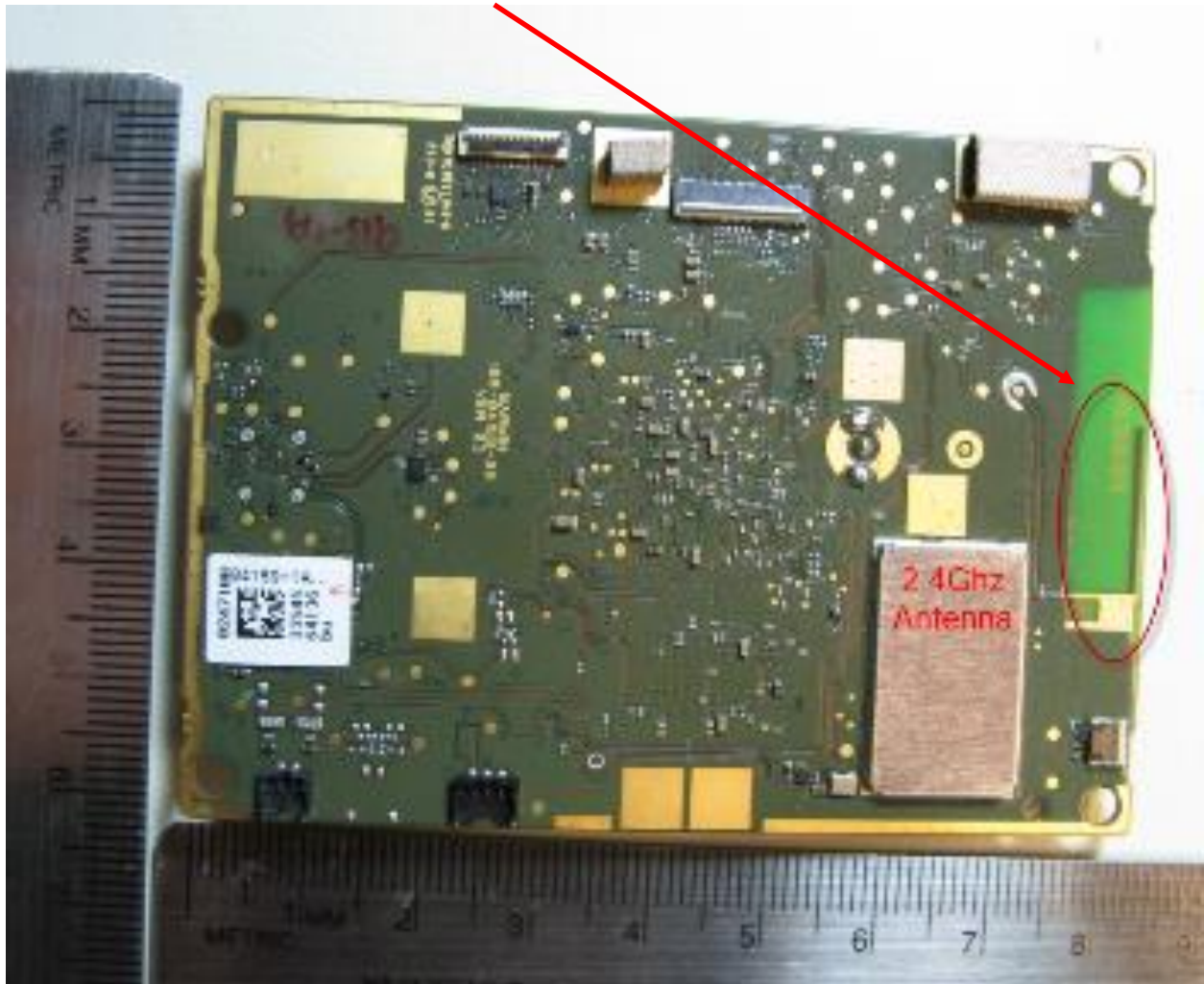
Front with shield and 2.4 GHz antenna
