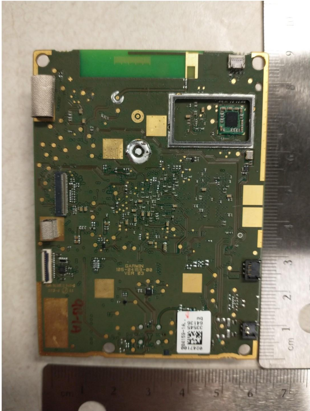
Front side without shield
