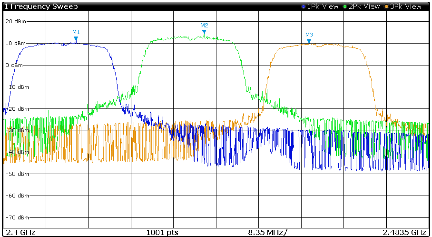
Figure 10 Plot of Transmitter Operation in 2412-2462 MHz Mode 7 802.11n
