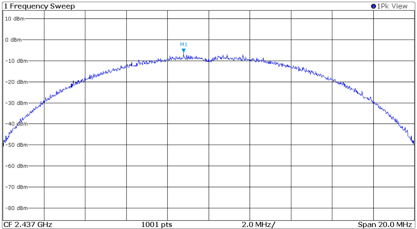
Figure 38 Plot of Transmitter Power Spectral Density Mode 5 802.11b
