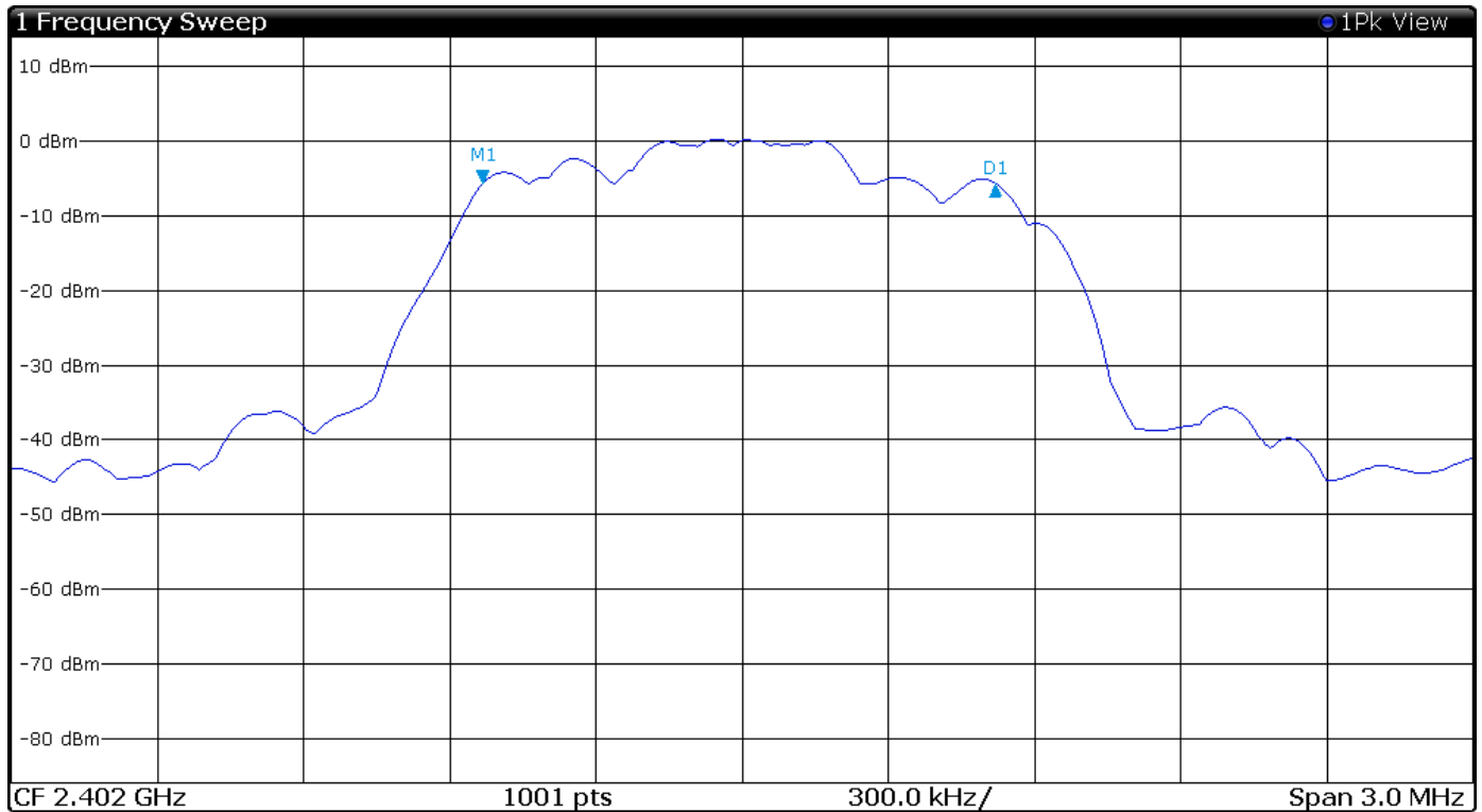
Figure 23 Plot of 6-dB Occupied Bandwidth Mode 2 BT 2EDR
