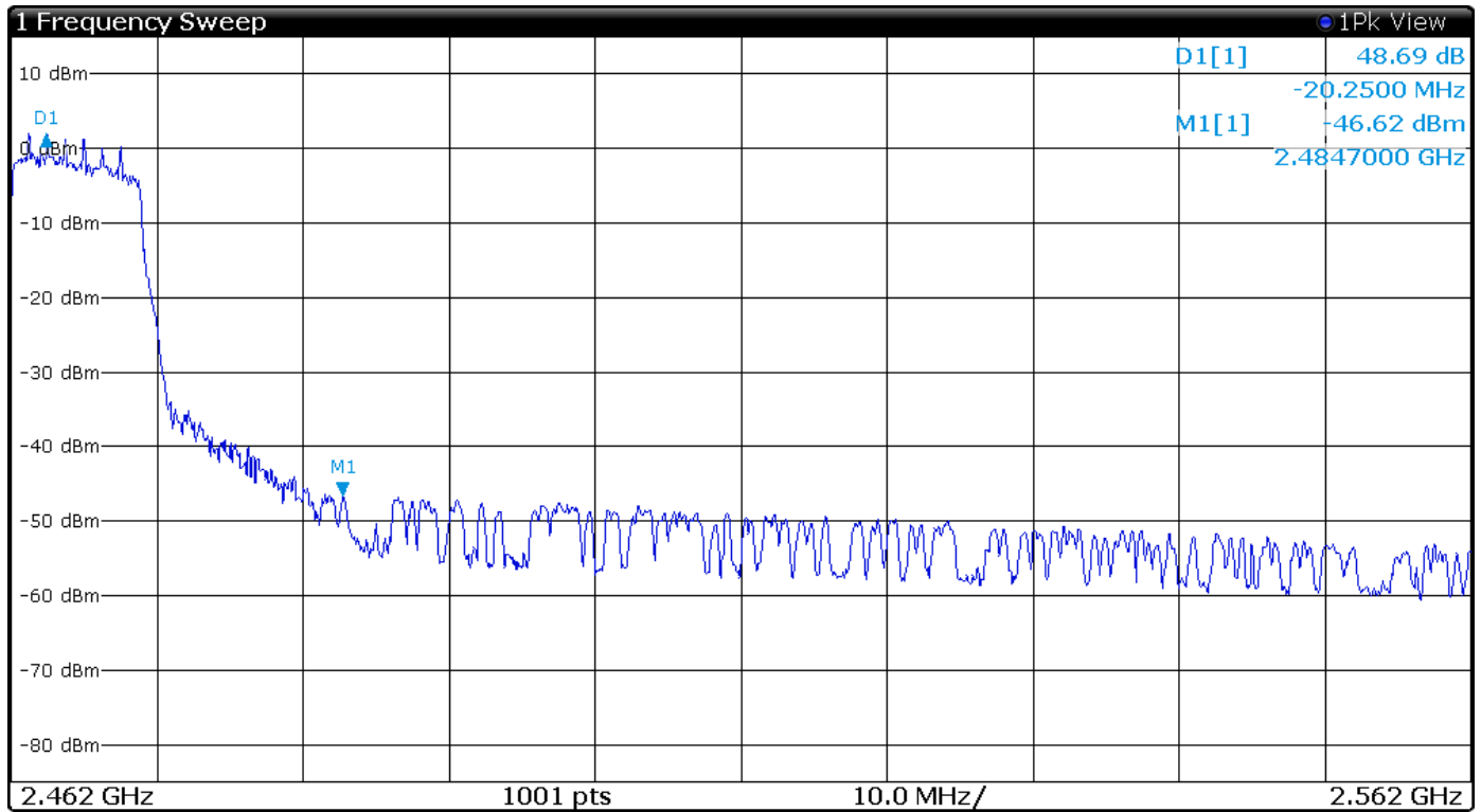
Figure 22 Plot of Transmitter Emissions High Band Edge Mode 7 802.11n
