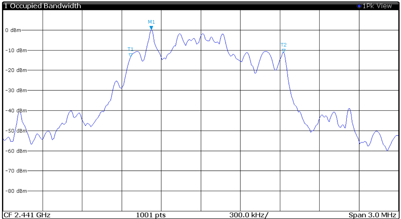
Figure 24 Plot of 99% Occupied Bandwidth Mode 2 BT 2EDR
