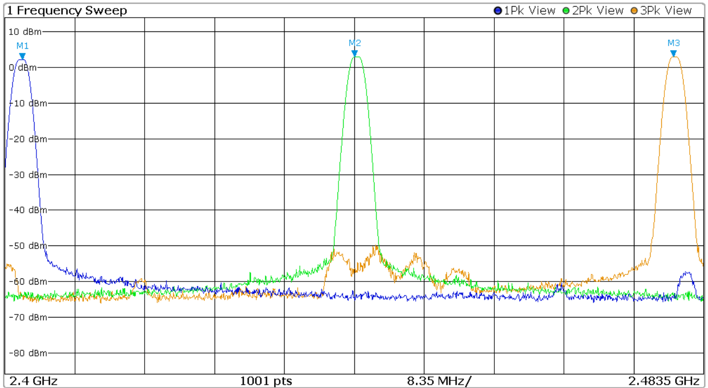
Figure 7 Plot of Transmitter Emissions Operation in 2402-2480 MHz Mode 4 BT BLE
