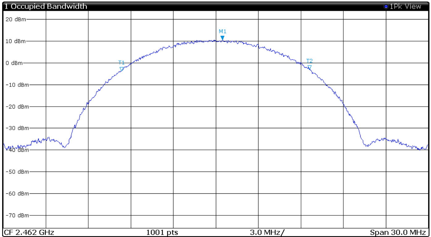
Figure 30 Plot of 99% Occupied Bandwidth Mode 5 802.11b
