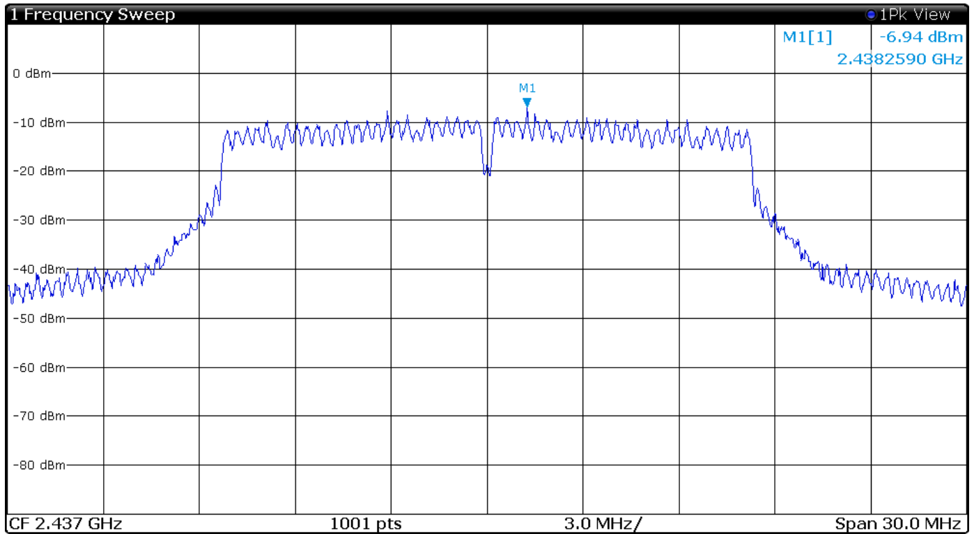
Figure 39 Plot of Transmitter Power Spectral Density Mode 6 802.11g
