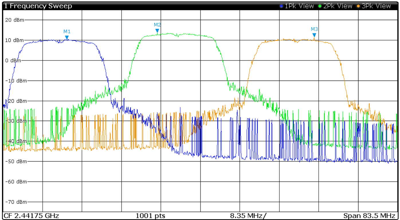
Figure 9 Plot of Transmitter Operation in 2412-2462 MHz Mode 6 802.11g
