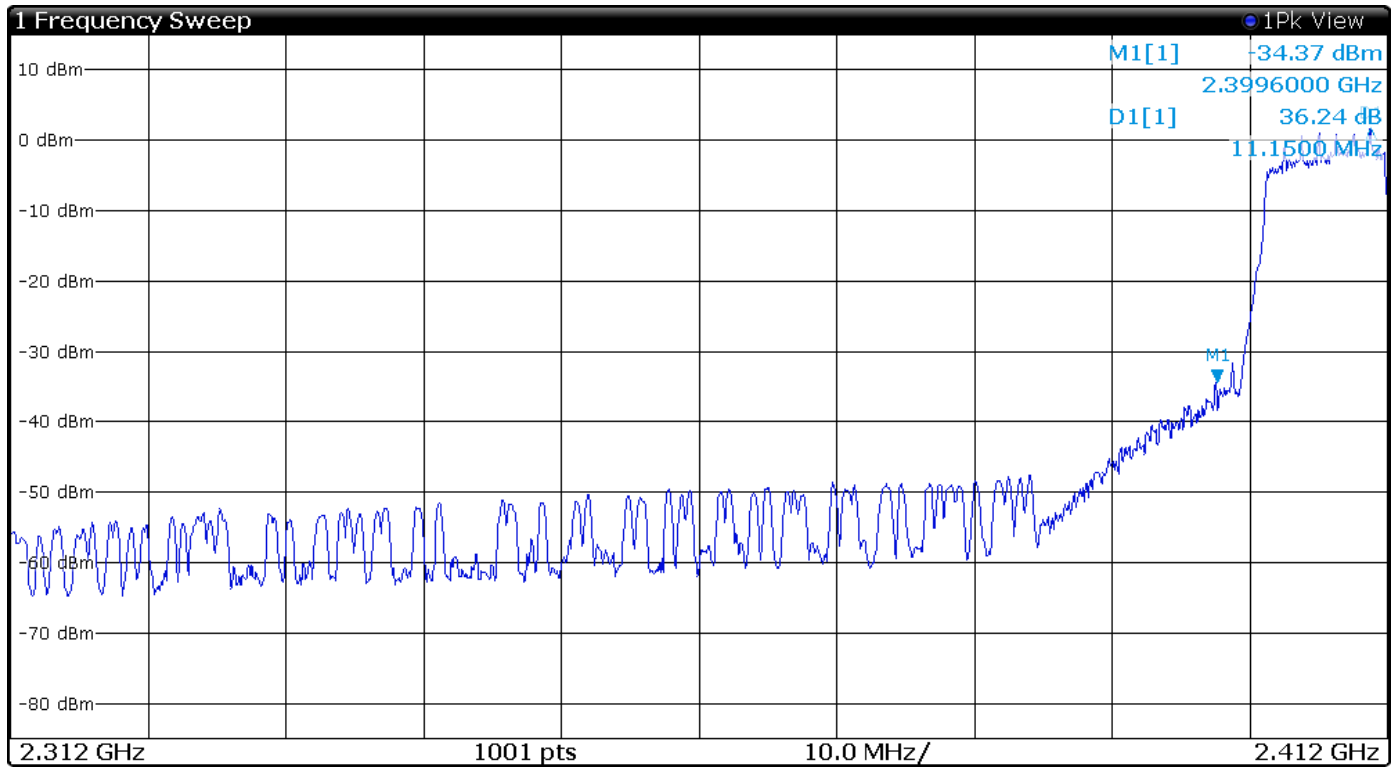
Figure 16 Plot of Transmitter Emissions Low Band Edge Mode 7 802.11n
