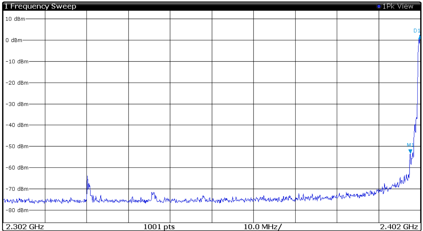
Figure 11 Plot of Transmitter Emissions Low Band Edge Mode 2 BT 2EDR
