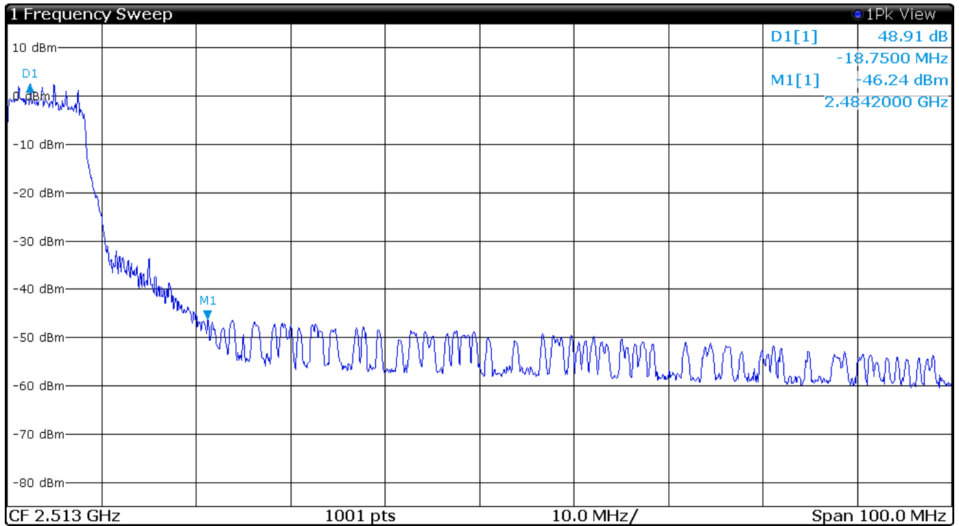
Figure 21 Plot of Transmitter Emissions High Band Edge Mode 6 802.11g
