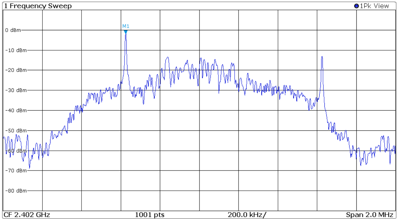
Figure 36 Plot of Transmitter Power Spectral Density Mode 3 BT 3EDR
