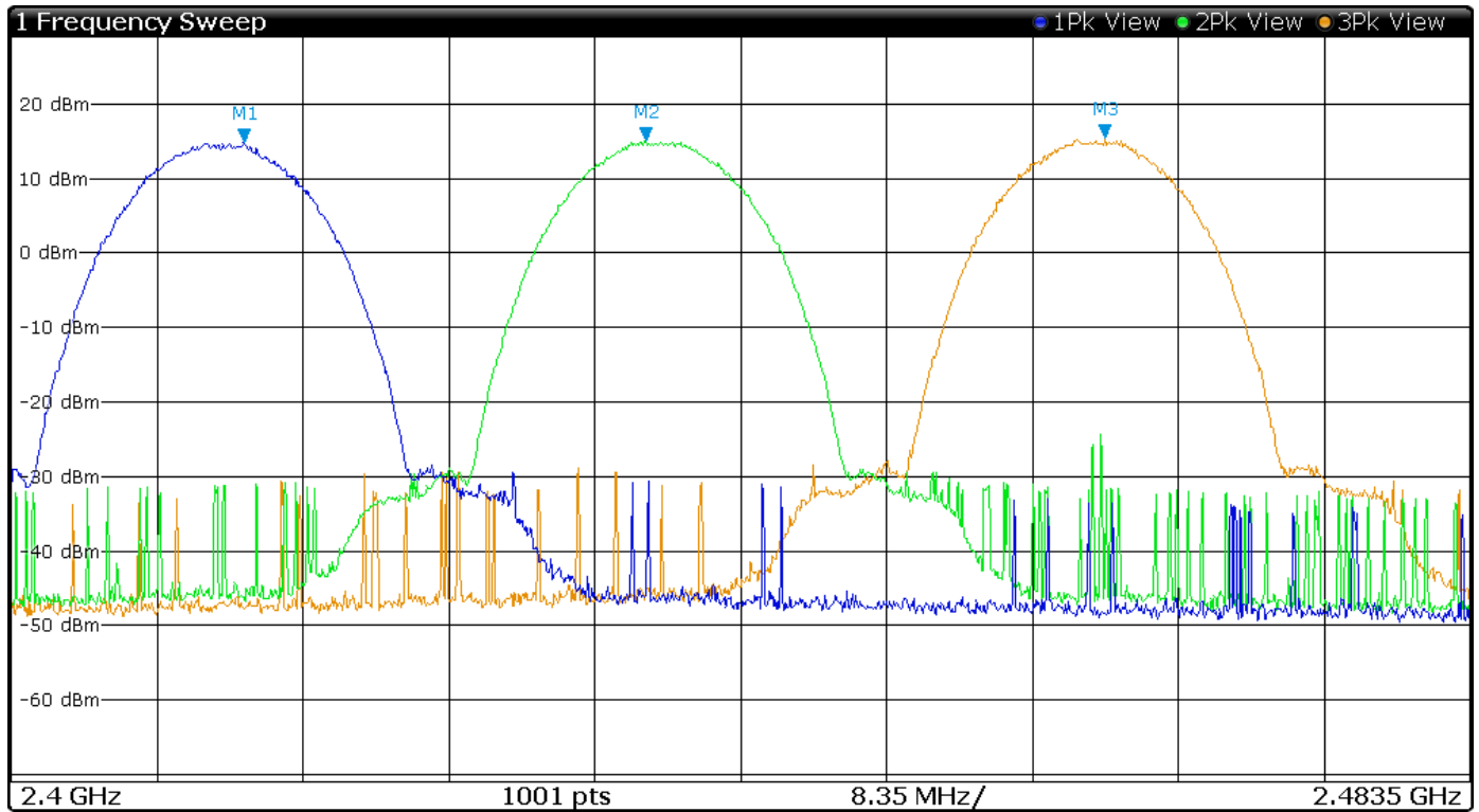
Figure 8 Plot of Transmitter Operation in 2412-2462 MHz Mode 5 802.11b
