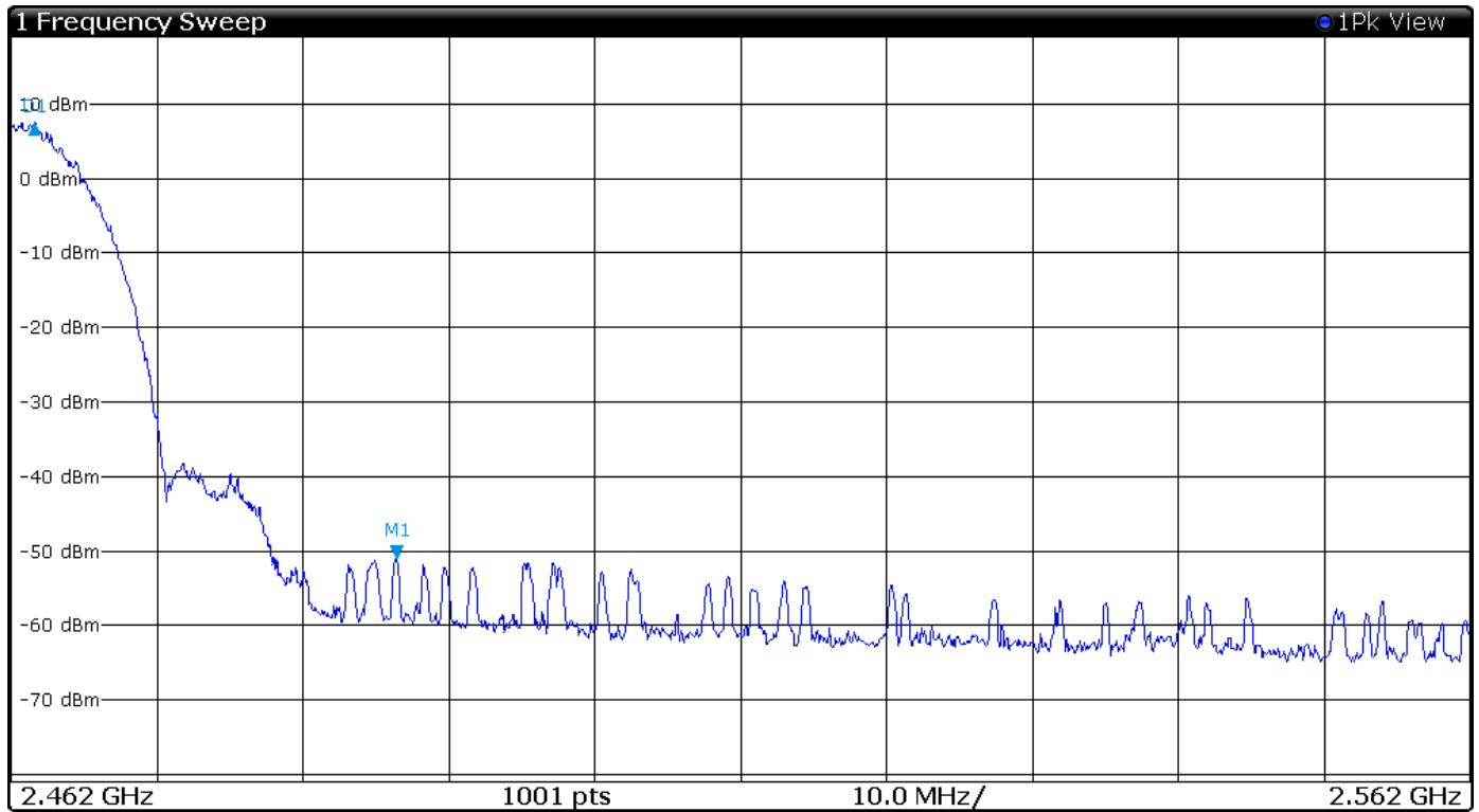
Figure 20 Plot of Transmitter Emissions High Band Edge Mode 5 802.11b
