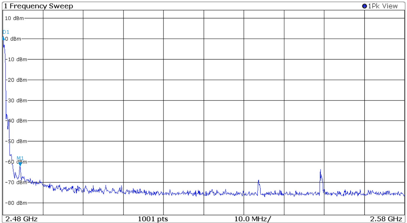
Figure 18 Plot of Transmitter Emissions High Band Edge Mode 3 BR 2EDR
