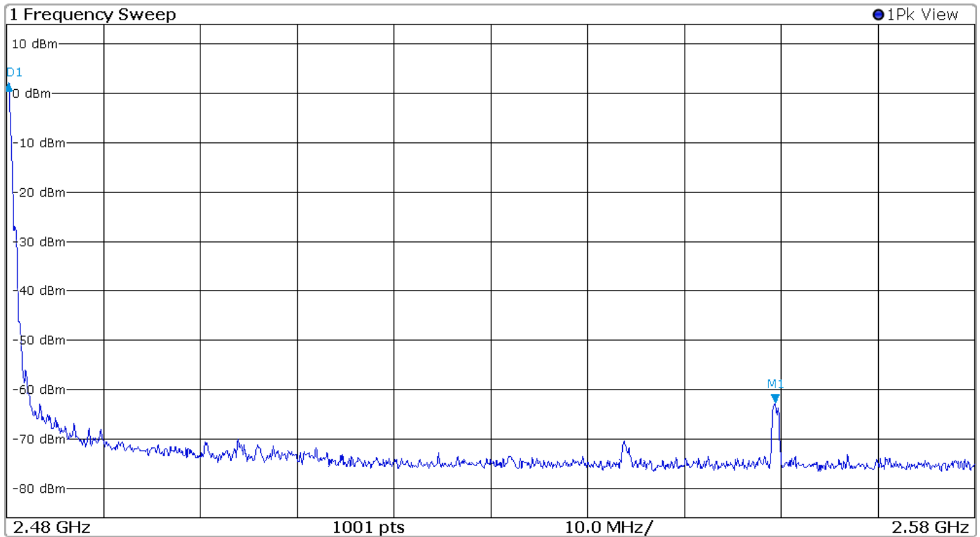
Figure 19 Plot of Transmitter Emissions High Band Edge Mode 4 BT BLE
