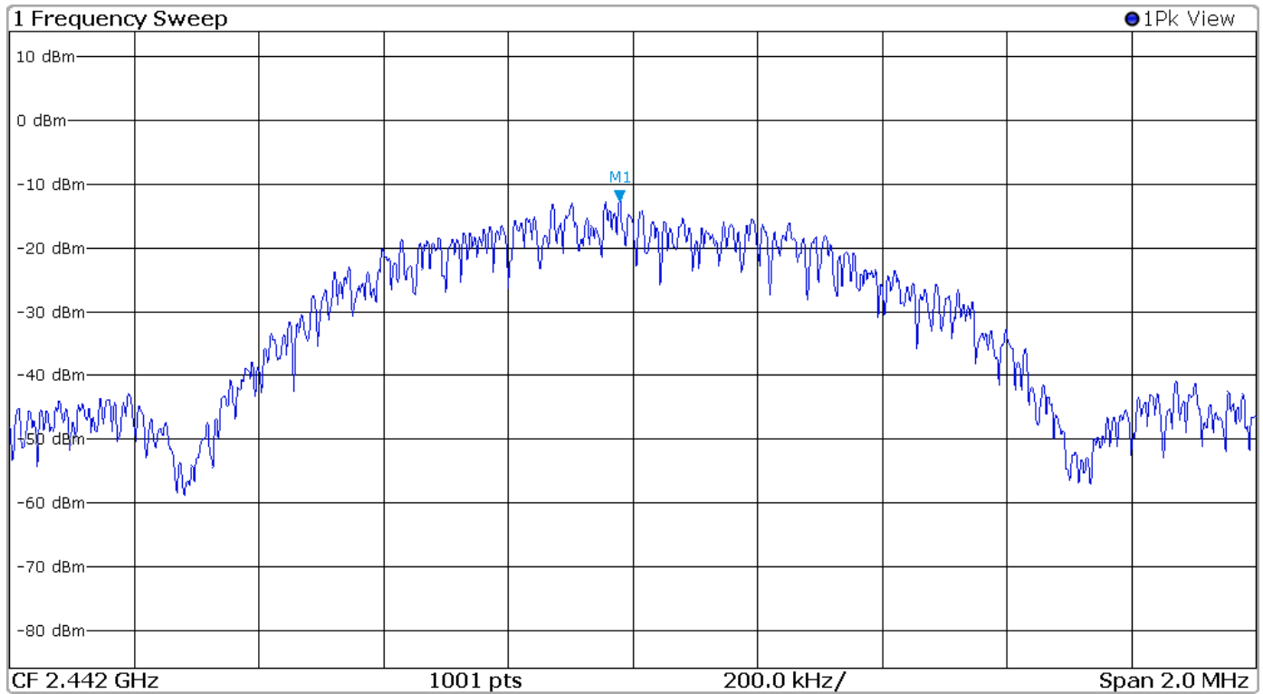
Figure 37 Plot of Transmitter Power Spectral Density Mode 4 BT BLE
