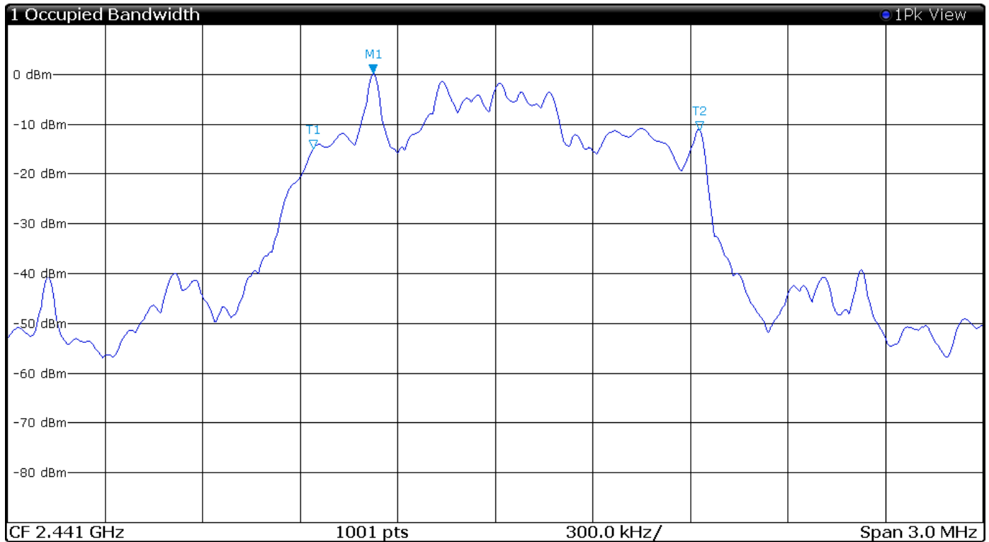
Figure 26 Plot of 99% Occupied Bandwidth Mode 3 BT 3EDR
