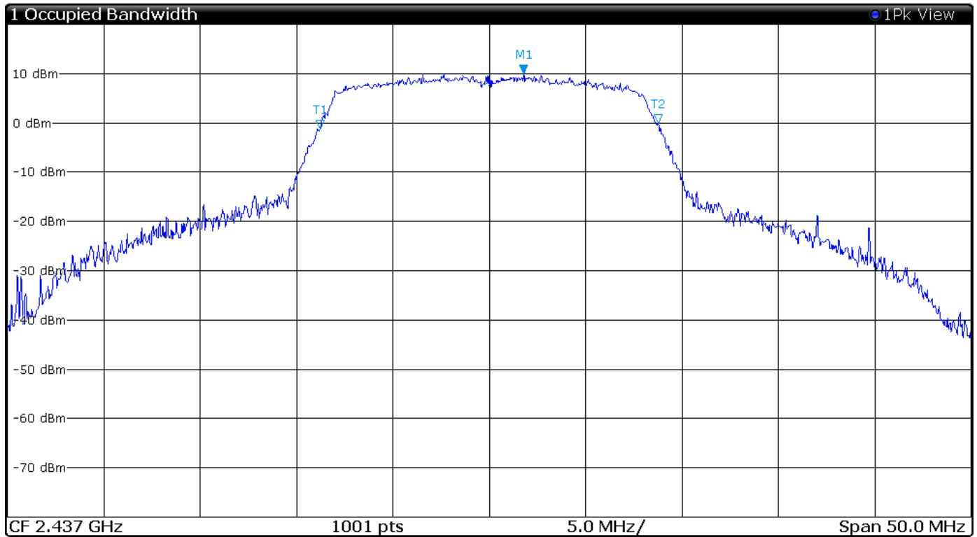
Figure 32 Plot of 99% Occupied Bandwidth Mode 7 802.11g
