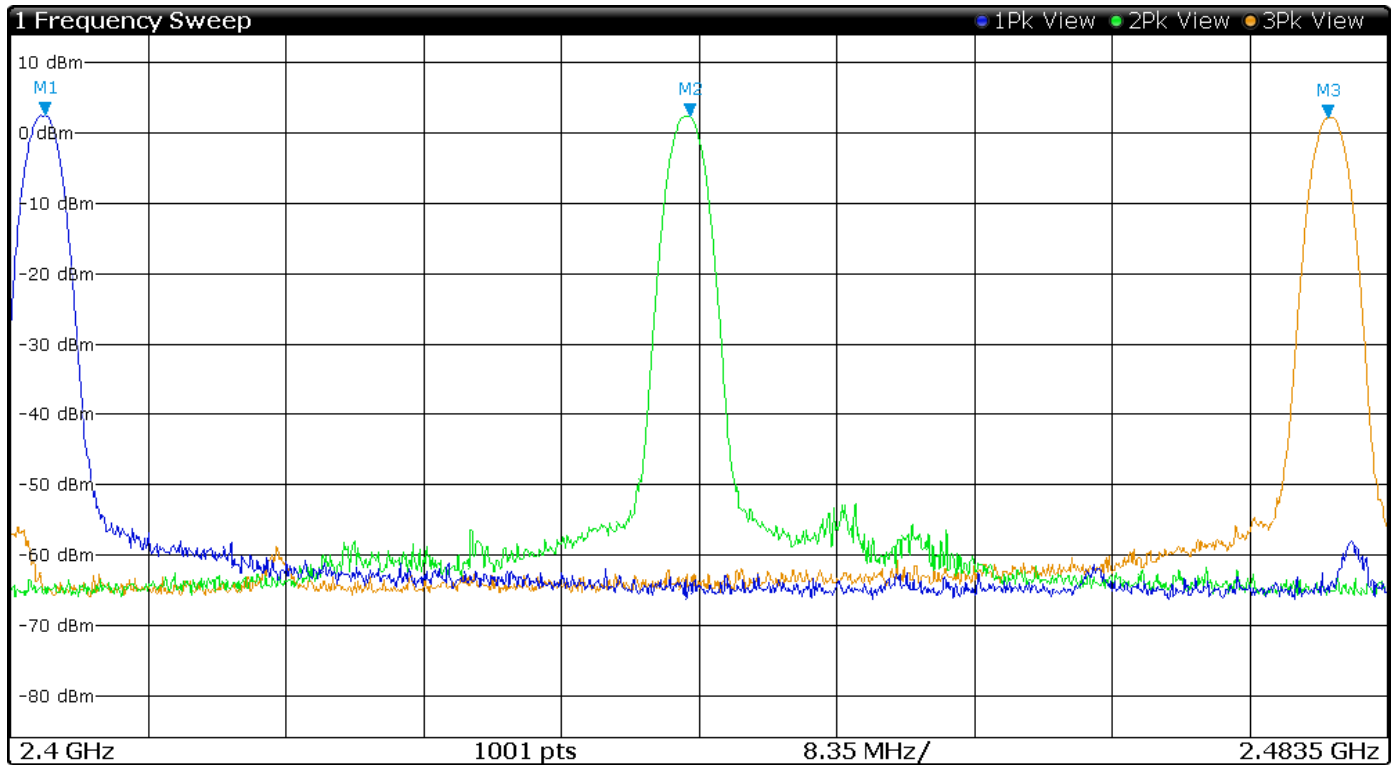
Figure 5 Plot of Transmitter Emissions Operation in 2402-2480 MHz Mode 2 BT 2EDR
