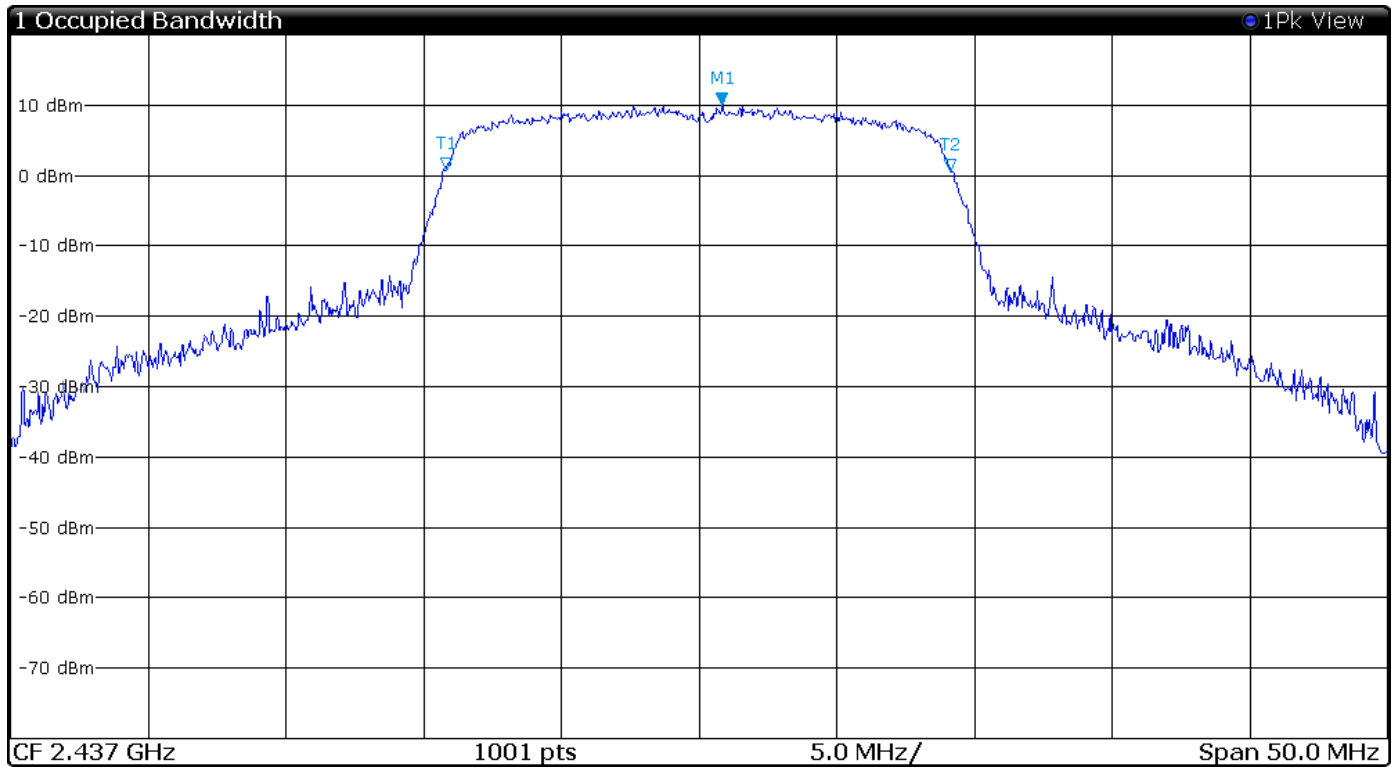
Figure 34 Plot of 99% Occupied Bandwidth Mode 9 802.11n
