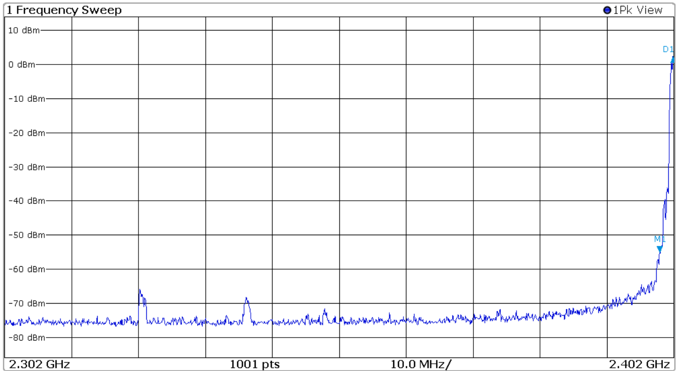
Figure 12 Plot of Transmitter Emissions Low Band Edge Mode 3 BT 3EDR
