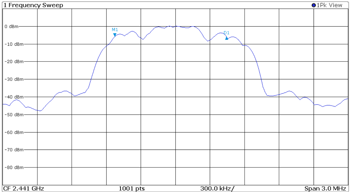
Figure 25 Plot of 6-dB Occupied Bandwidth Mode 3 BT 3EDR
