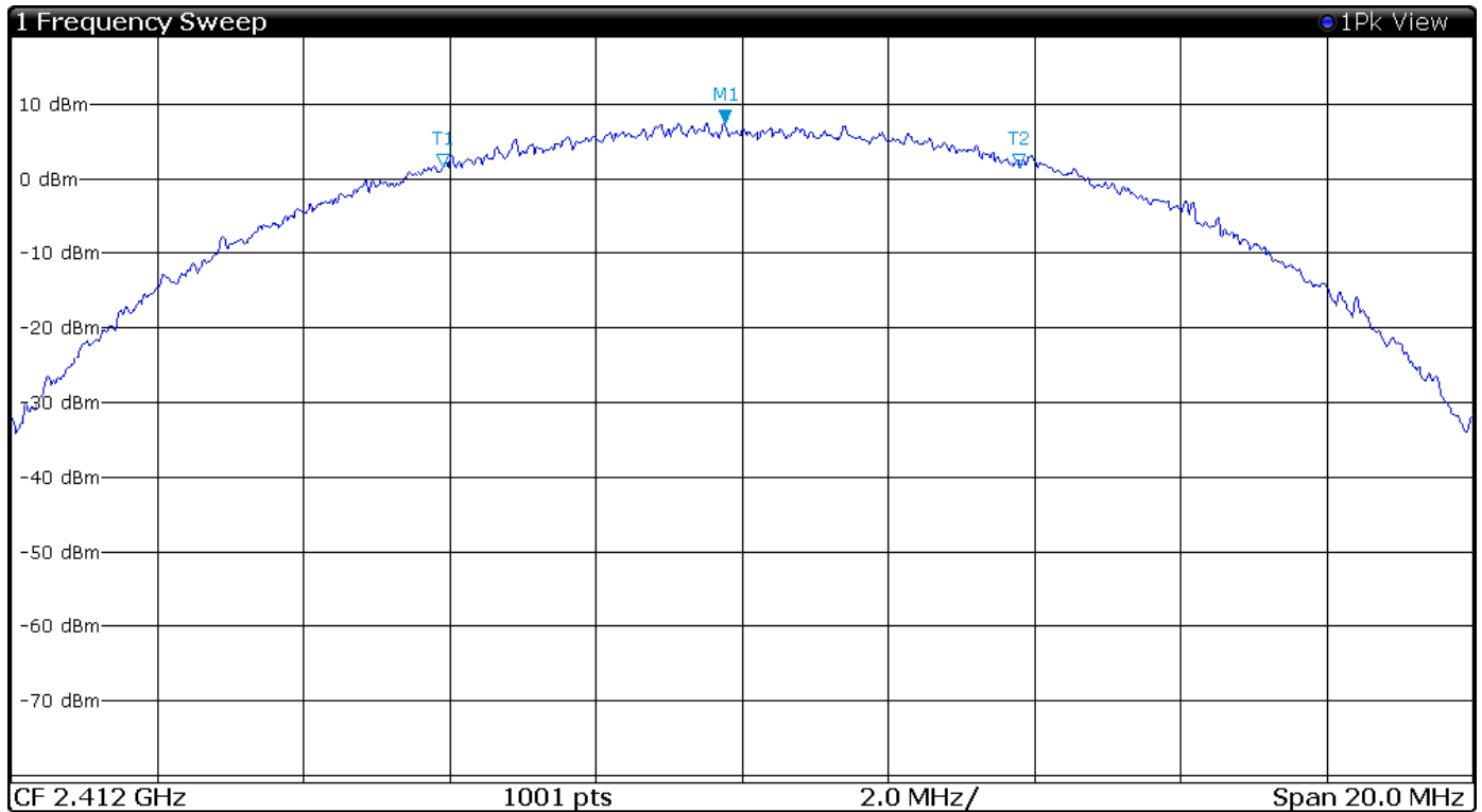
Figure 29 Plot of 6-dB Occupied Bandwidth Mode 5 802.11b
