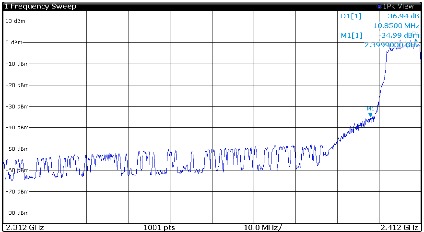
Figure 15 Plot of Transmitter Emissions Low Band Edge Mode 6 802.11g
