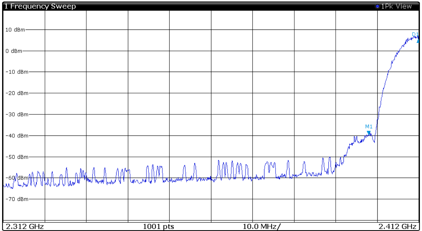
Figure 14 Plot of Transmitter Emissions Low Band Edge Mode 5 802.11b
