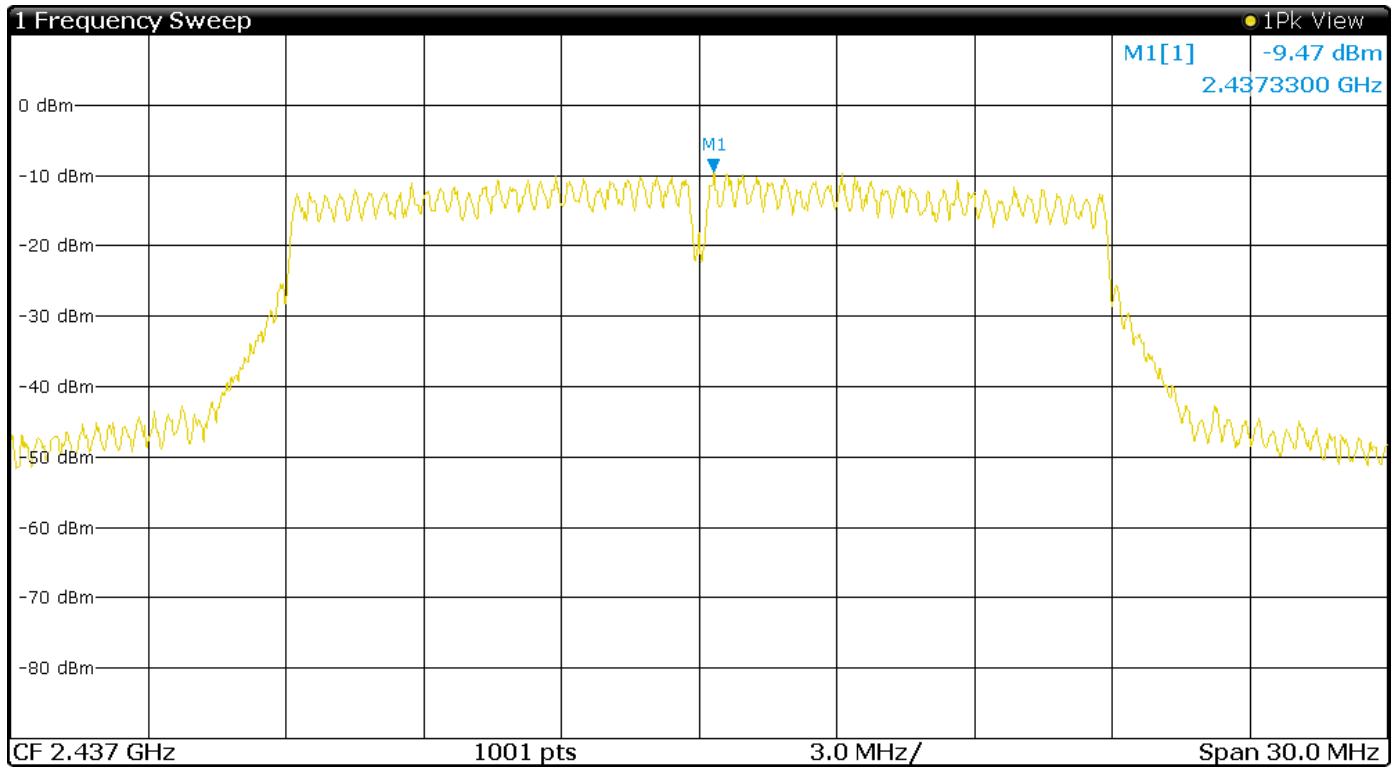
Figure 40 Plot of Transmitter Power Spectral Density Mode 7 802.11n
