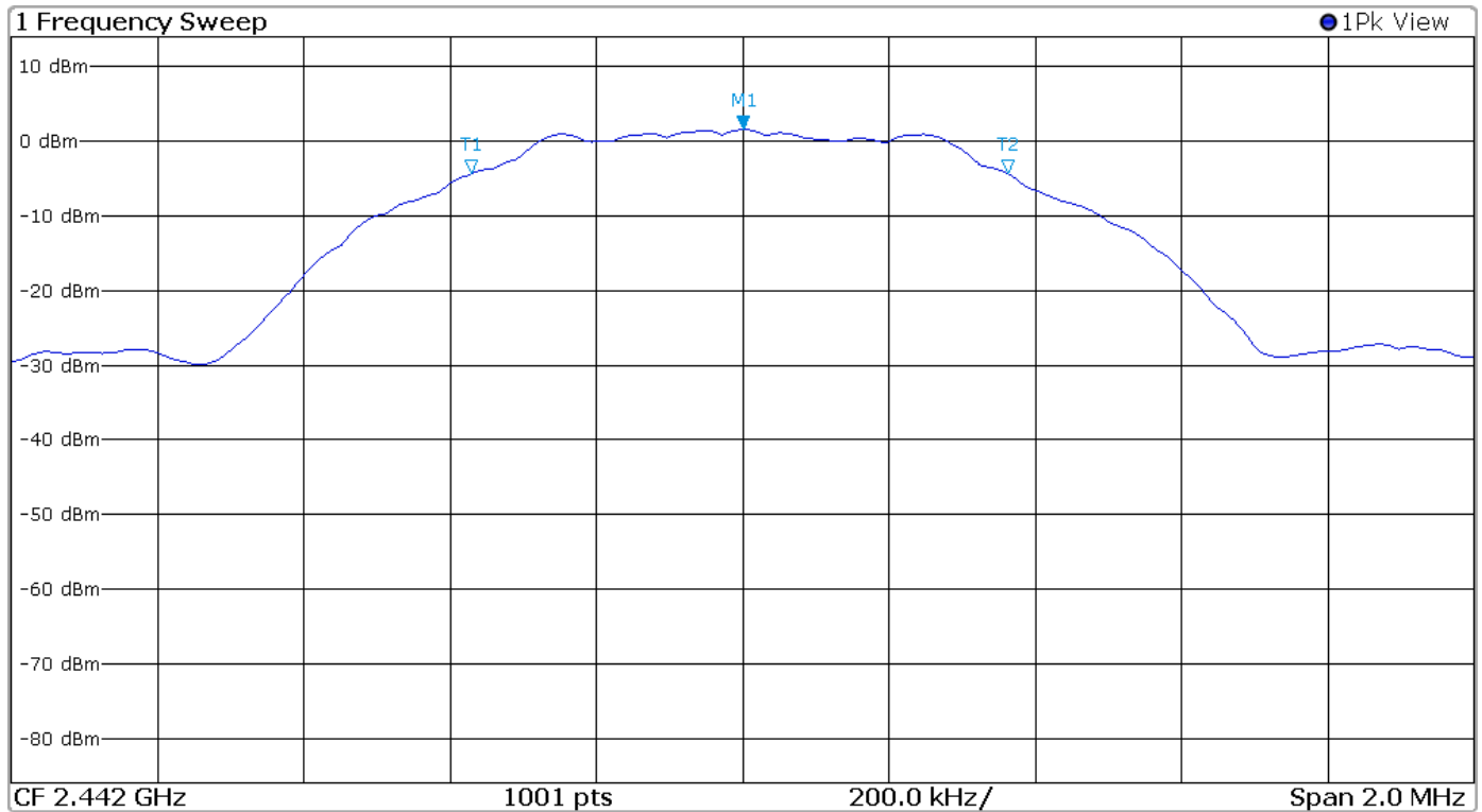
Figure 27 Plot of 6-dB Occupied Bandwidth Mode 4 BT BLE
