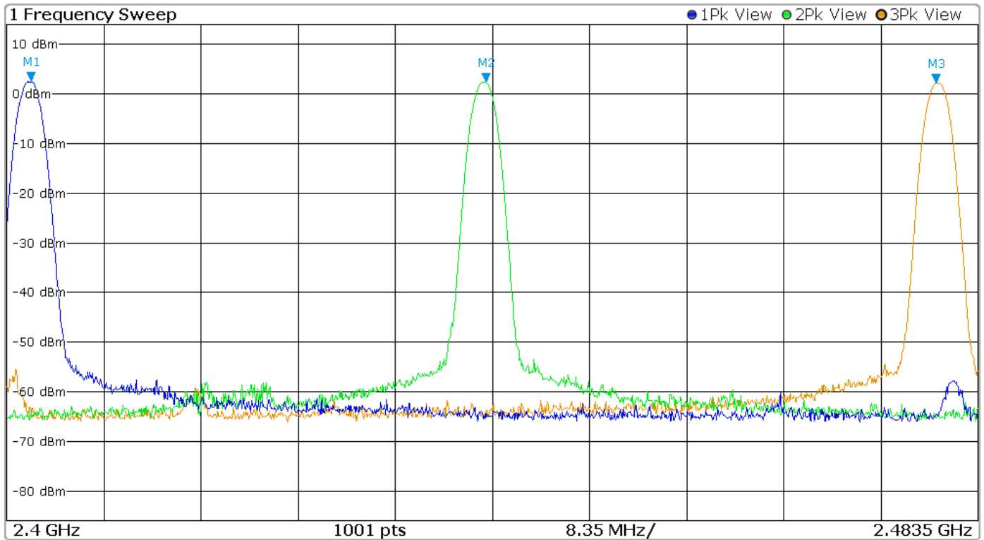
Figure 6 Plot of Transmitter Emissions Operation in 2402-2480 MHz Mode 3 BT 3EDR
