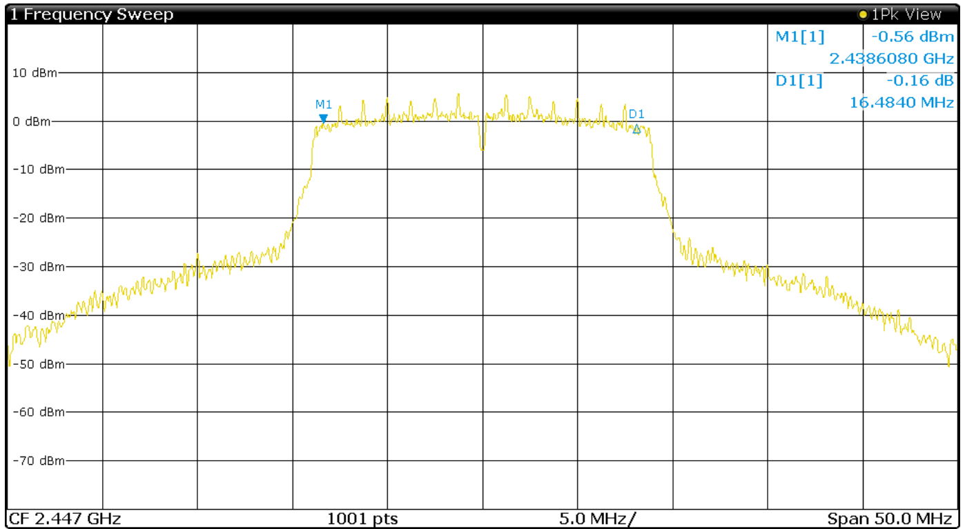
Figure 33 Plot of 6-dB Occupied Bandwidth Mode 8 802.11n
