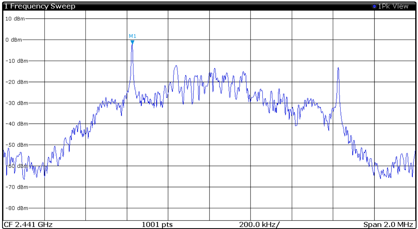
Figure 35 Plot of Transmitter Power Spectral Density Mode 2 BT 2EDR
