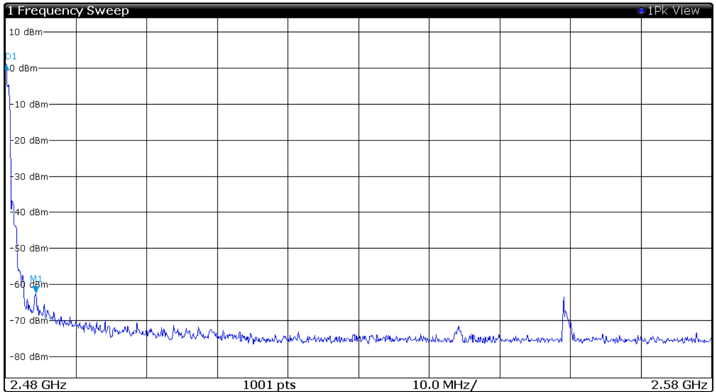
Figure 17 Plot of Transmitter Emissions High Band Edge Mode 2 BT 2EDR
