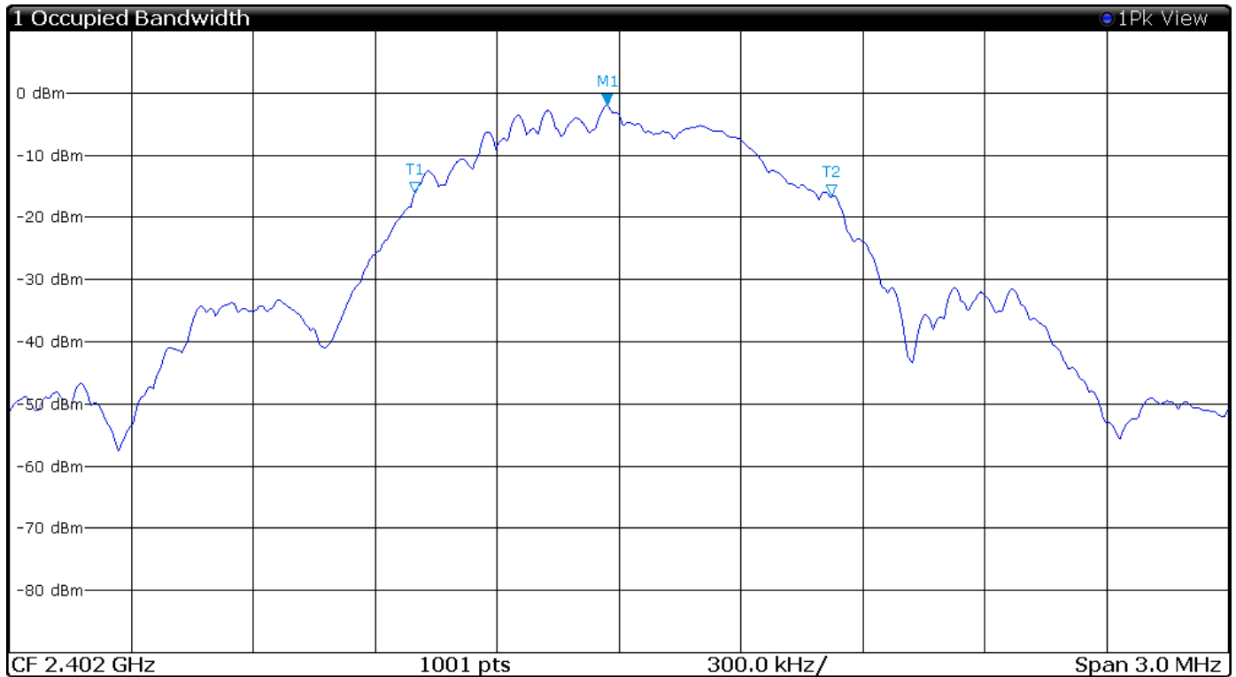
Figure 28 Plot of 99% Occupied Bandwidth Mode 4 BT BLE
