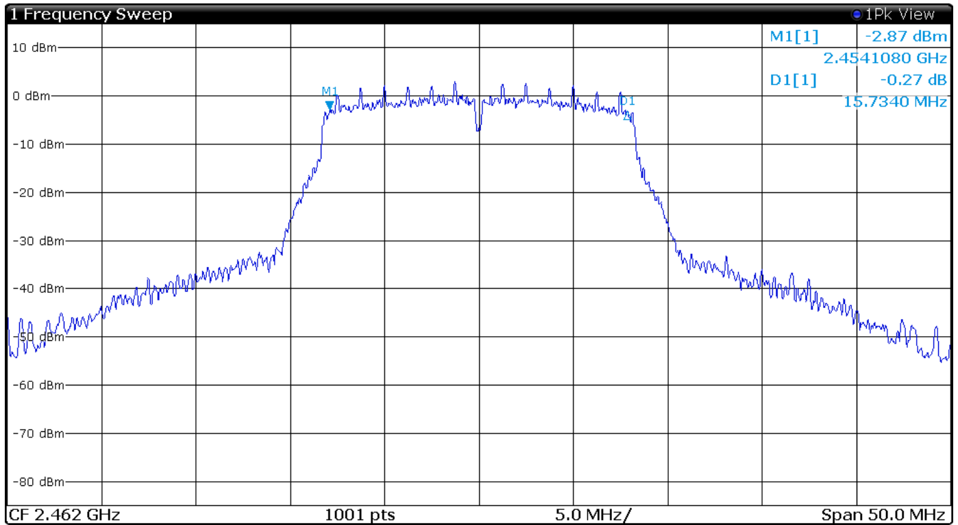
Figure 31 Plot of 6-dB Occupied Bandwidth Mode 6 802.11g
