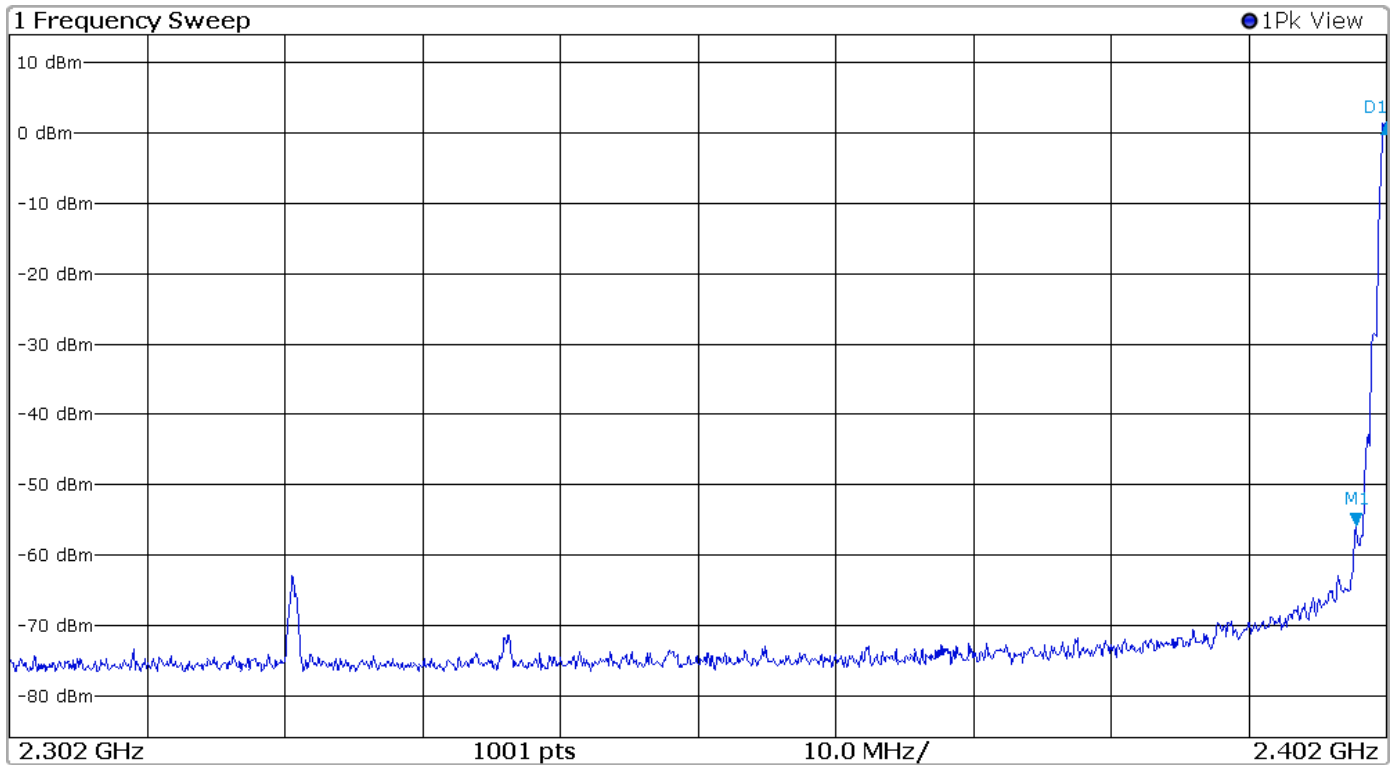
Figure 13 Plot of Transmitter Emissions Low Band Edge Mode 4 BT BLE
