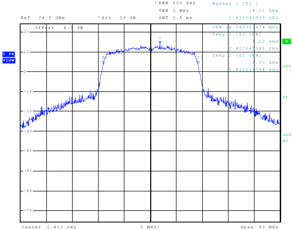
Figure 22 Plot of 99% Occupied Bandwidth Mode 9 802.11n
