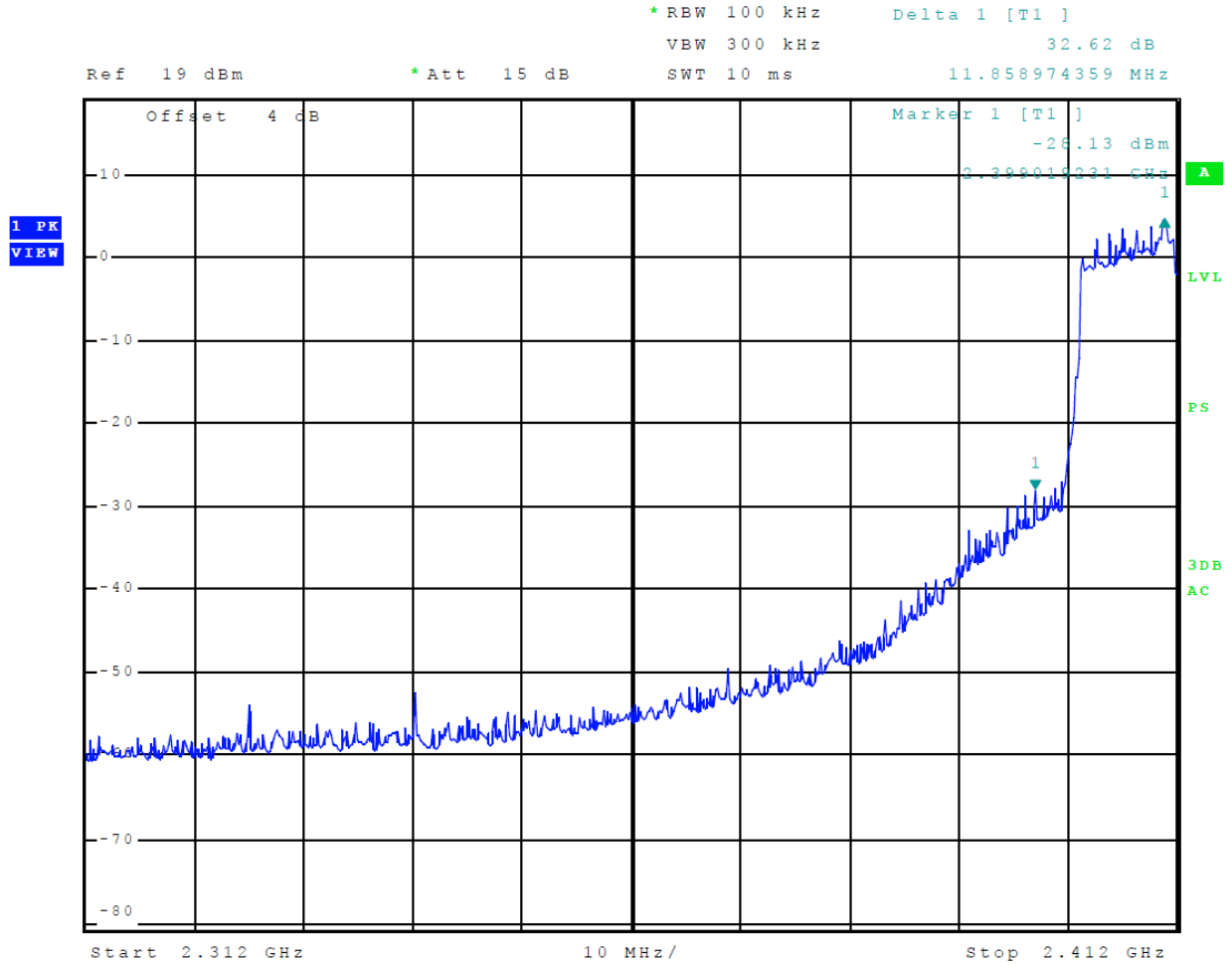
Figure 10 Plot of Transmitter Emissions Low Band Edge Mode 7 802.11n
