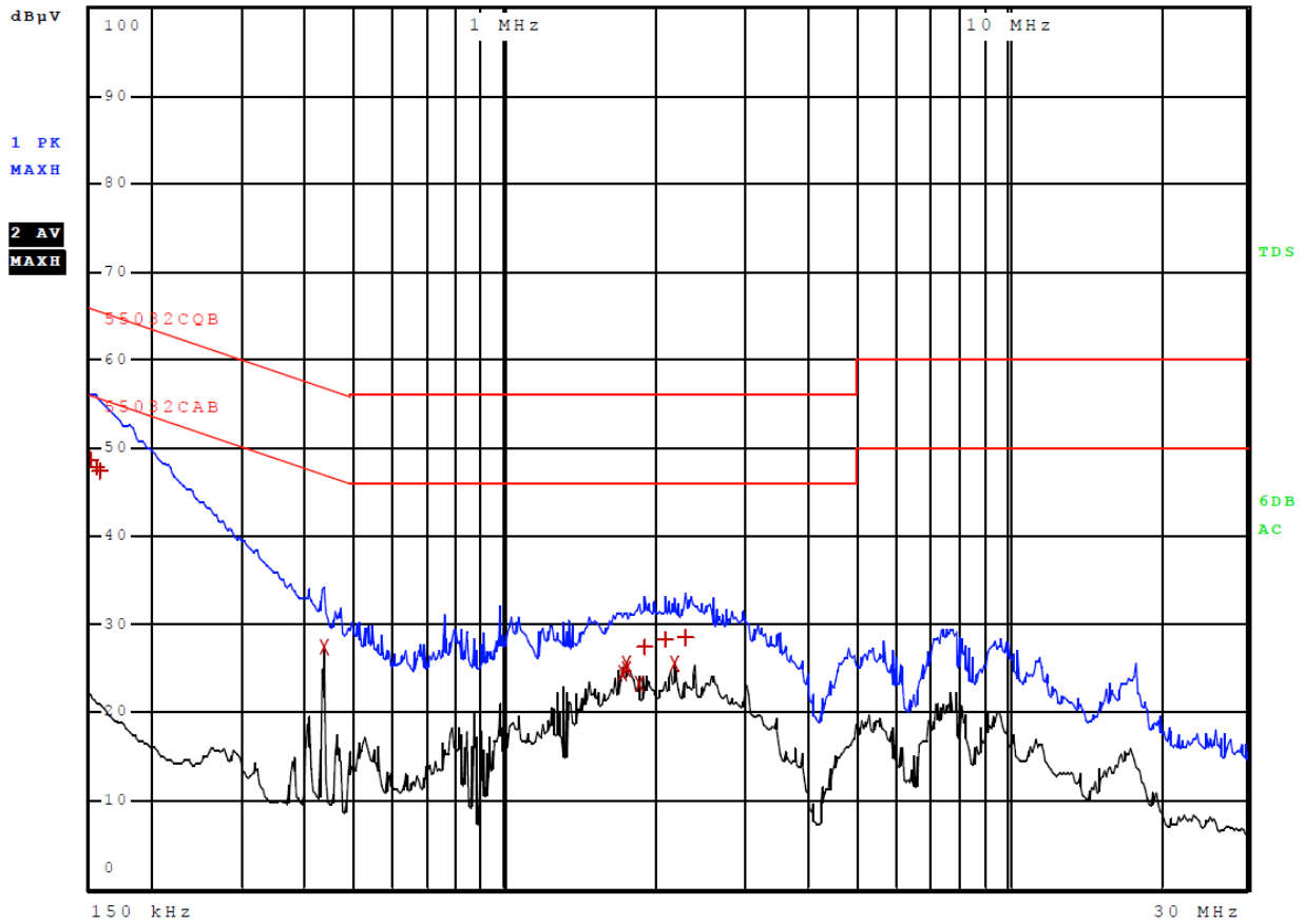
Figure 2 AC Line Conducted emissions of EUT line 2 (EUT – Computer)
