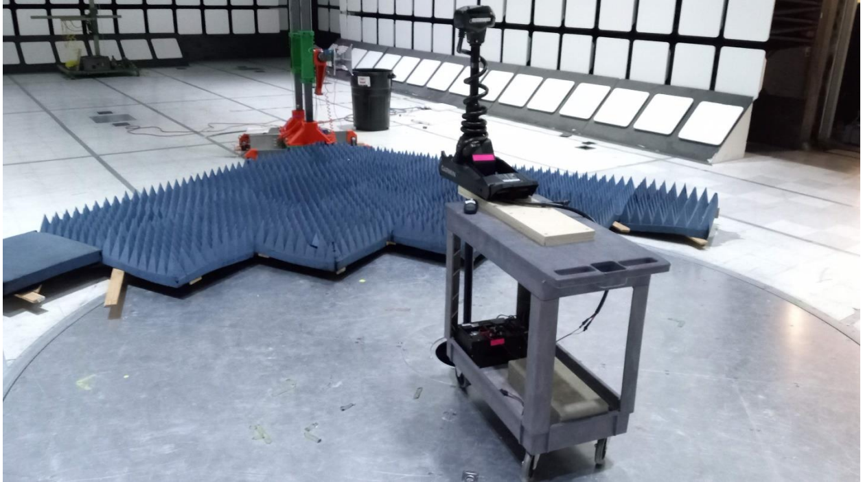
1 – 26GHz Test Setup (BT)
