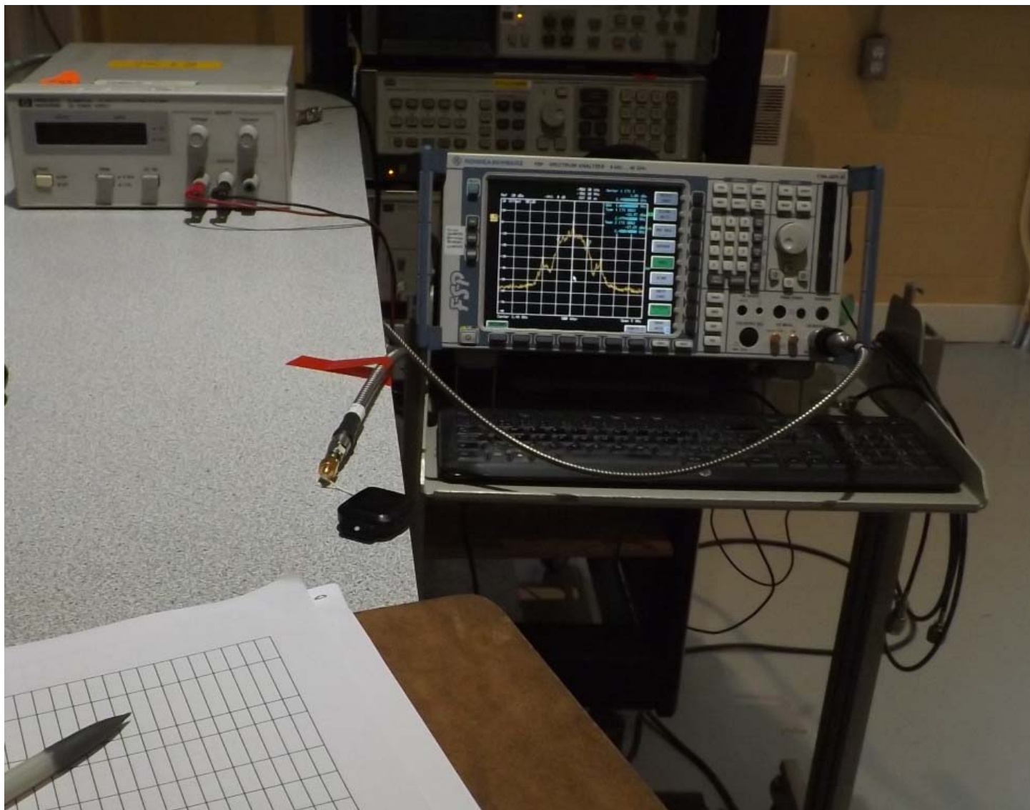
Figure E20.1 – Setup Photo – Conducted Measurements
