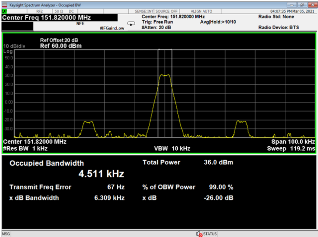
151.82 MHz, GFSK, no audio modulation
