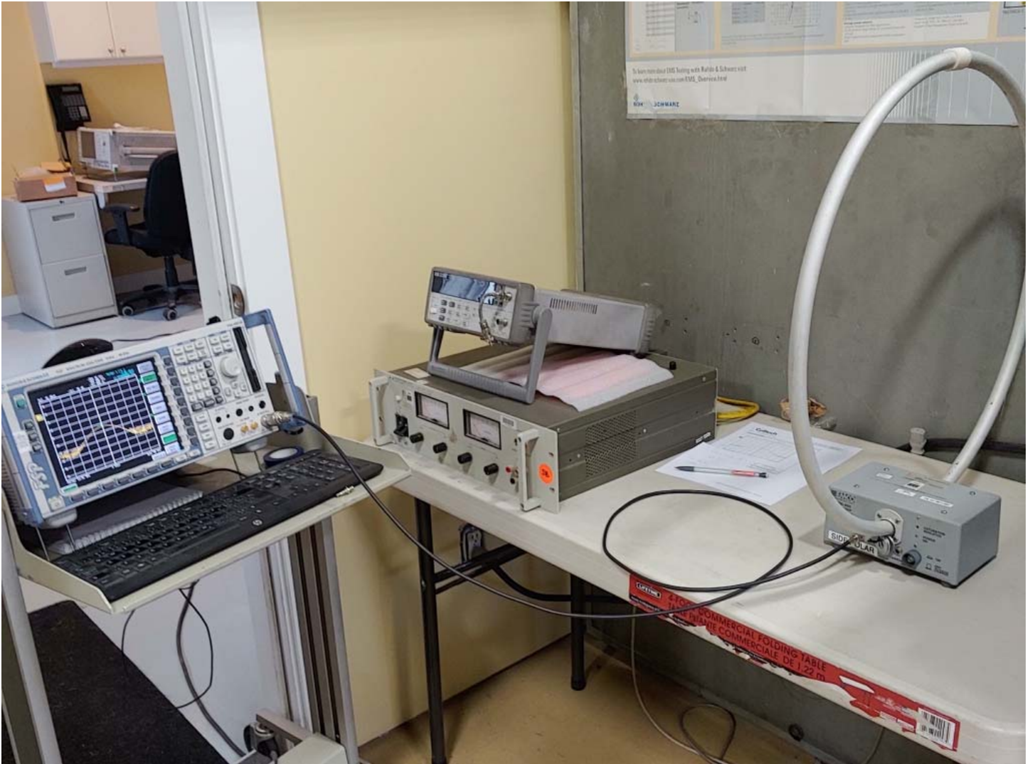
Figure E20.2 – Setup Photo – Frequency Stability Measurements
