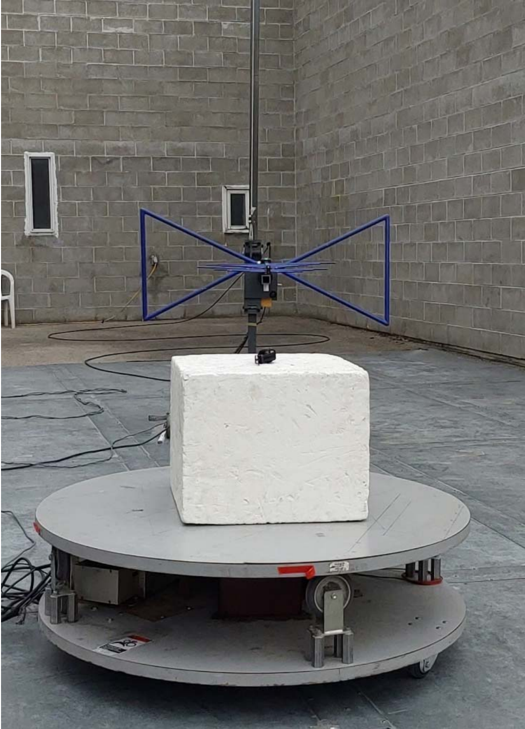
Figure E20.7 – Setup Photo – Radiated Emissions – 30-1000MHz Horizontal
