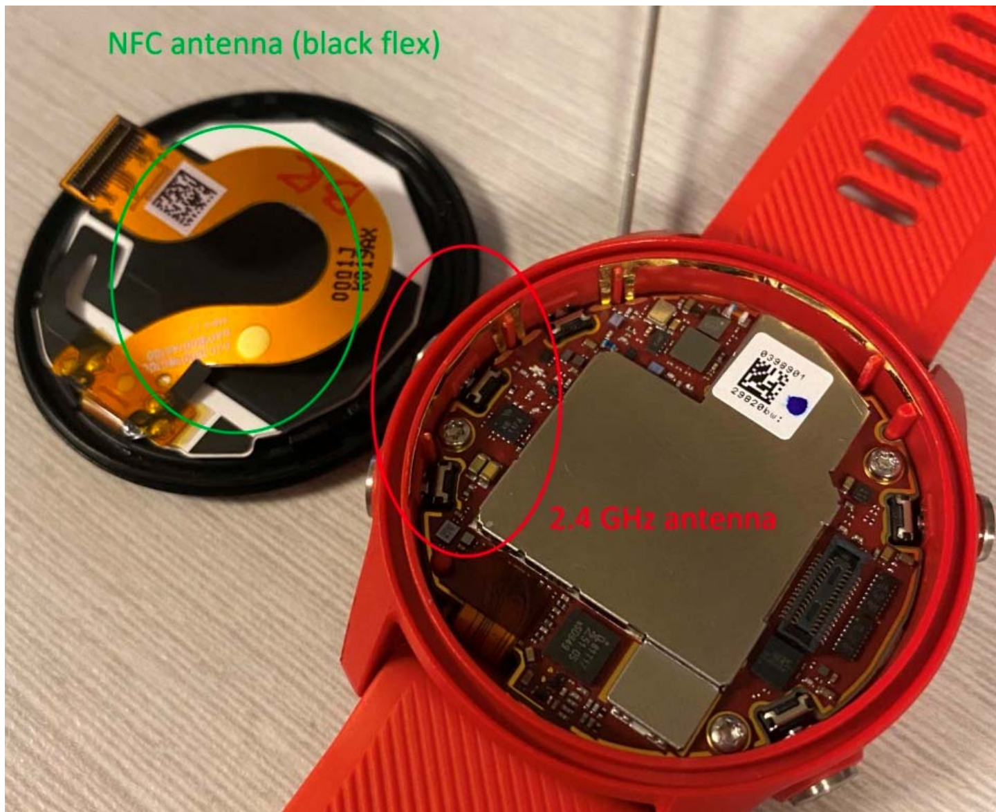
Figure E19.3 – Internal Photo – Antenna Locations
