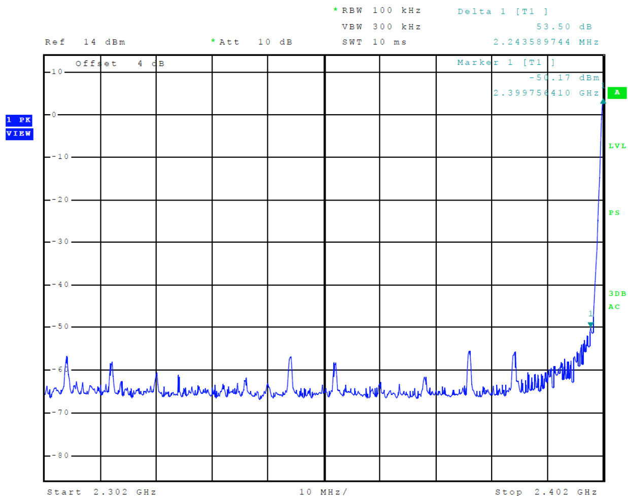
Figure 11 Plot of Transmitter Emissions Low Band Edge Mode 2 BLE (GMSK)
