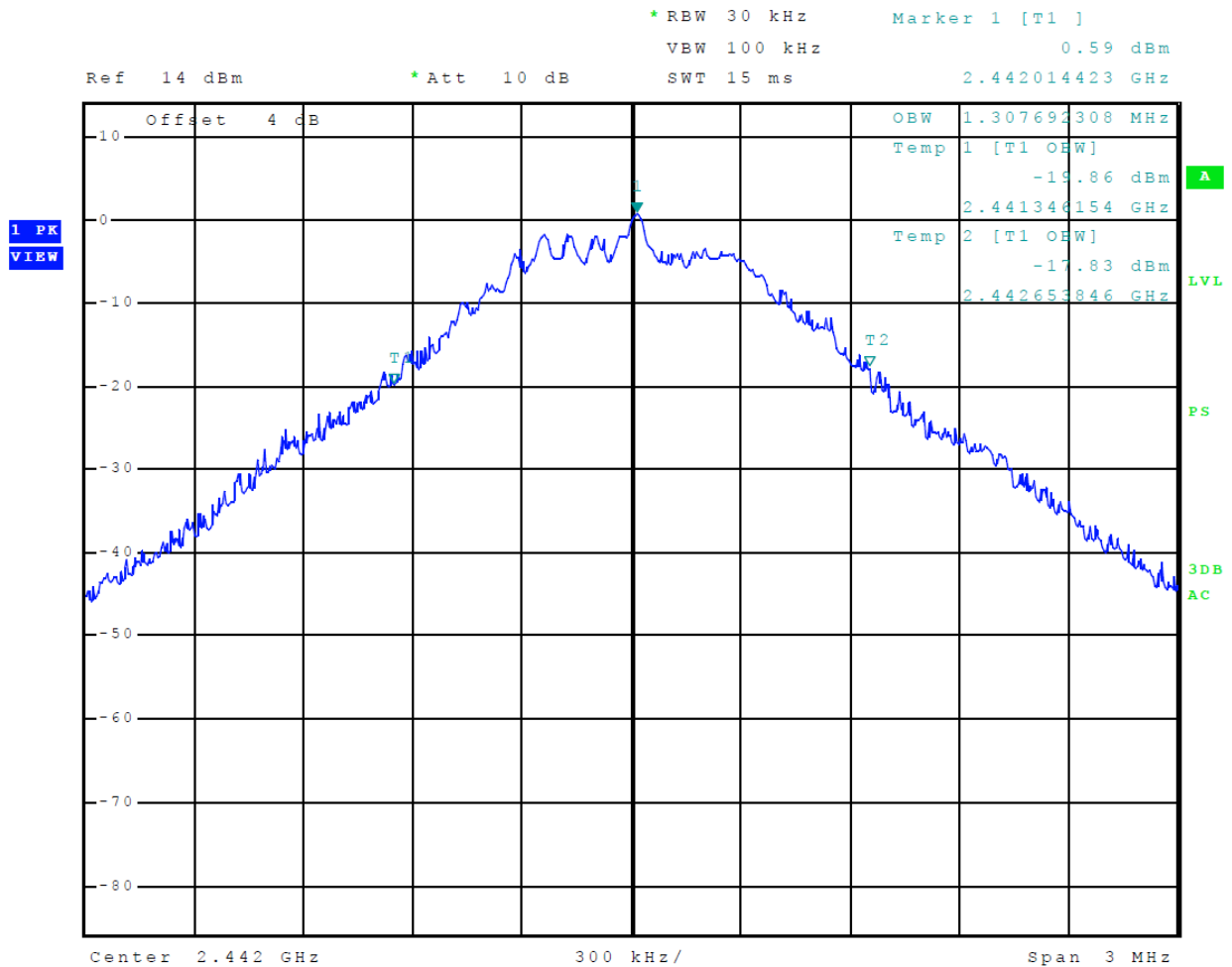
Figure 10 Plot of Transmitter Emissions 99% Occupied Bandwidth Mode 2 BLE (GMSK)
