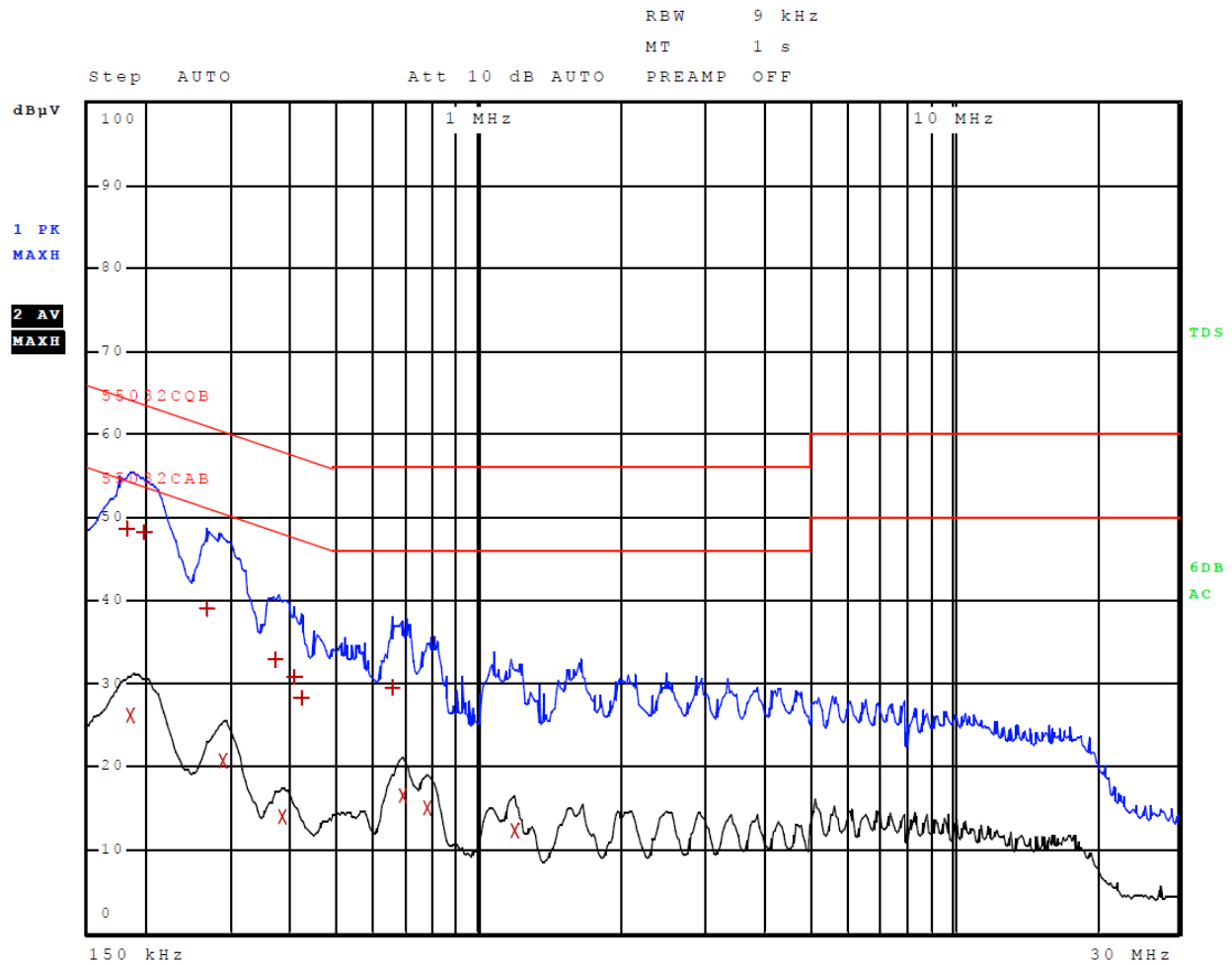
Figure 1 AC Line Conducted emissions of EUT line 1 Configuration #2
