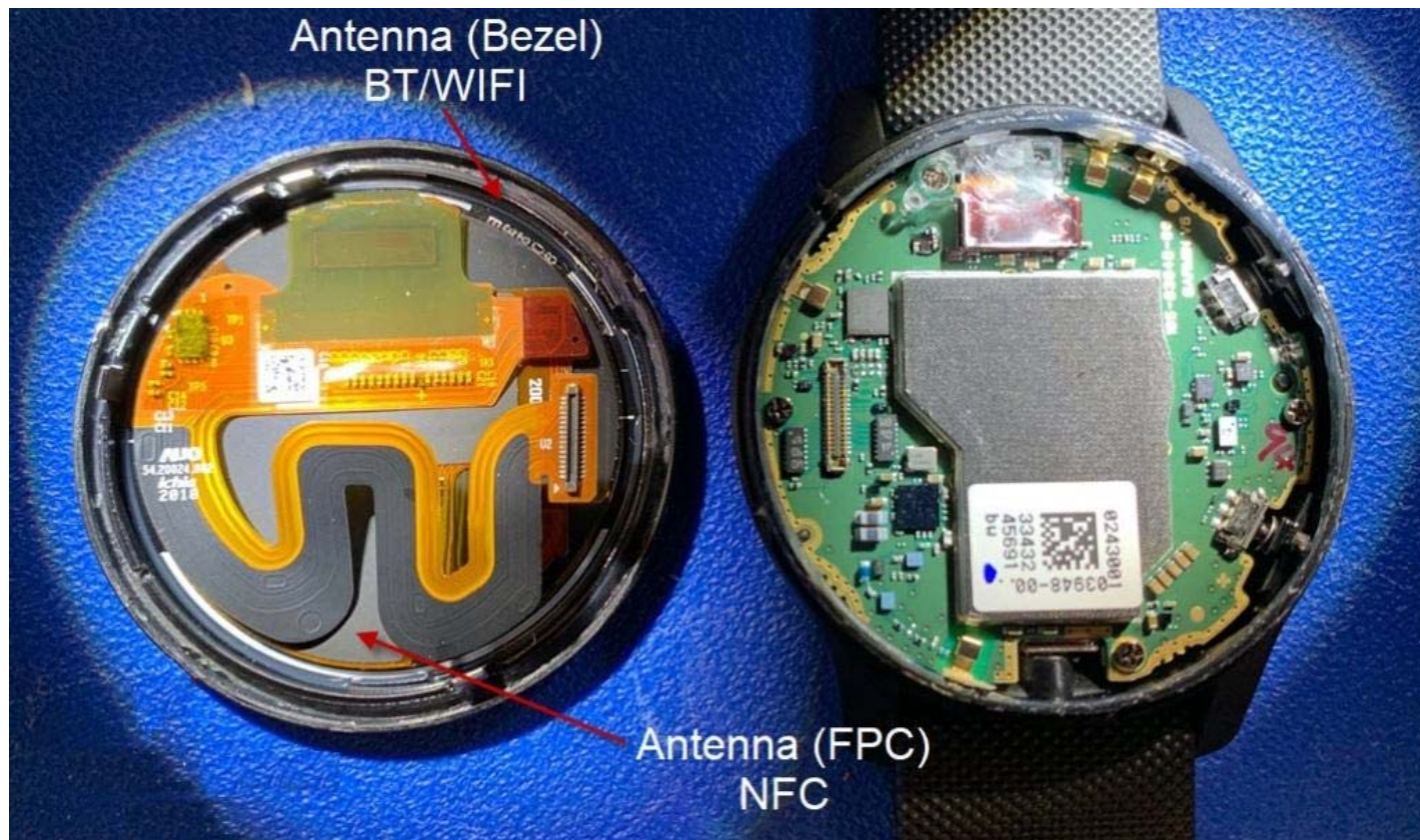
Figure E19.3 – Internal Photo – Antennas
