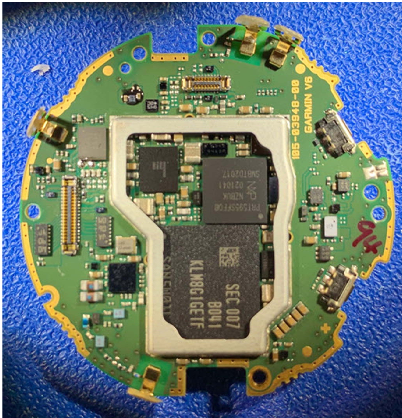
Figure E19.2 – Internal Photo – PCB Top
