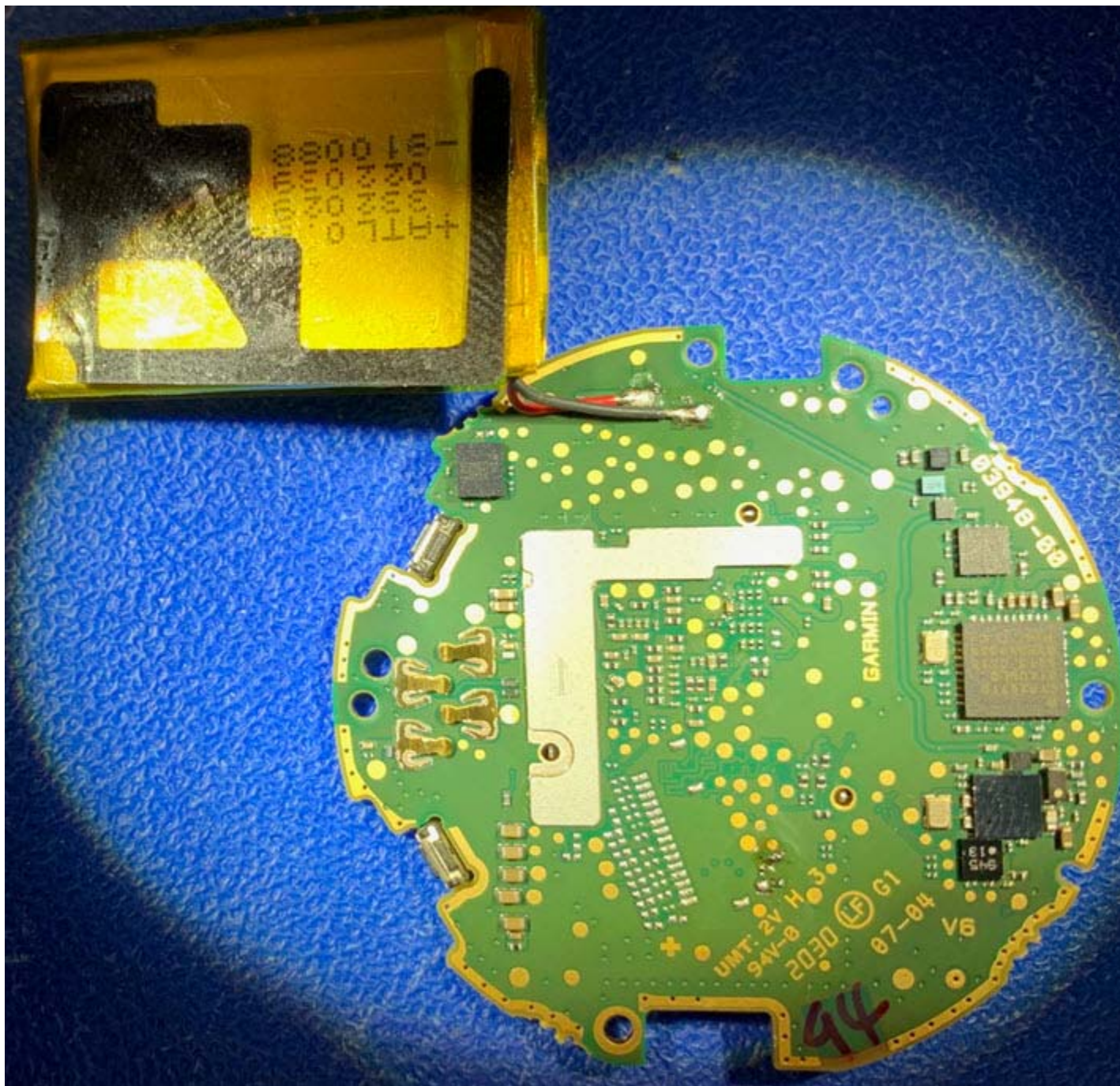
Figure E19.1 – Internal Photo – PCB Bottom
