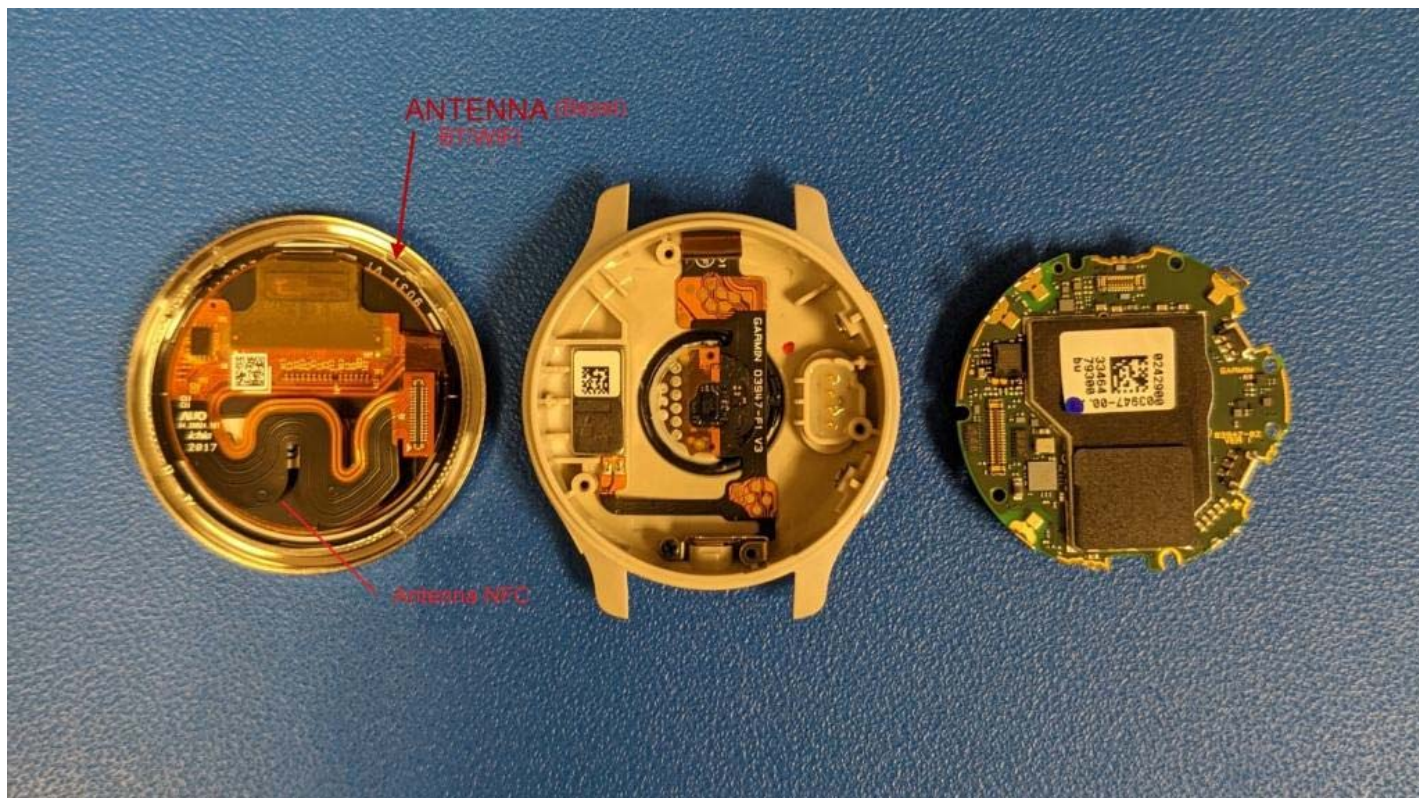
Figure E19.4 – Internal Photo – Antennas
