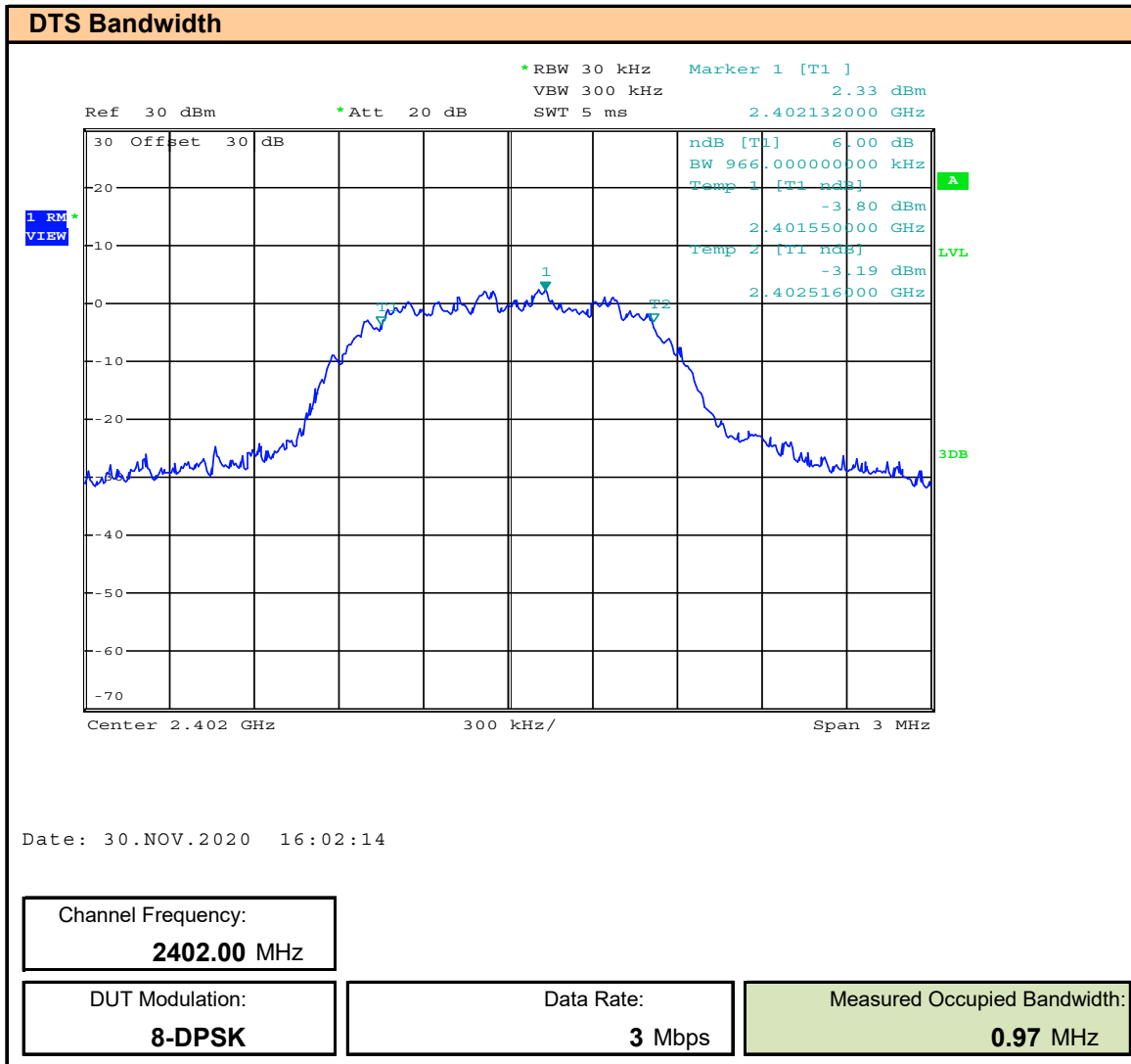
Plot 8.8 – 6dB DTS Bandwidth BT EDR 3MB, 2402MHz
