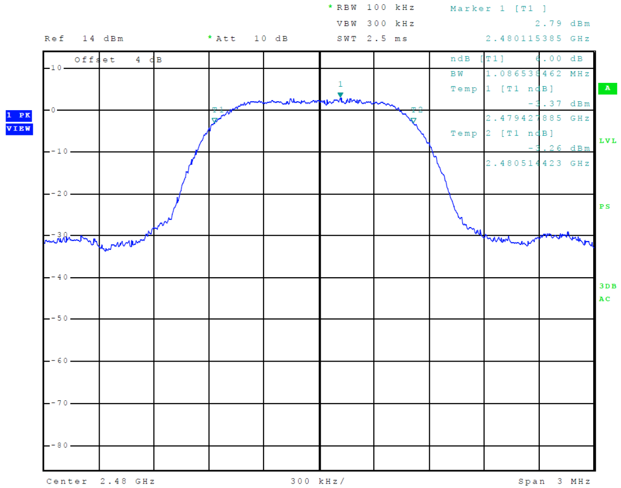
Figure 16 Plot of 6-dB Occupied Bandwidth Mode 3 ( \pi/4 DQPSK)
