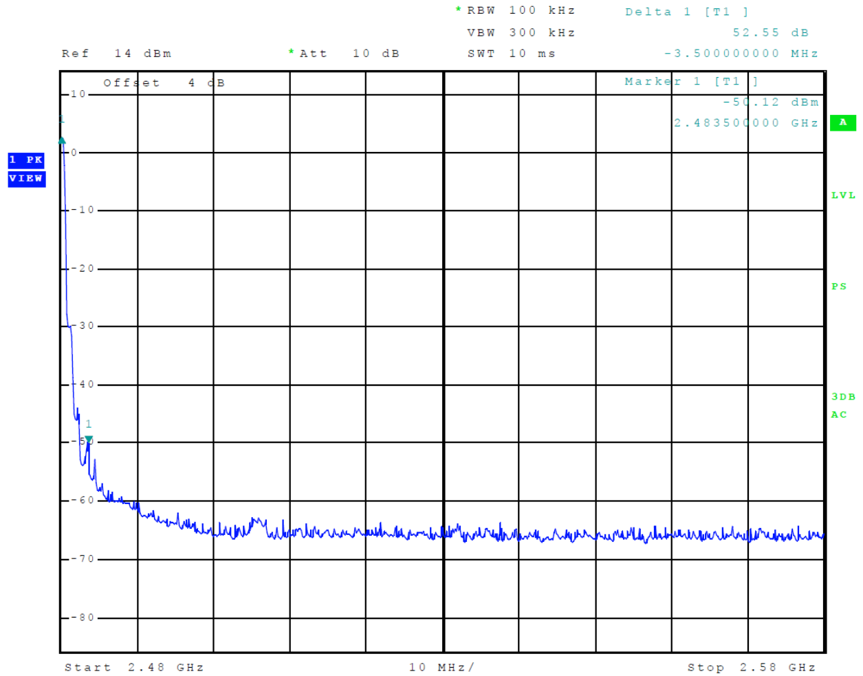
Figure 11 Plot of Transmitter Emissions High Band Edge Mode 3 ( \pi/4 DQPSK)
