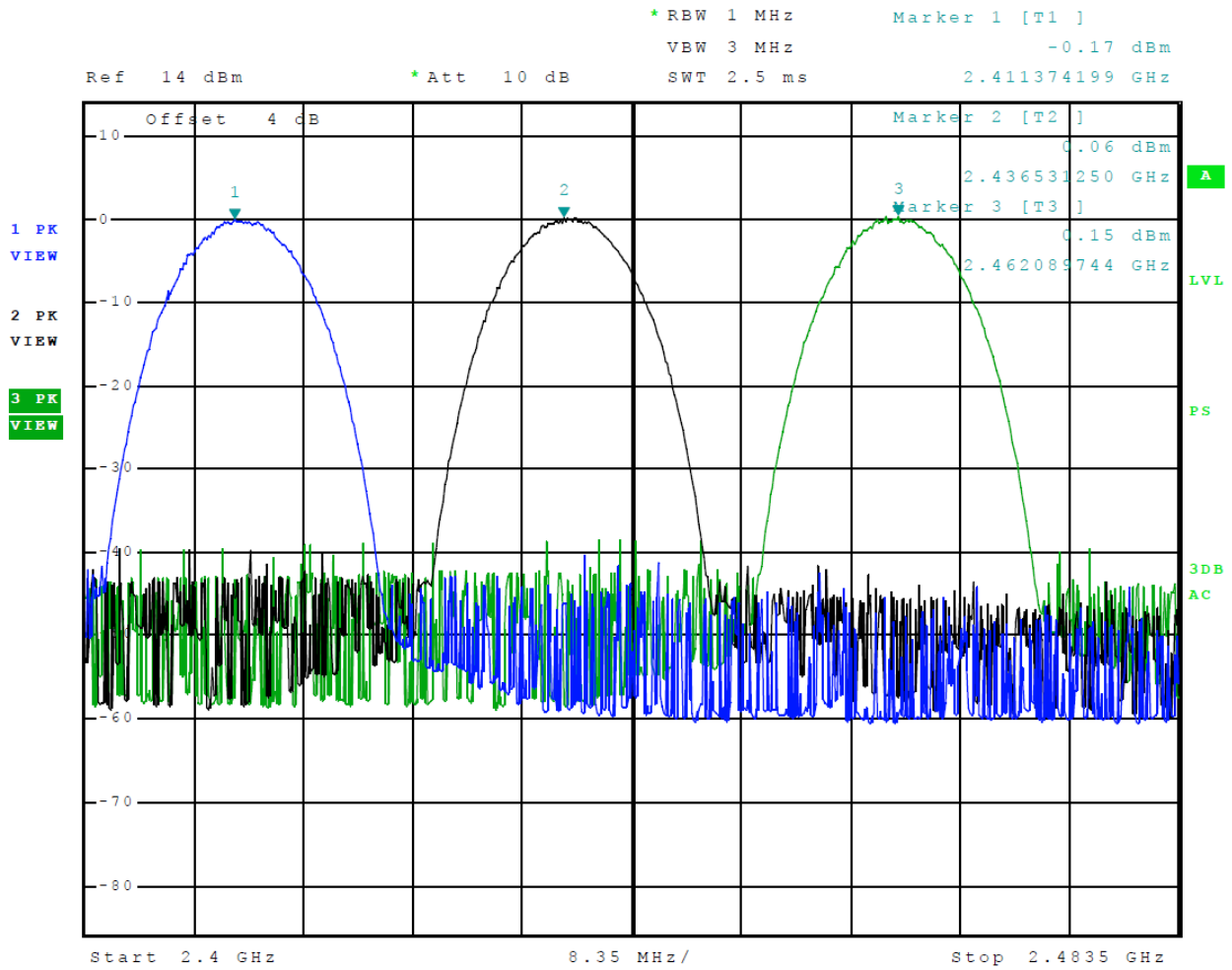
Figure 3 Plot of Transmitter Operation in 2412-2462 MHz Mode 5 (DSSS)
