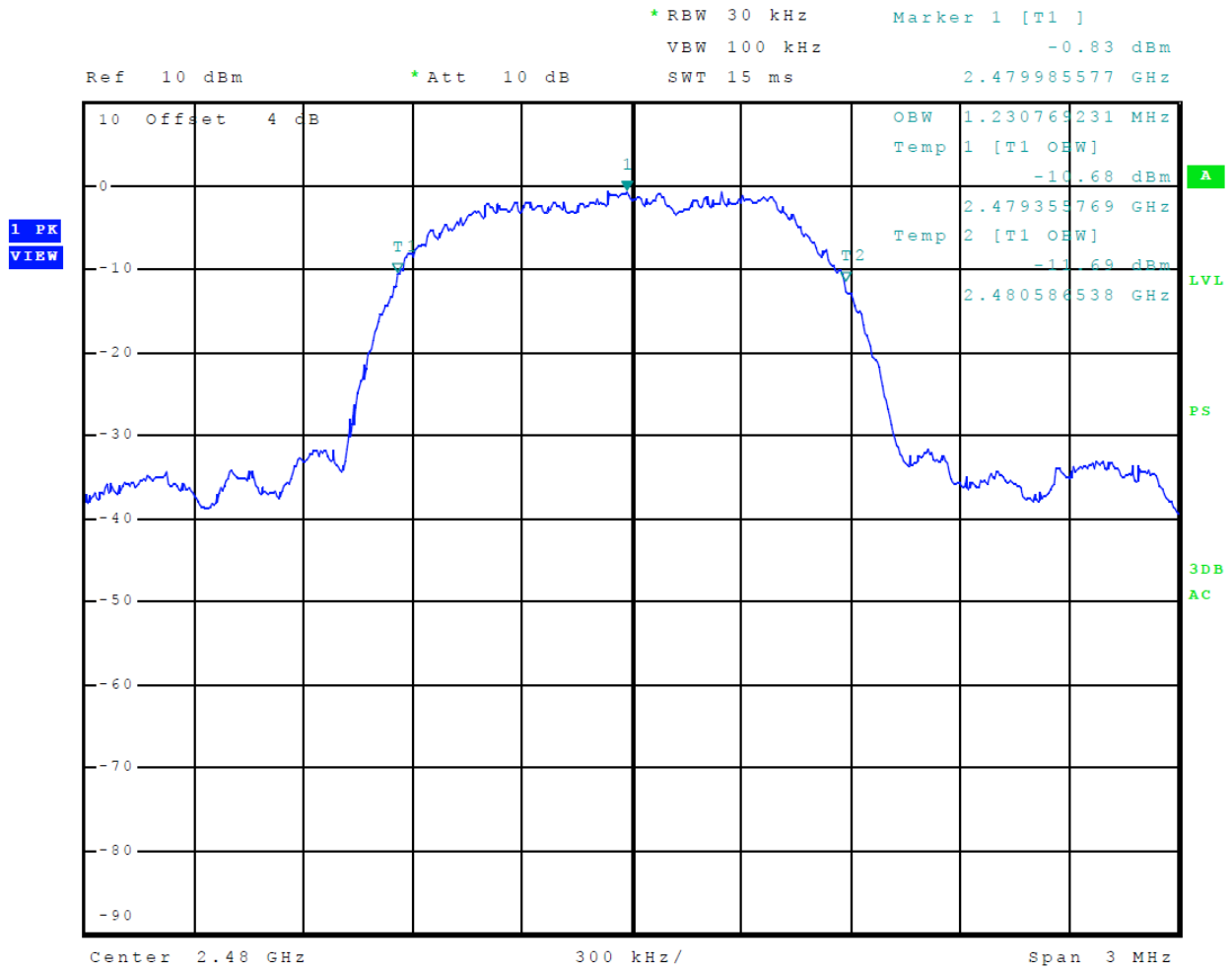
Figure 19 Plot of Transmitter Emissions 99% Occupied Bandwidth Mode 4 (8DPSK)
