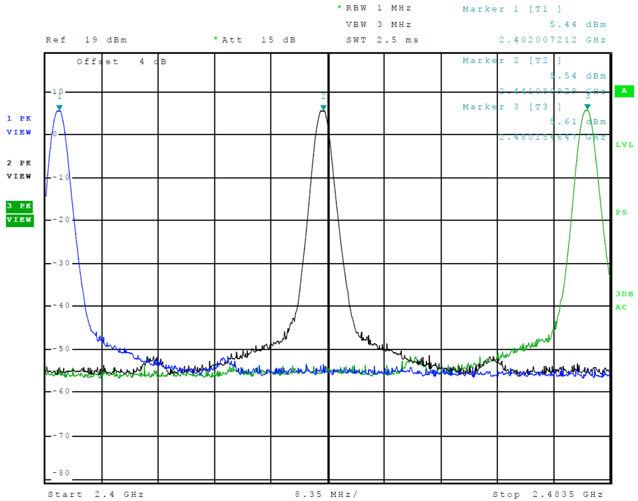
Figure 1 Plot of Transmitter Emissions Operation in 2402-2480 MHz Mode 3 ( \pi/4 DQPSK)
