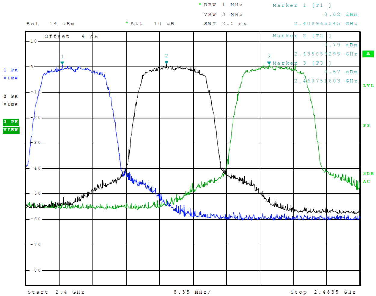
Figure 4 Plot of Transmitter Operation in 2412-2462 MHz Mode 6 (OFDM)
