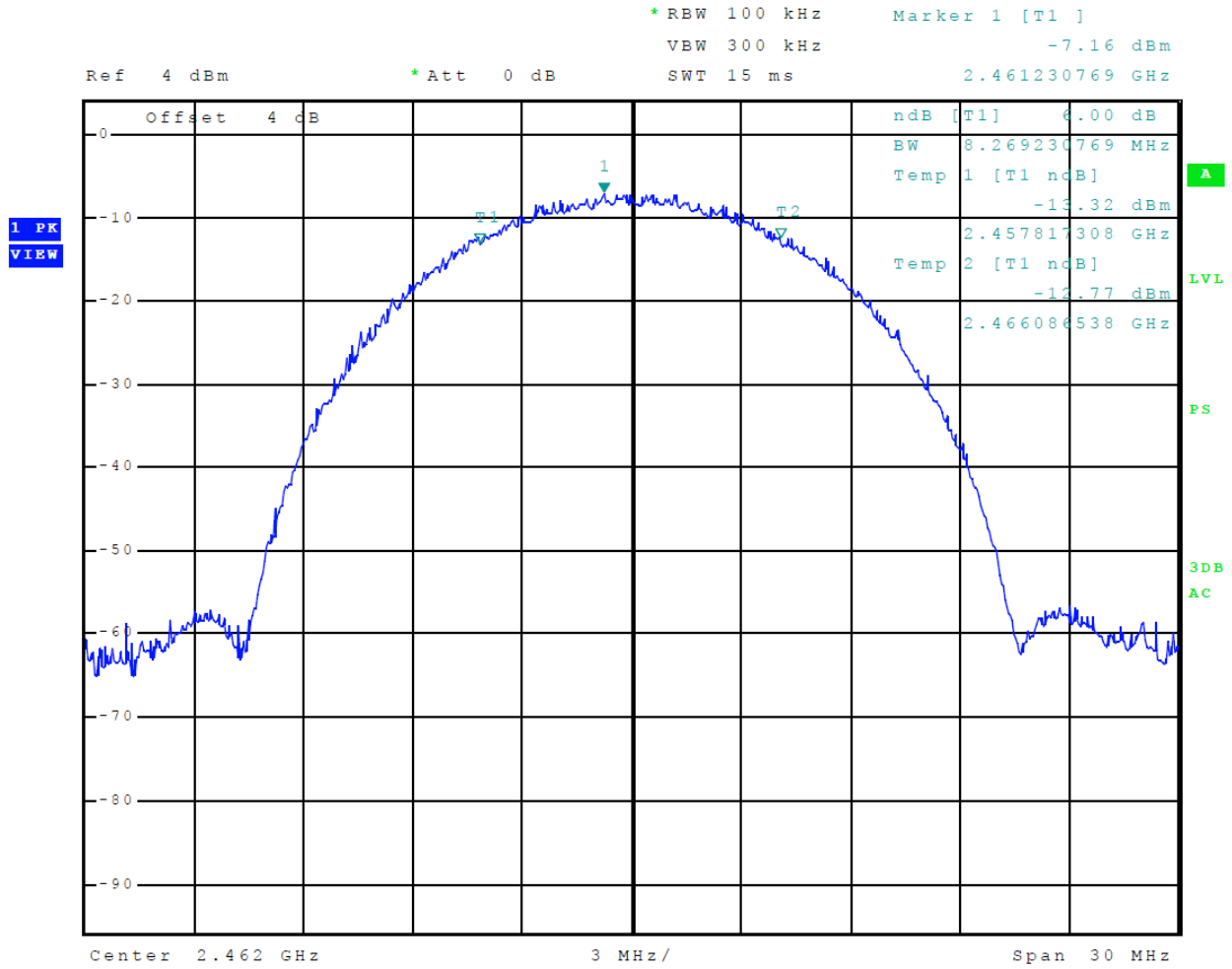
Figure 20 Plot of 6-dB Occupied Bandwidth Mode 5 (DSSS)
