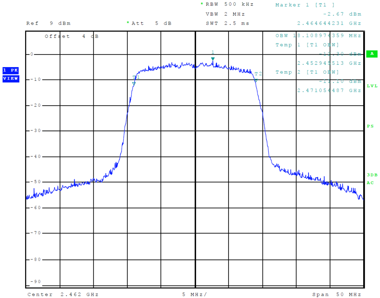
Figure 25 Plot of 99% Occupied Bandwidth Mode 7 (MCS)
