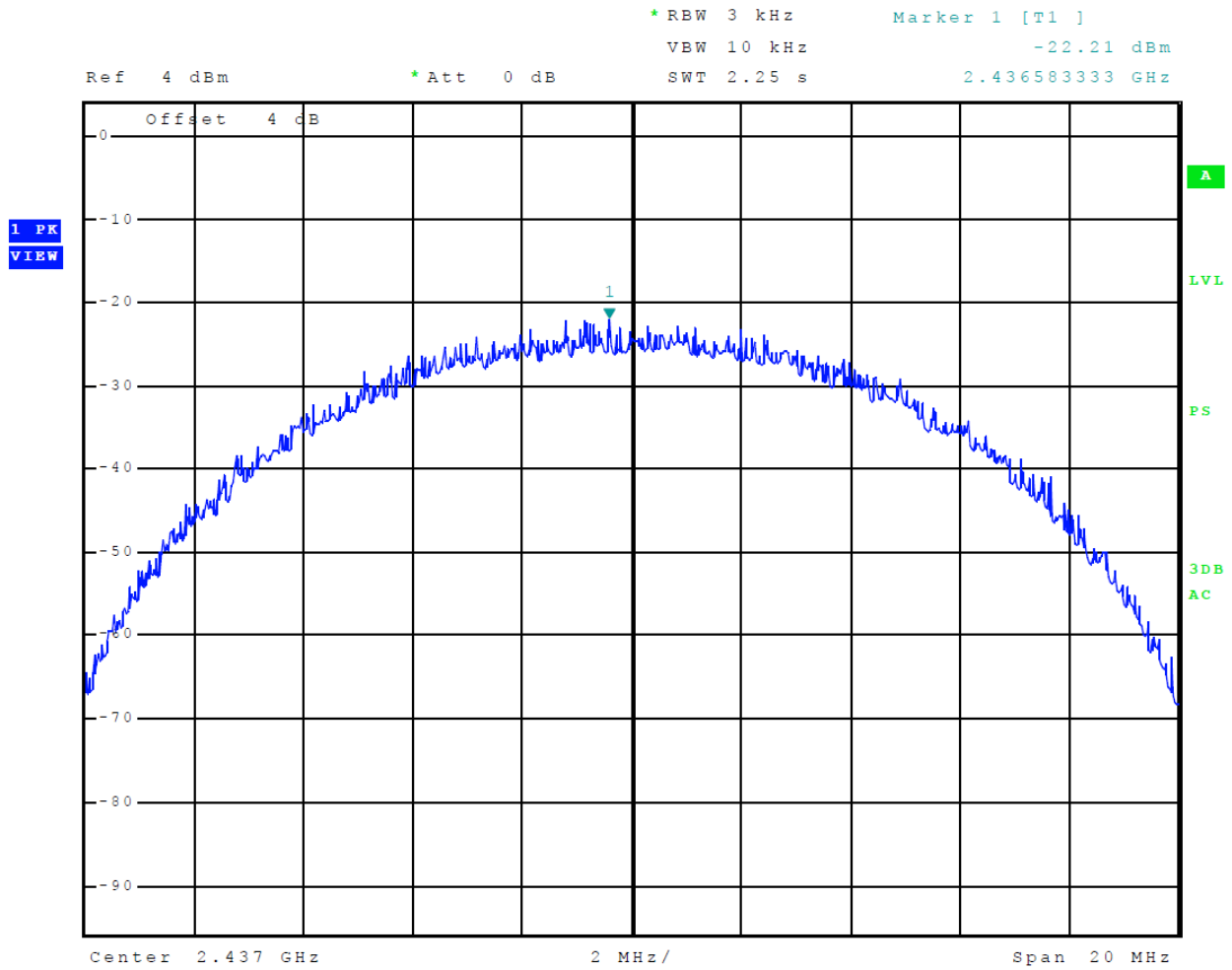
Figure 28 Plot of Transmitter Power Spectral Density Mode 5 (DSSS)
