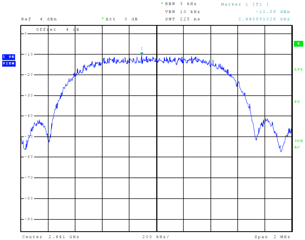
Figure 27 Plot of Transmitter Power Spectral Density Mode 4 (8DPSK)
