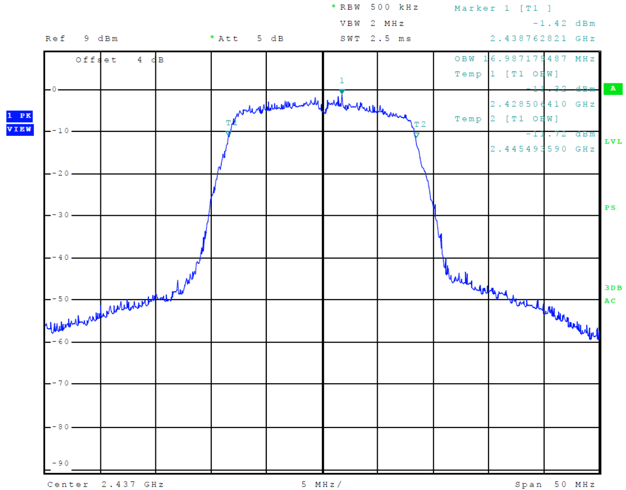
Figure 23 Plot of 99% Occupied Bandwidth Mode 6 (OFDM)
