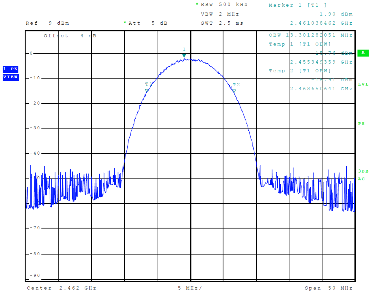
Figure 21 Plot of 99% Occupied Bandwidth Mode 5 (DSSS)
