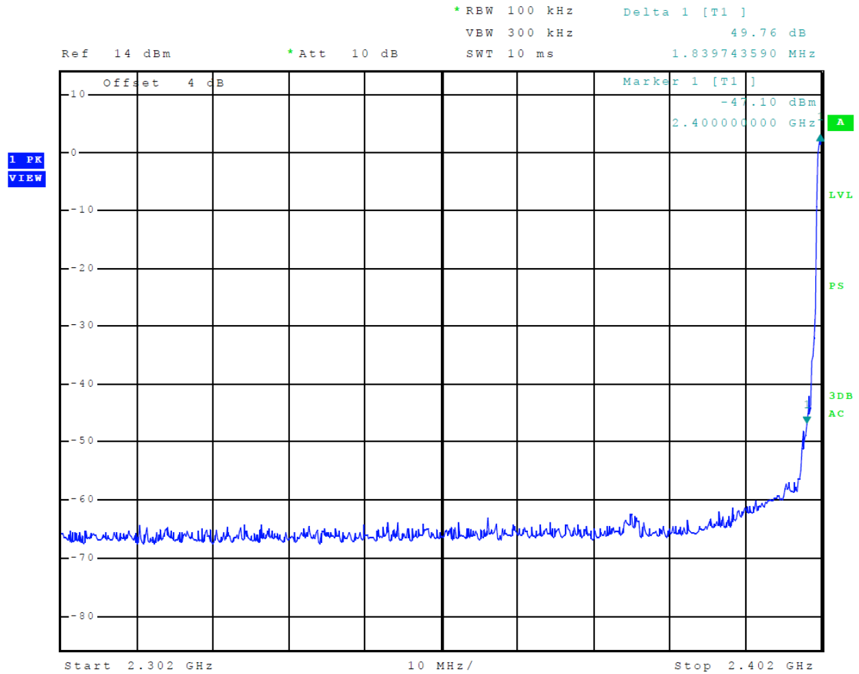
Figure 6 Plot of Transmitter Emissions Low Band Edge Mode 3 ( \pi/4 DQPSK)
