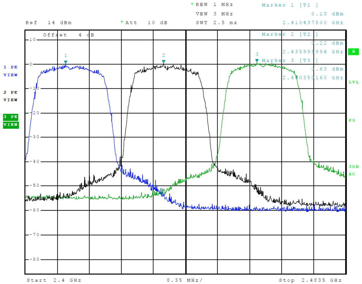
Figure 5 Plot of Transmitter Operation in 2412-2462 MHz Mode 7 (MCS)
