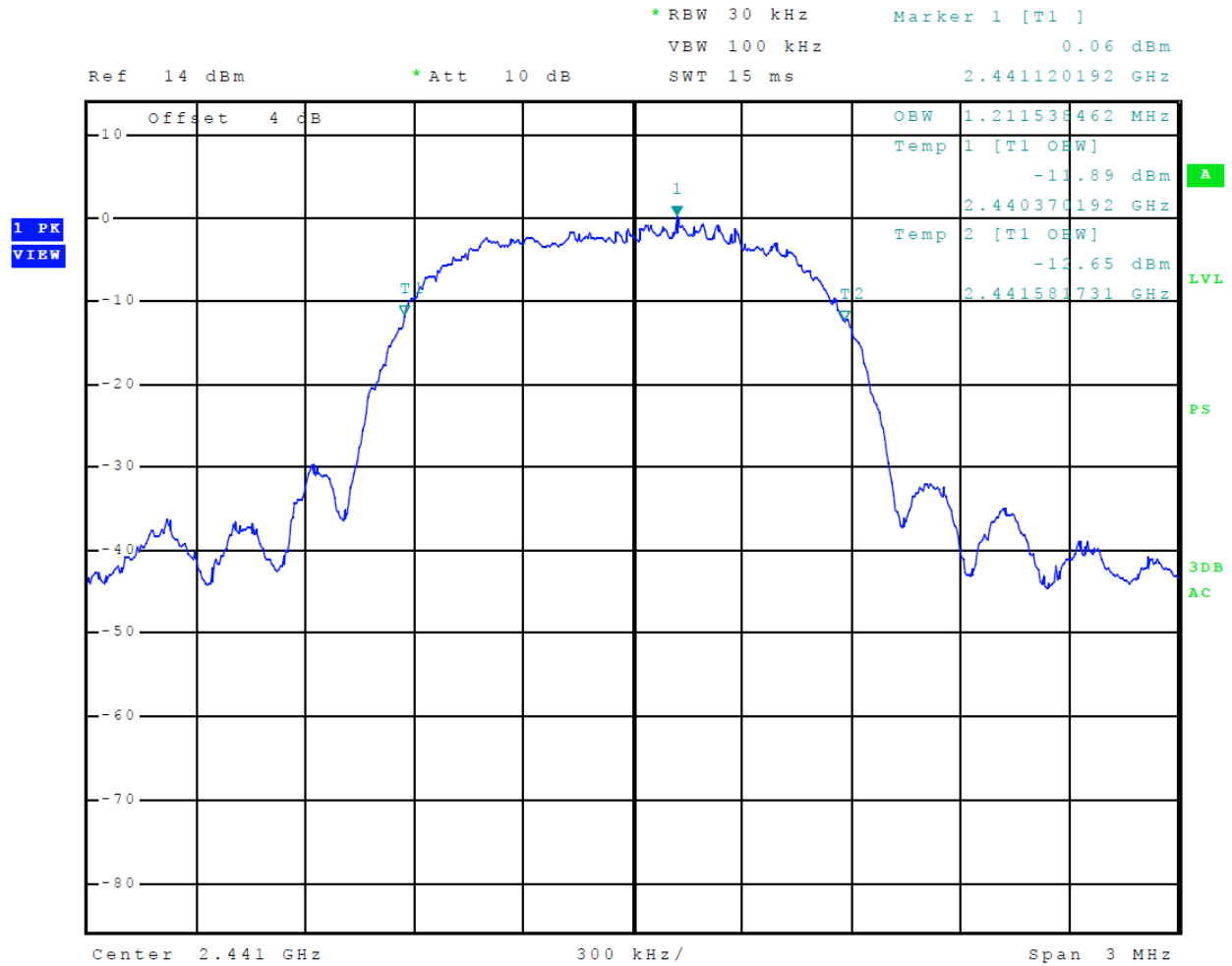
Figure 17 Plot of Transmitter Emissions 99% Occupied Bandwidth Mode 3 ( \pi/4 DQPSK)
