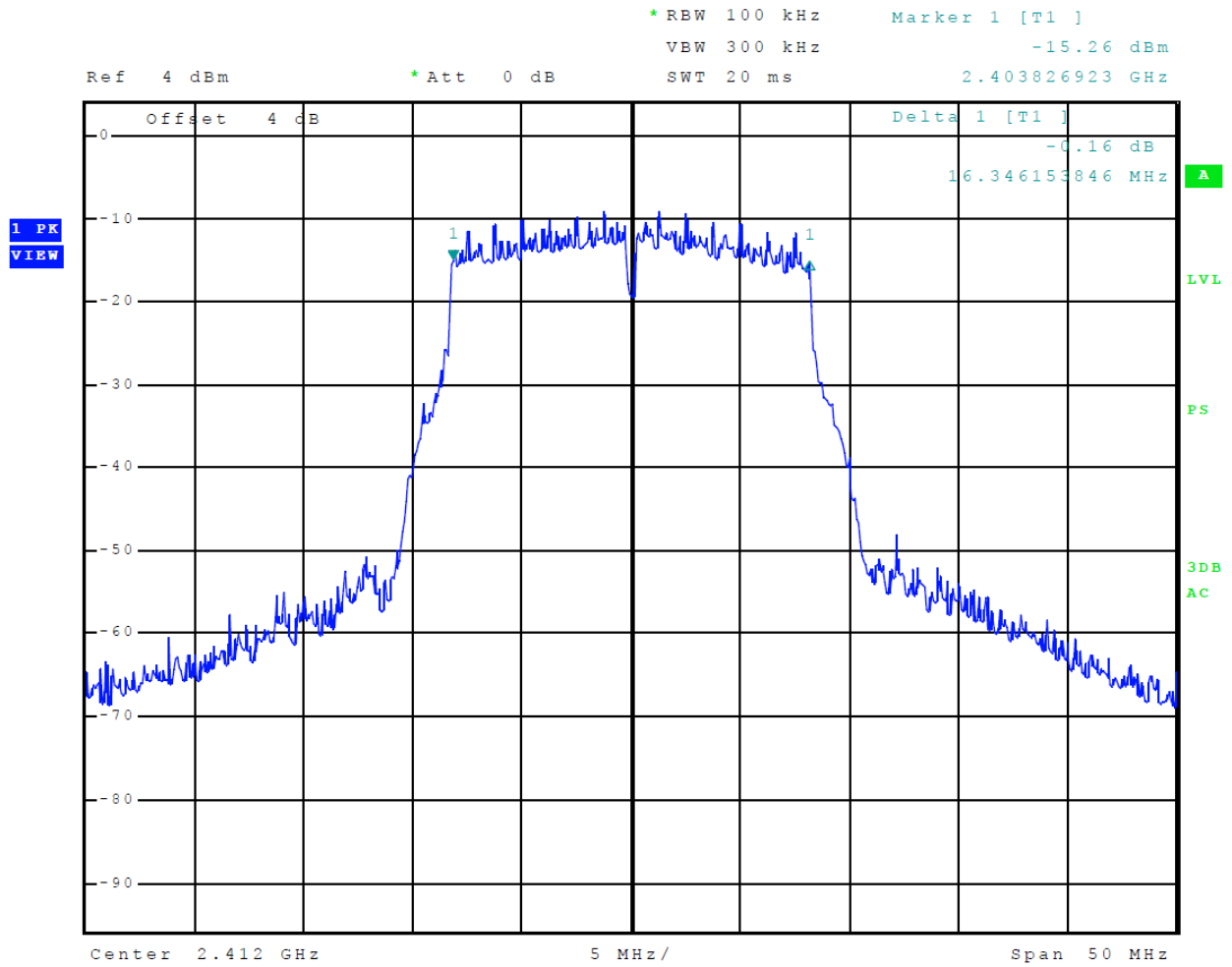
Figure 22 Plot of 6-dB Occupied Bandwidth Mode 6 (OFDM)
