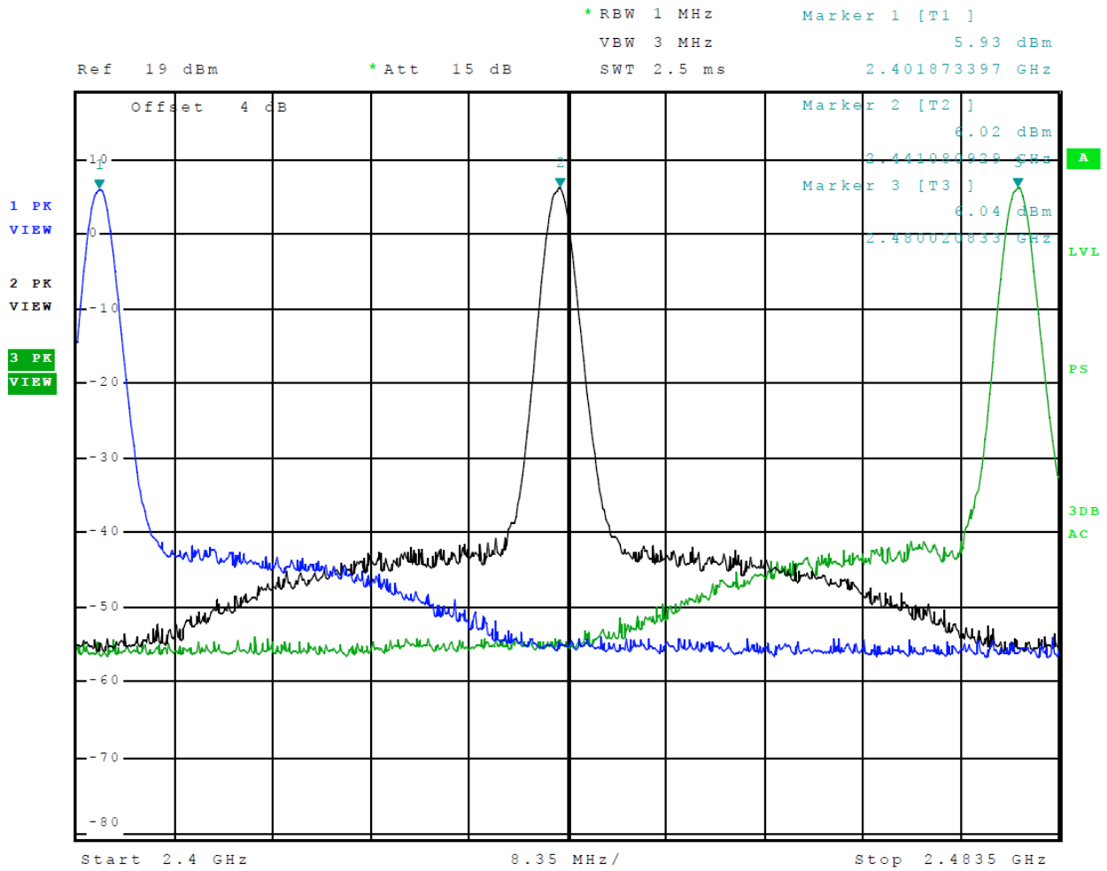
Figure 2 Plot of Transmitter Emissions Operation in 2402-2480 MHz Mode 4 (8DPSK)
