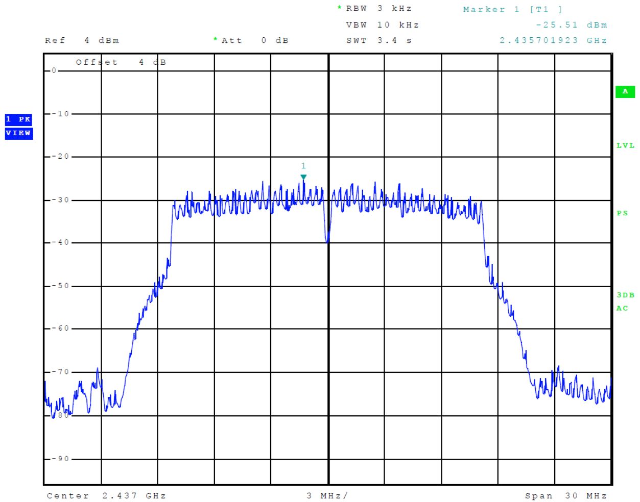
Figure 29 Plot of Transmitter Power Spectral Density Mode 6 (OFDM)
