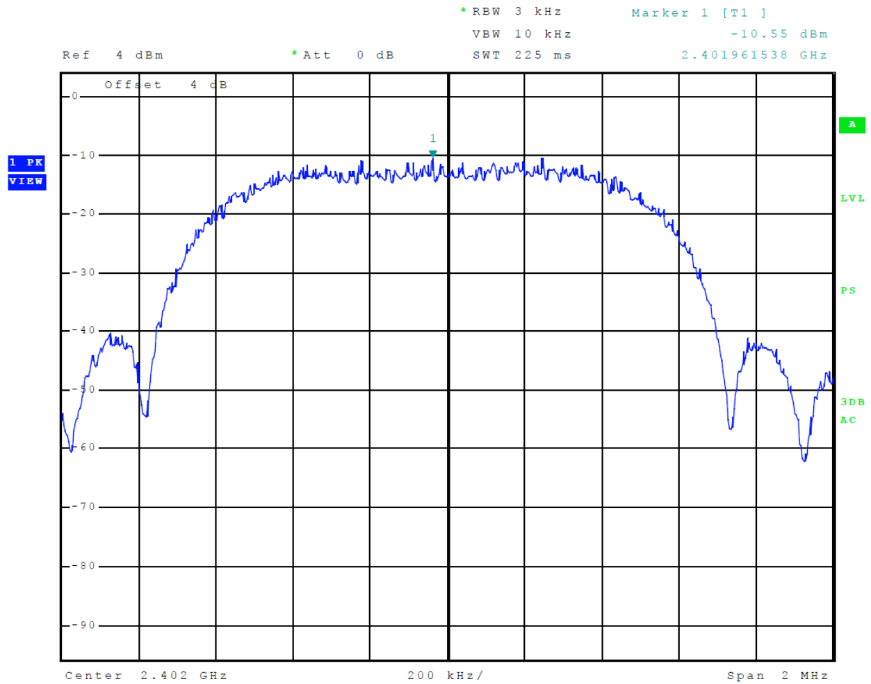
Figure 26 Plot of Transmitter Power Spectral Density Mode 3 ( \pi/4 DQPSK)
