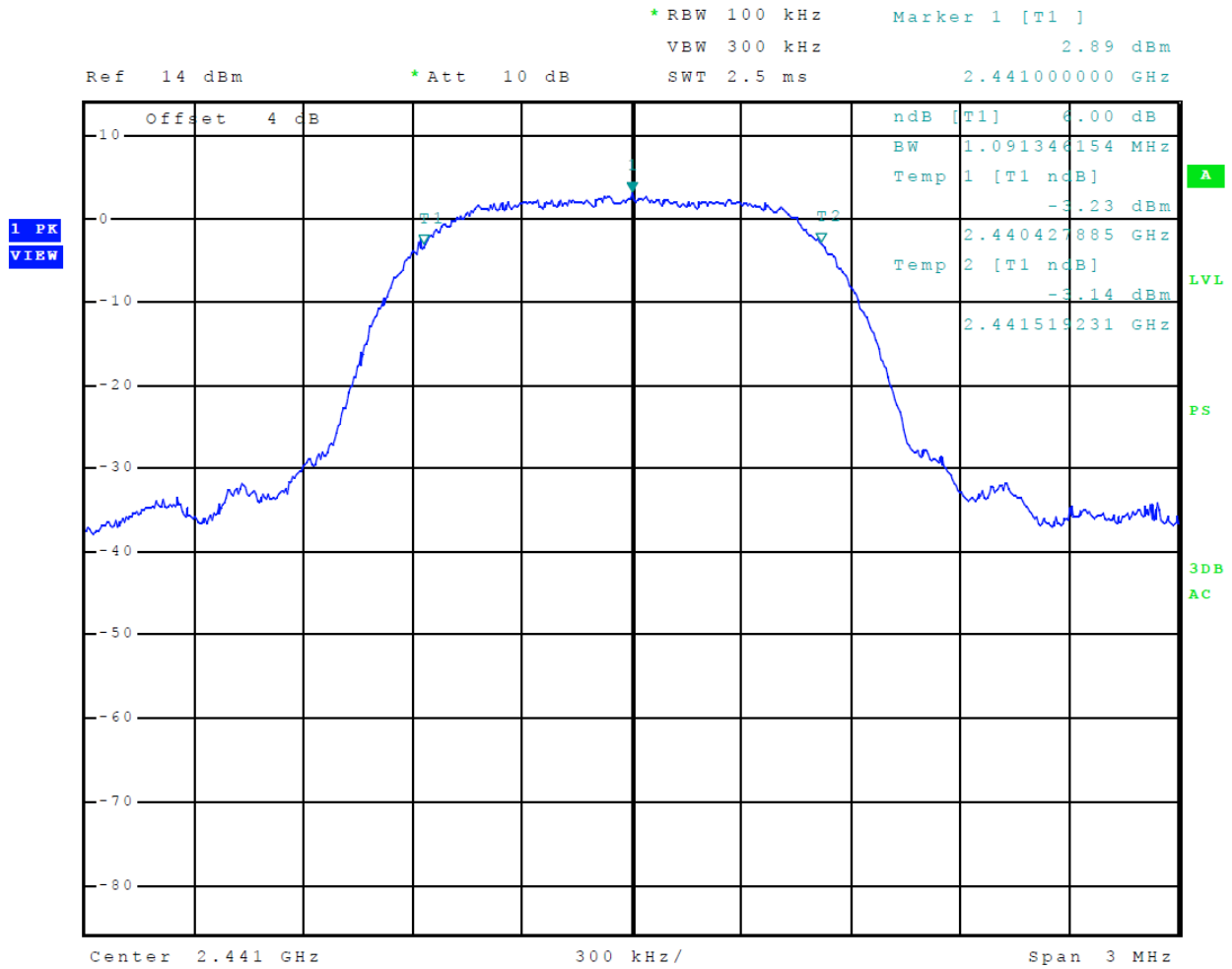
Figure 18 Plot of 6-dB Occupied Bandwidth Mode 4 (8DPSK)
