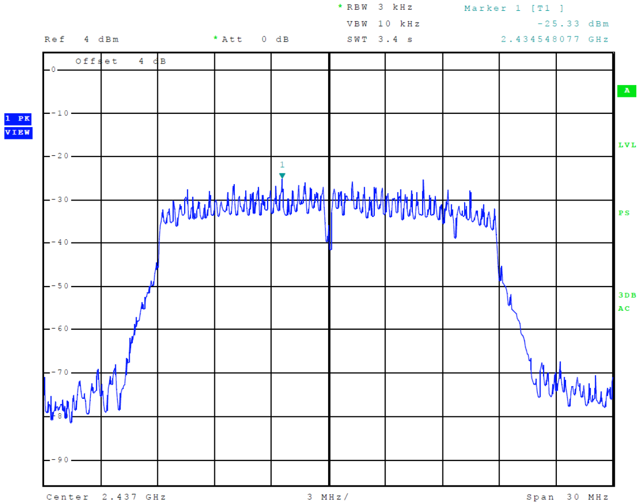
Figure 30 Plot of Transmitter Power Spectral Density Mode 7 (MCS)
