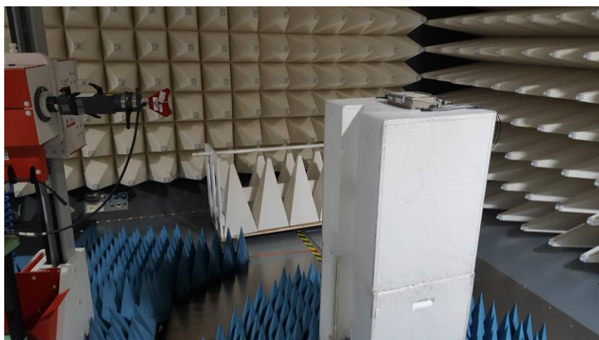
Figure B7. High Range Radiated Emission test setup 18-40GHz
