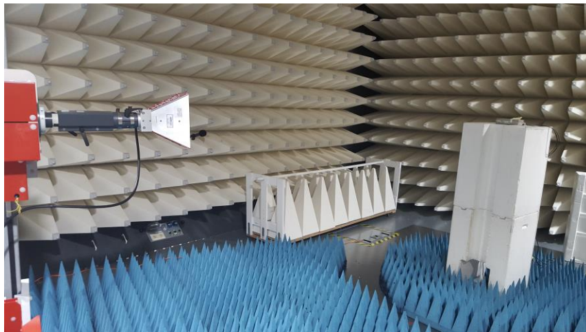
Figure B6. High Range Radiated Emission test setup 1-18GHz
