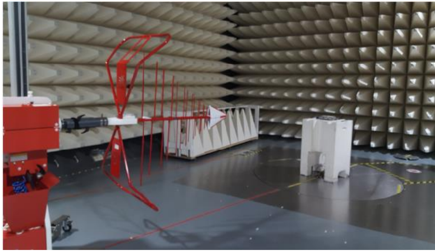
Figure D5. Radiated Emission test setup 1
