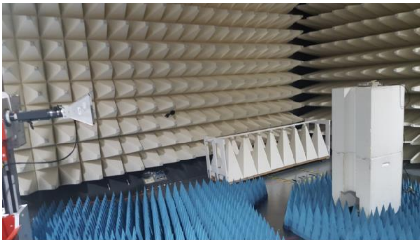
Figure D6. Radiated Emission test setup 2
