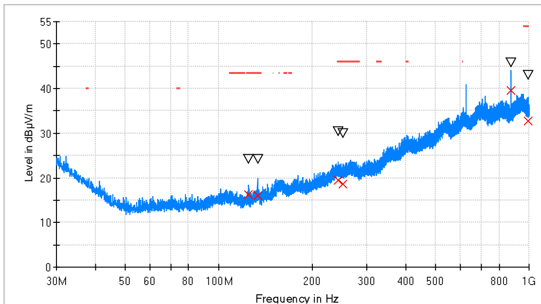
RF_FCC_15.247_E Field_30MHz_1GHz
