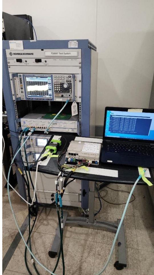
Figure C3. DFS test setup 1
