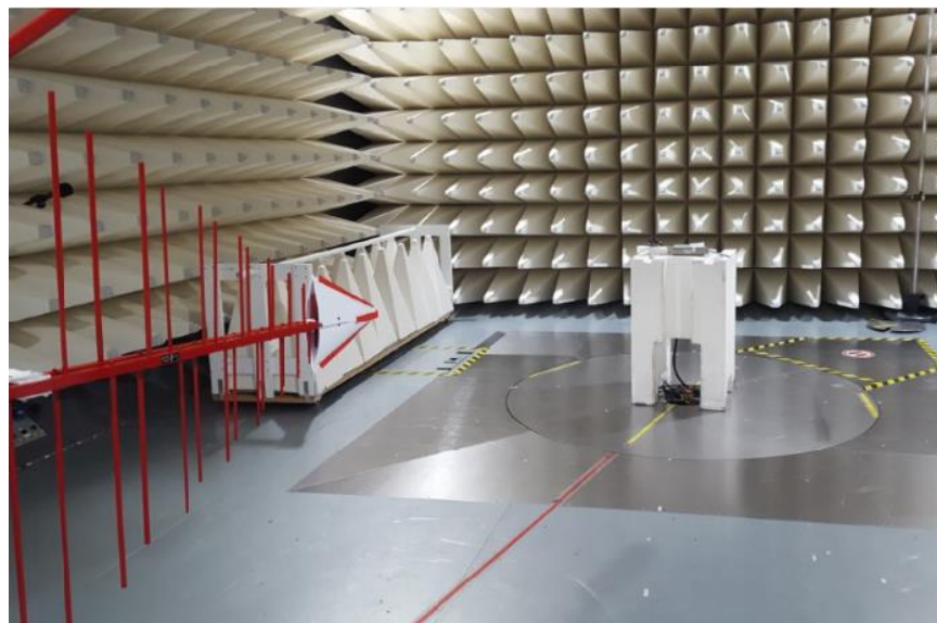
Figure B4. Radiated emission Setup 1
