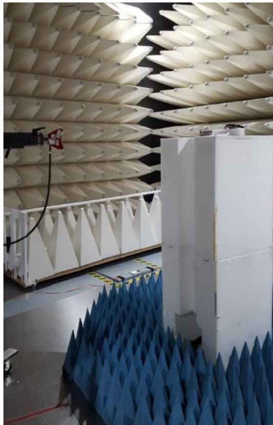
Figure B5. Radiated emission Setup 3
