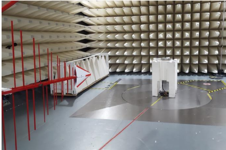
Figure B3. Radiated emission Setup 1
