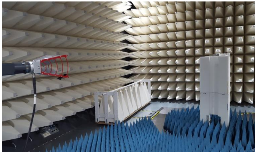
Figure B4. Radiated emission Setup 2
