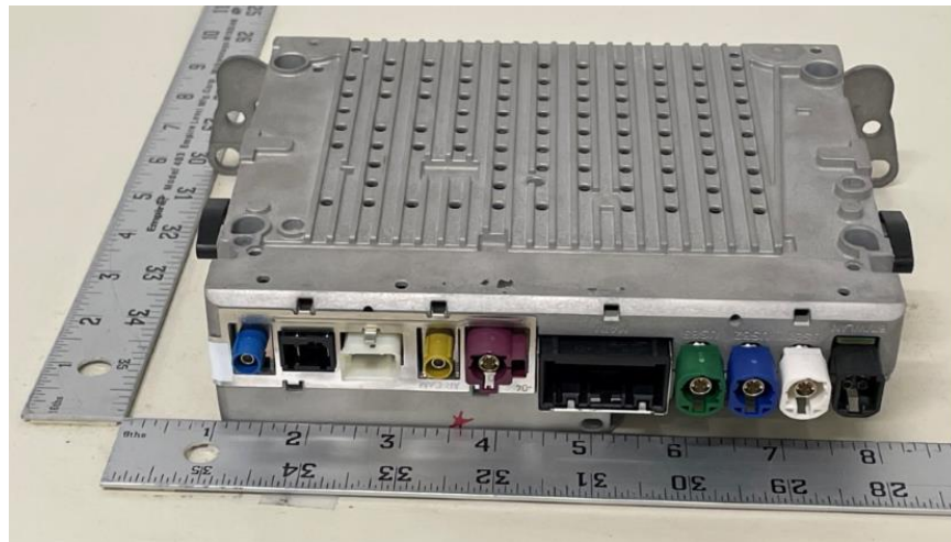
Figure B2. DUT rear view
