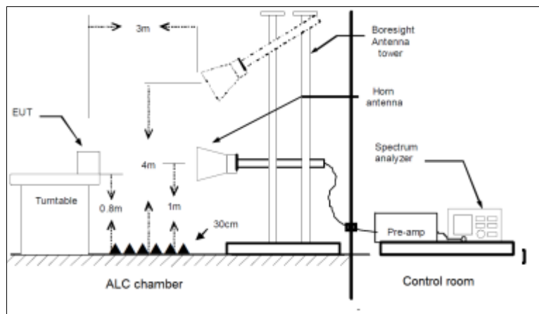
Radiated measurements setup f > 18 GHz
