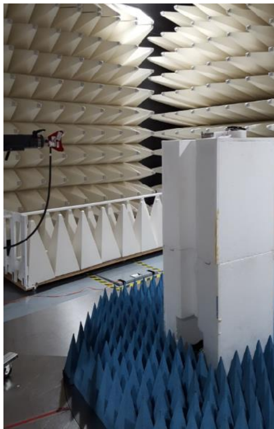
Figure B6. Radiated emission Setup 3
