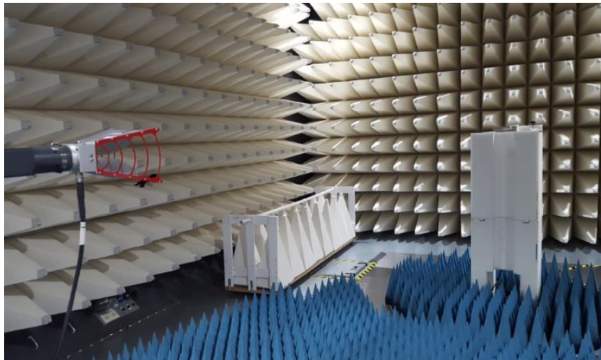
Figure B5. Radiated emission Setup 2
