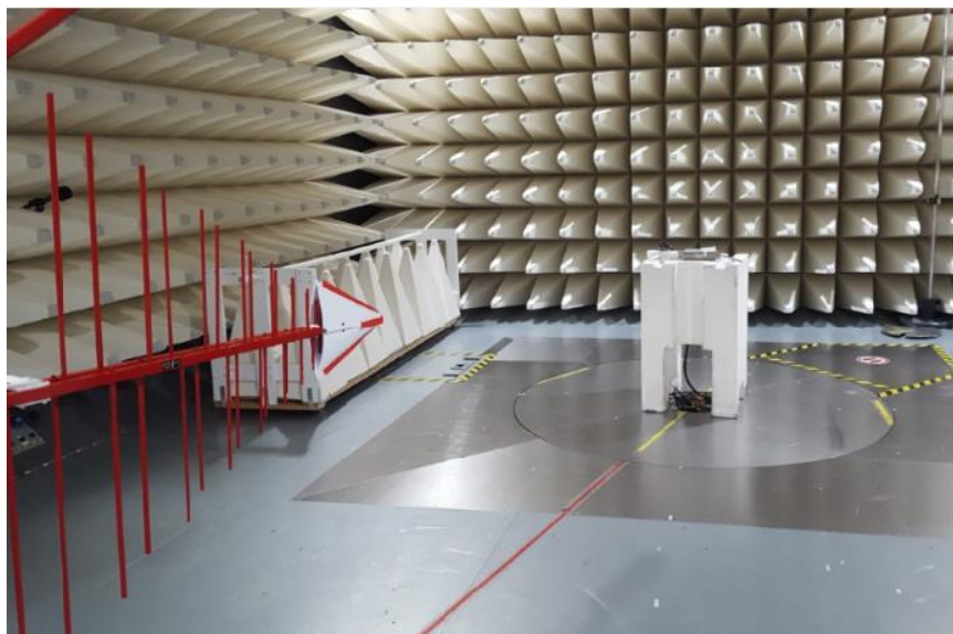
Figure B4. Radiated emission Setup 1
