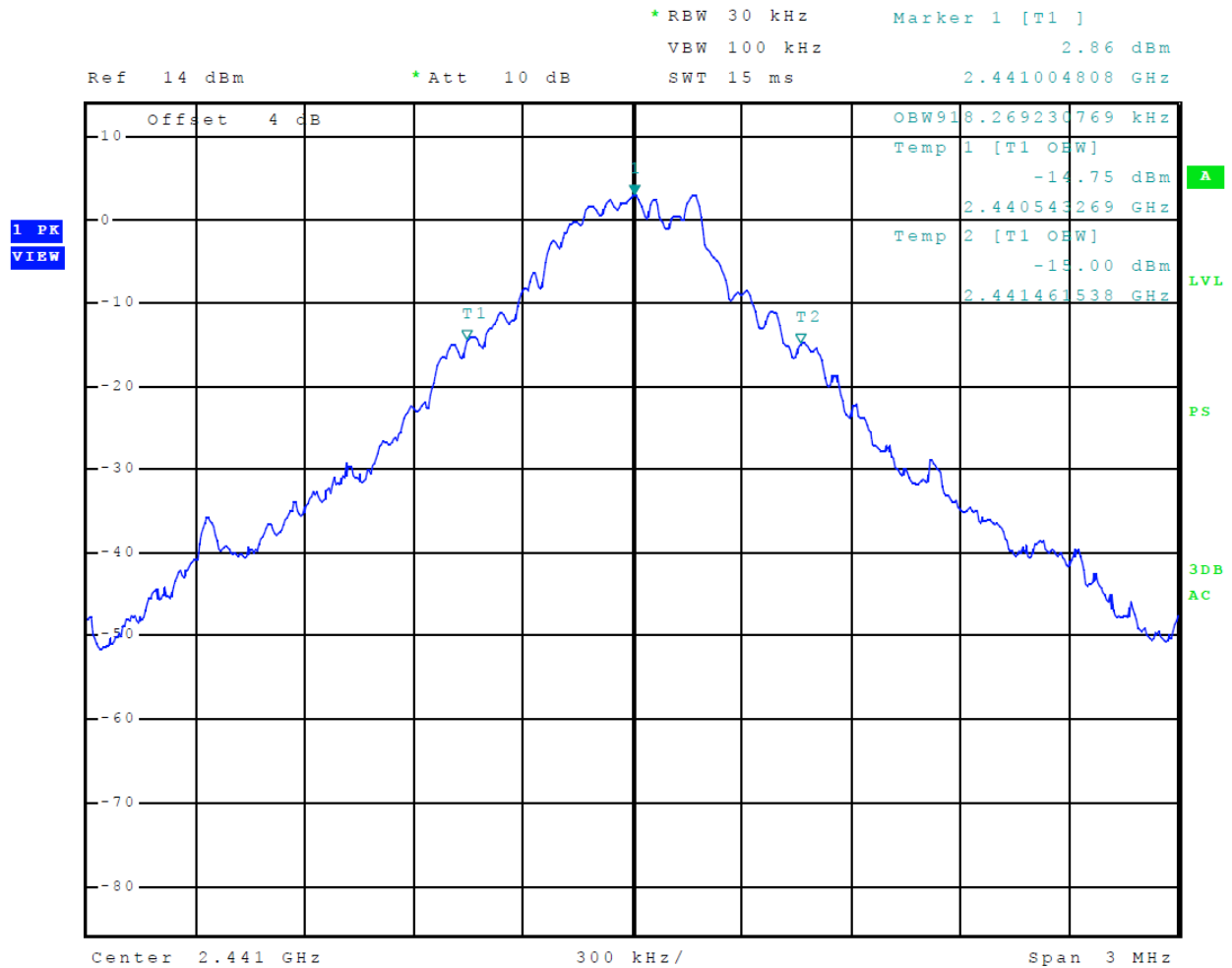
Figure 7 Plot of Transmitter Emissions 99% Occupied Bandwidth BT BR (GMSK)
