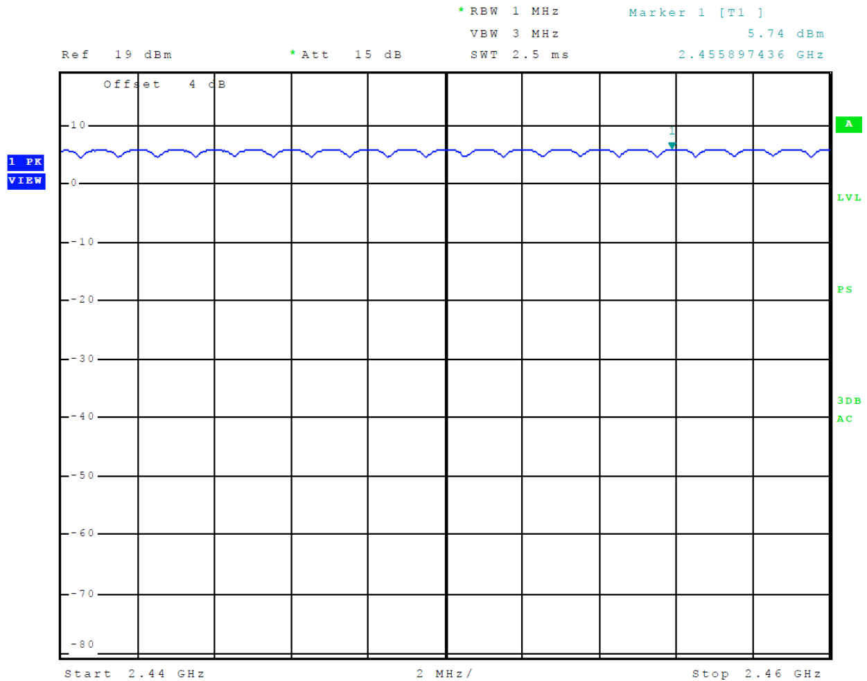
Figure 10 Plot of Number of Hopping Channels BT BR (GMSK)
