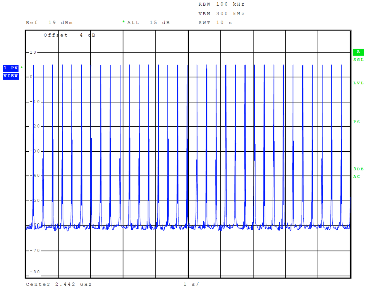
Figure 14 Plot of 34 Times on Channel over 10 second period BT BR (GMSK)
