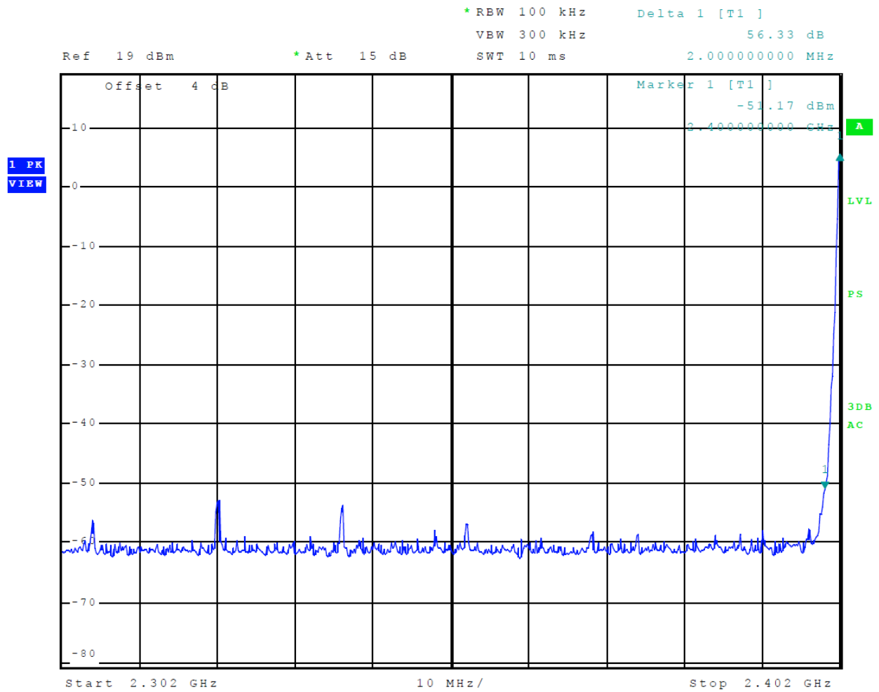
Figure 15 Plot of Transmitter Emissions Low Band Edge Channels Hopping BT BR (GFSK)
