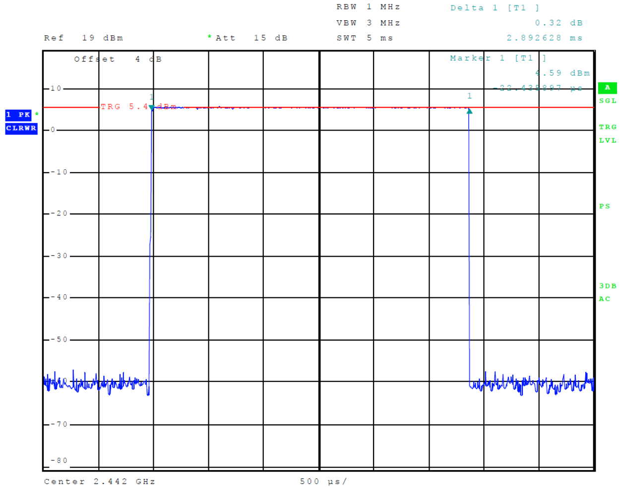
Figure 13 Plot of Dwell Time on Channel BT BR (GMSK)
