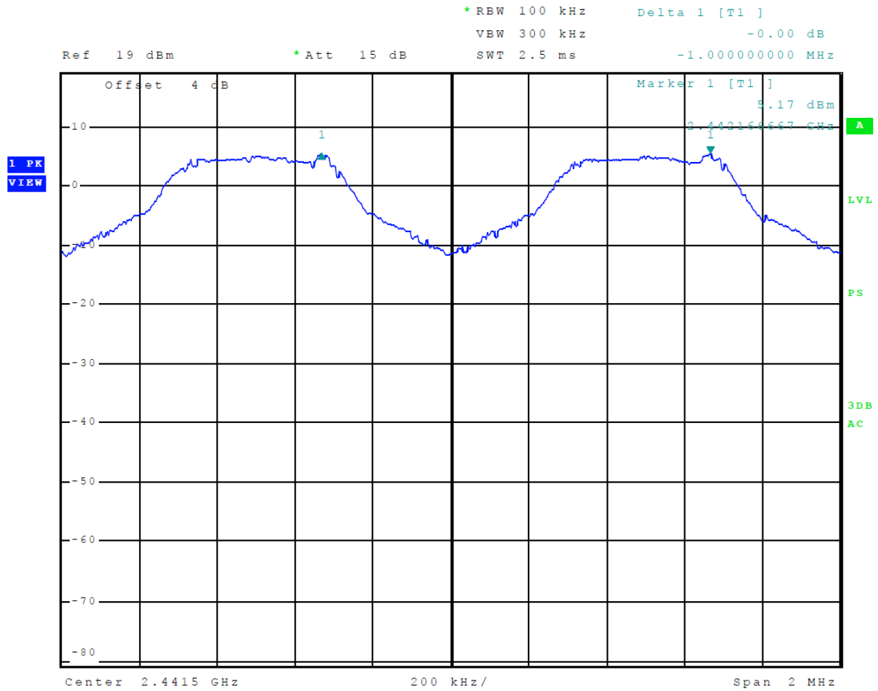
Figure 12 Plot of Channel Separation BT BR (GMSK)
