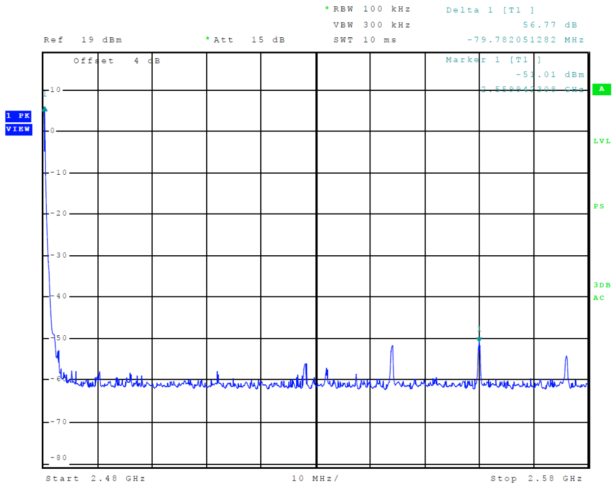
Figure 16 Plot of Transmitter Emissions High Band Edge Channels Hopping BT BR (GFSK)
