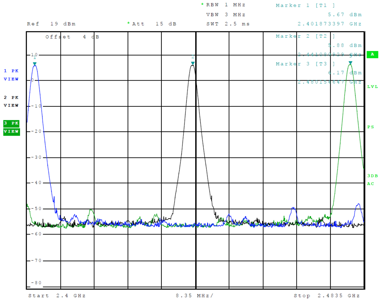
Figure 5 Plot of Transmitter Operation across 2402-2480 MHz band BT BR (GFSK)
