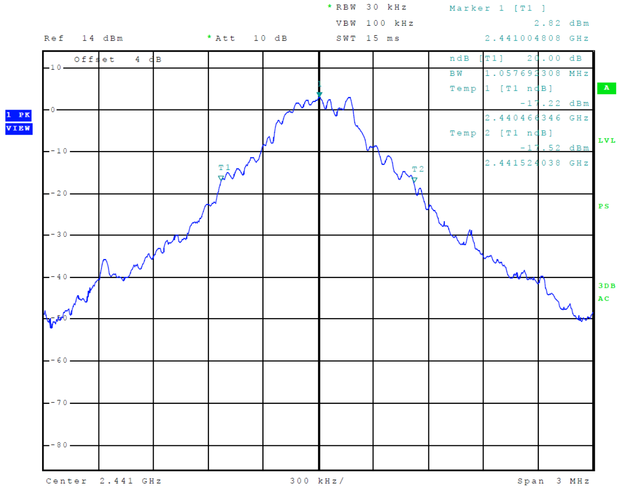
Figure 6 Plot of Transmitter Emissions 20-dB Occupied Bandwidth BT BR (GMSK)
