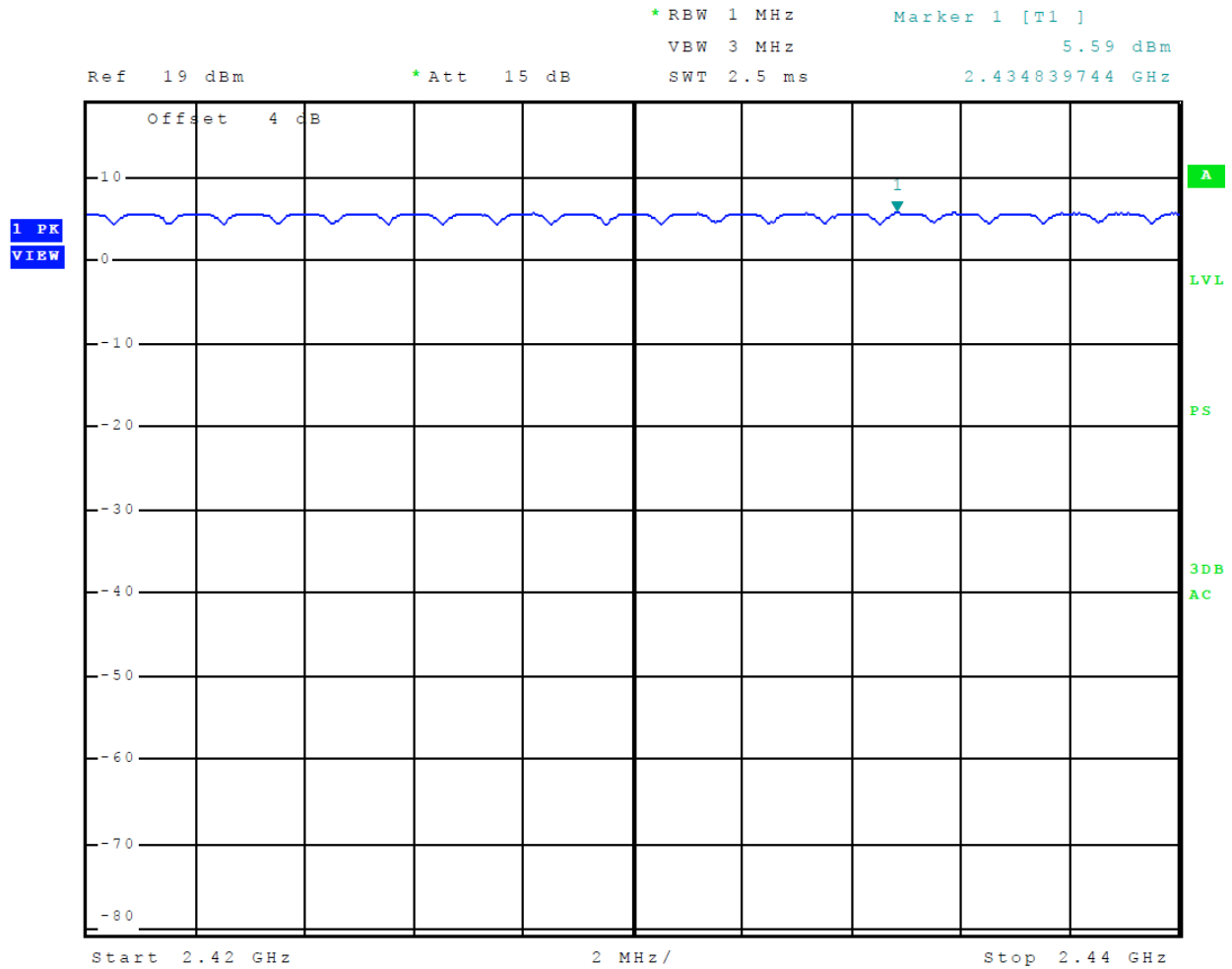
Figure 9 Plot of Number of Hopping Channels BT BR (GMSK)
