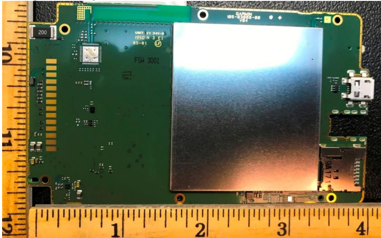
PCB Top with shielding
