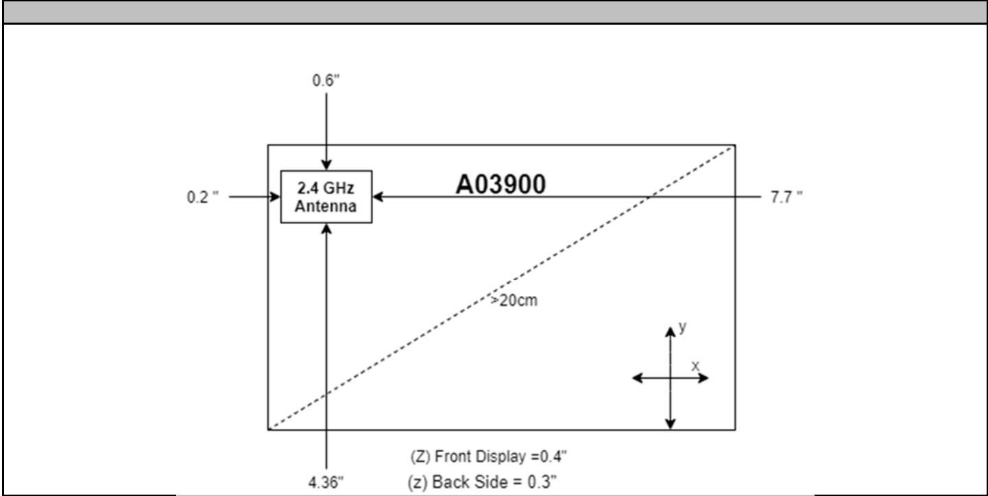
Figure A03900 (P/N:011-05116-XX) – 2.4GHz Antenna Location Diagram D6
