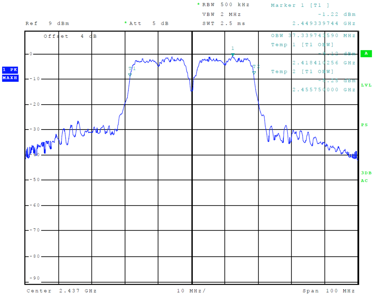
Figure 39 Plot of 99% Occupied Bandwidth (Mode 8, 802.11n40)
