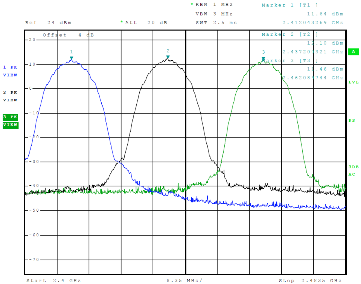
Figure 8 Plot of Transmitter Operation in 2412-2462 MHz (Mode 5, 802.11b)
