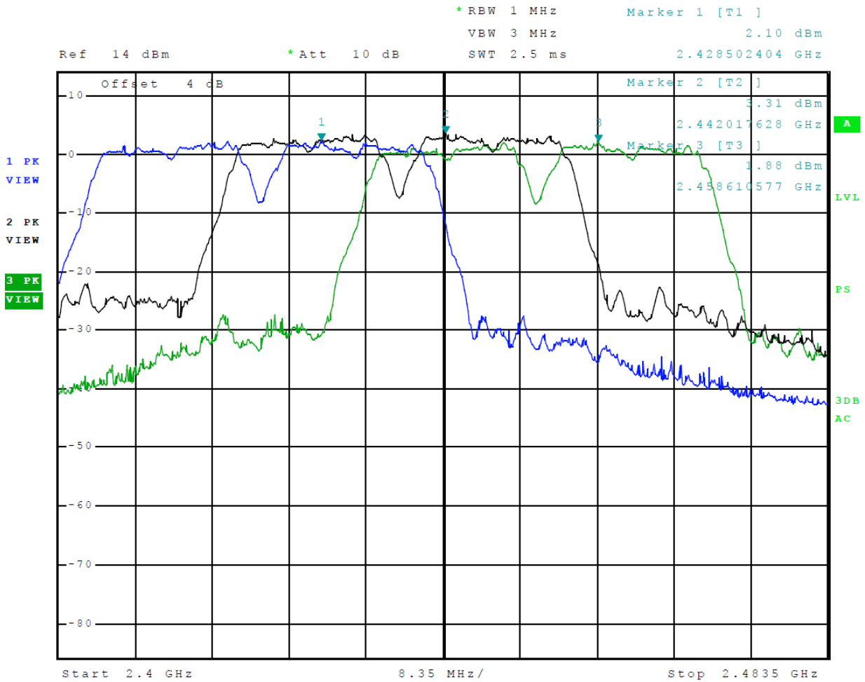
Figure 11 Plot of Transmitter Operation in 2412-2462 MHz (Mode 8, 802.11n40)
