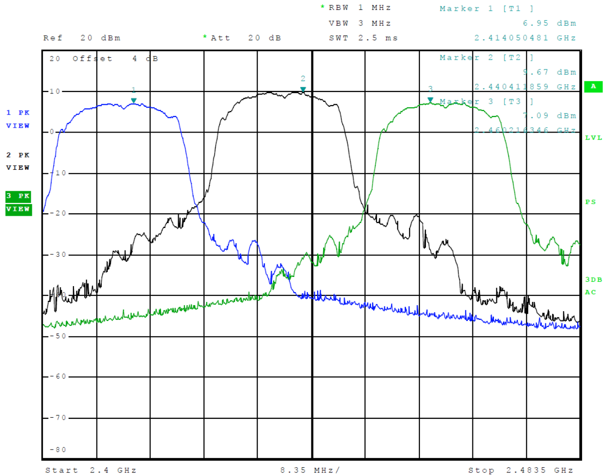
Figure 9 Plot of Transmitter Operation in 2412-2462 MHz (Mode 6, 802.11g)
