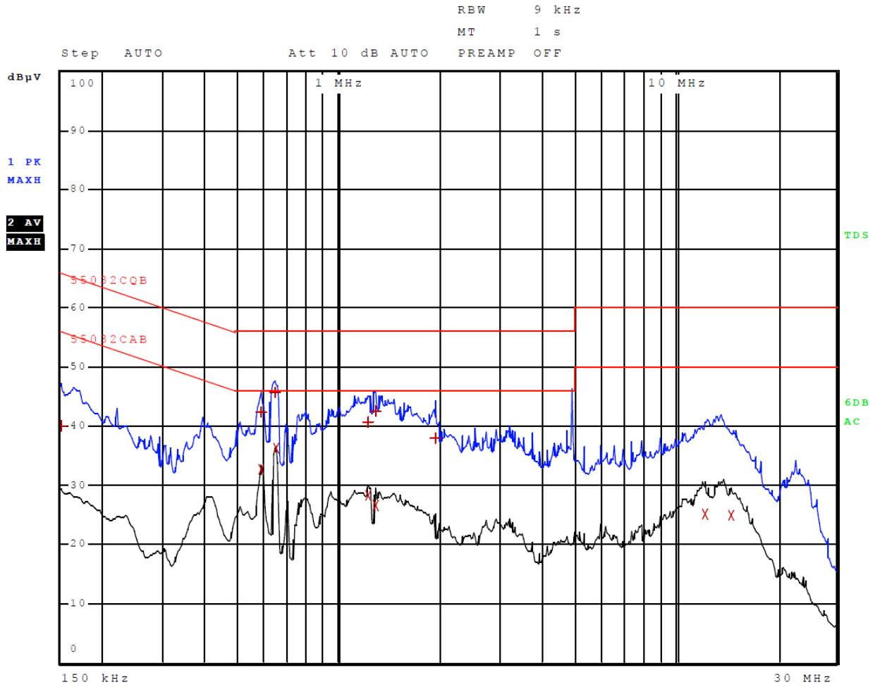
Figure 1 AC Line Conducted emissions of EUT line 1 (Configuration #3, EUT – 362-00096-00)
