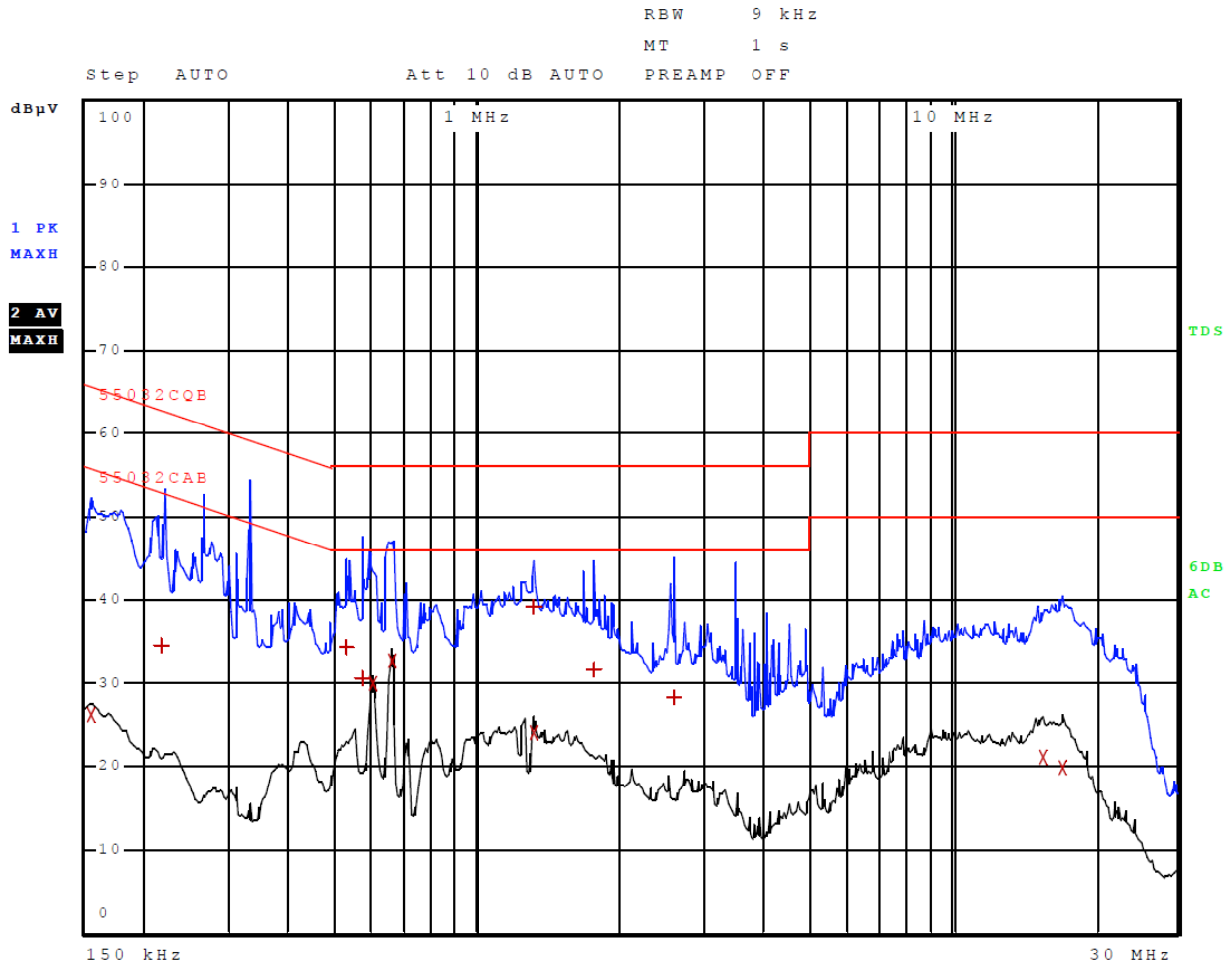
Figure 2 AC Line Conducted emissions of EUT line 2 (Configuration #3, EUT – 362-00096-00)
