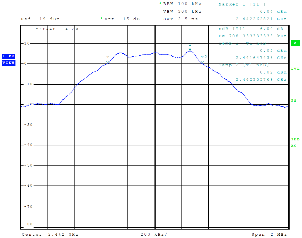
Figure 30 Plot of 6-dB Occupied Bandwidth (Mode 4, BLE)
