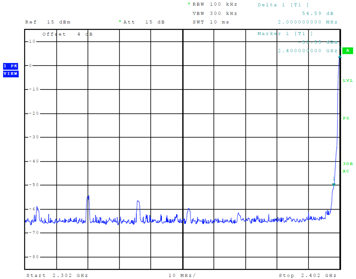
Figure 13 Plot of Transmitter Emissions Low Band Edge (Mode 3, 3EDR)
