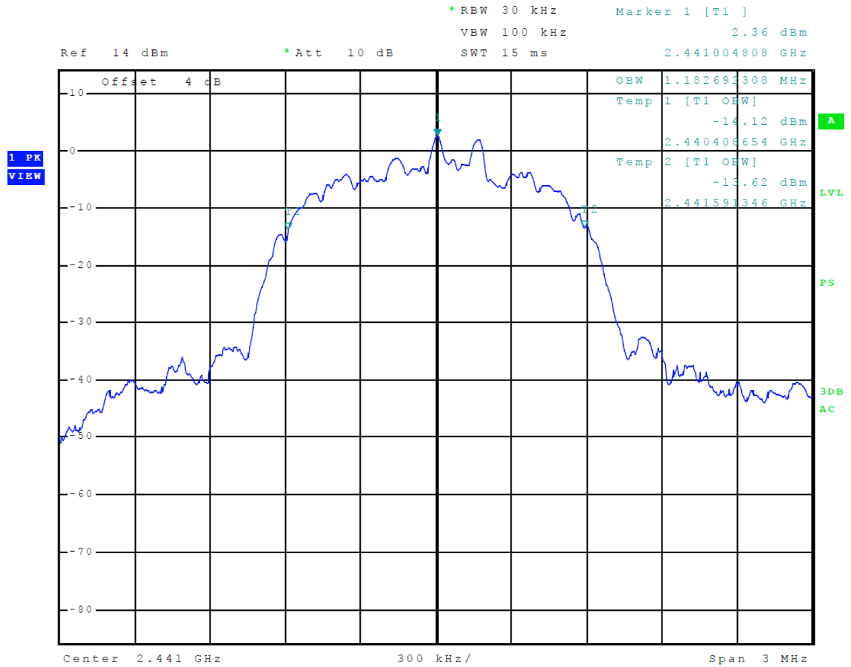
Figure 29 Plot of 99% Occupied Bandwidth (Mode 3, 3EDR)
