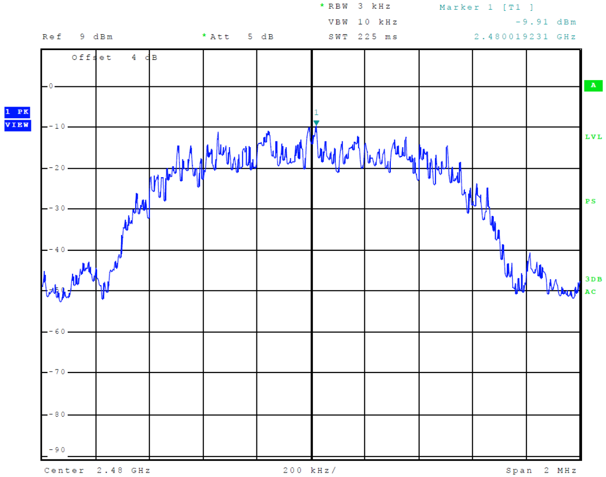
Figure 40 Plot of Transmitter Power Spectral Density (Mode 2, 2EDR)
