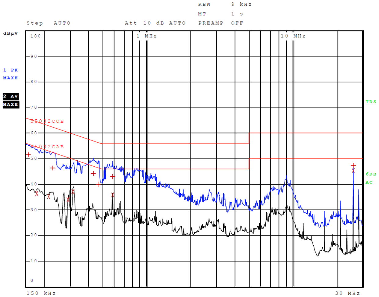
Figure 4 AC Line Conducted emissions of EUT line 2 (Configuration #4, EUT – Computer)
