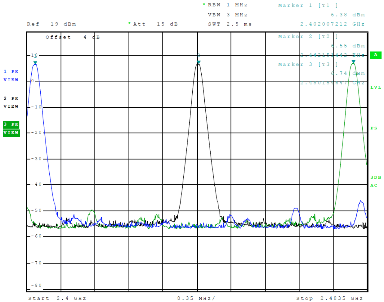
Figure 7 Plot of Transmitter Operation in 2402-2480 MHz (Mode 4, BLE)
