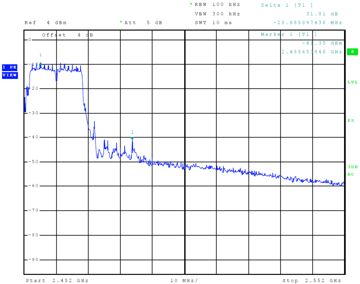
Figure 25 Plot of Transmitter Emissions High Band Edge (Mode 8, 802.11n40)
