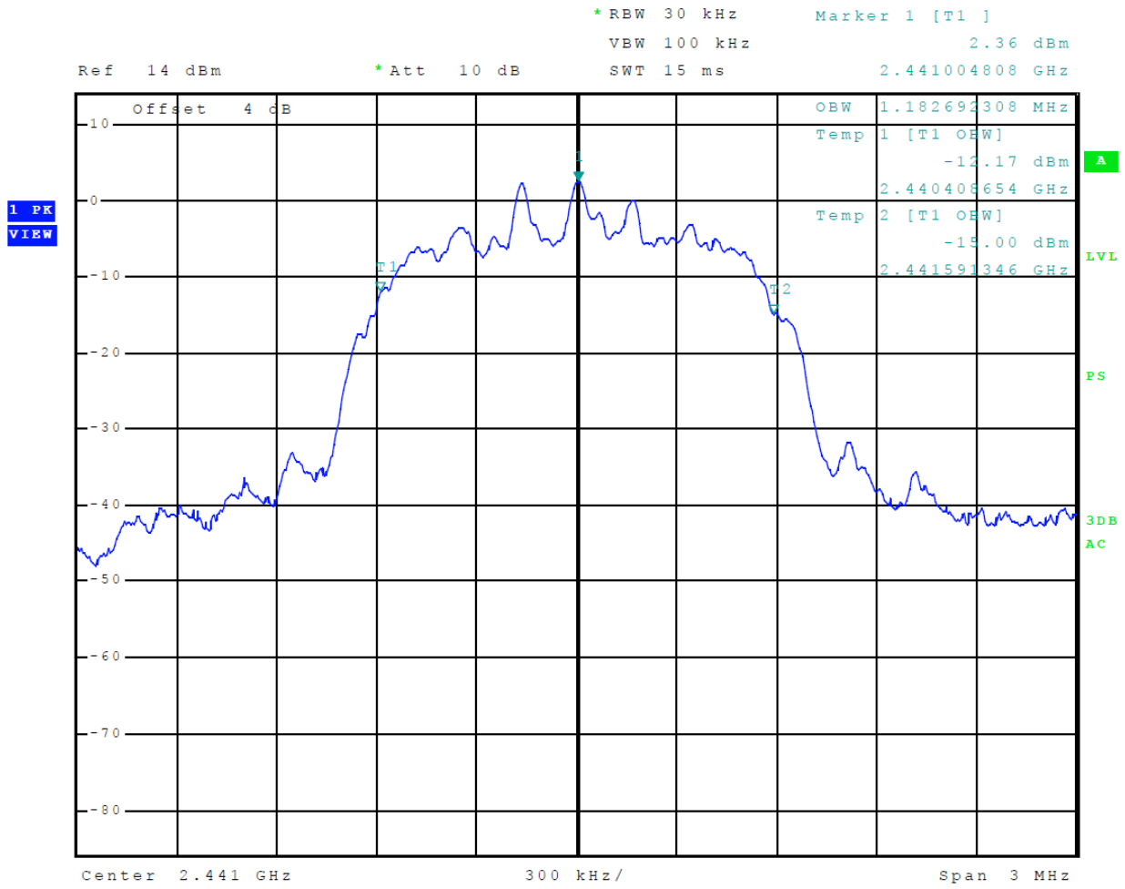
Figure 27 Plot of 99% Occupied Bandwidth (Mode 2, 2EDR)
