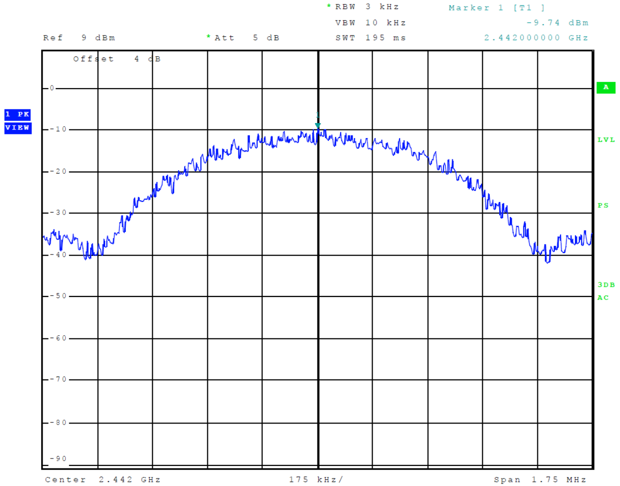
Figure 42 Plot of Transmitter Power Spectral Density (Mode 4, BLE)
