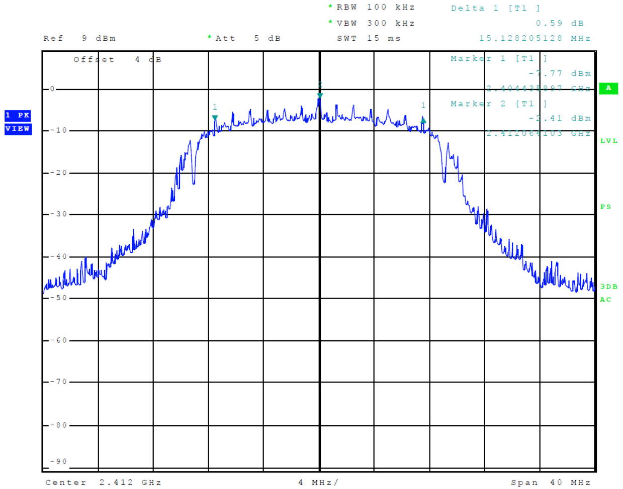
Figure 36 Plot of 6-dB Occupied Bandwidth (Mode 7, 802.11n)
