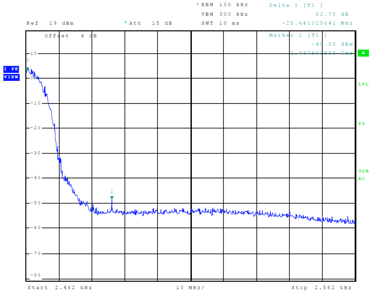
Figure 22 Plot of Transmitter Emissions High Band Edge (Mode 5, 802.11b)
