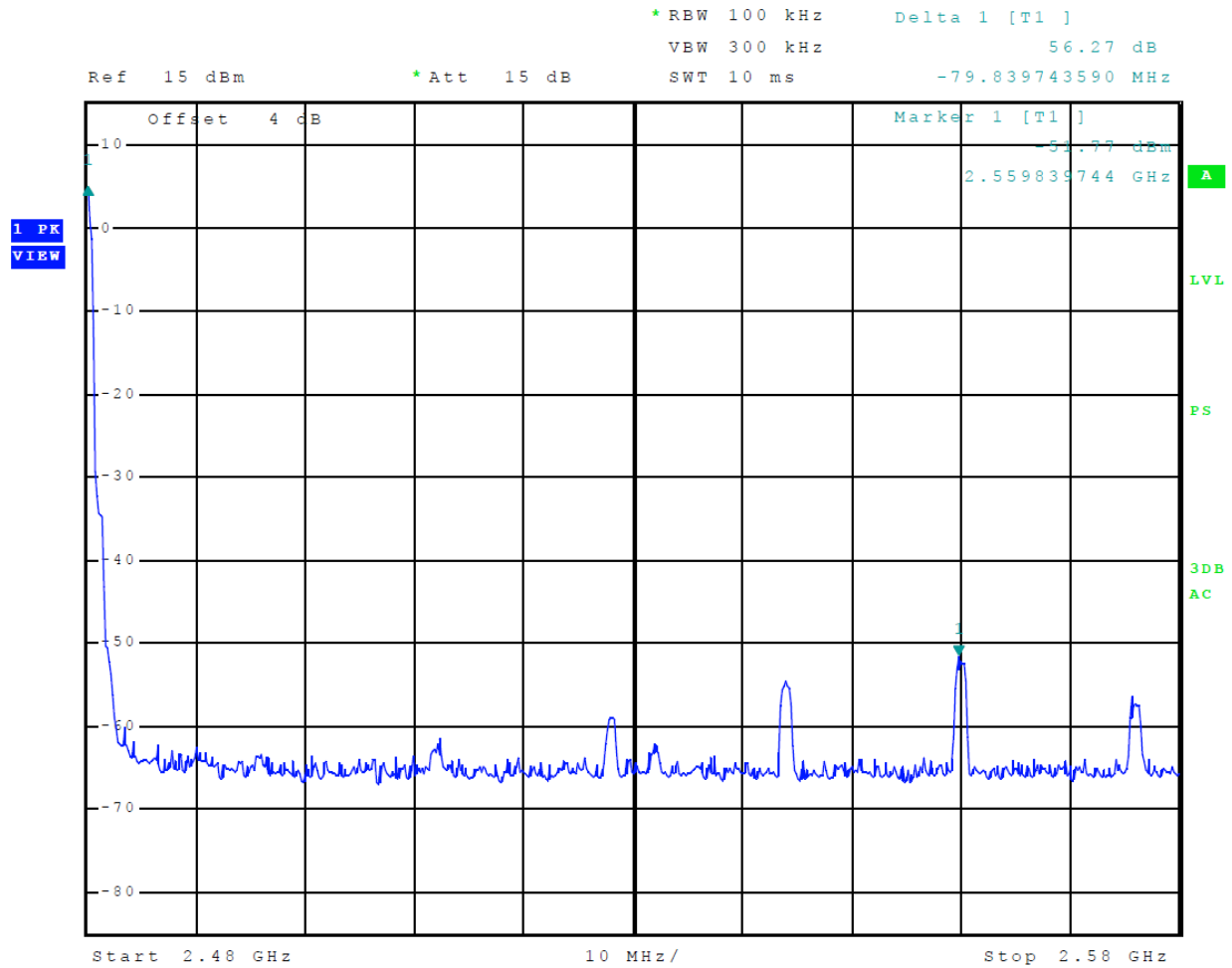
Figure 19 Plot of Transmitter Emissions High Band Edge (Mode 2, 2EDR)
