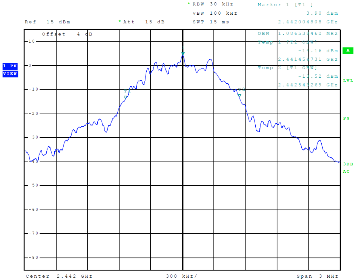
Figure 31 Plot of 99% Occupied Bandwidth (Mode 4, BLE)
