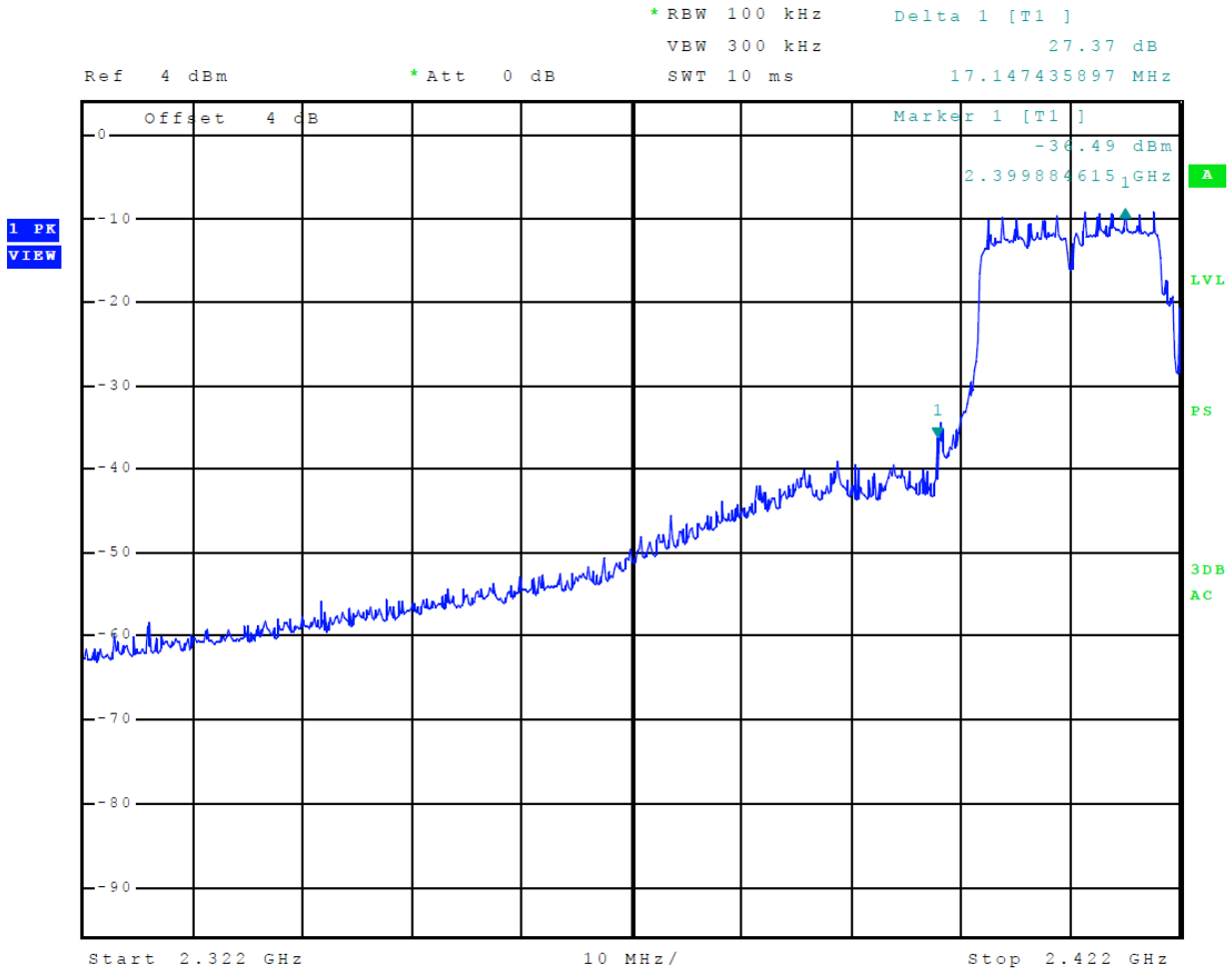
Figure 18 Plot of Transmitter Emissions Low Band Edge (Mode 8, 802.11n40)
