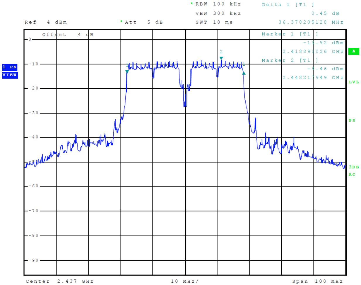
Figure 38 Plot of 6-dB Occupied Bandwidth (Mode 8, 802.11n40)
