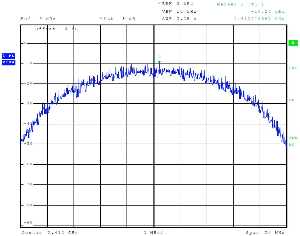
Figure 43 Plot of Transmitter Power Spectral Density (Mode 5, 802.11b)
