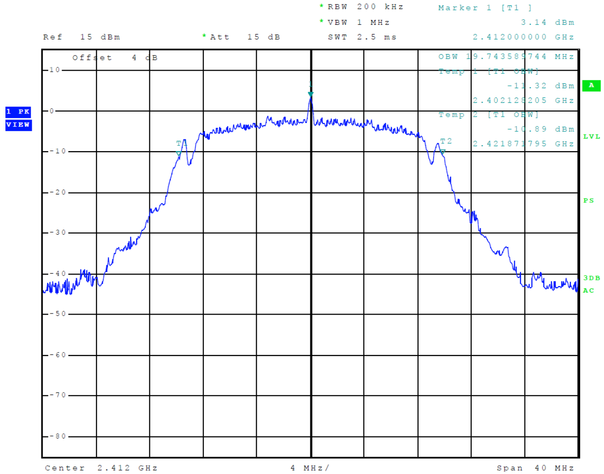
Figure 37 Plot of 99% Occupied Bandwidth (Mode 7, 802.11n)
