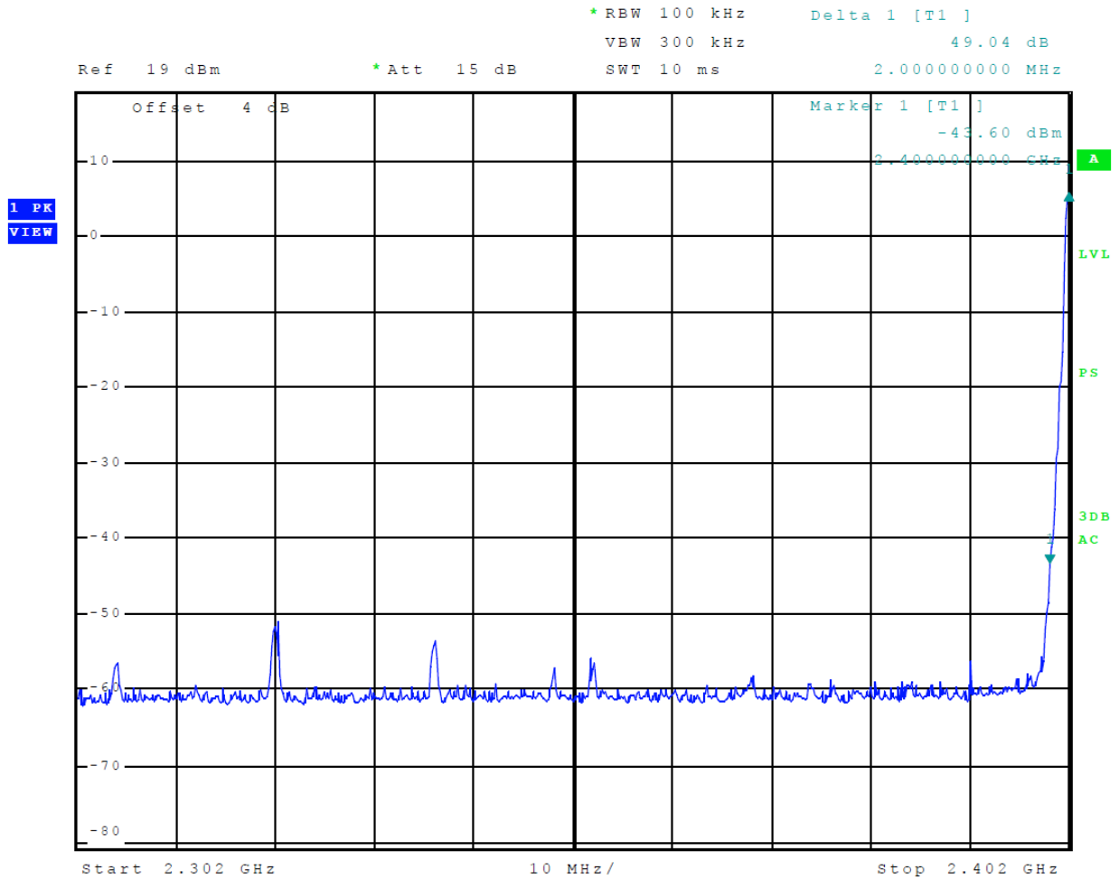
Figure 14 Plot of Transmitter Emissions Low Band Edge (Mode 4, BLE)
