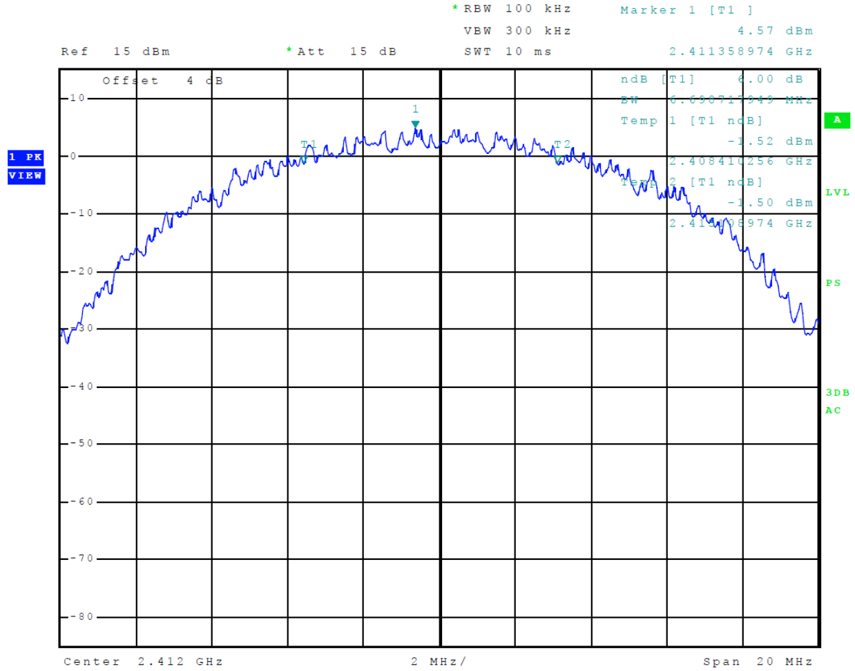
Figure 32 Plot of 6-dB Occupied Bandwidth (Mode 5, 802.11b)
