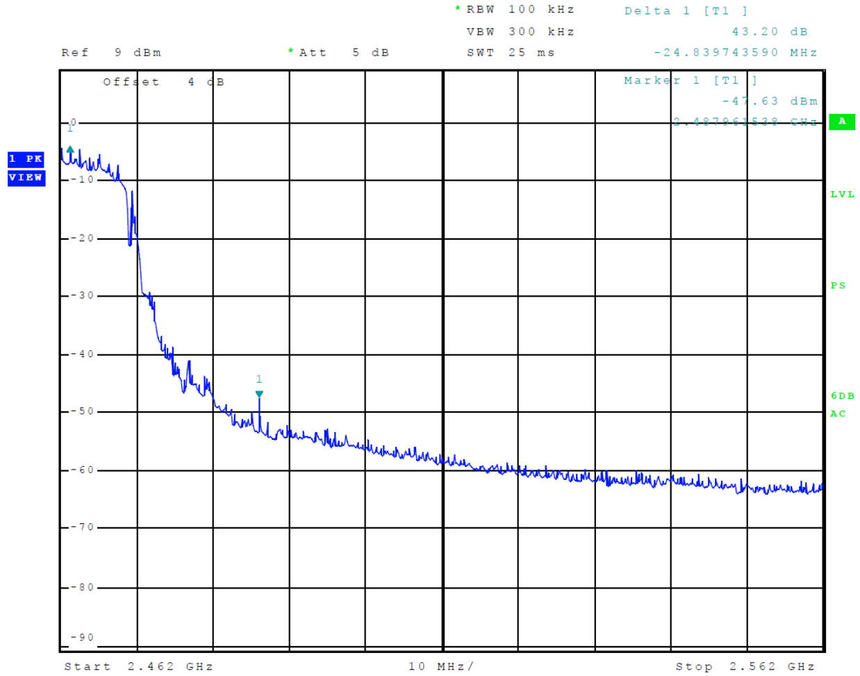
Figure 24 Plot of Transmitter Emissions High Band Edge (Mode 7, 802.11n)
