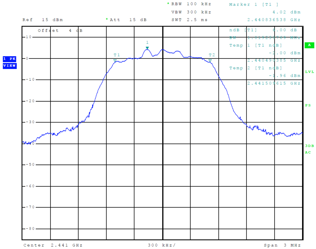
Figure 26 Plot of 6-dB Occupied Bandwidth (Mode 2, 2EDR)
