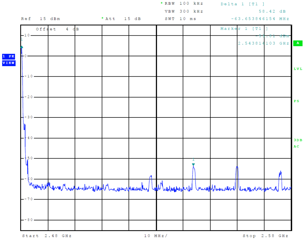
Figure 20 Plot of Transmitter Emissions High Band Edge (Mode 3, 3EDR)
