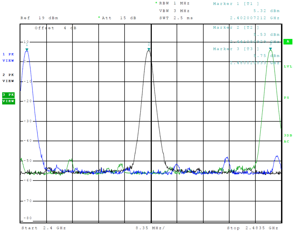
Figure 5 Plot of Transmitter Operation in 2402-2480 MHz (Mode 2, 2EDR)
