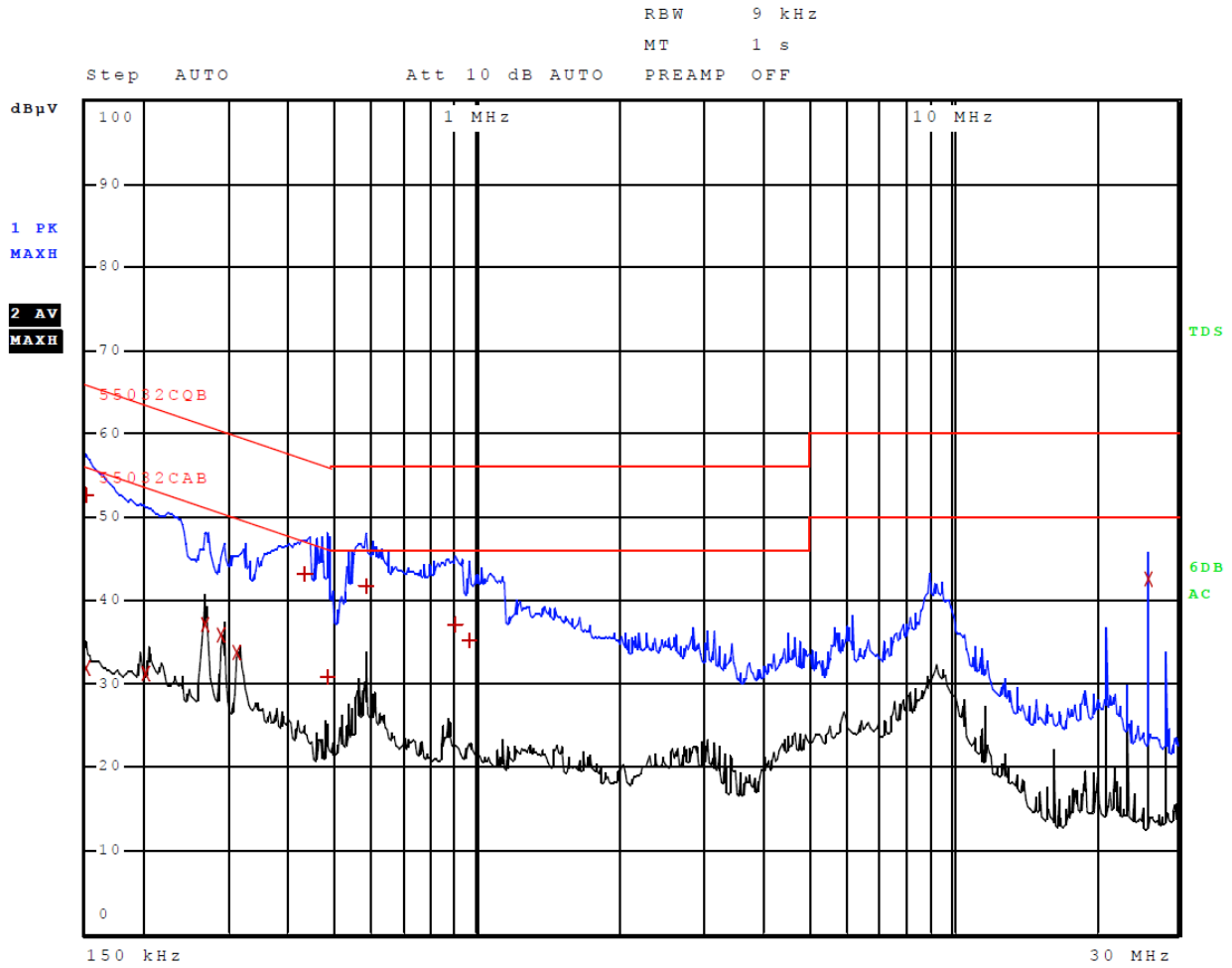
Figure 3 AC Line Conducted emissions of EUT line 1 (Configuration #4, EUT – Computer)
