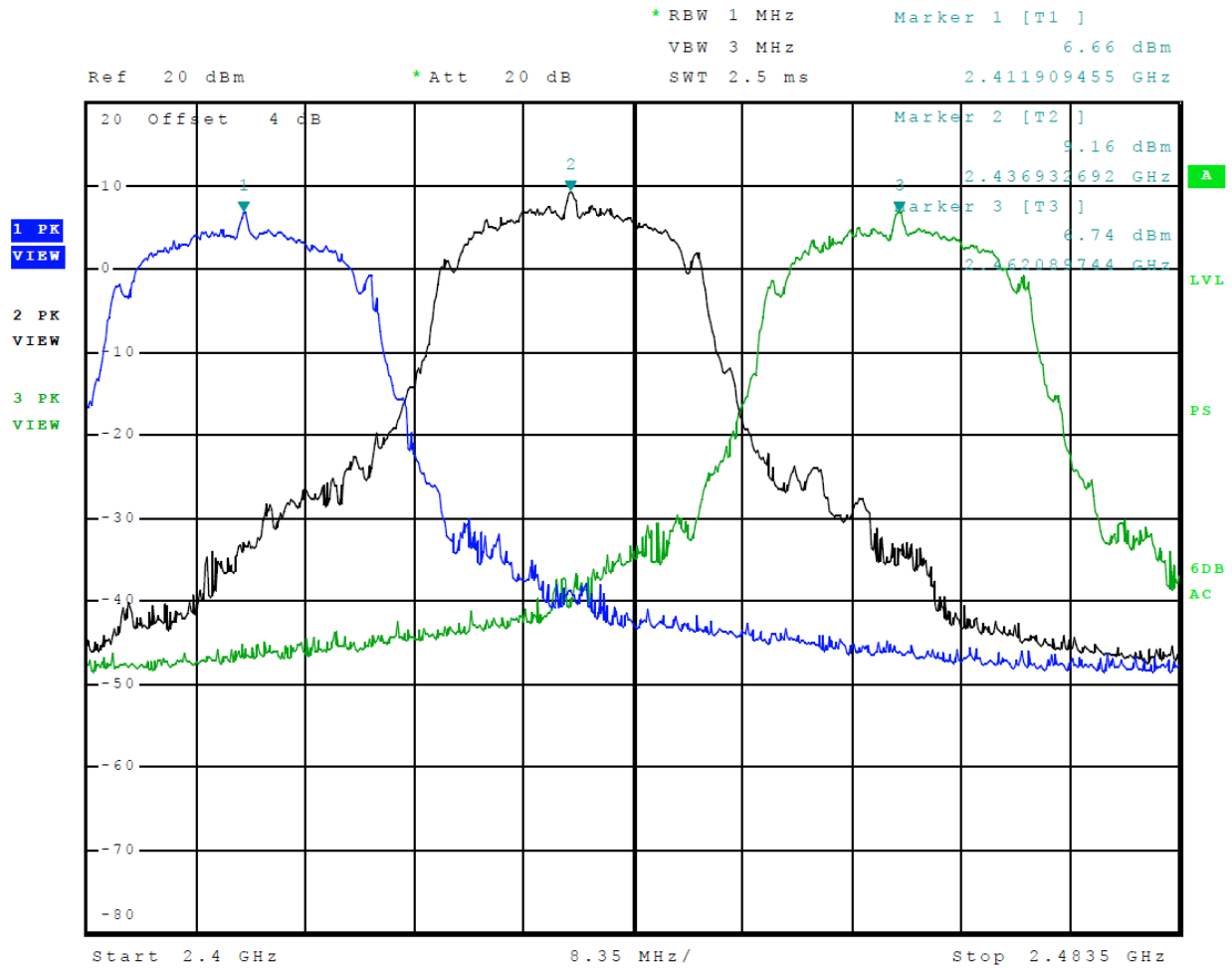
Figure 10 Plot of Transmitter Operation in 2412-2462 MHz (Mode 7, 802.11n)
