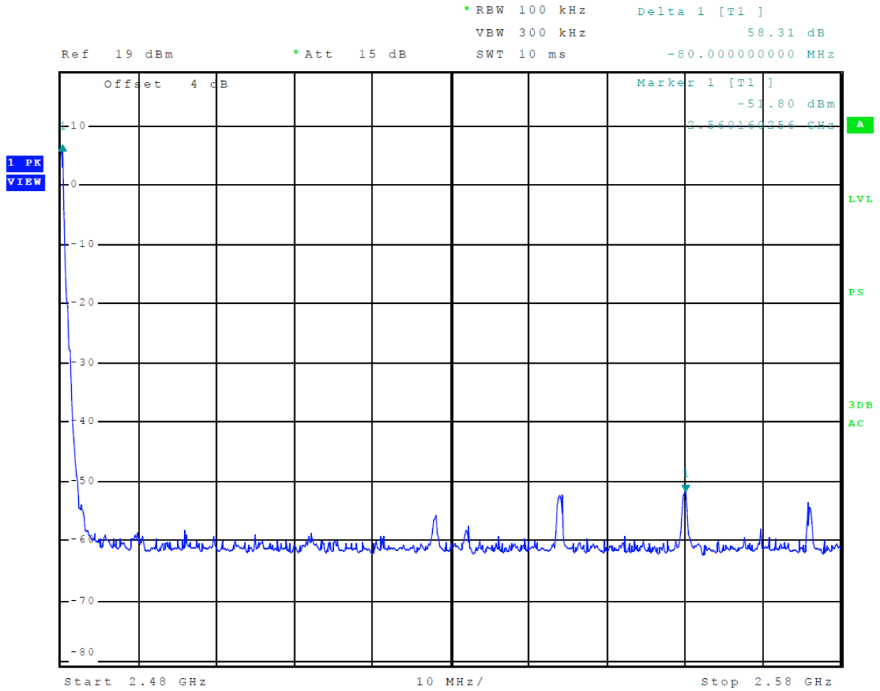
Figure 21 Plot of Transmitter Emissions High Band Edge (Mode 4, BLE)
