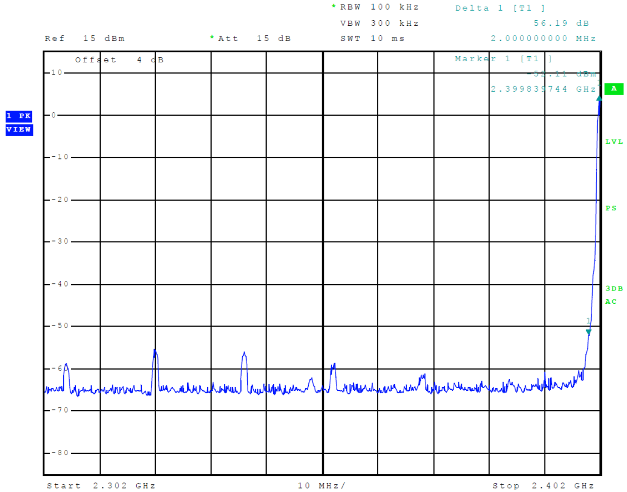
Figure 12 Plot of Transmitter Emissions Low Band Edge (Mode 2, 2EDR)
