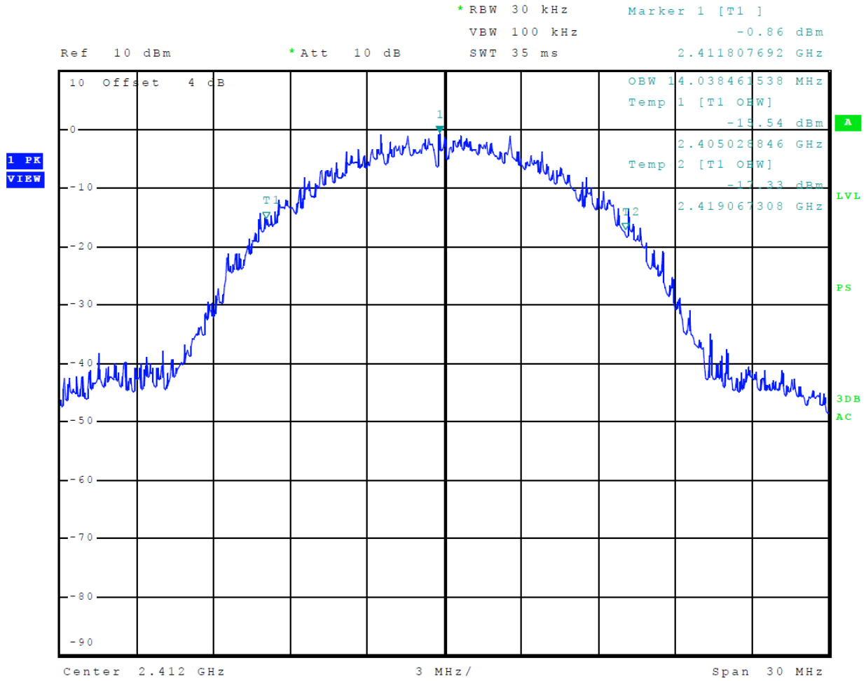
Figure 33 Plot of 99% Occupied Bandwidth (Mode 5, 802.11b)
