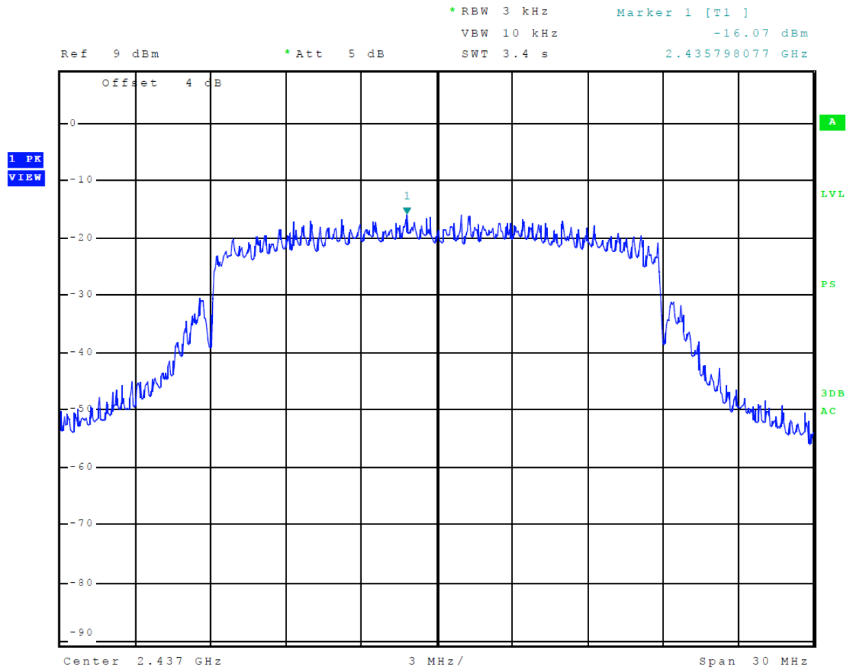
Figure 45 Plot of Transmitter Power Spectral Density (Mode 7, 802.11n)
