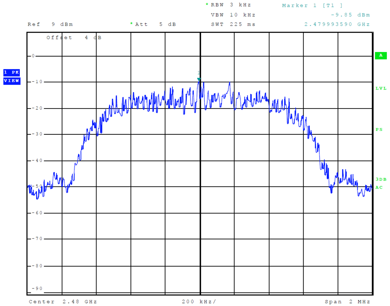
Figure 41 Plot of Transmitter Power Spectral Density (Mode 3, 3EDR)
