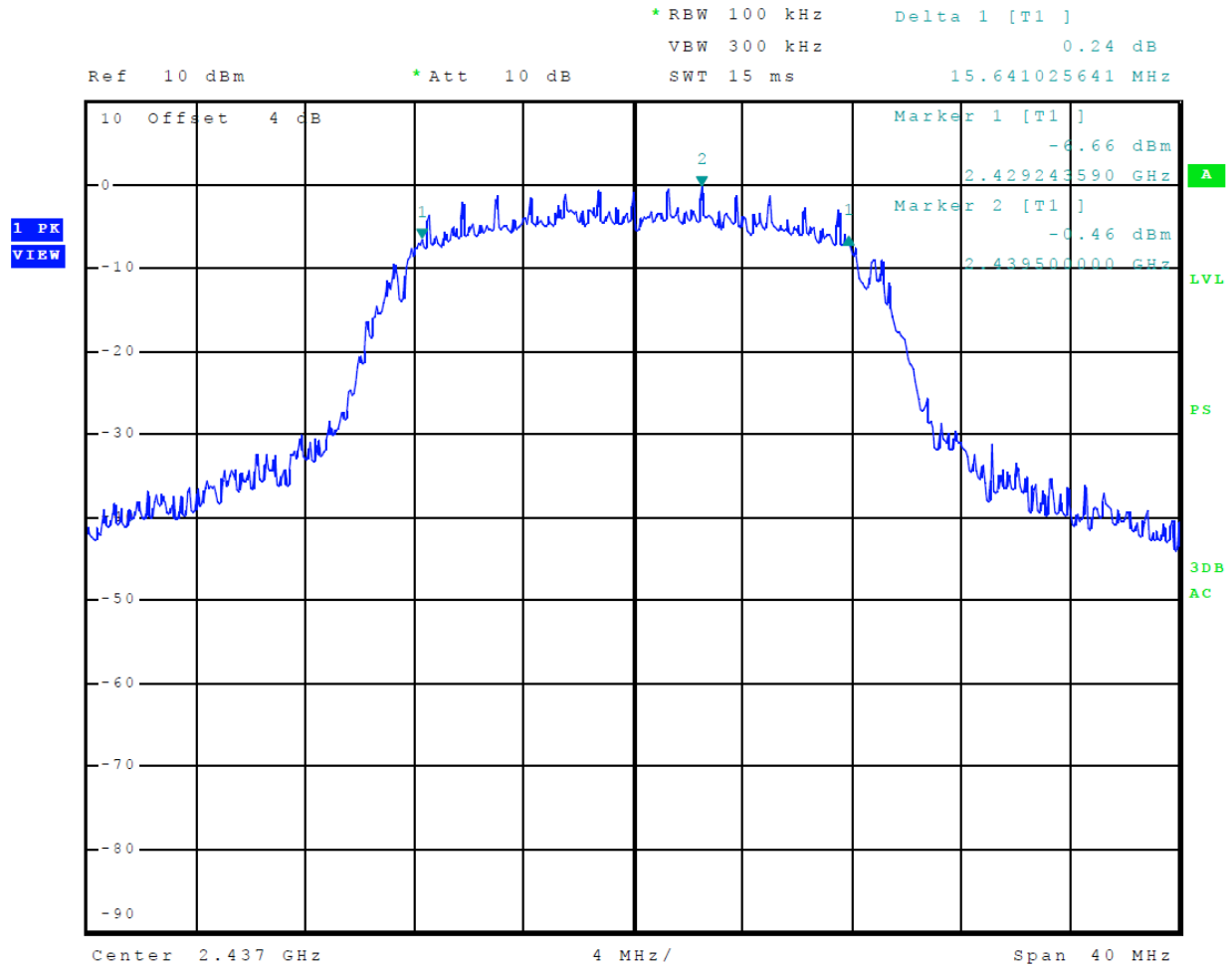
Figure 34 Plot of 6-dB Occupied Bandwidth (Mode 6, 802.11g)
