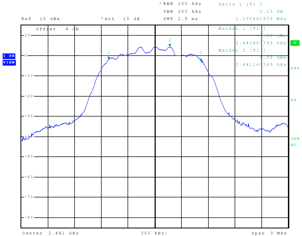
Figure 28 Plot of 6-dB Occupied Bandwidth (Mode 3, 3EDR)
