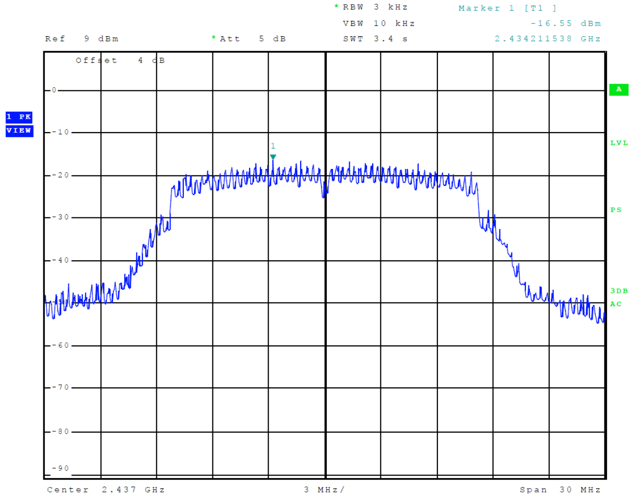
Figure 44 Plot of Transmitter Power Spectral Density (Mode 6, 802.11g)
