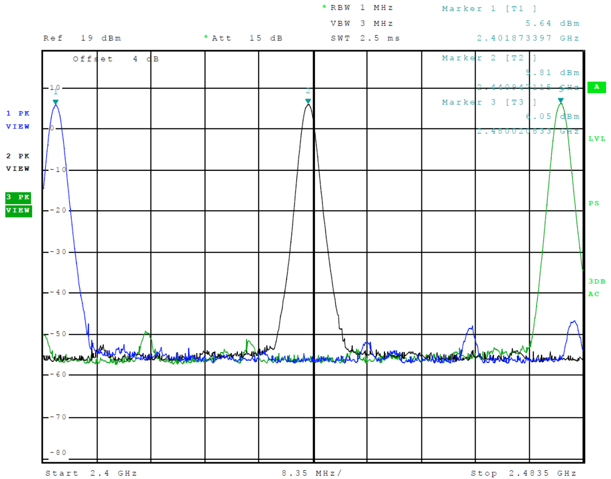
Figure 6 Plot of Transmitter Operation in 2402-2480 MHz (Mode 3, 3EDR)
