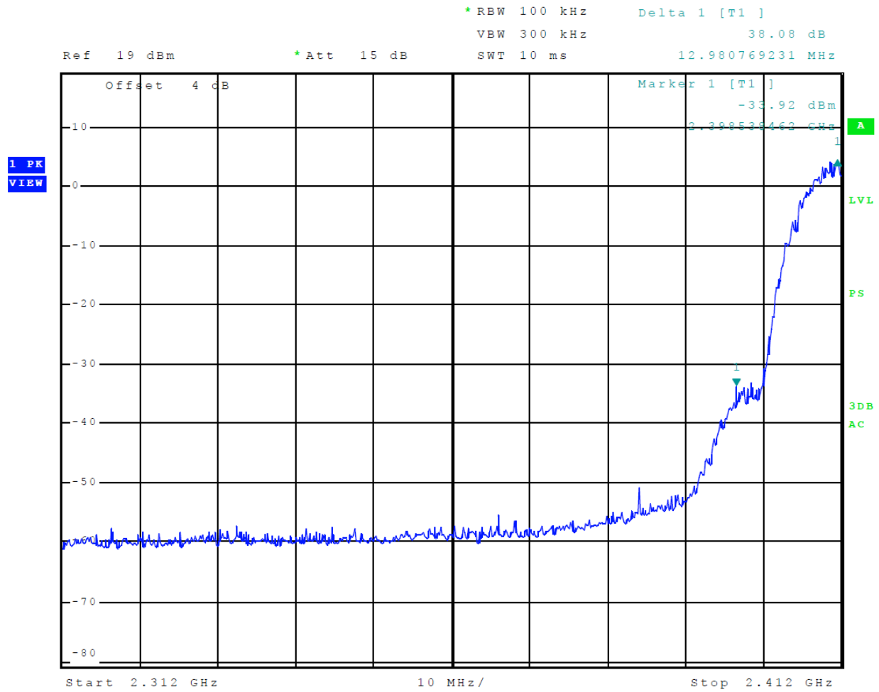
Figure 15 Plot of Transmitter Emissions Low Band Edge (Mode 5, 802.11b)
