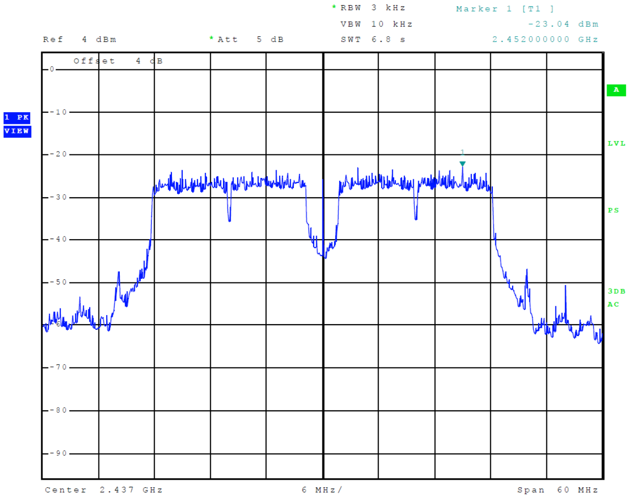
Figure 46 Plot of Transmitter Power Spectral Density (Mode 8, 802.11n40)
