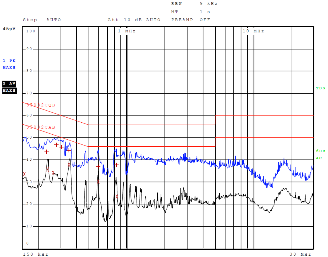
Figure 3 AC Line Conducted emissions of EUT line 1 Configuration #3
