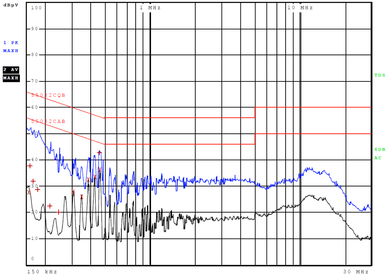
Figure 1 AC Line Conducted emissions of EUT line 1 Configuration #2
