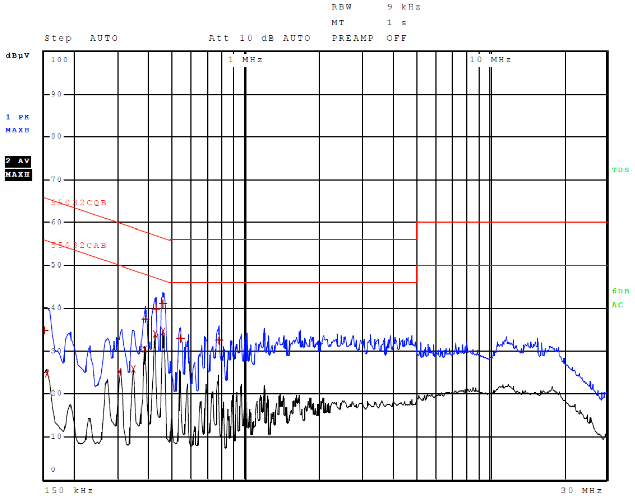
Figure 2 AC Line Conducted emissions of EUT line 2 Configuration #2
