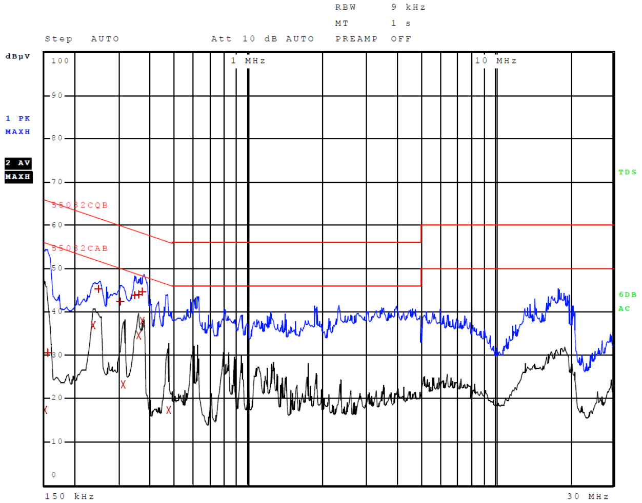
Figure 4 AC Line Conducted emissions of EUT line 2 Configuration #3
