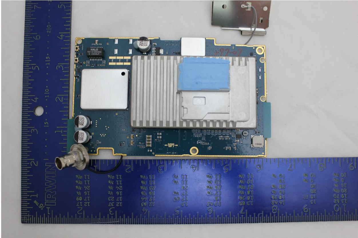
PCB Back with shields
