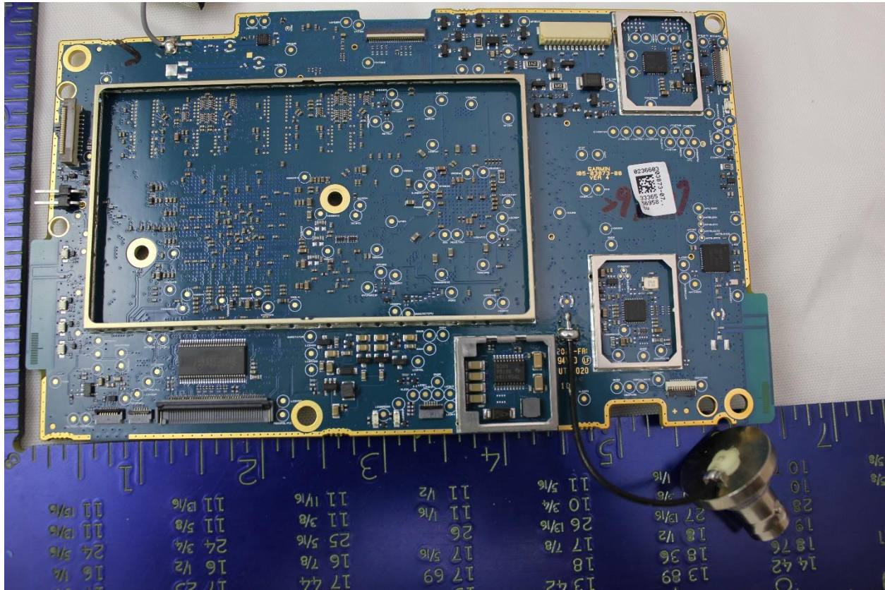
PCB Front without shields
