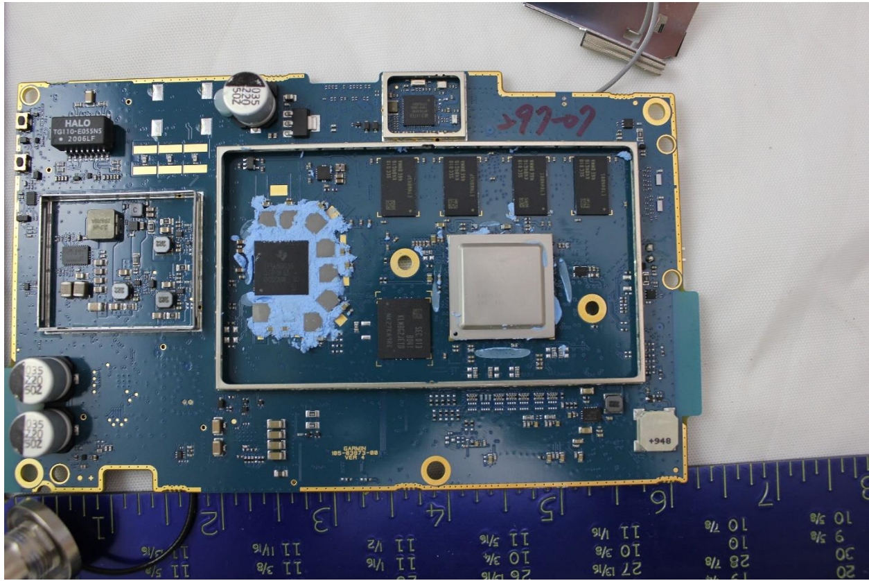
PCB Back without shields
