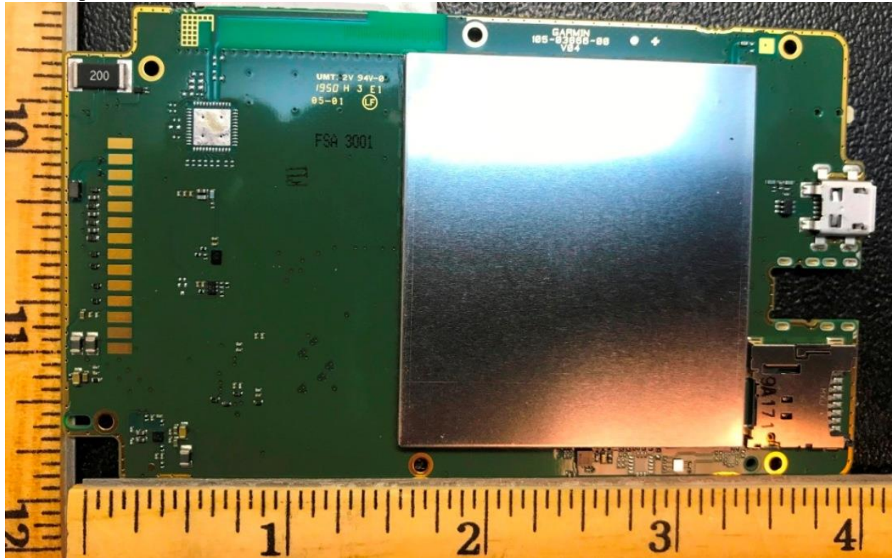
PCB Top With shields
