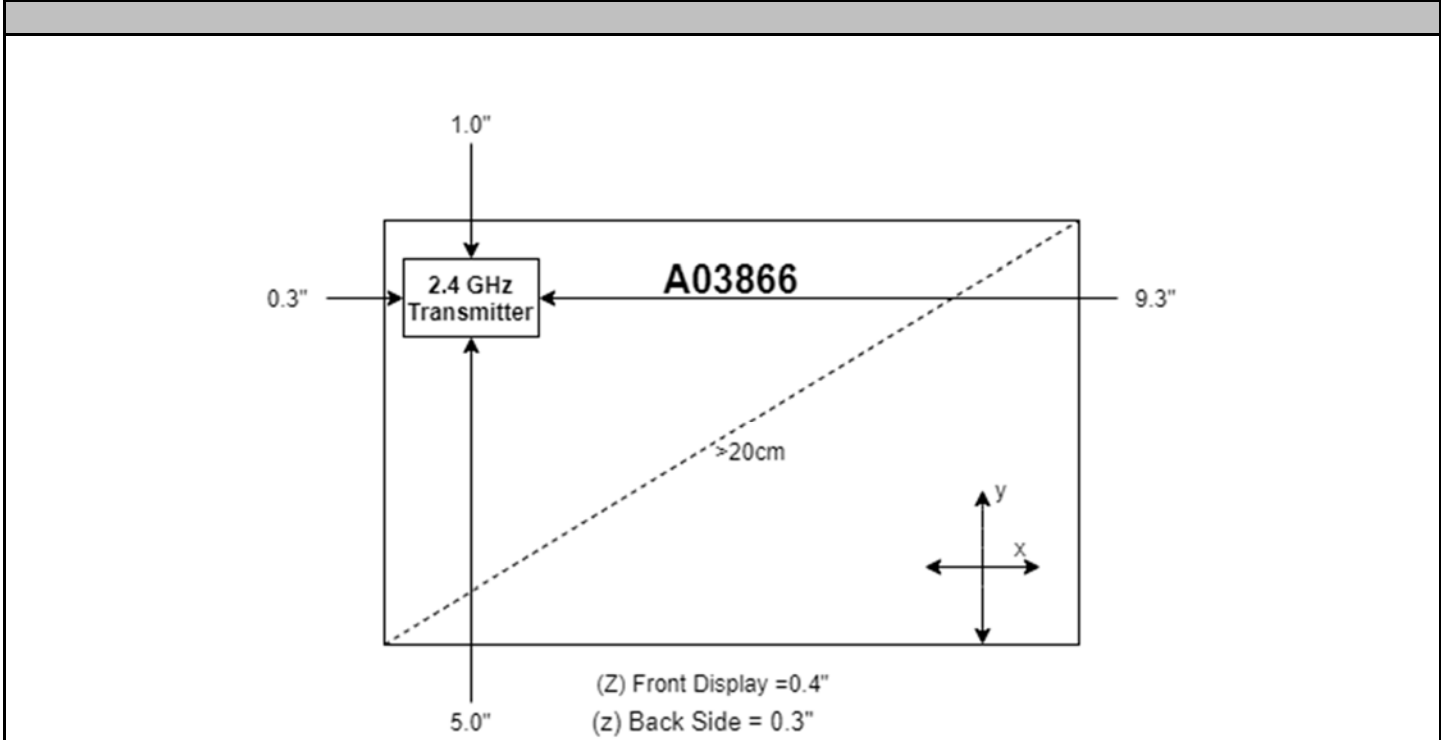
Figure A03866 (P/N:011-05116-XX) – 2.4GHz Antenna Location Diagram D6
