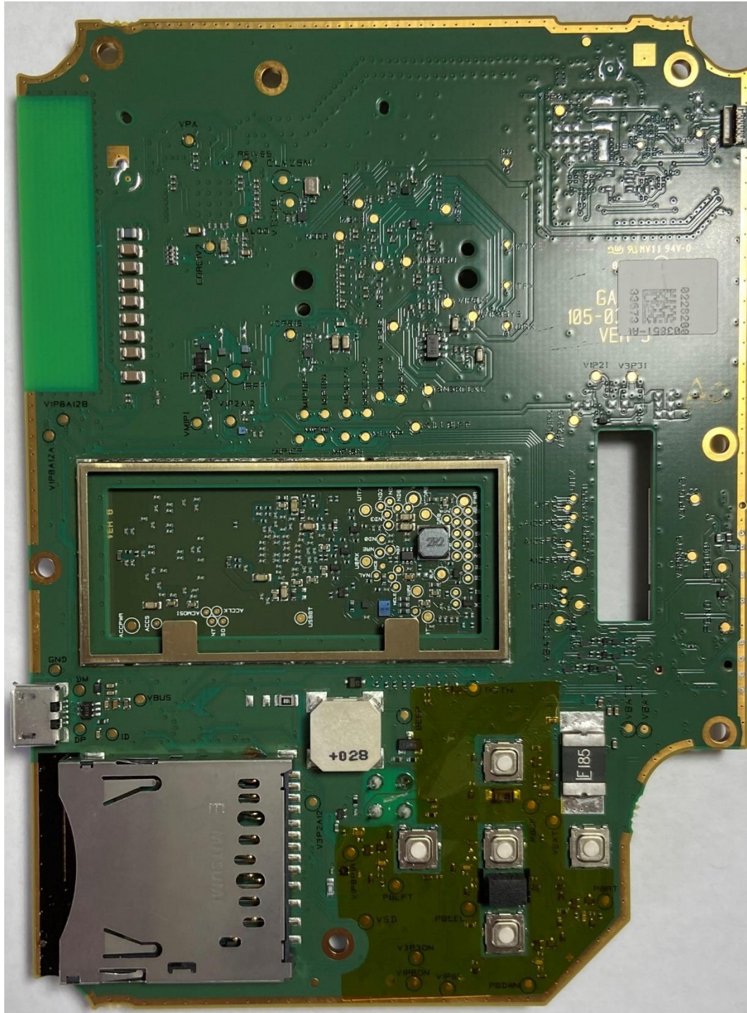
Bottom side without shield
