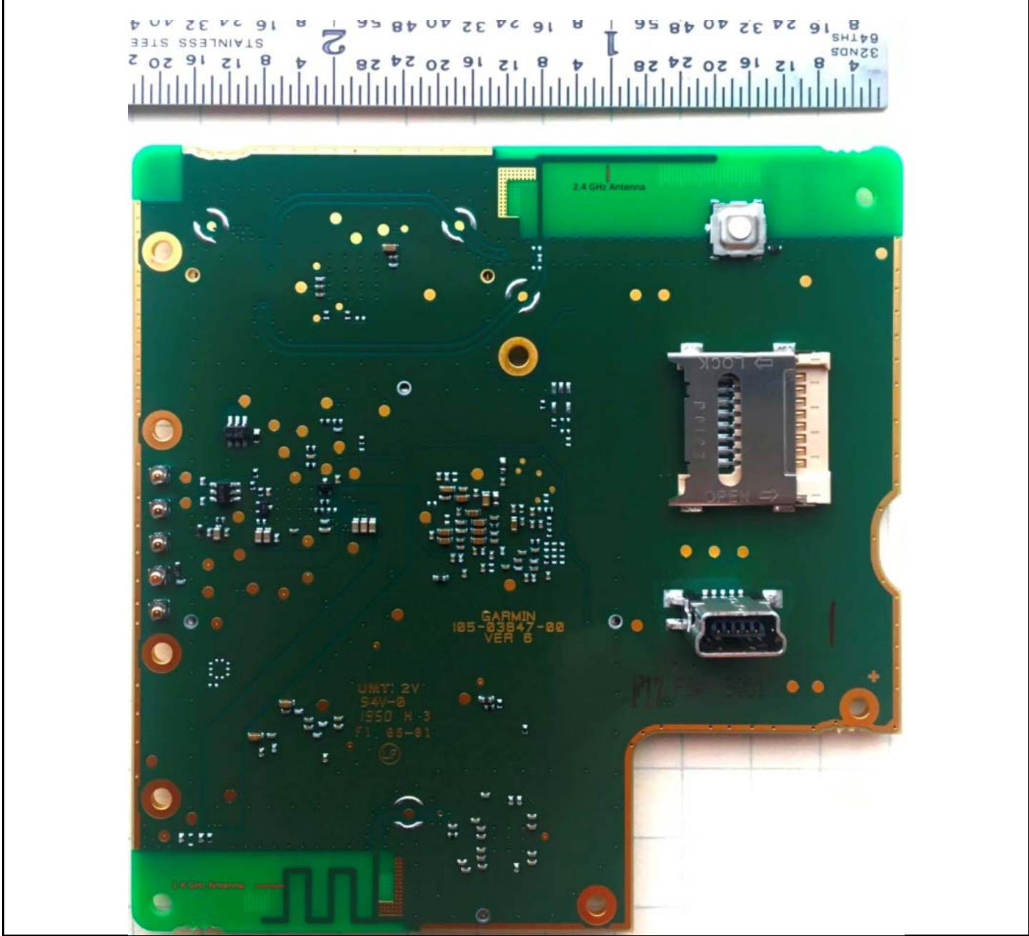
Figure A03847 – 2.4GHz Antenna Location PCB D5
