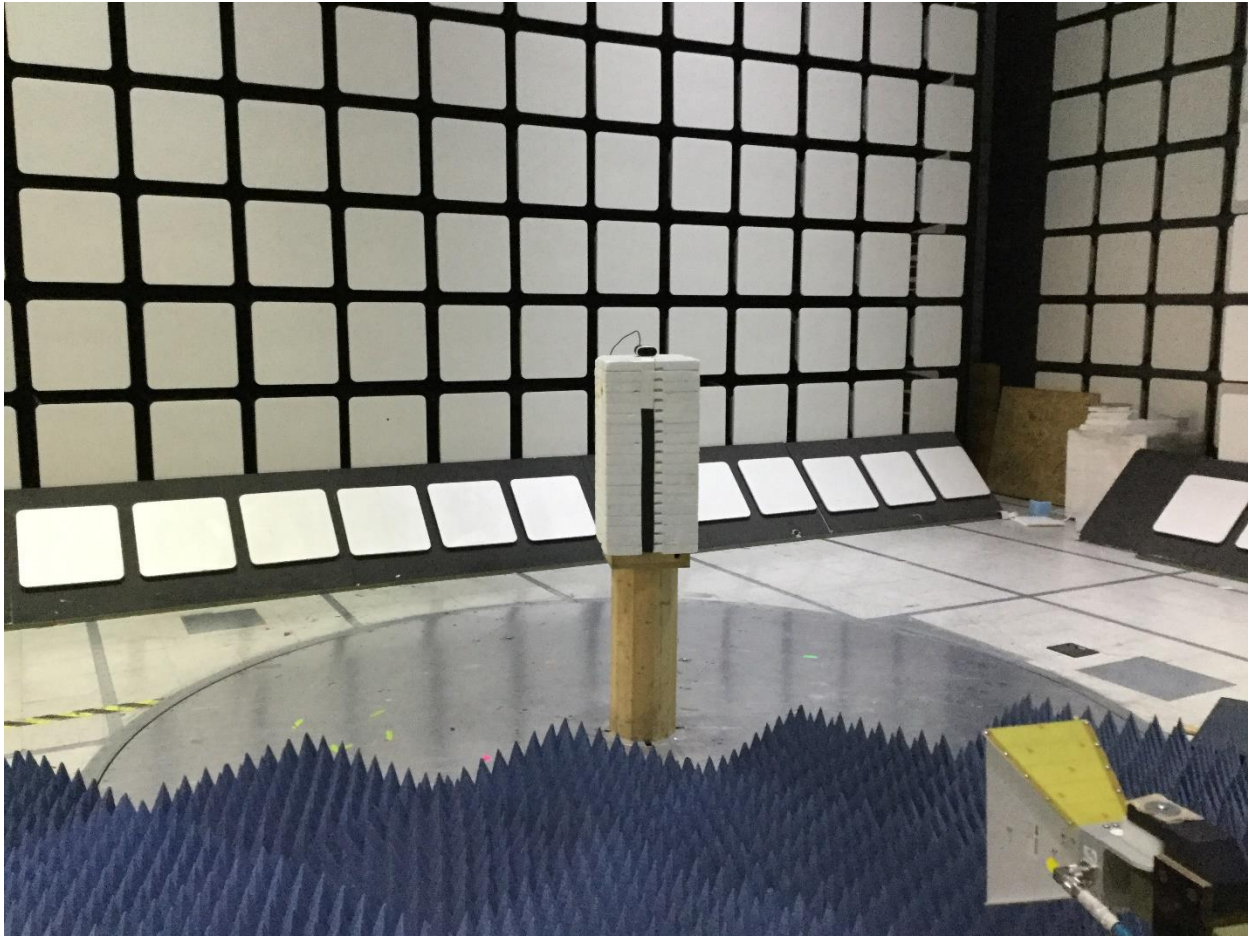
1 GHz – 25 GHz test setup
