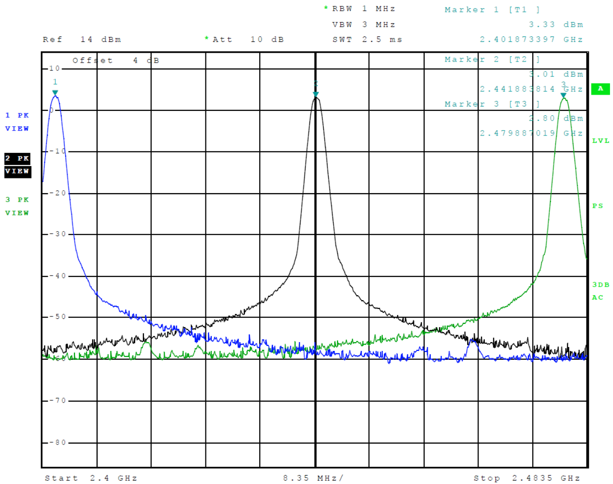
Figure 9 Plot of Transmitter Emissions Operation in 2402-2480 MHz Mode 2 (GMSK)
