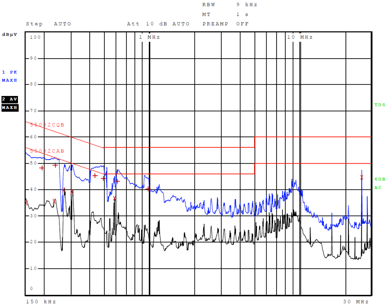
Figure 4 AC Line Conducted emissions of EUT line 2 Configuration #3, (EUT – CPU)
