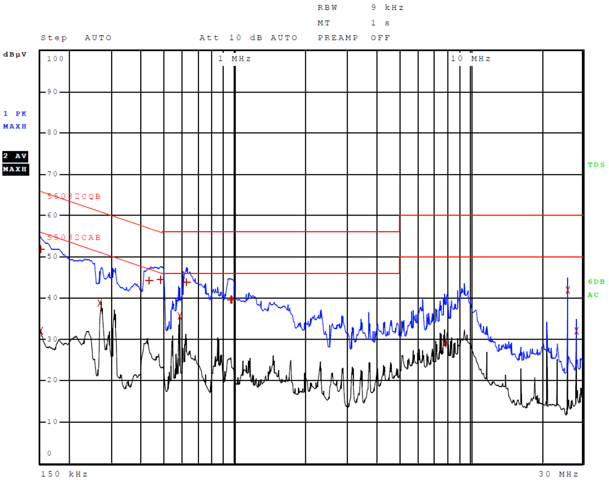
Figure 3 AC Line Conducted emissions of EUT line 1 Configuration #3, (EUT – CPU)
