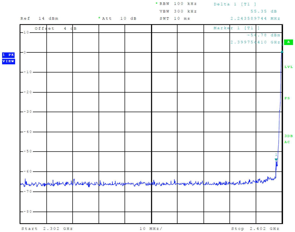
Figure 5 Plot of Transmitter Emissions Low Band Edge Mode 1 BLE (GMSK)
