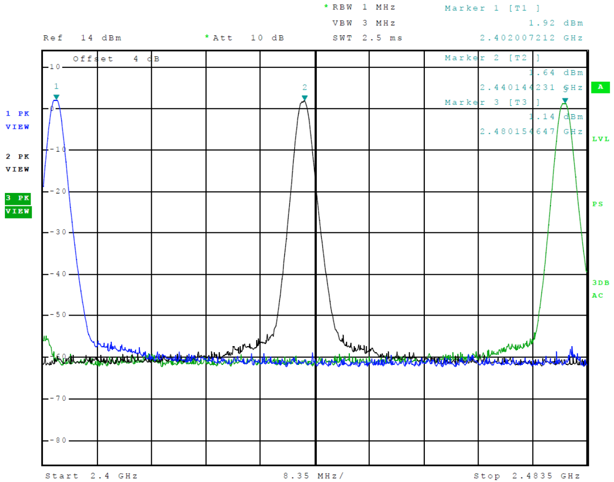
Figure 1 Plot of Transmitter Operation in 2402-2480 MHz Mode 1 BLE (GMSK)
