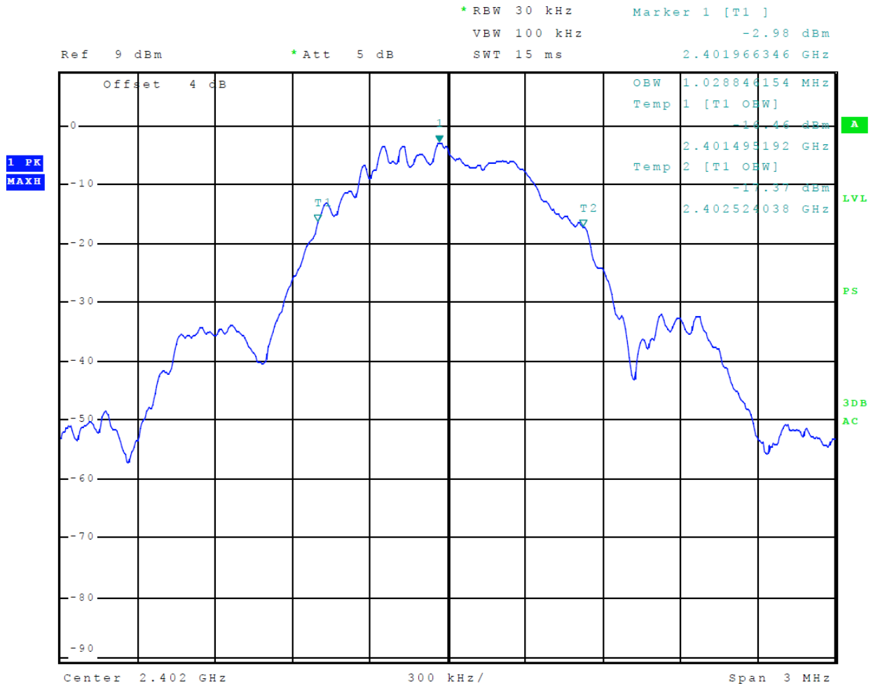
Figure 13 Plot of 99% Occupied Bandwidth Mode 1 BLE (GMSK)
