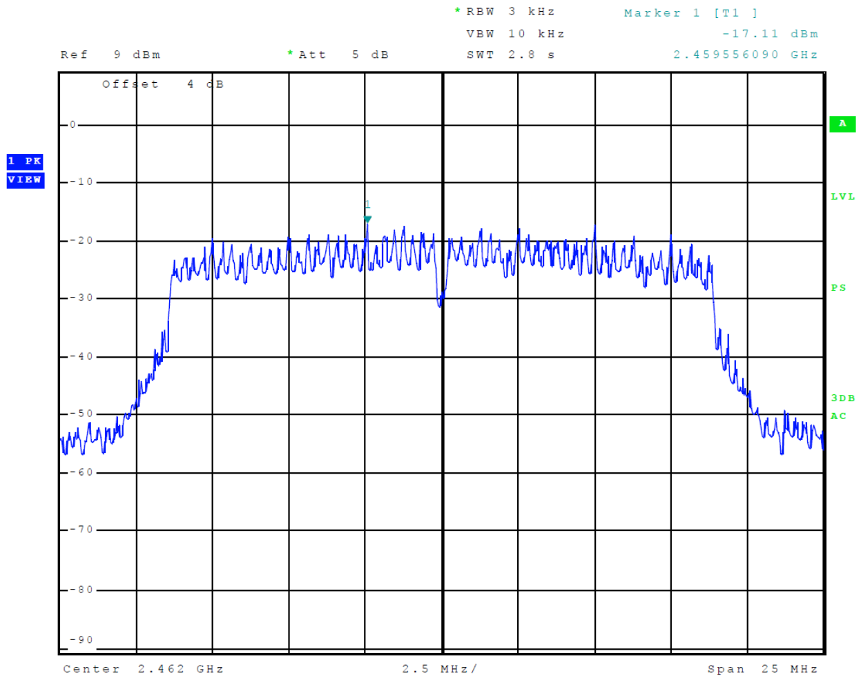
Figure 24 Plot of Transmitter Power Spectral Density Mode 4 802.11n
