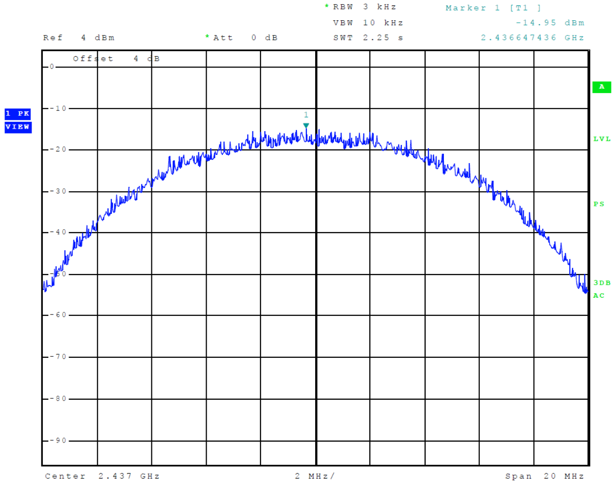
Figure 22 Plot of Transmitter Power Spectral Density Mode 2 802.11b
