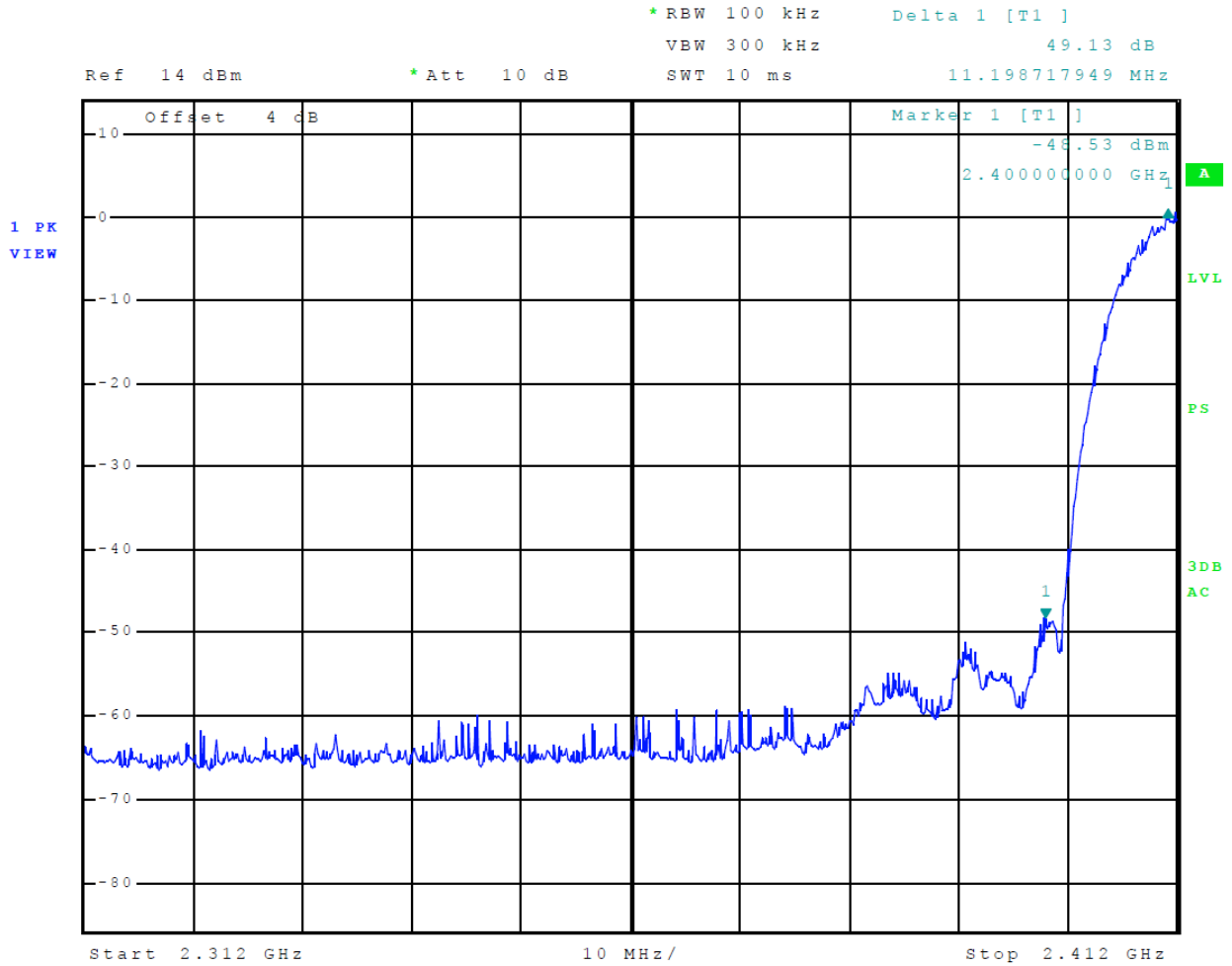
Figure 6 Plot of Transmitter Emissions Low Band Edge Mode 2 802.11b
