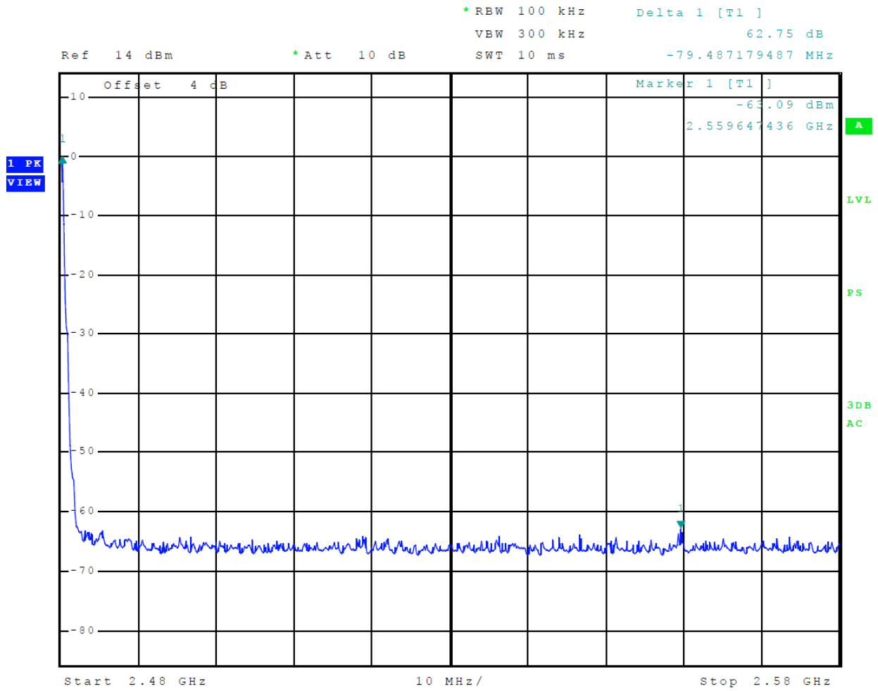
Figure 9 Plot of Transmitter Emissions High Band Edge Mode 1 BLE (GMSK)
