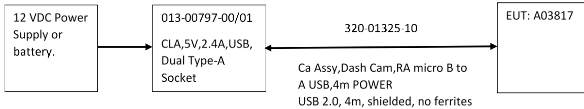
Configuration 1, Dual CLA with 4.0m USB cable (power only), Block Diagram.
