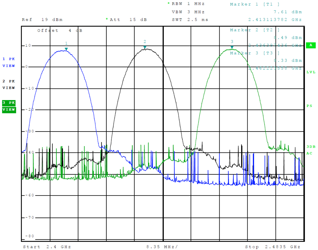
Figure 2 Plot of Transmitter Operation in 2402-2480 MHz Mode 2 802.11b
