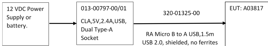
Configuration 2, Dual CLA with 1.5 m USB cable, Block Diagram.
