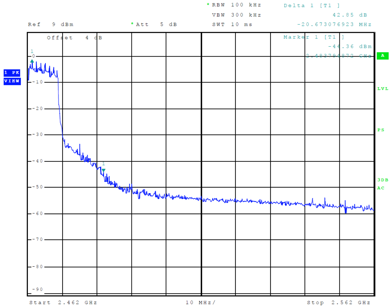
Figure 12 Plot of Transmitter Emissions High Band Edge Mode 4 802.11n
