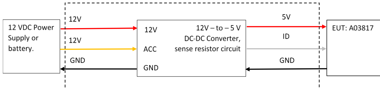
Configuration 3, Parking Mode Cable (car running), Block Diagram.
