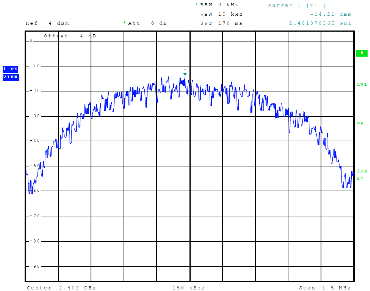
Figure 21 Plot of Transmitter Power Spectral Density Mode 1 BLE (GMSK)
