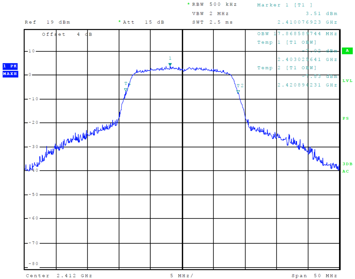
Figure 15 Plot of 99% Occupied Bandwidth Mode 3 802.11g
