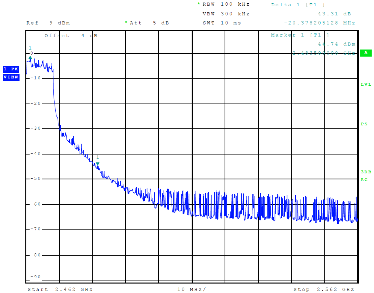
Figure 11 Plot of Transmitter Emissions High Band Edge Mode 3 802.11g
