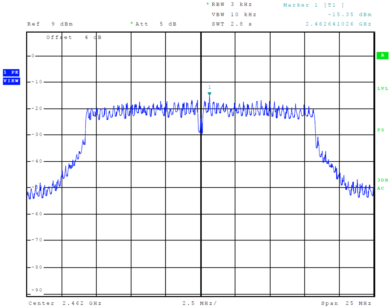
Figure 23 Plot of Transmitter Power Spectral Density Mode 3 802.11g
