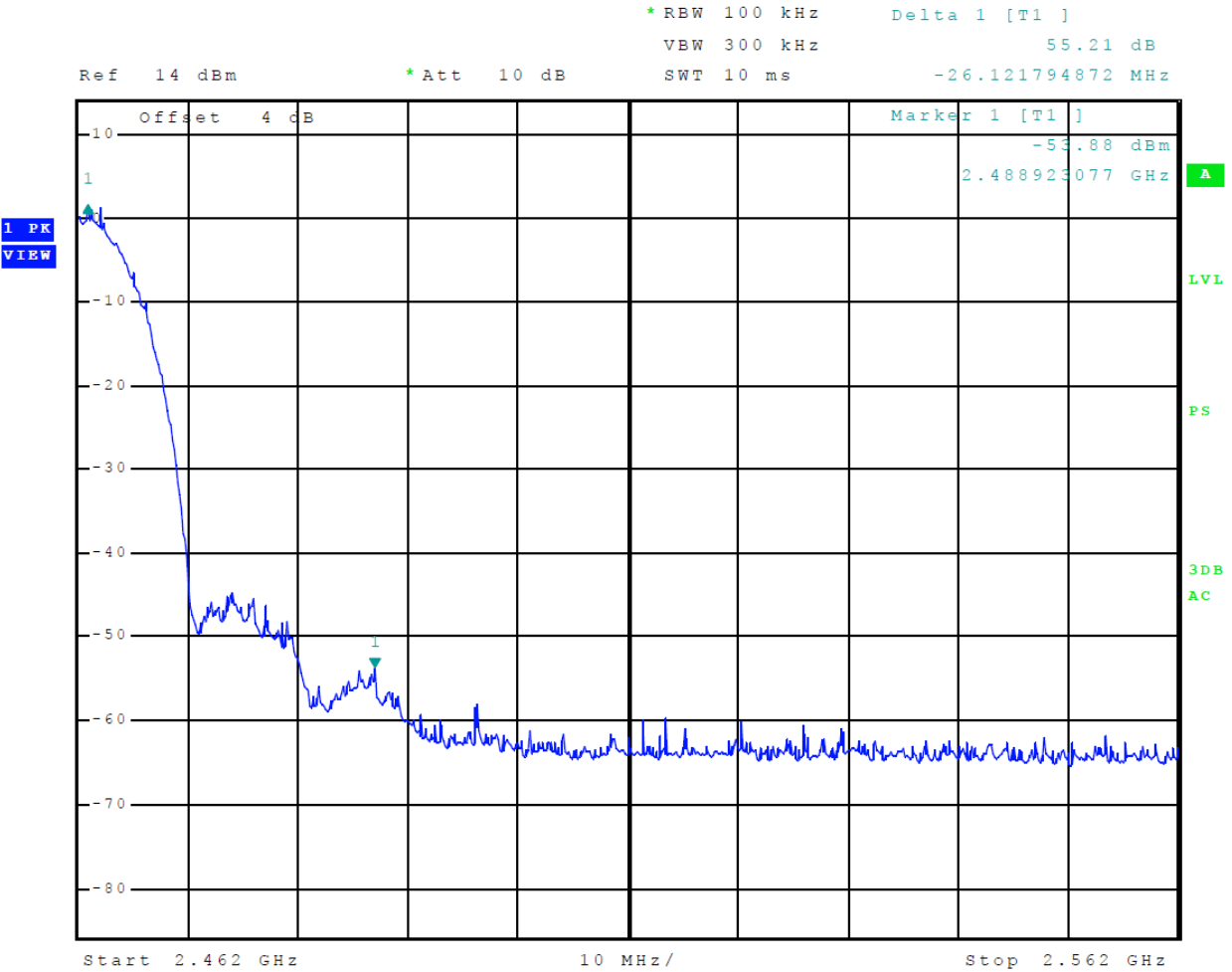
Figure 10 Plot of Transmitter Emissions High Band Edge Mode 2 802.11b
