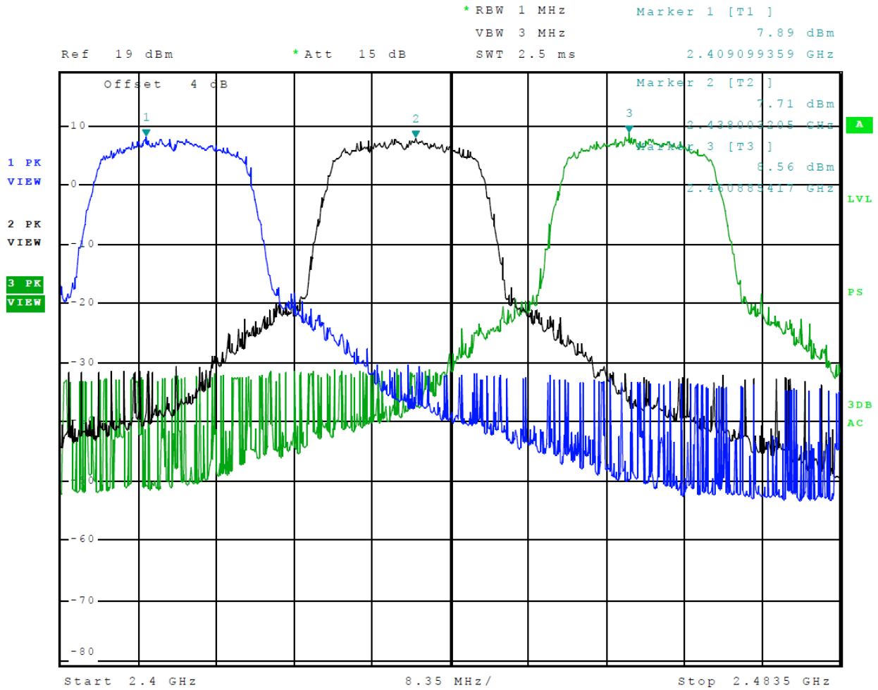
Figure 3 Plot of Transmitter Operation in 2402-2480 MHz Mode 3 802.11g
