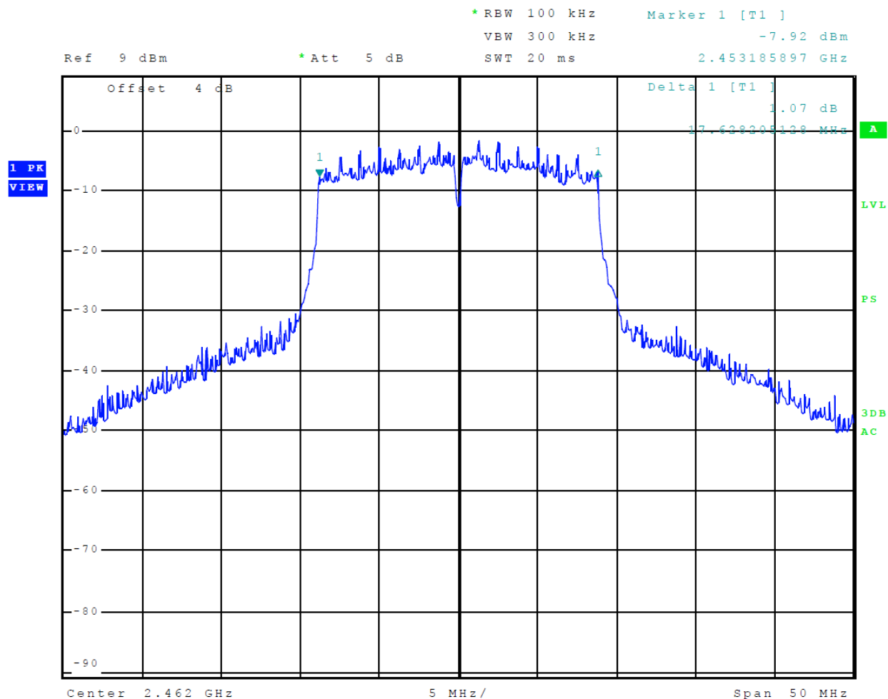
Figure 20 Plot of 6-dB Occupied Bandwidth Mode 4 802.11n
