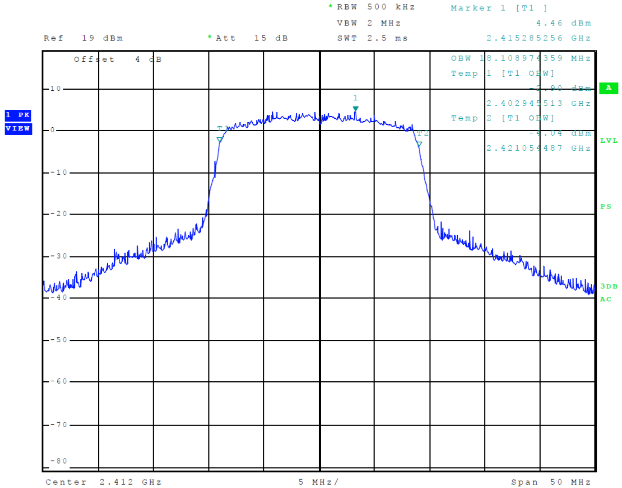
Figure 16 Plot of 99% Occupied Bandwidth Mode 4 802.11n
