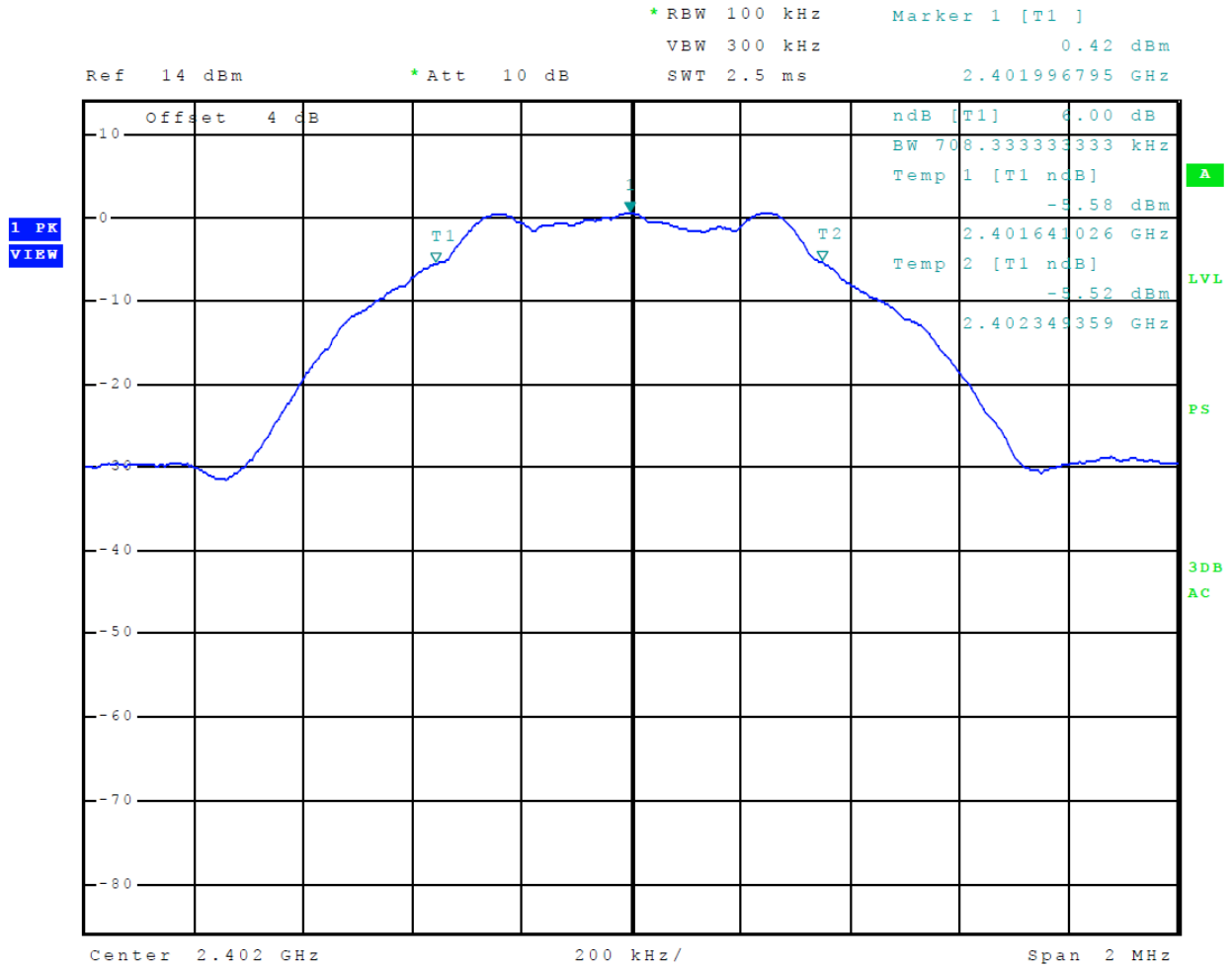
Figure 17 Plot of 6-dB Occupied Bandwidth Mode 1 BLE (GMSK)
