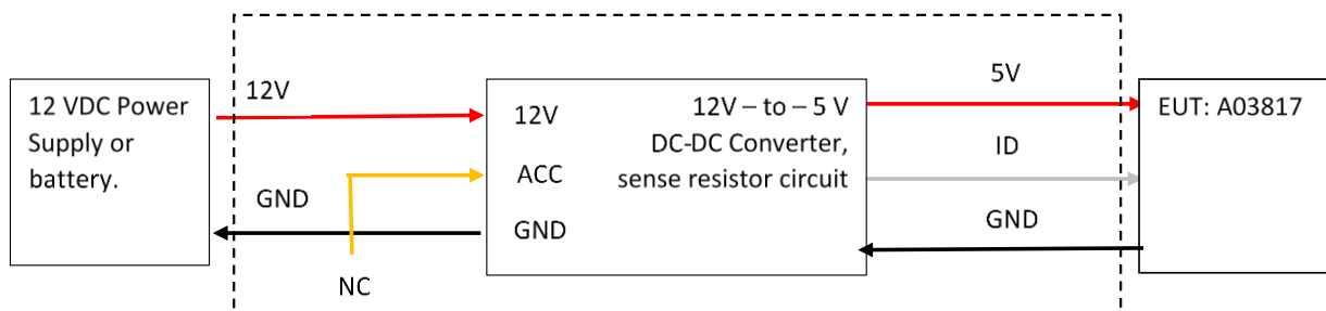
Configuration 4, Parking Mode Cable (car off), Block Diagram. Testing Not Required.
