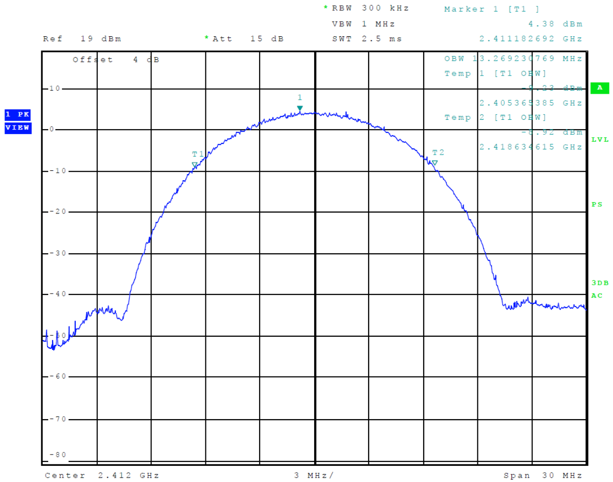
Figure 14 Plot of 99% Occupied Bandwidth Mode 2 802.11b
