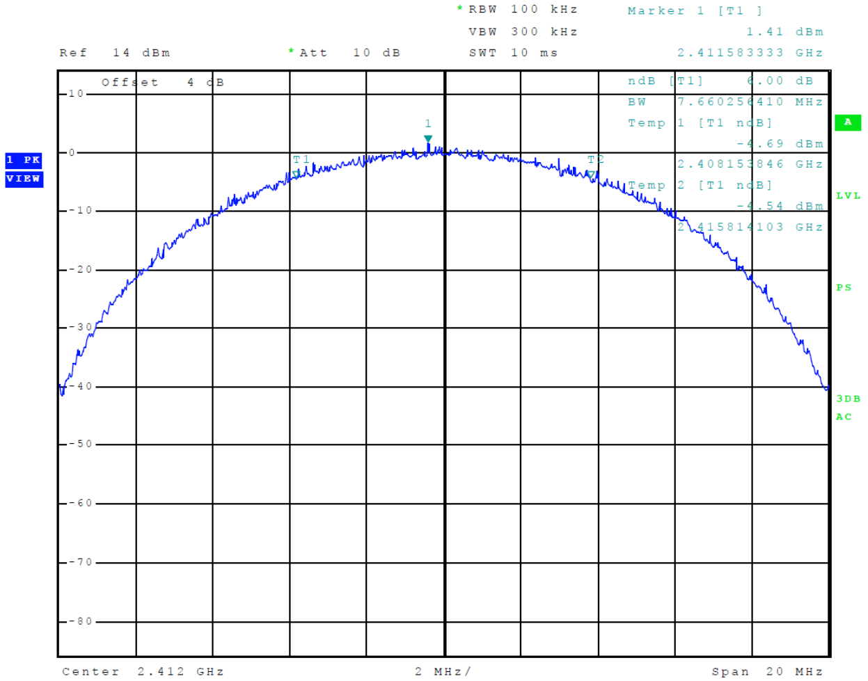
Figure 18 Plot of 6-dB Occupied Bandwidth Mode 2 802.11b
