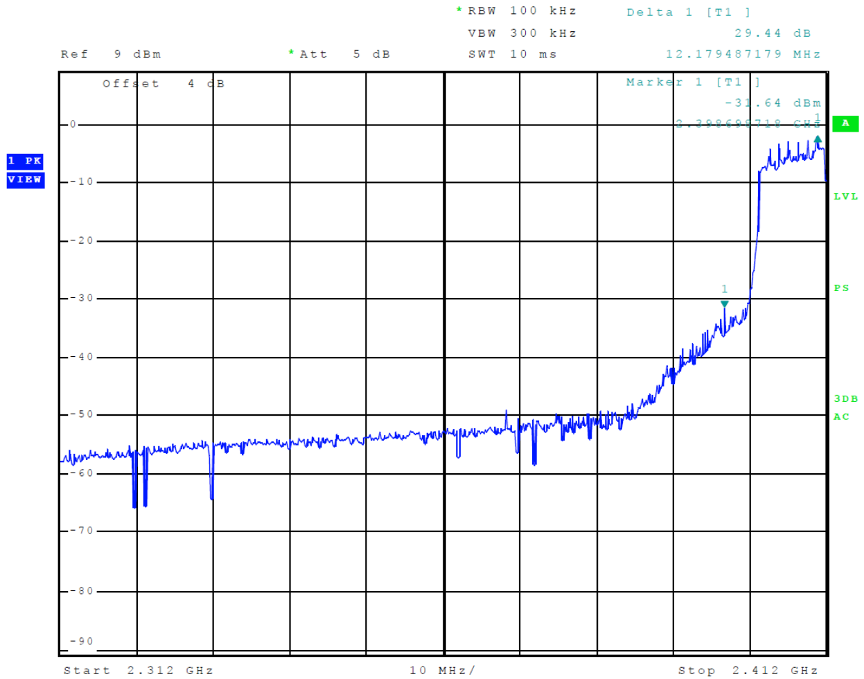
Figure 8 Plot of Transmitter Emissions Low Band Edge Mode 4 802.11n
