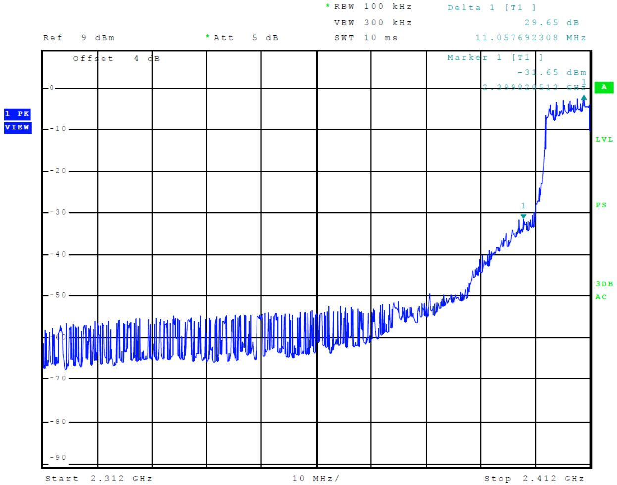
Figure 7 Plot of Transmitter Emissions Low Band Edge Mode 3 802.11g
