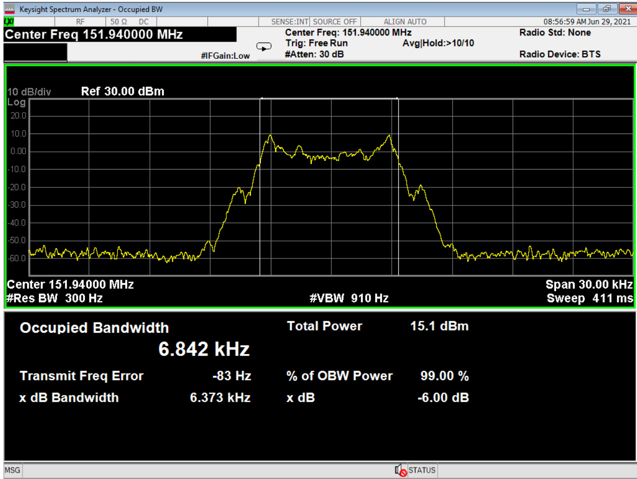
Figure 11 - Bandwidth, 151.940 MHz
