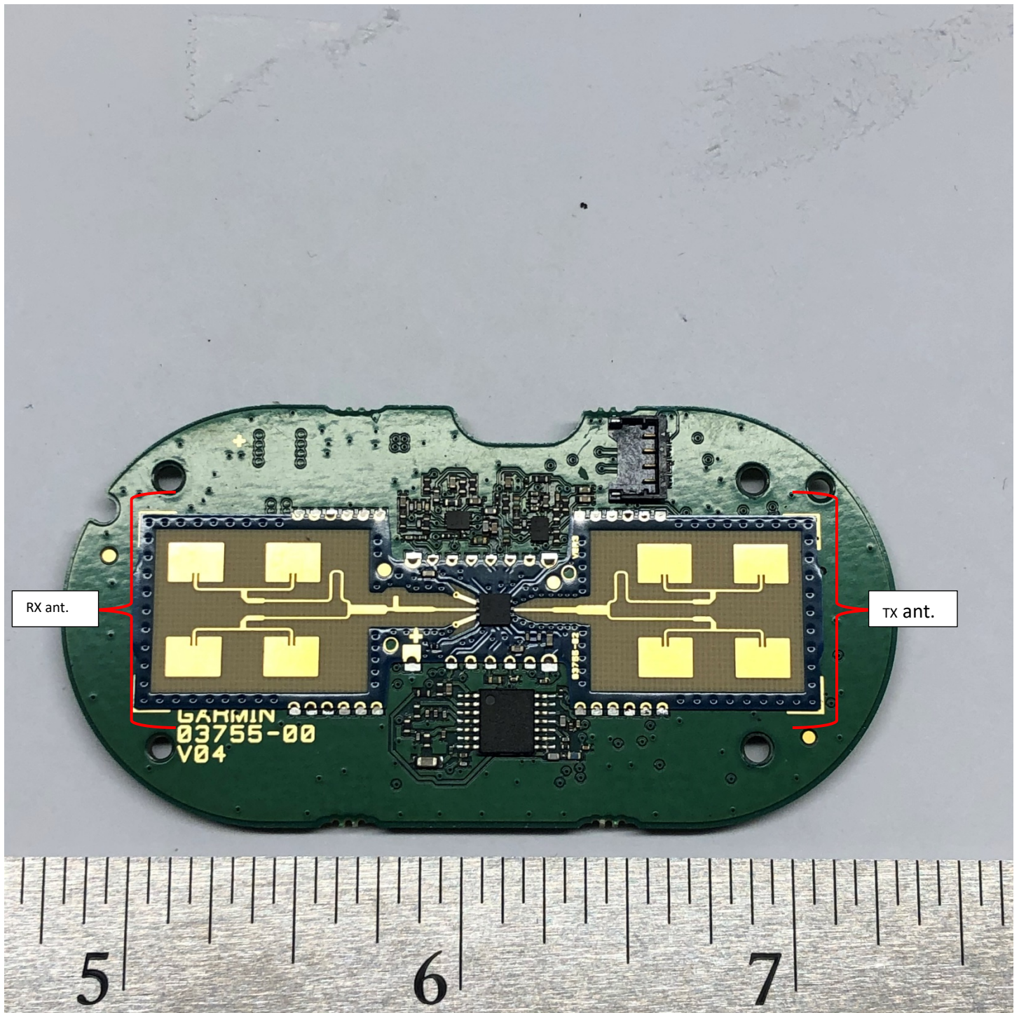
Figure 4- PCB Front
