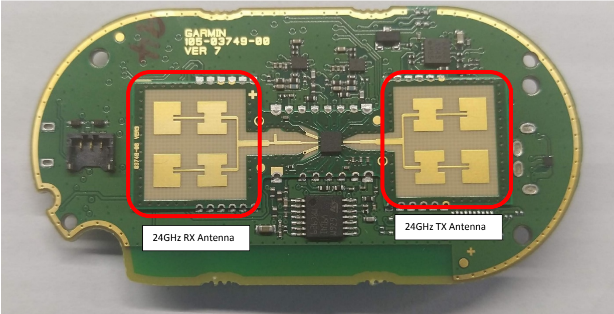
Figure 6 - PCB Front
