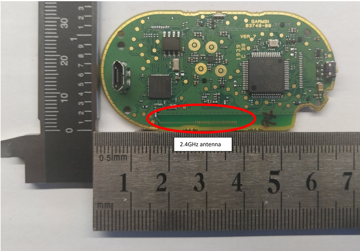
Figure 5 - PCB Rear
