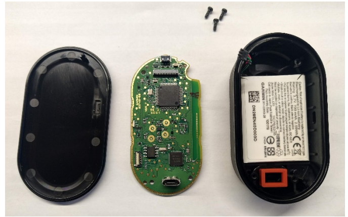
Figure 4 - EUT Internal
