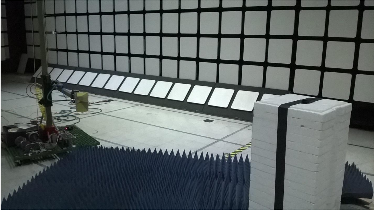
Figure 1 - Radiated Emissions Test Setup, 1 - 25 GHz (EUT not shown. Photo intended to show equipment setup)
