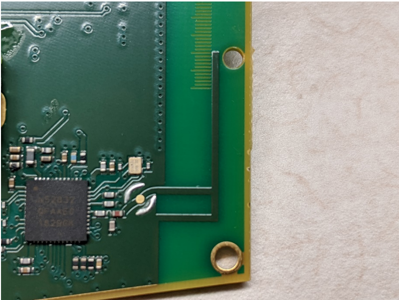
Figure 4 - Antenna
