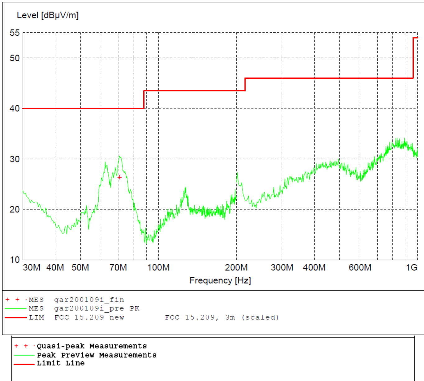
Figure 27 - Radiated Emissions Plot, 3EDR
