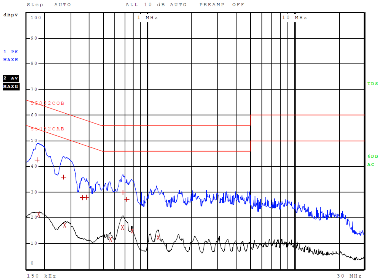
Figure 4 AC Line Conducted emissions of EUT line 2 (#3, EUT – 362-00087-00)
