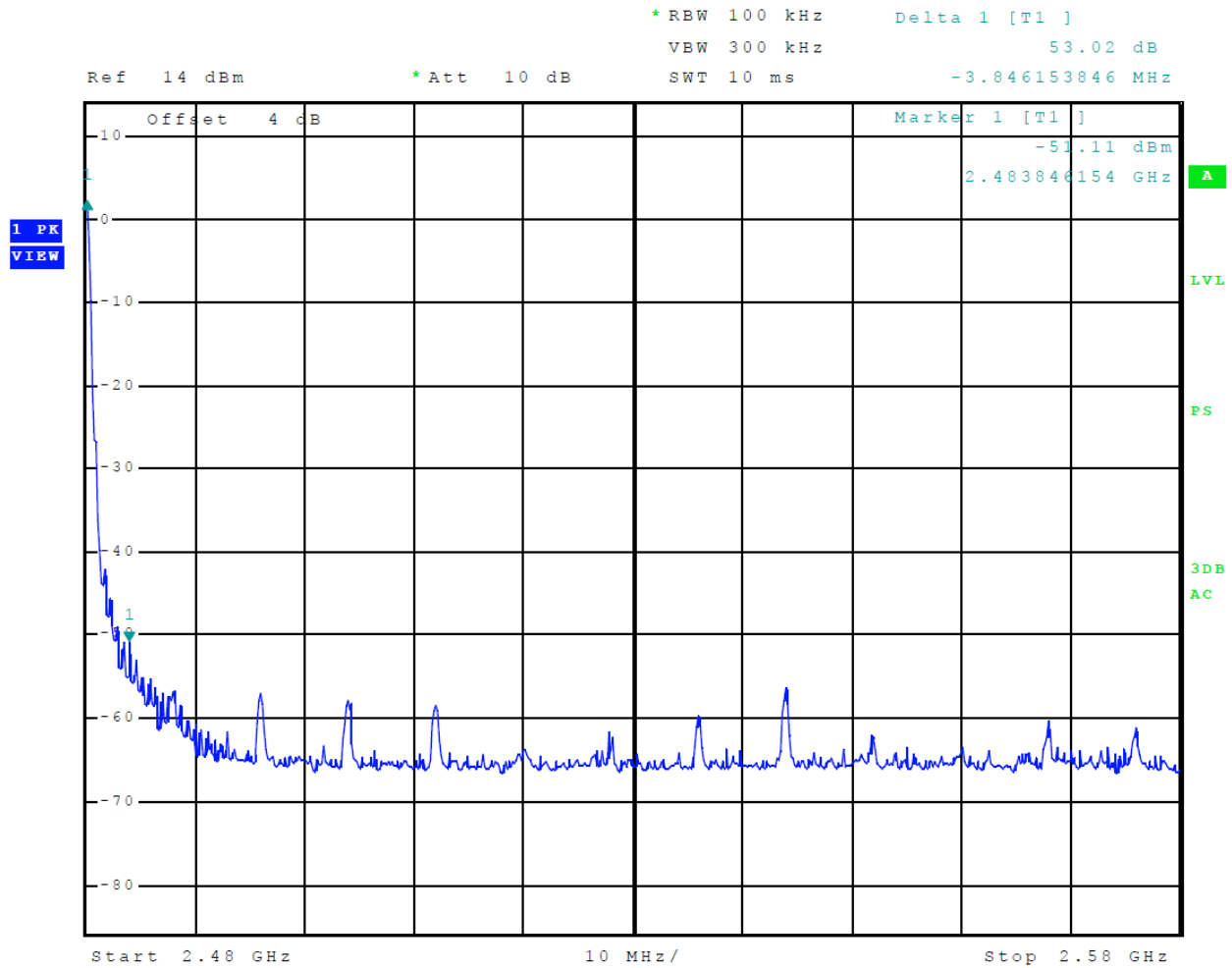
Figure 12 Plot of Transmitter Emissions High Band Edge Mode 2 BLE (GMSK)
