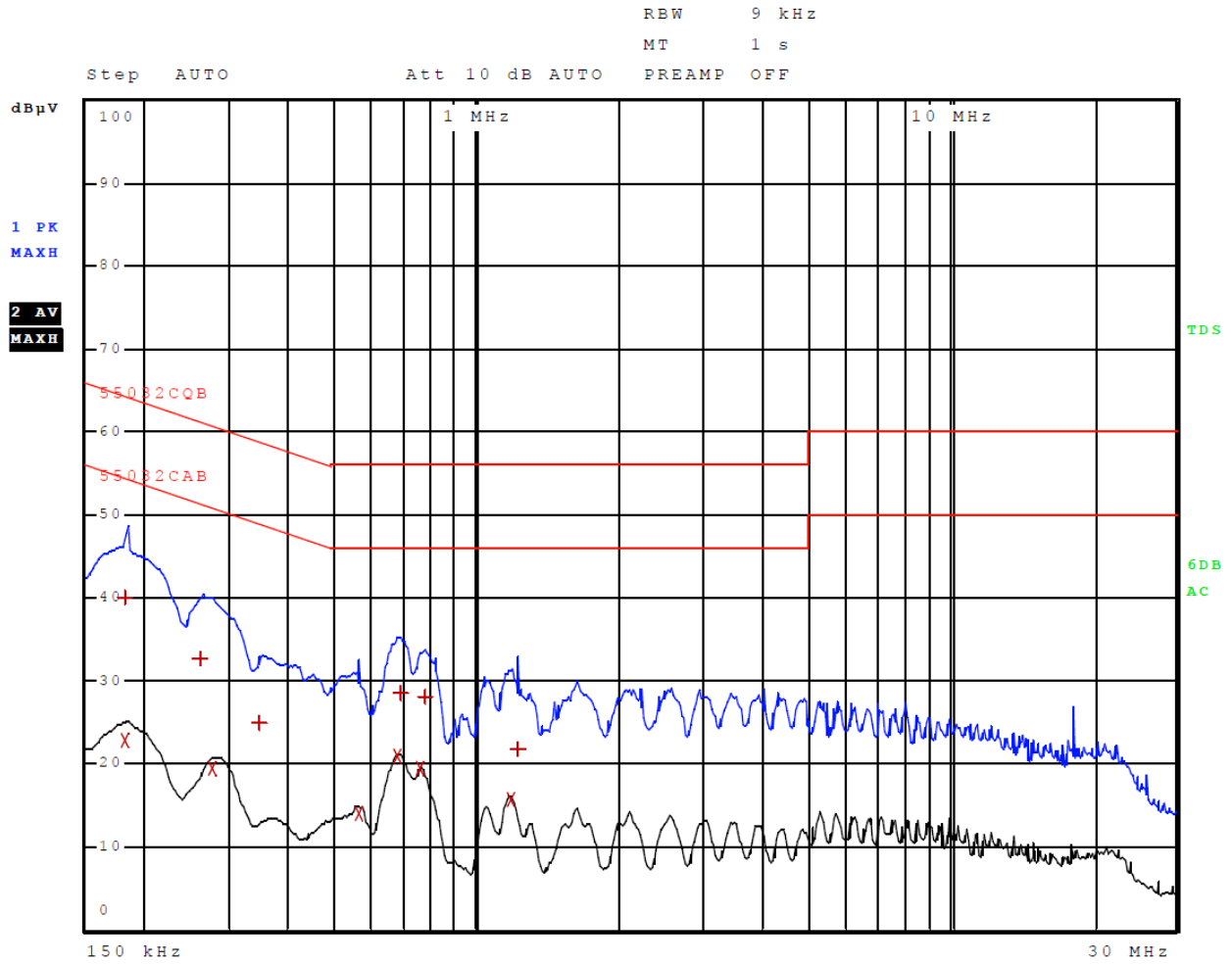
Figure 3 AC Line Conducted emissions of EUT line 1 (#3, EUT – 362-00087-00)
