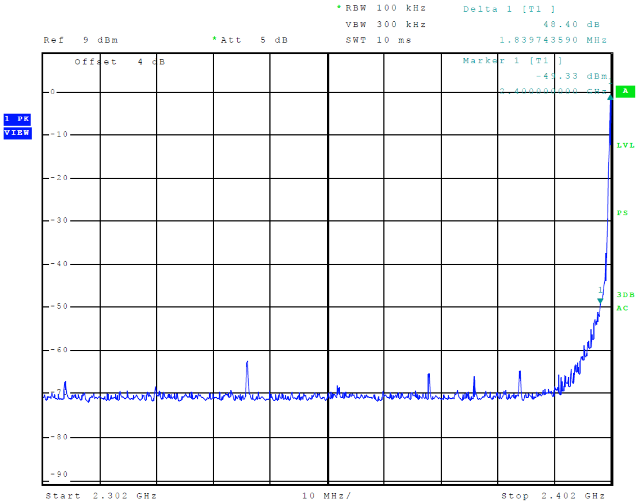
Figure 9 Plot of Transmitter Emissions Low Band Edge Mode 1 ANT (GFSK)
