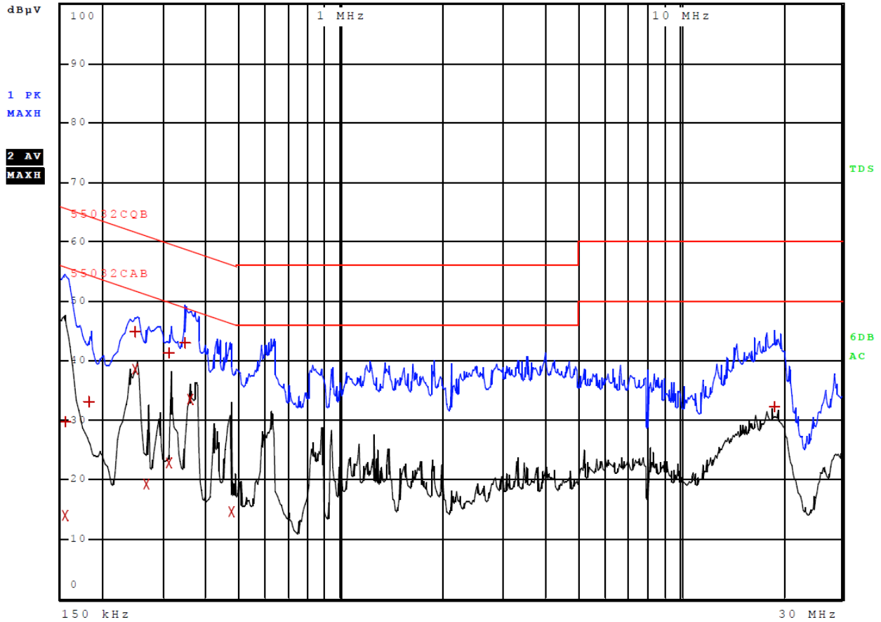
Figure 2 AC Line Conducted emissions of EUT line 2 (#2, EUT – Computer)
