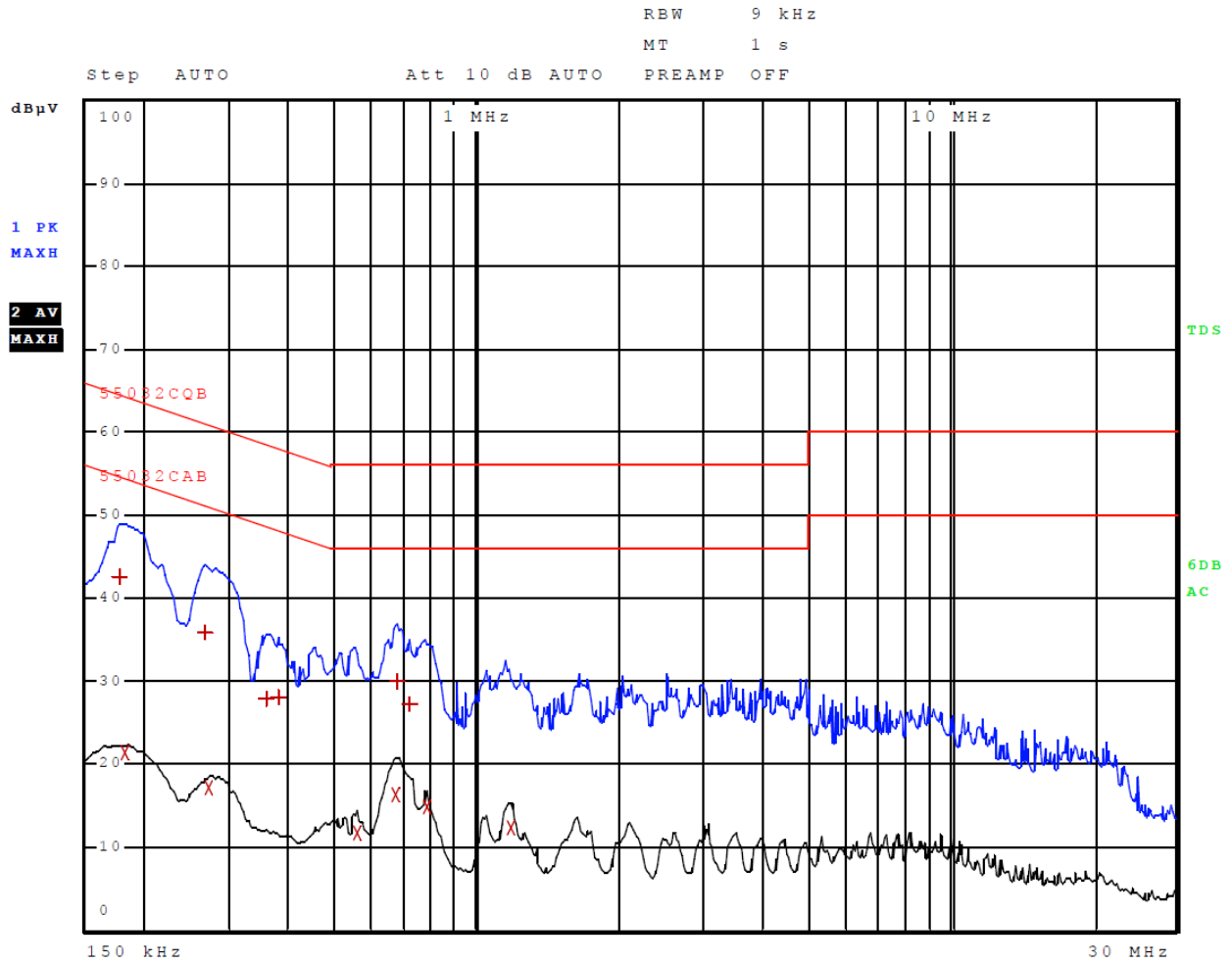
Figure 4 AC Line Conducted emissions of EUT line 2 (#3, EUT – 362-00087-00)
