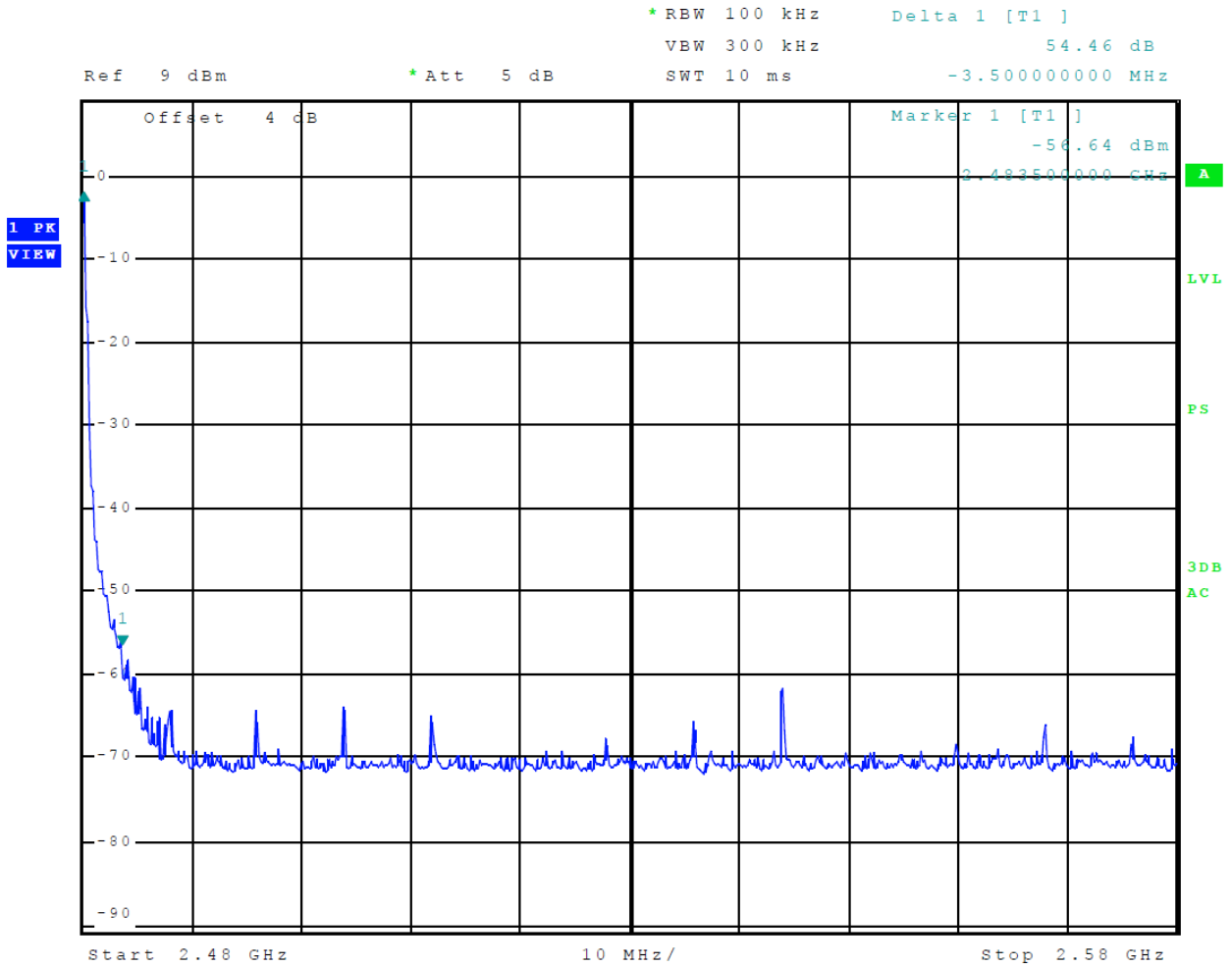
Figure 11 Plot of Transmitter Emissions High Band Edge Mode 1 ANT (GFSK)
