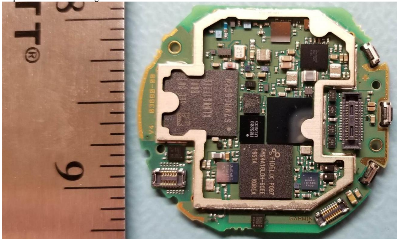
Top side PCB Shielding removed
