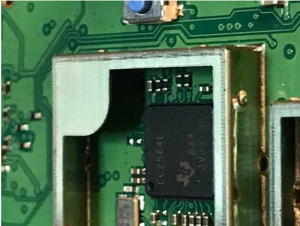
Bottom IC1
